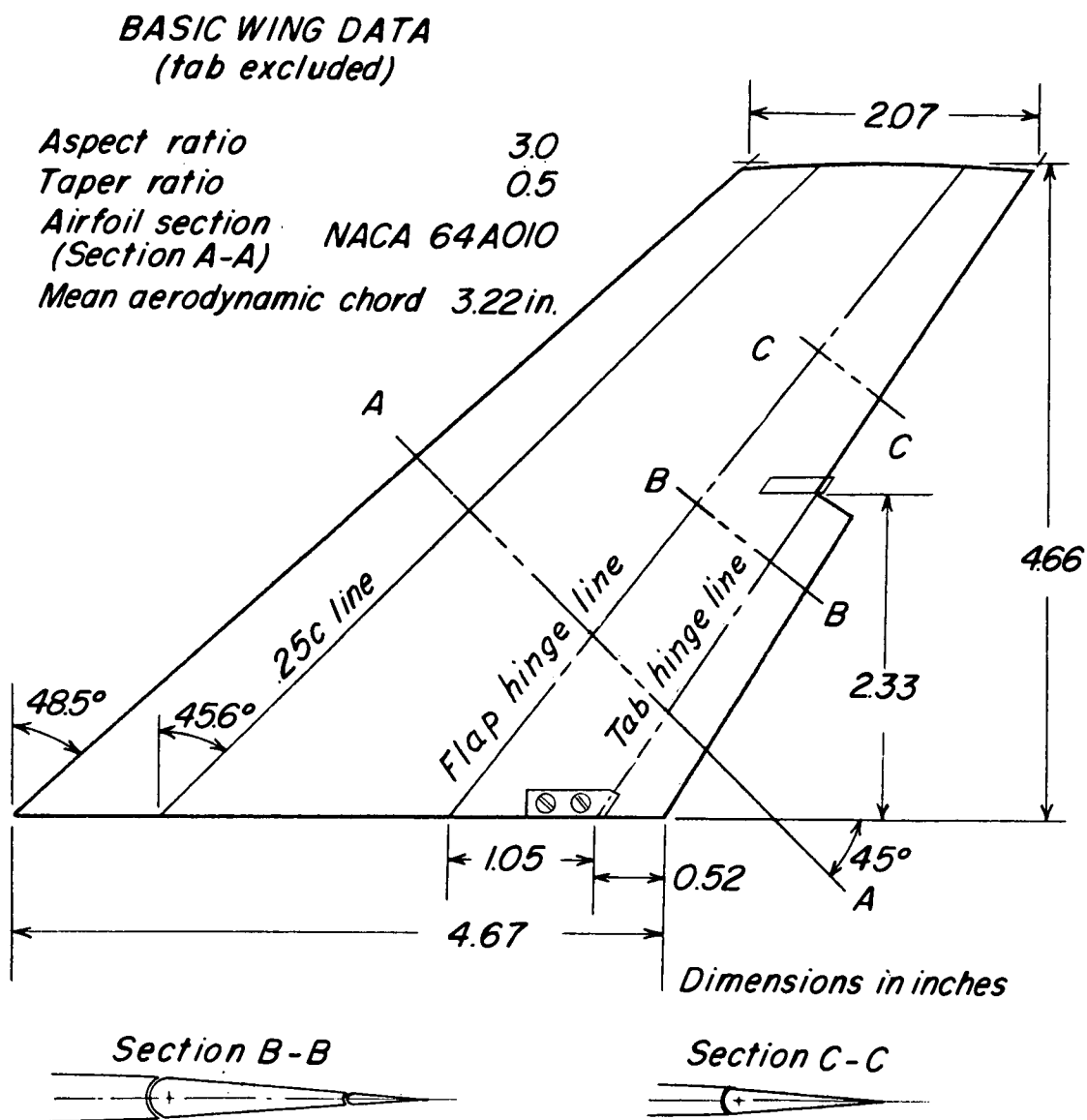
Figure 1.- Geometric characteristics of the model.
