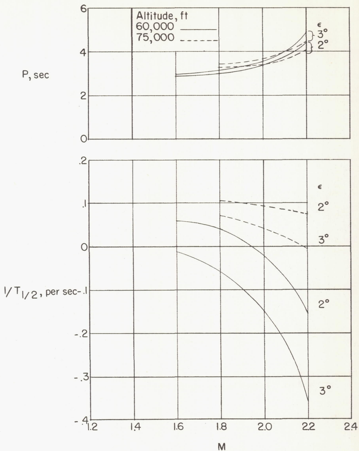
Figure 13.- Calculated period and damping for principal-axis inclination of 2^\circ and 3^\circ .
