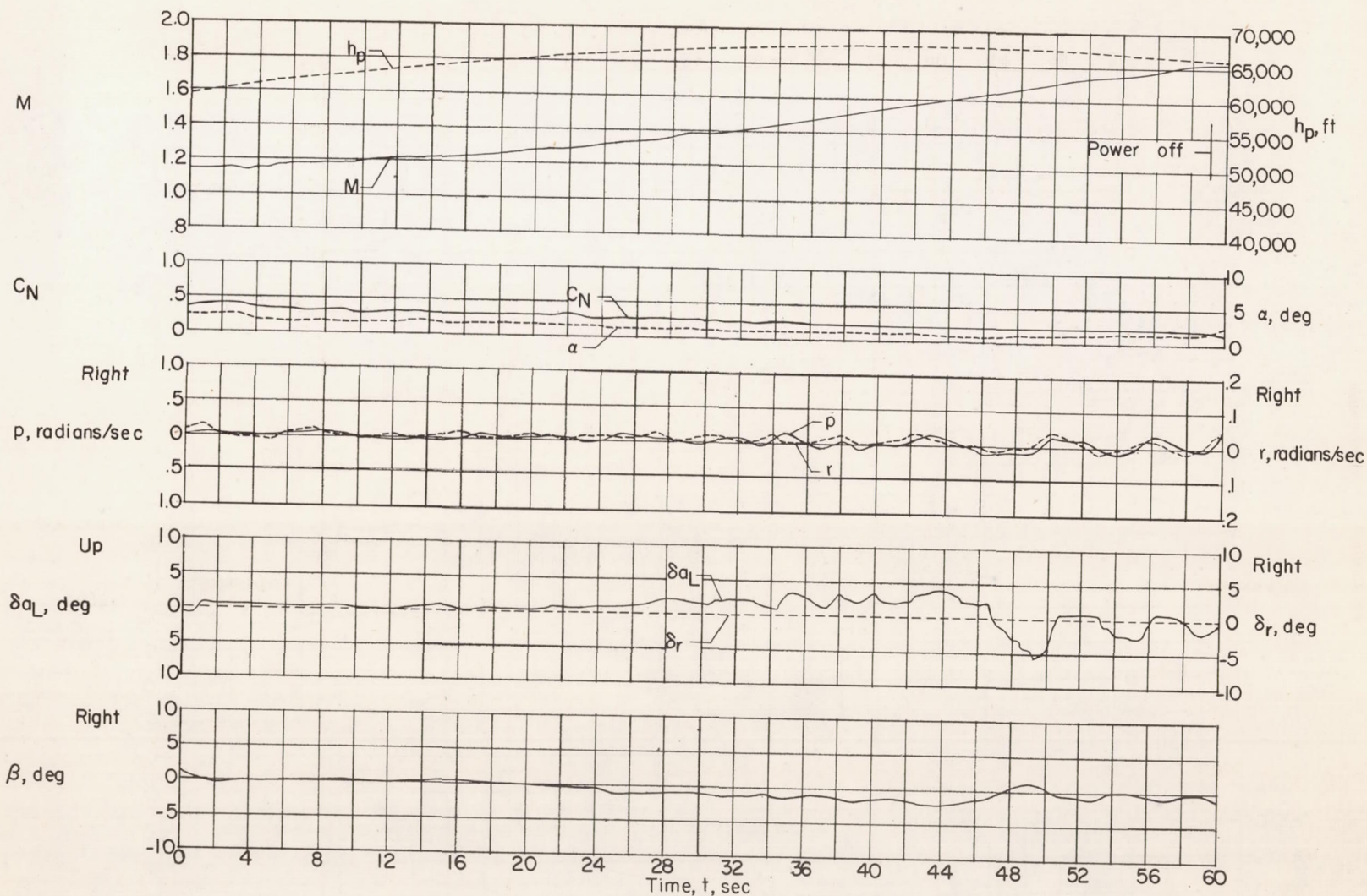
Figure 6.- Time history of data obtained during a straight flight at moderate angle of attack. Rudder locked.
