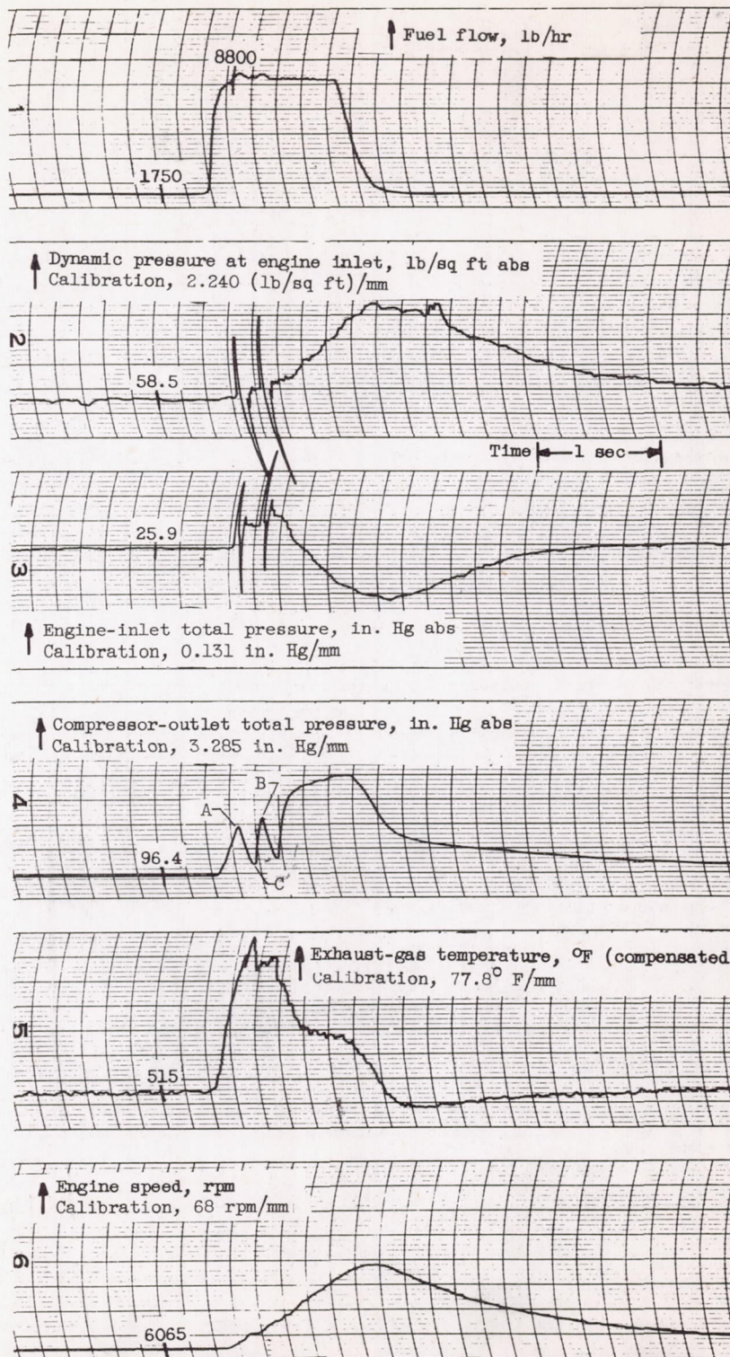
Figure 12. - Concluded. Oscillograph traces of performance parameters during engine acceleration. Inlet guide vanes open; flight Mach number, 0.8.
