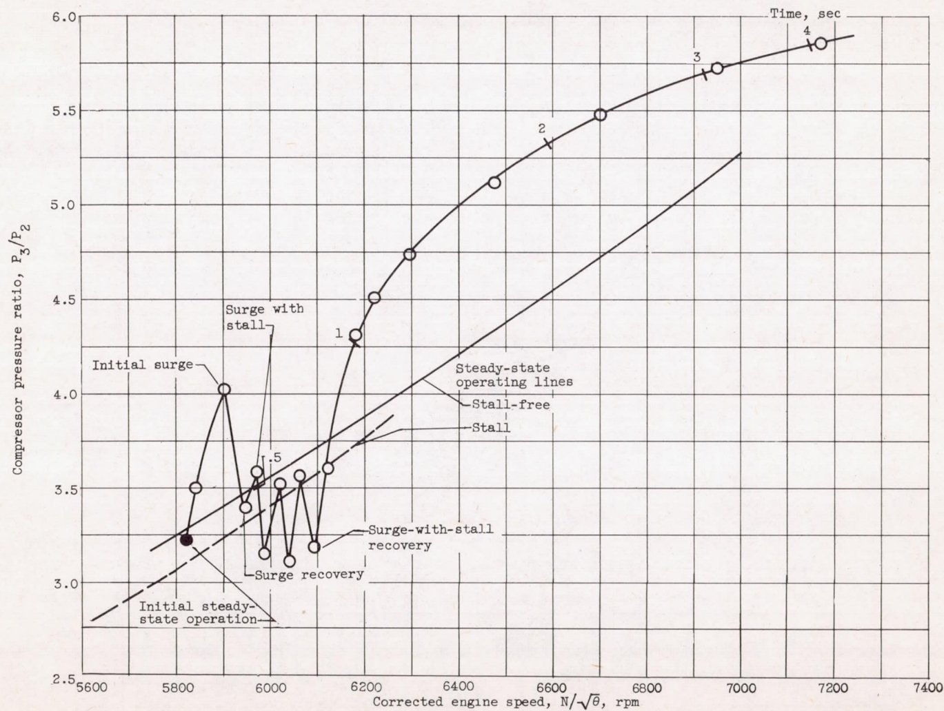
Figure 15. - Continued. Effects of acceleration with inlet guide vanes open. Altitude, 35,000 feet; flight Mach number, 0.8.
