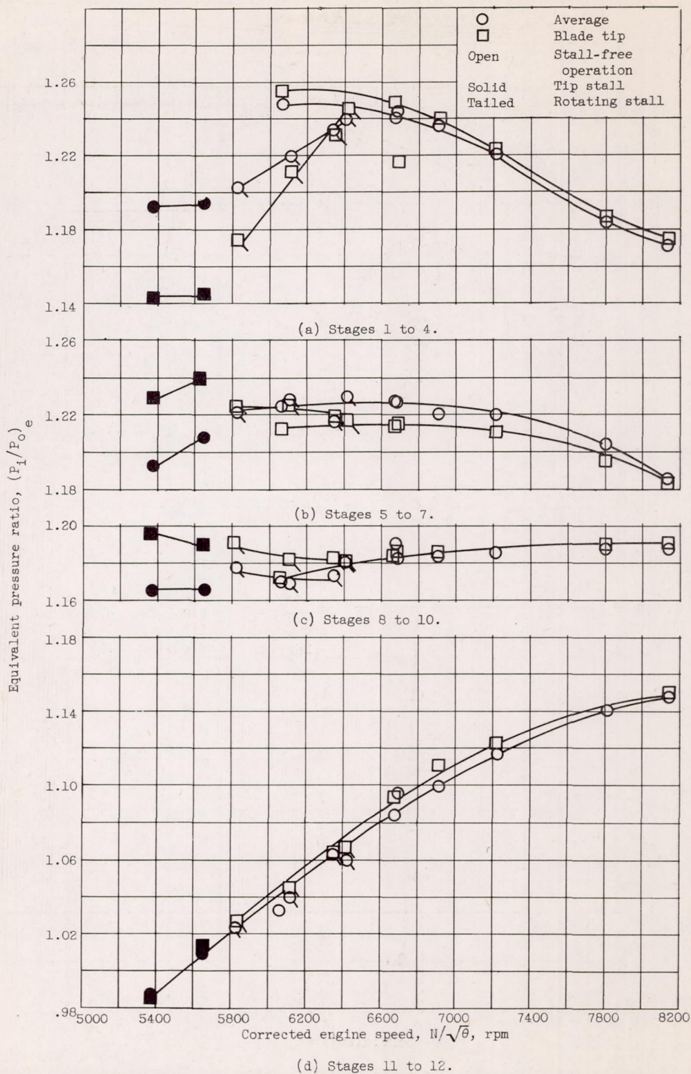
Figure 9. - Variation of equivalent pressure ratio with corrected engine speed for several groups of compressor stages. Inlet guide vanes open.
