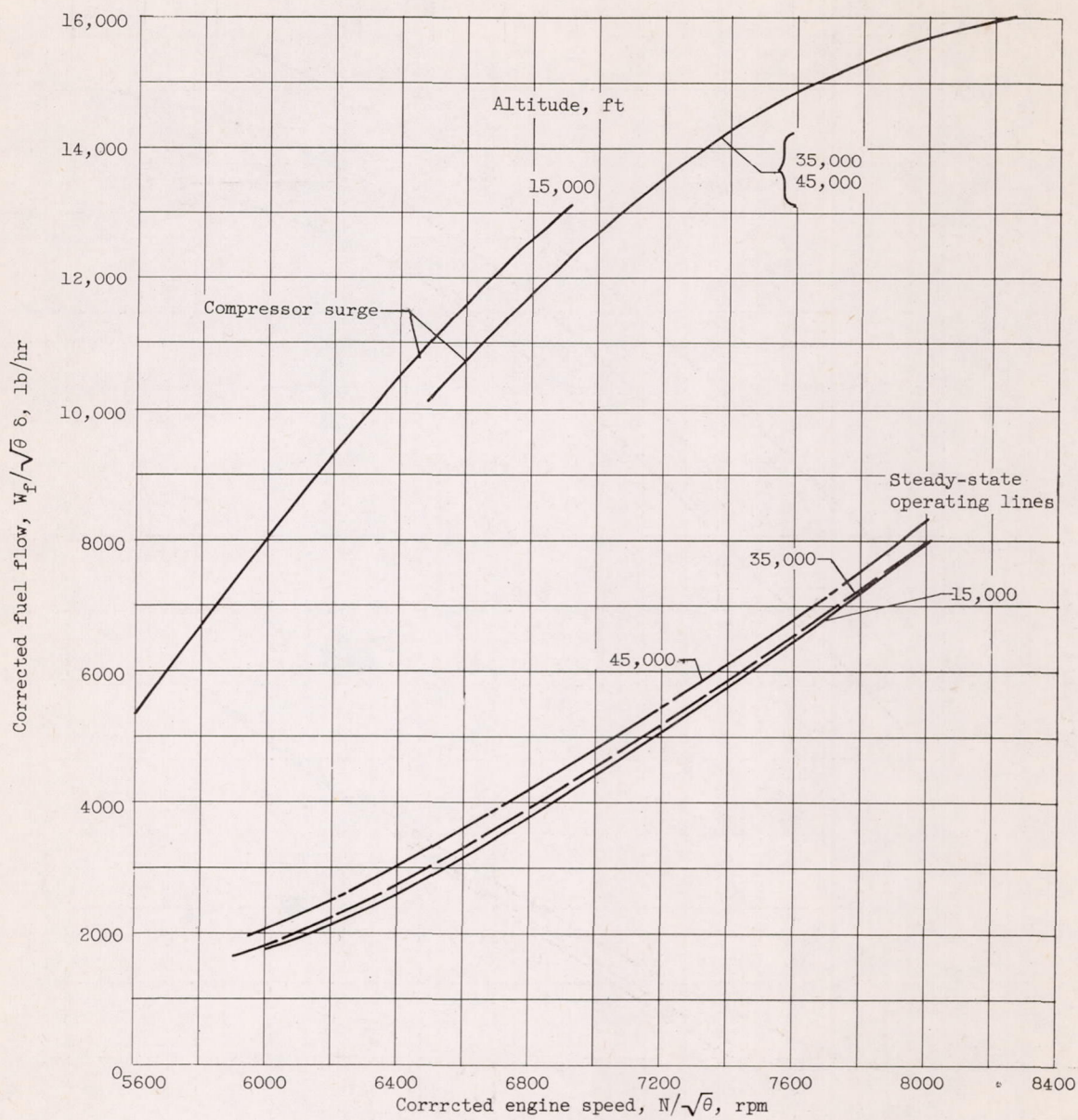
Figure 22. - Effect of operating conditions on fuel-flow surge lines. Inlet guide vanes open.
