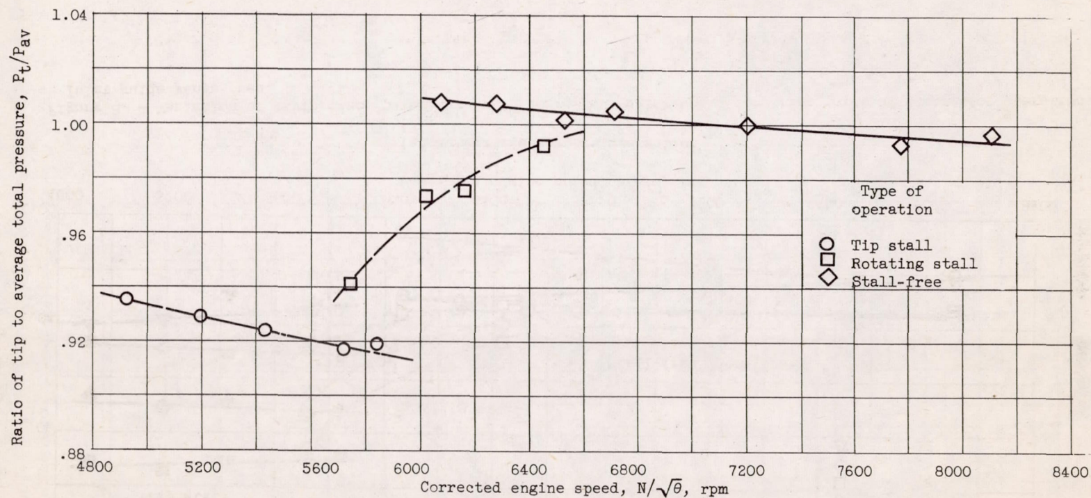
(b) Interstage pressure ratios. Fourth stator stage.
