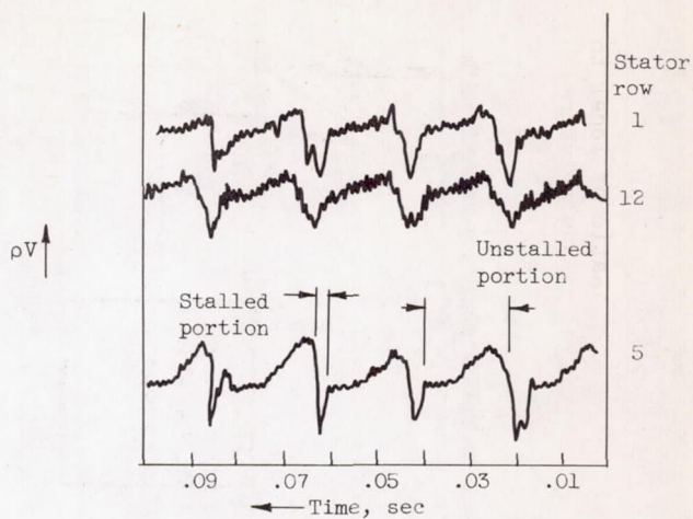
(b) Rotating stall. High intermediate speed (about 6400 rpm).
