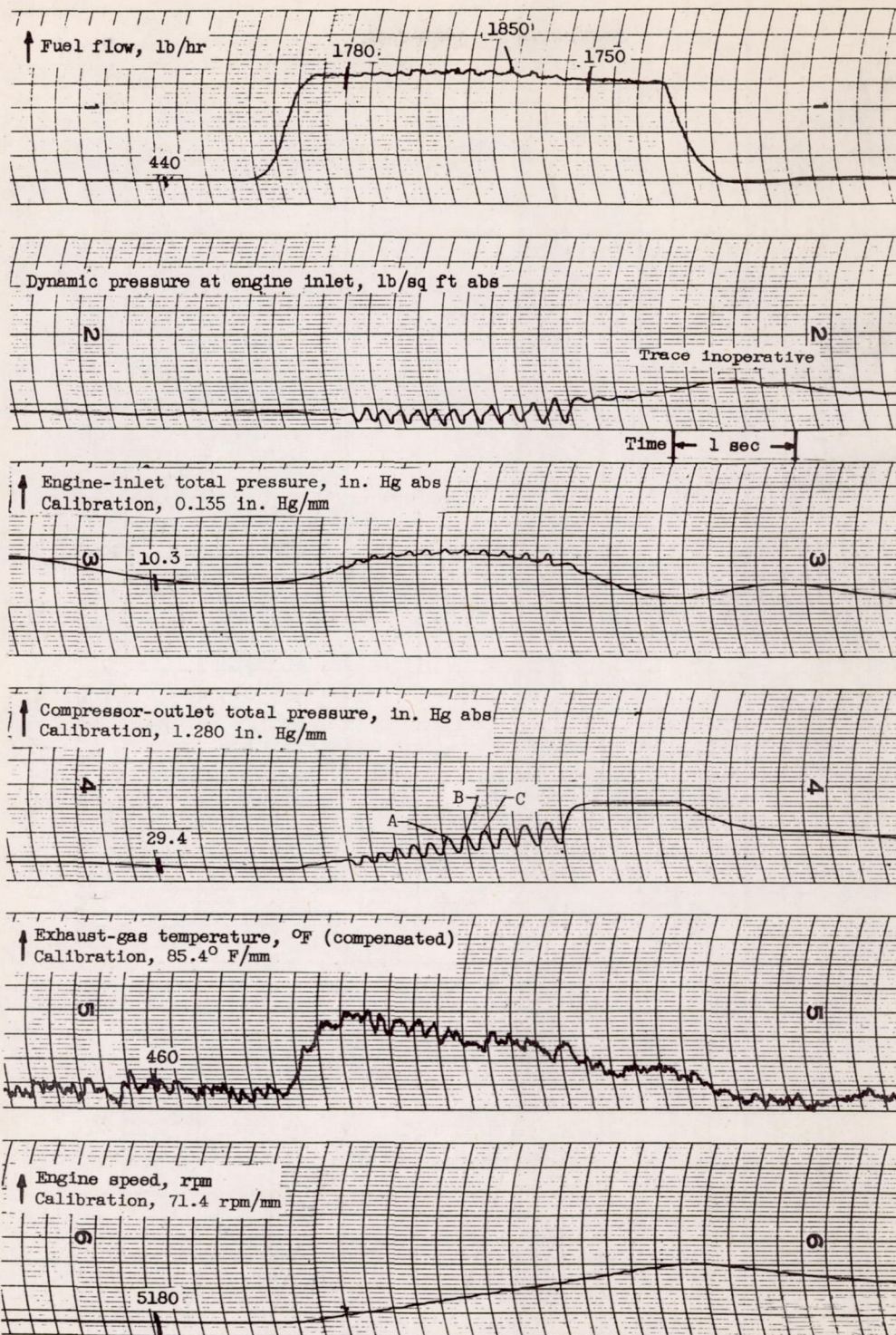
(a) Encountering surge with stall. Altitude, 35,000 feet; engine-inlet air temperature, -10^{\circ} F.
