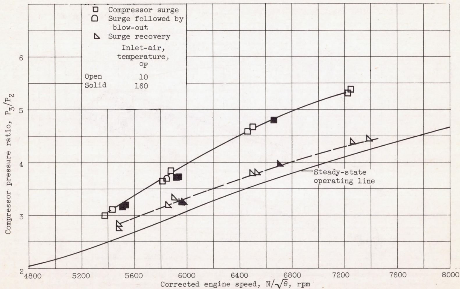
Figure 19. - Concluded. Effects of operating conditions on compressor surge during acceleration. Inlet guide vanes closed.
