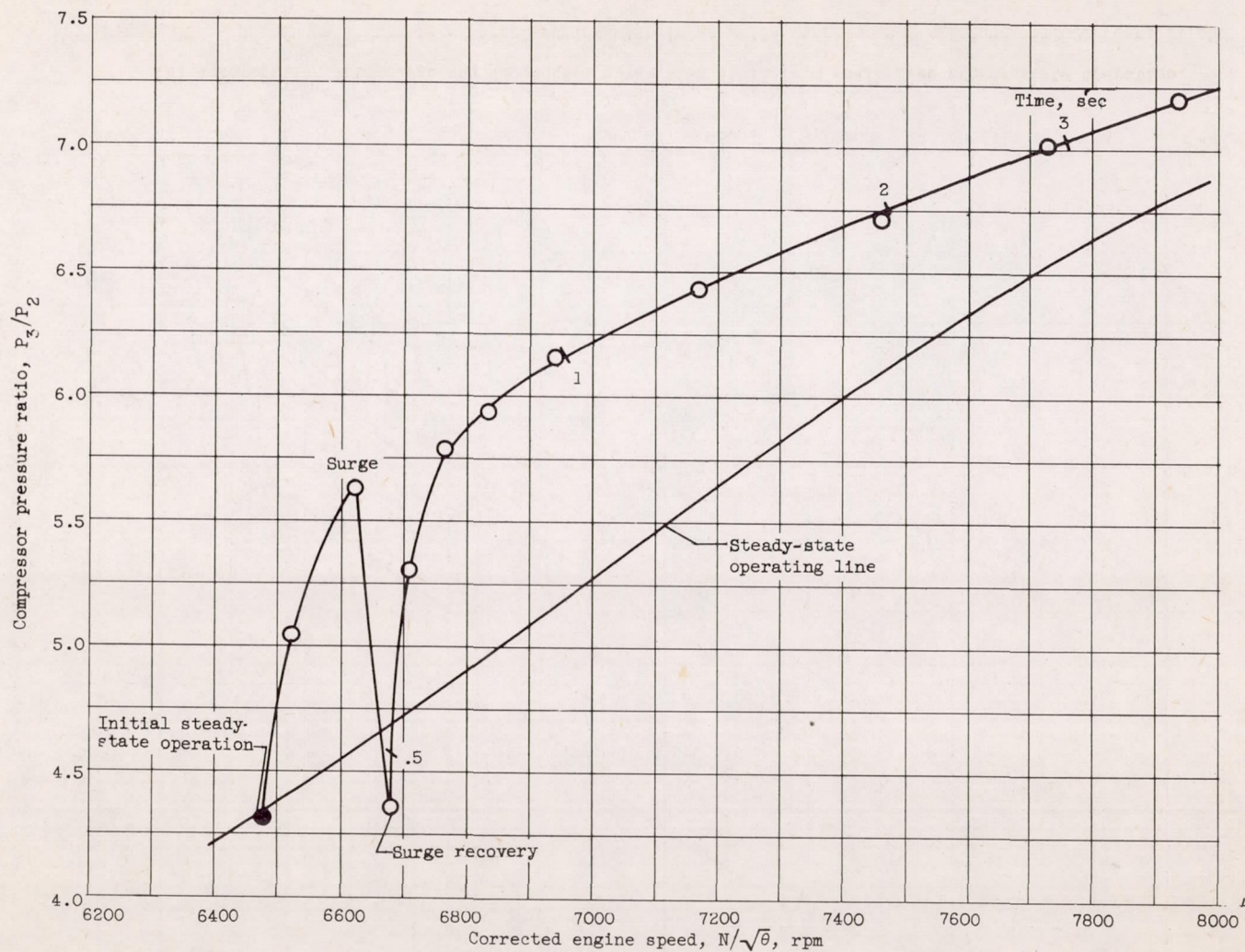
(c) Acceleration into surge from stall-free steady-state operation.
