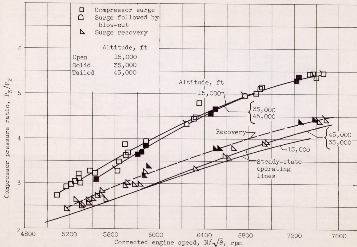
(b) Altitude. Flight Mach number, 0.8.
