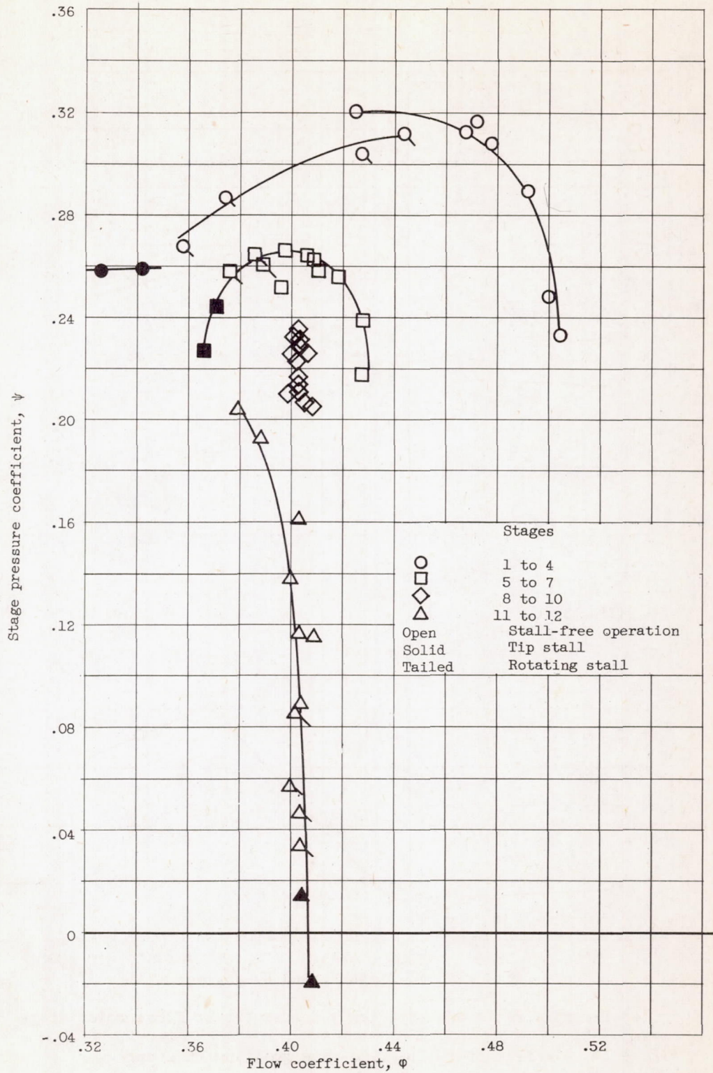
Figure 10. - Variation of stage pressure coefficient with flow coefficient for several groups of compressor stages. Inlet guide vanes open.
