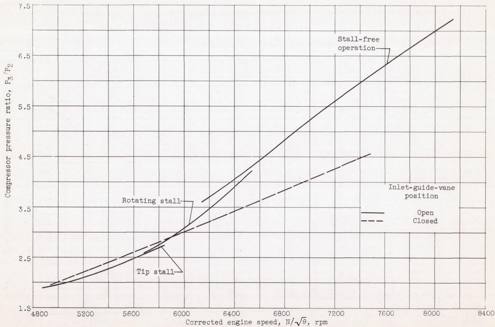
Figure 11. - Continued. Effect of inlet-guide-vane position on compressor operation.
