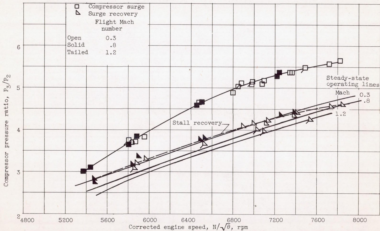
(a) Flight Mach number. Altitude, 35,000 feet.
