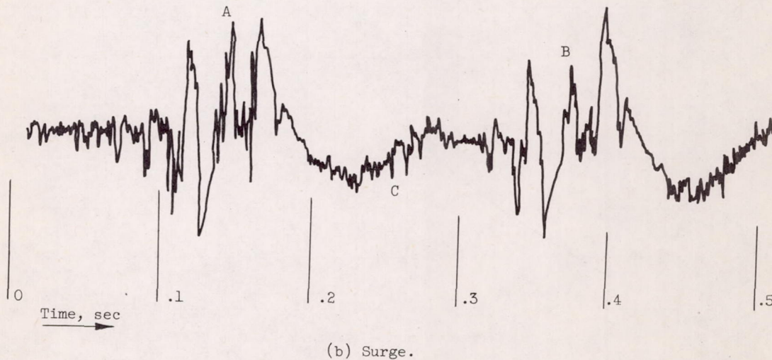
Figure 13. - Oscillograph traces of hot-wire-anemometer probe during accelerations encountering two types of compressor surge.
