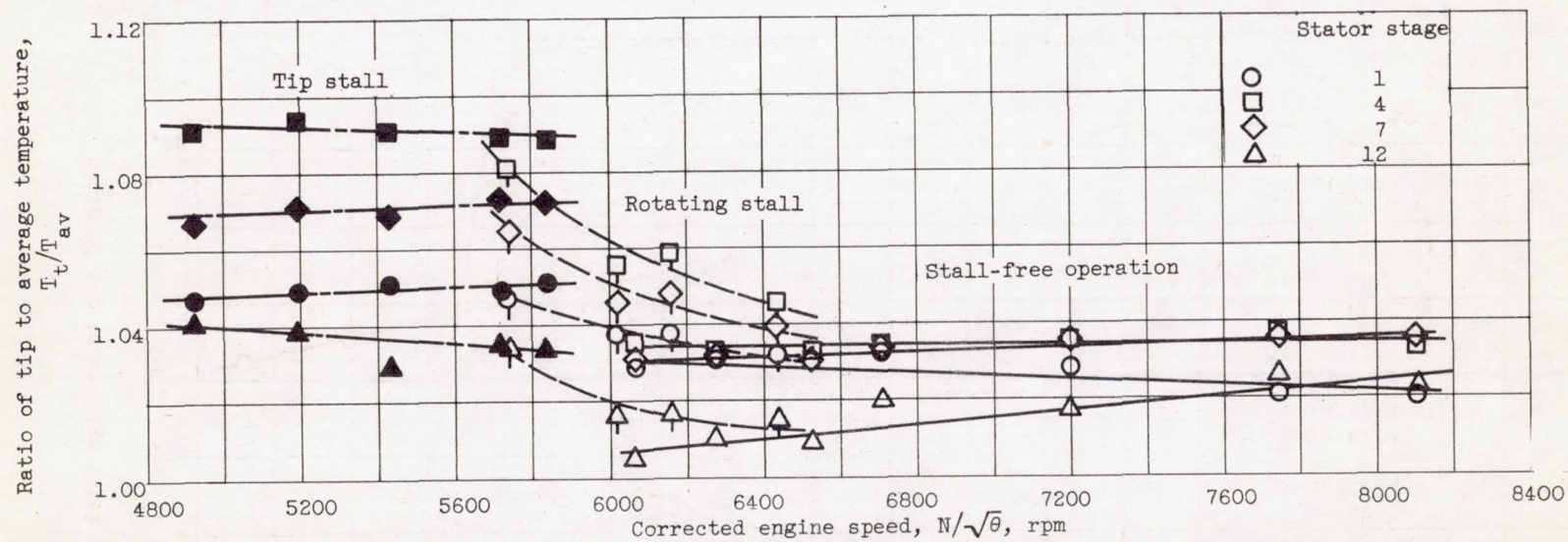
(a) Interstage temperature ratios.
