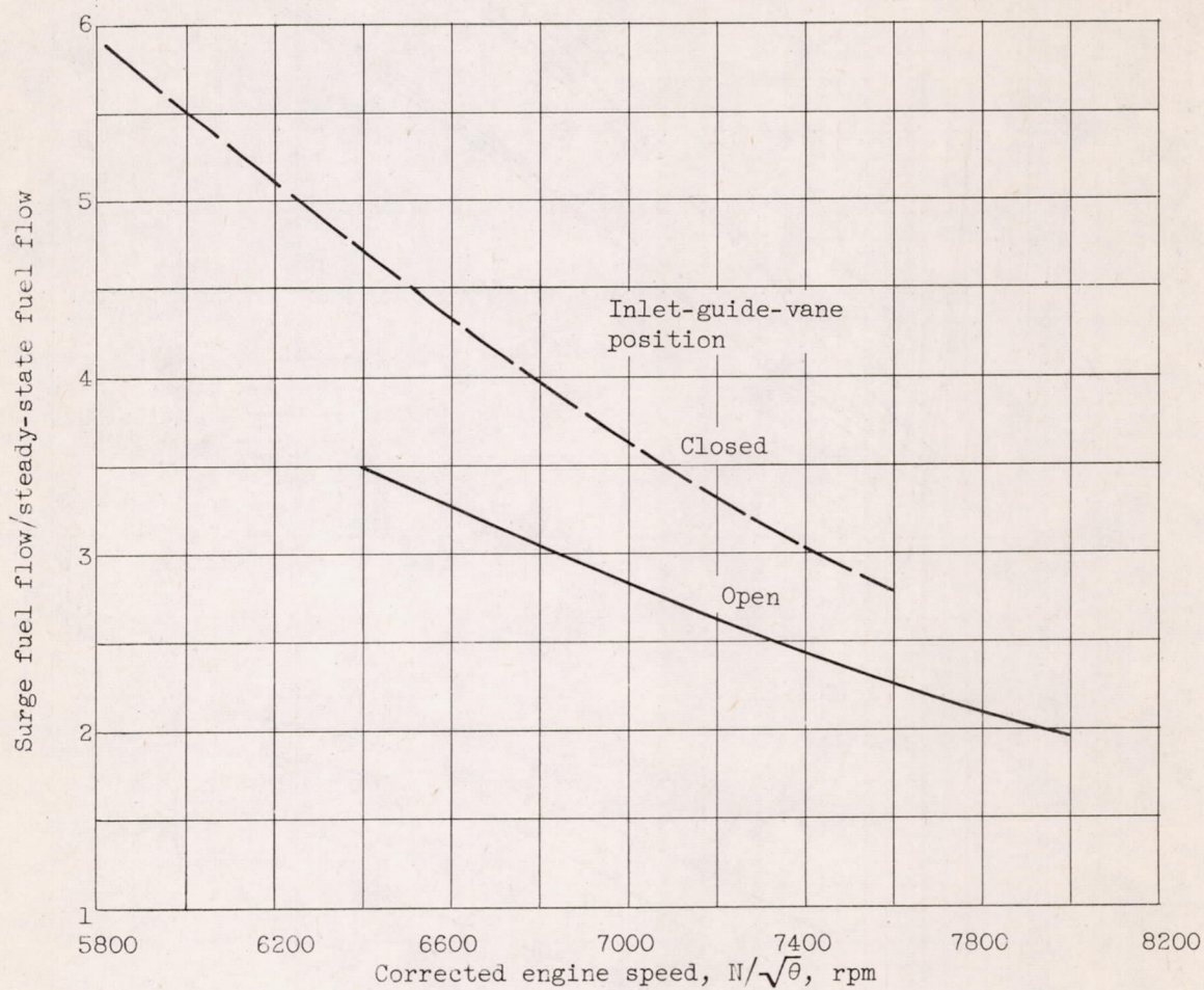
Figure 24. - Variation of fuel-flow margin available for acceleration with corrected engine speed for open and closed inlet guide vanes. Altitude, 35,000 feet; flight Mach number, 0.8.
