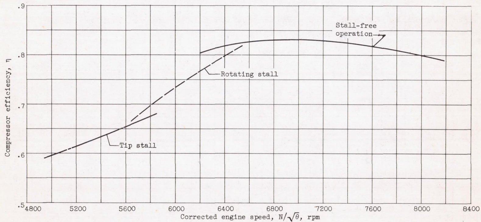
(c) Compressor efficiency.
