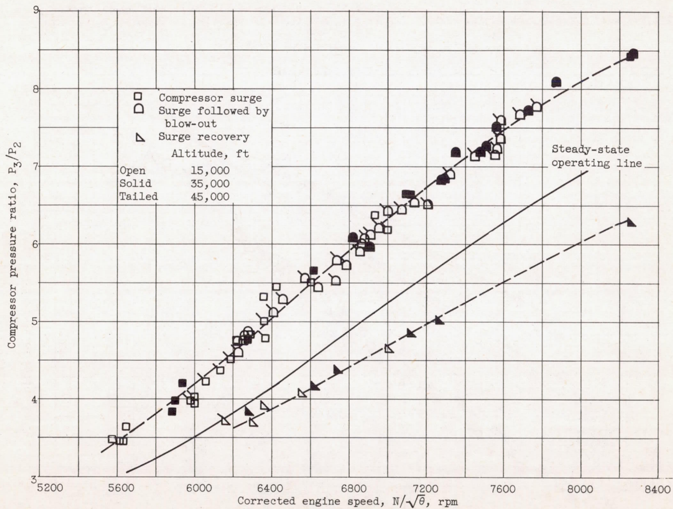
(b) Altitude. Flight Mach number, 0.8.
