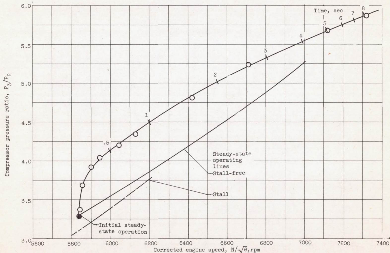
(d) Successful acceleration from stall-free steady-state operation.
