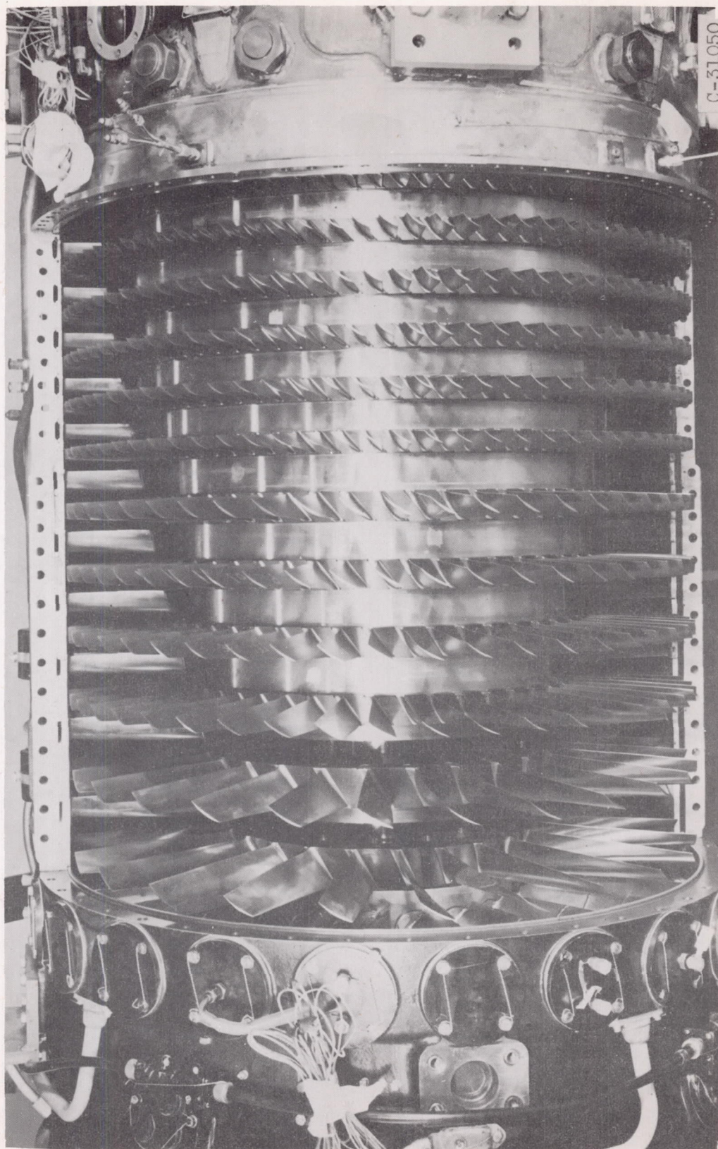
Figure 2. - Compressor rotor.
