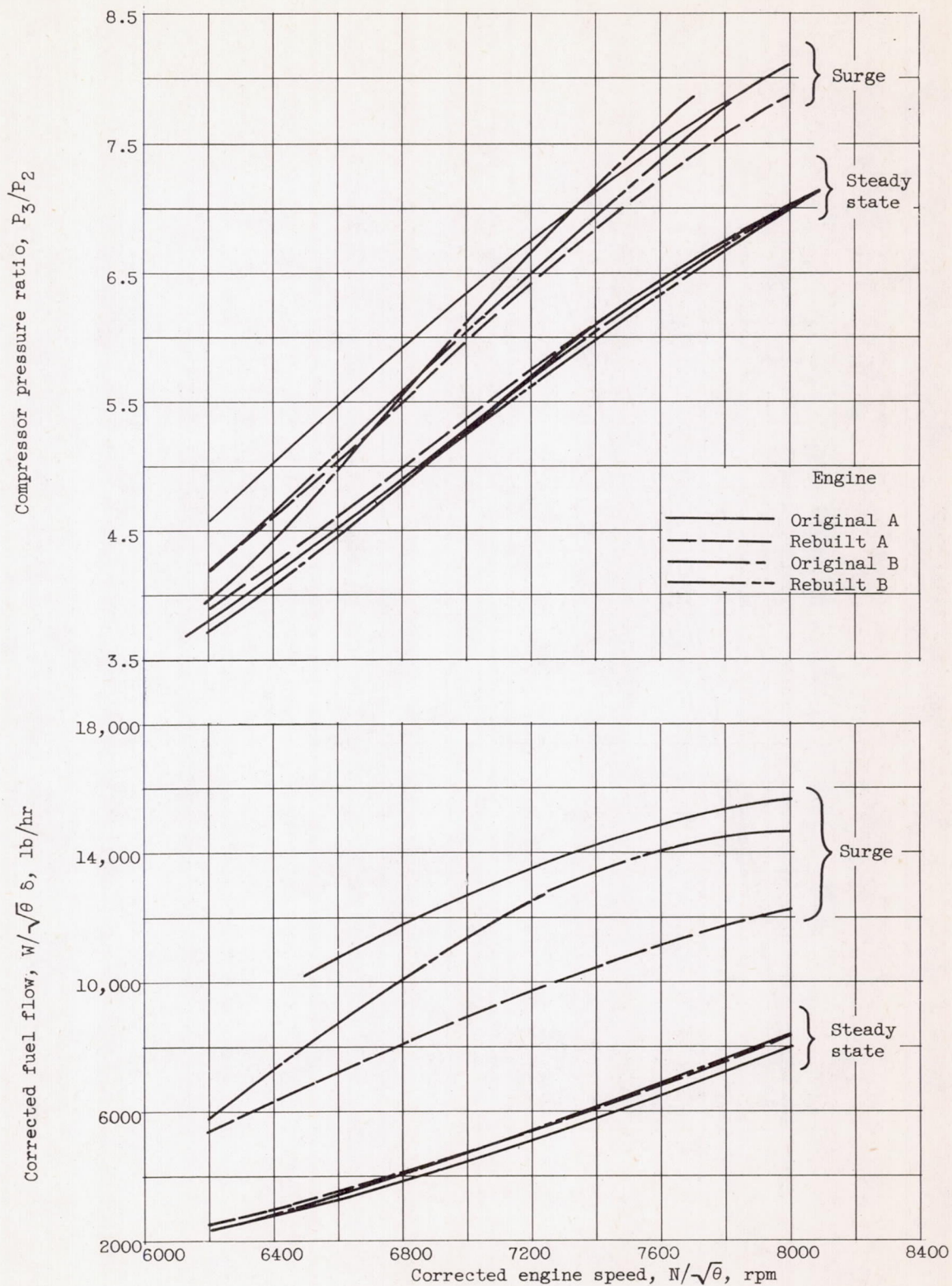
Figure 25. - Comparison of operating limits obtained from engines used in investigation.
