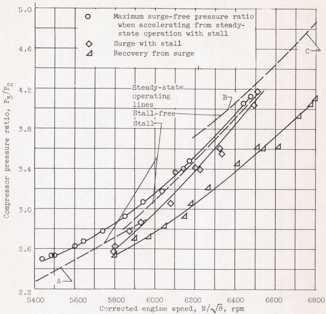
Figure 17. - Surge characteristics in steady-state stall region. Altitude, 35,000 feet; flight Mach number, 0.8. (For typical acceleration from regions A, B, and C, see figs. 15(a), (b), and (c), respectively.)
