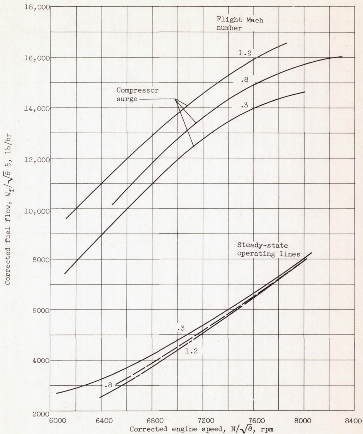
(b) Flight Mach number. Altitude, 35,000 feet.
