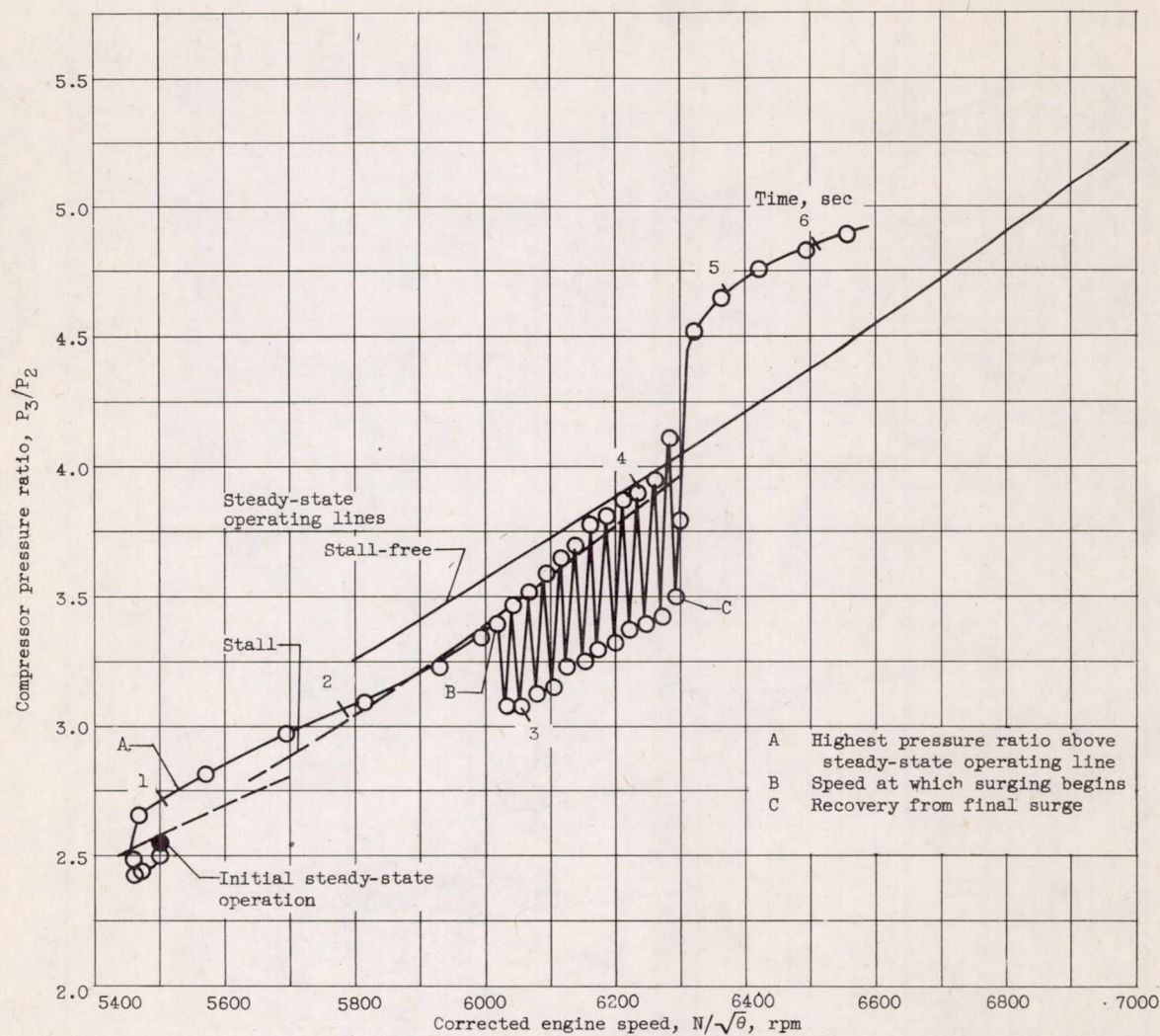
(a) Acceleration into surge with stall from steady-state operation in tip stall.
