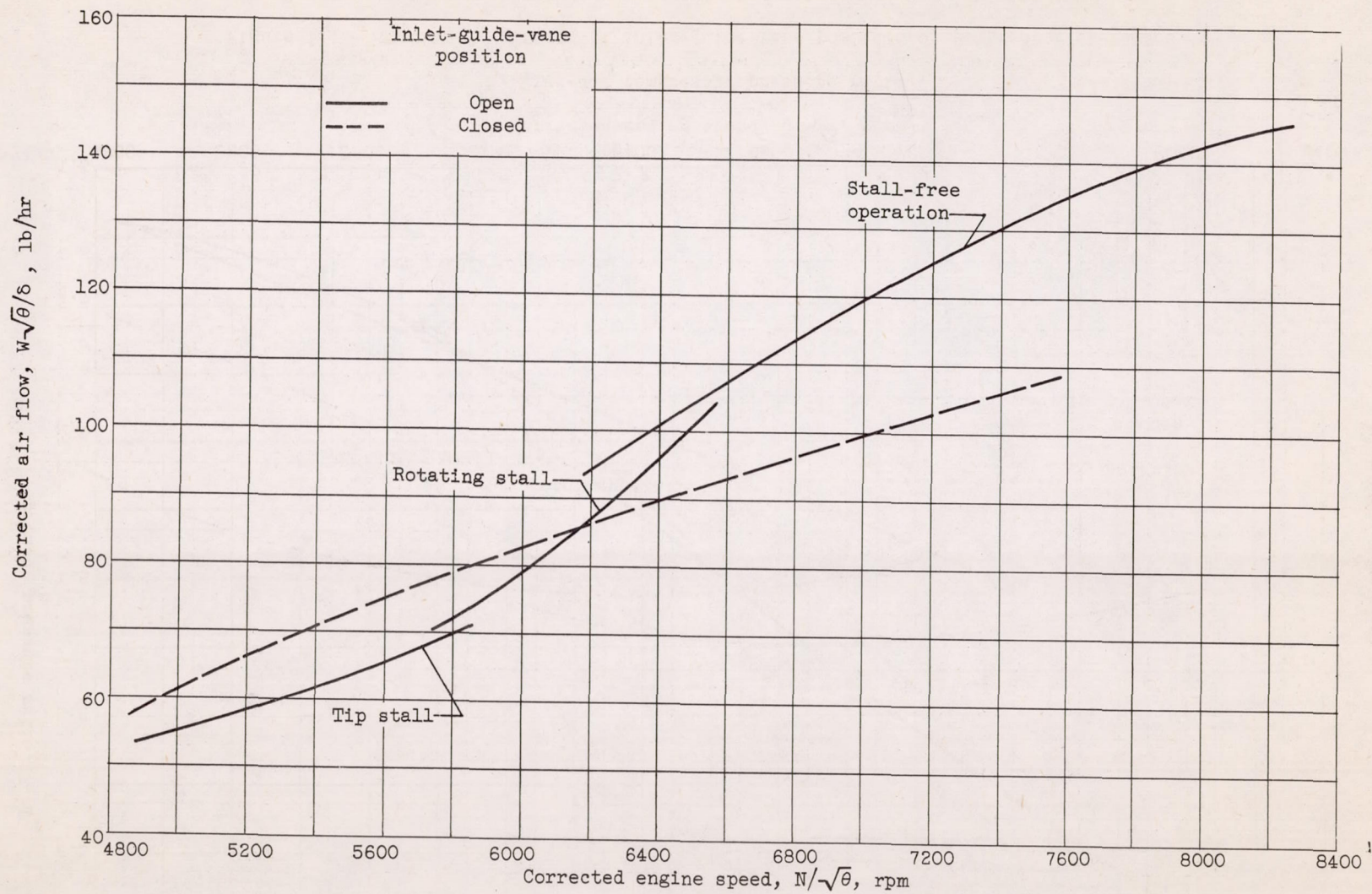
(c) Corrected air flow.
