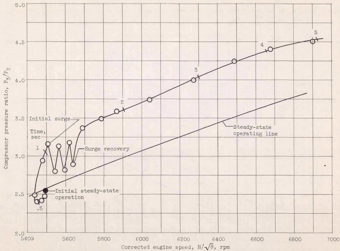
Figure 16. - Stall encountered in acceleration with inlet guide vanes closed. Altitude, 35,000 feet; flight Mach number, 0.8.
