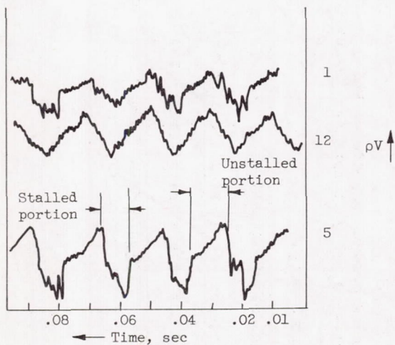
(c) Rotating stall. Low intermediate speed (about 5800 rpm).
