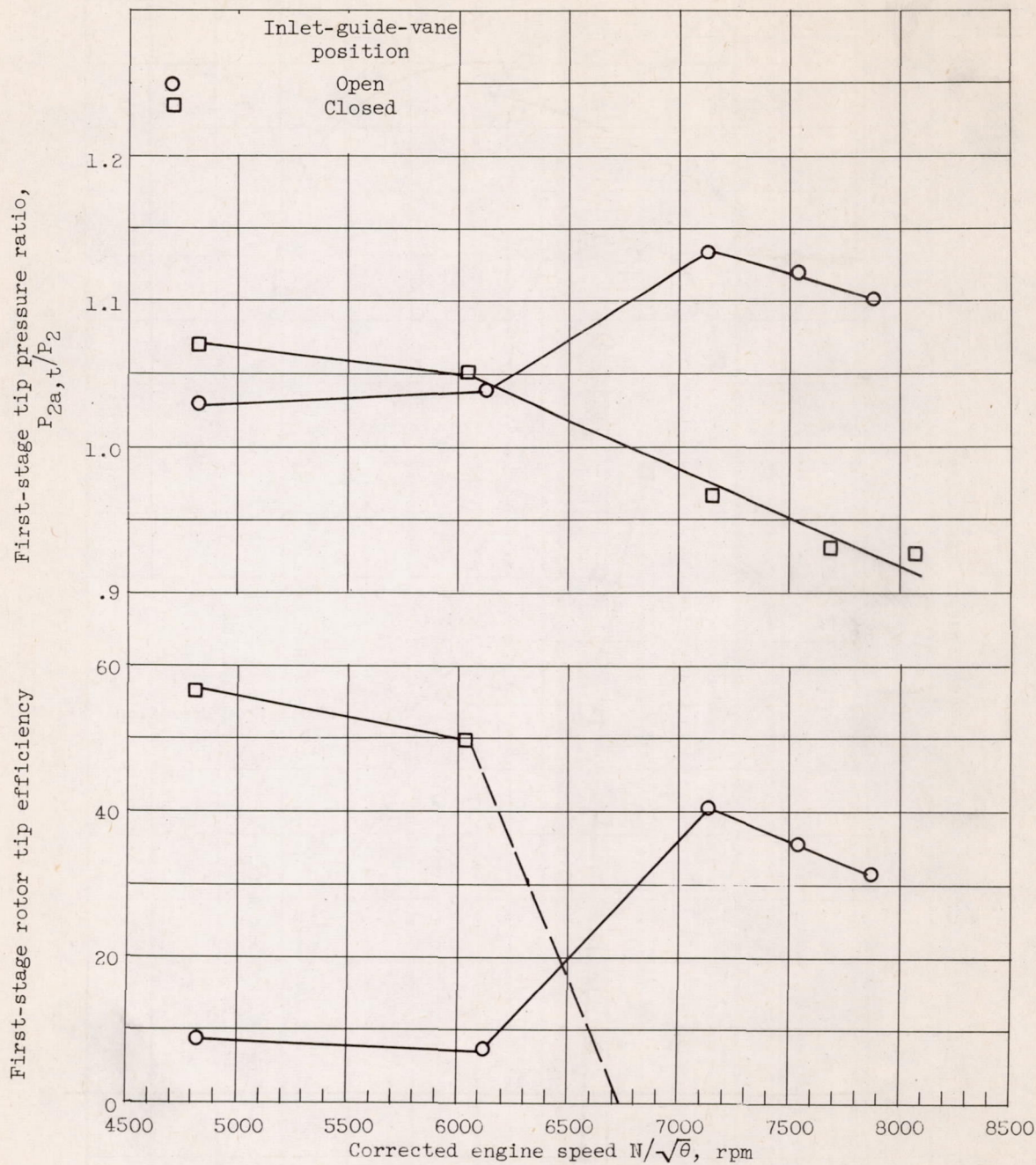
(a) Pressure ratio and efficiency across tip of first rotor stage.
