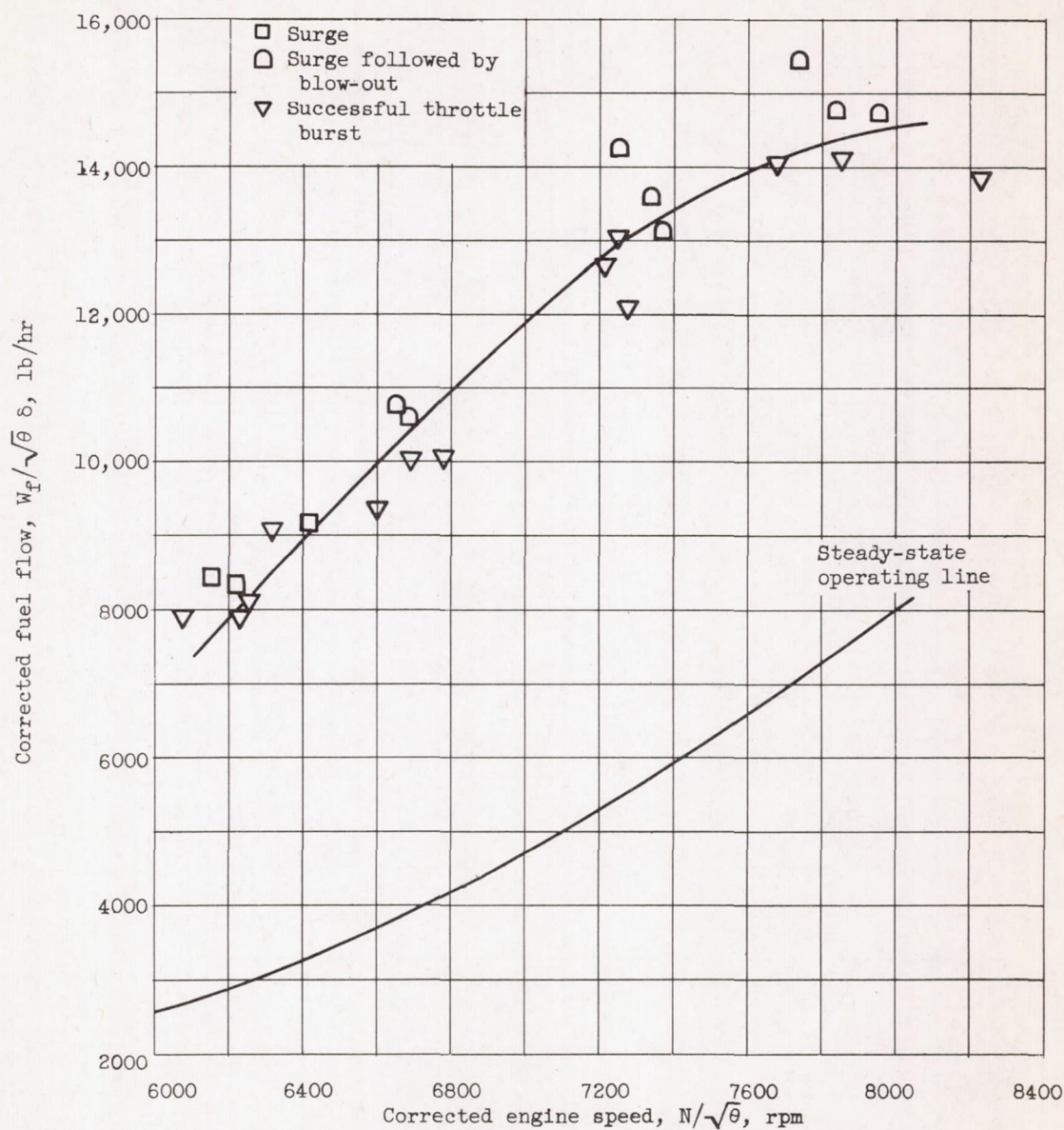
Figure 21. - Determination of engine fuel-flow surge limit. Altitude, 35,000 feet; flight Mach number, 0.3; inlet guide vanes open.
