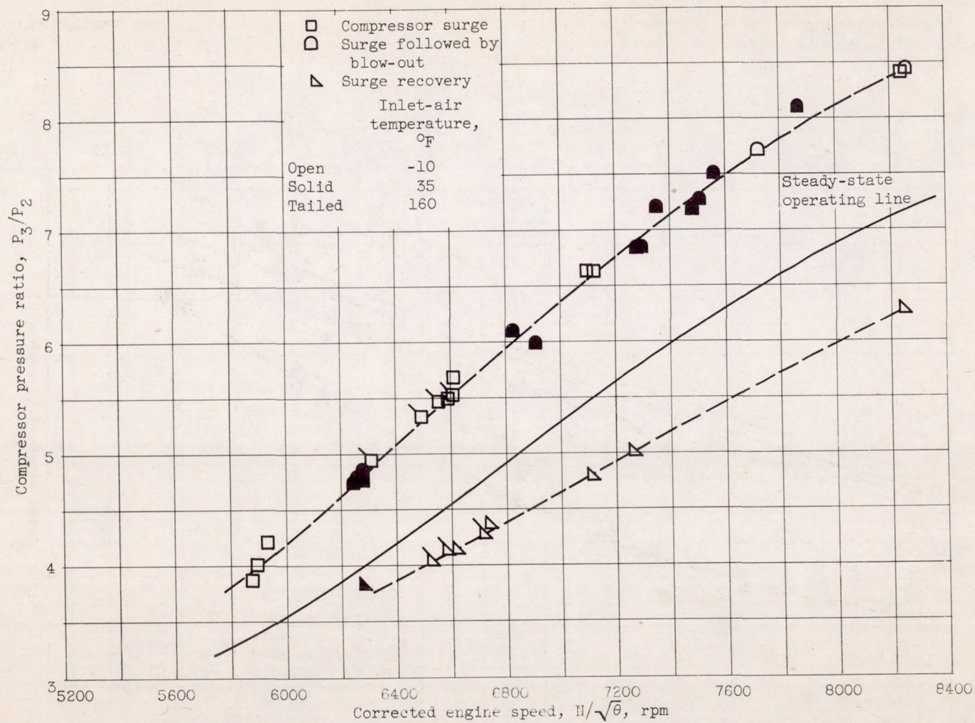
Figure 18. - Concluded. Effects of operating conditions on compressor surge during acceleration from stall-free steady-state operation. Inlet guide vanes open.
