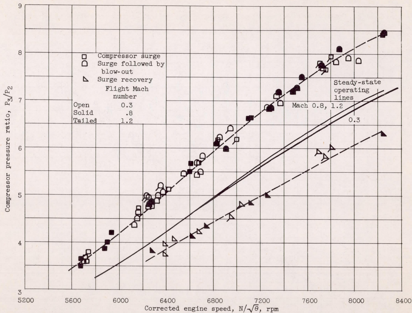
(a) Flight Mach number. Altitude, 35,000 feet.
