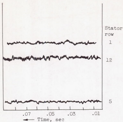
(a) Stall-free operation (speeds above about 6000 rpm).
