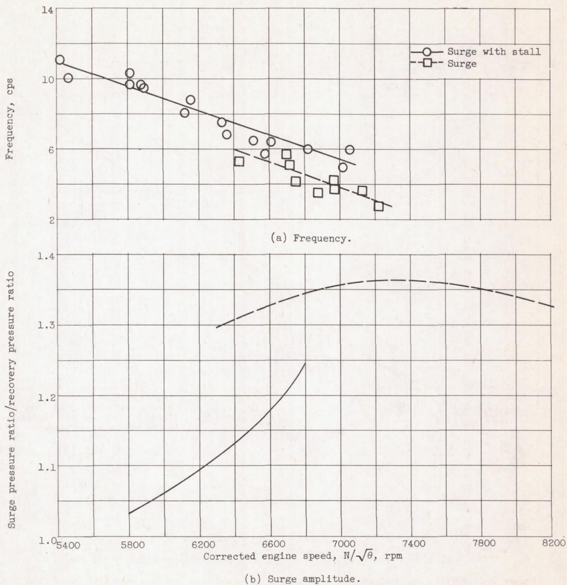
Figure 14. - Variation of frequency and surge amplitude with engine speed for two types of surge.
