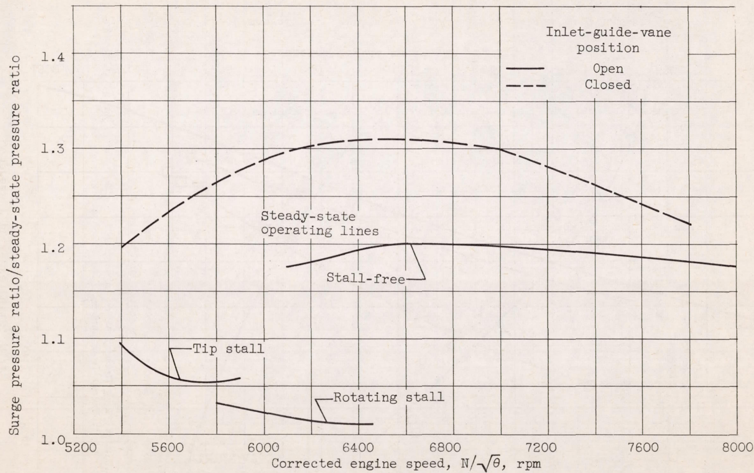
Figure 20. - Effect of inlet-guide-vane position on margin of compressor pressure ratio available for acceleration.
