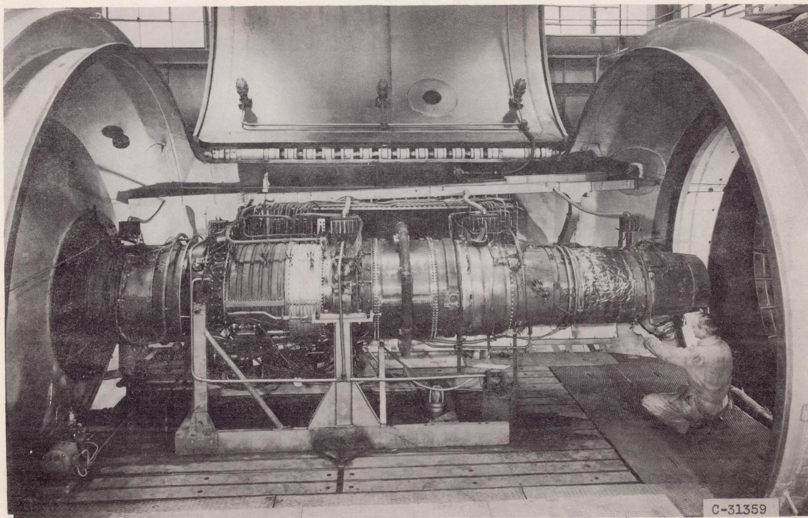
Figure 1. - Turbojet installation in altitude chamber.
