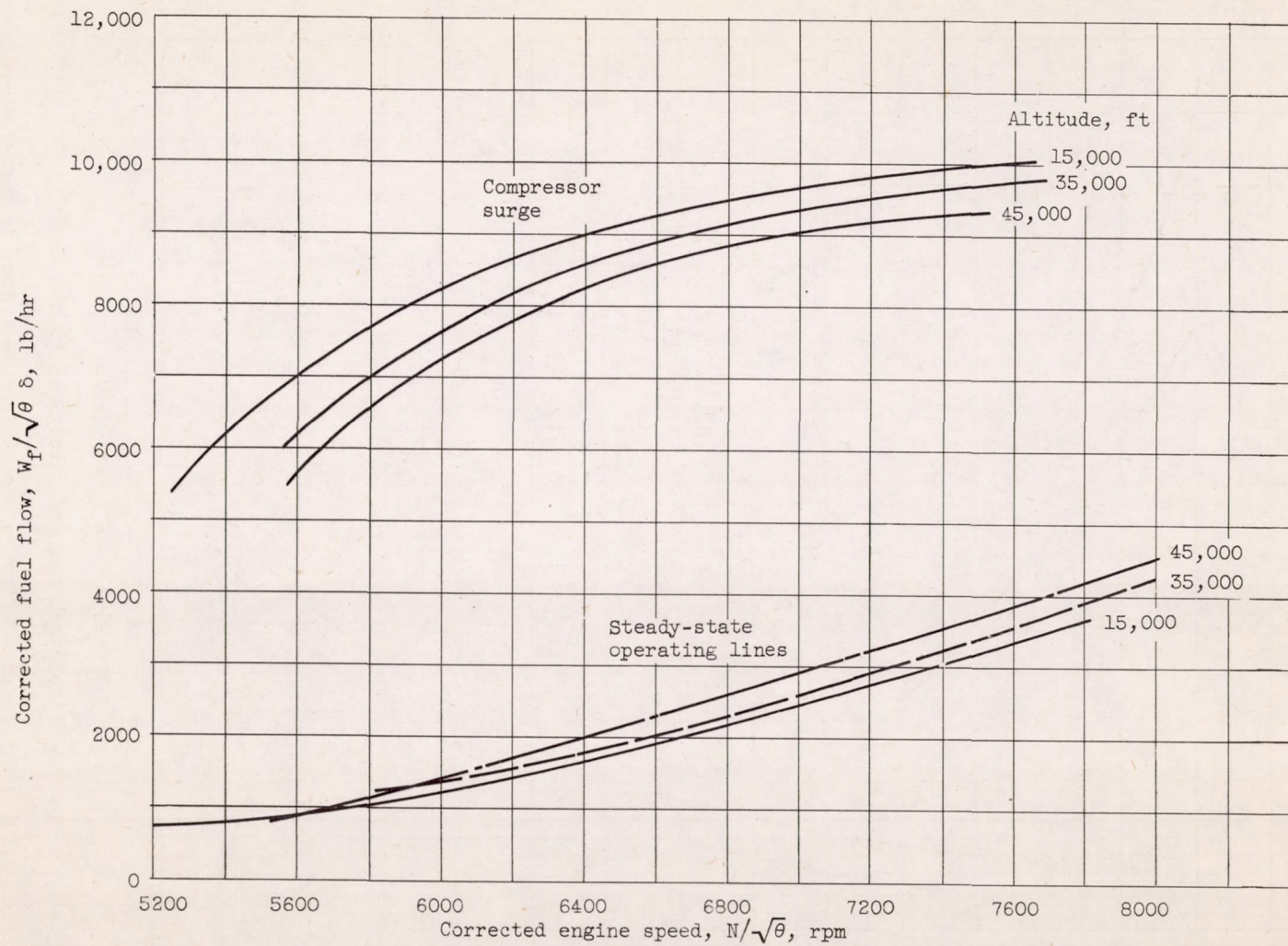
Figure 23. - Effect of operating conditions on fuel-flow surge lines. Inlet guide vanes closed.
