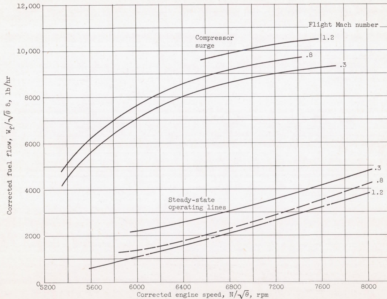
Figure 23. - Concluded. Effect of operating conditions on fuel-flow surge lines. Inlet guide vanes closed.
