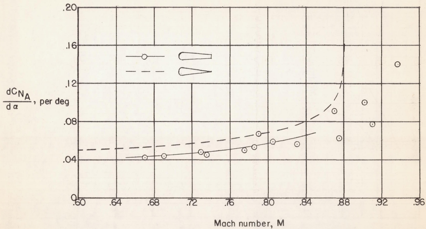
Figure 11.- The variation of normal-force-coefficient slope with Mach number near level flight. h_p \approx 30,000 feet.
