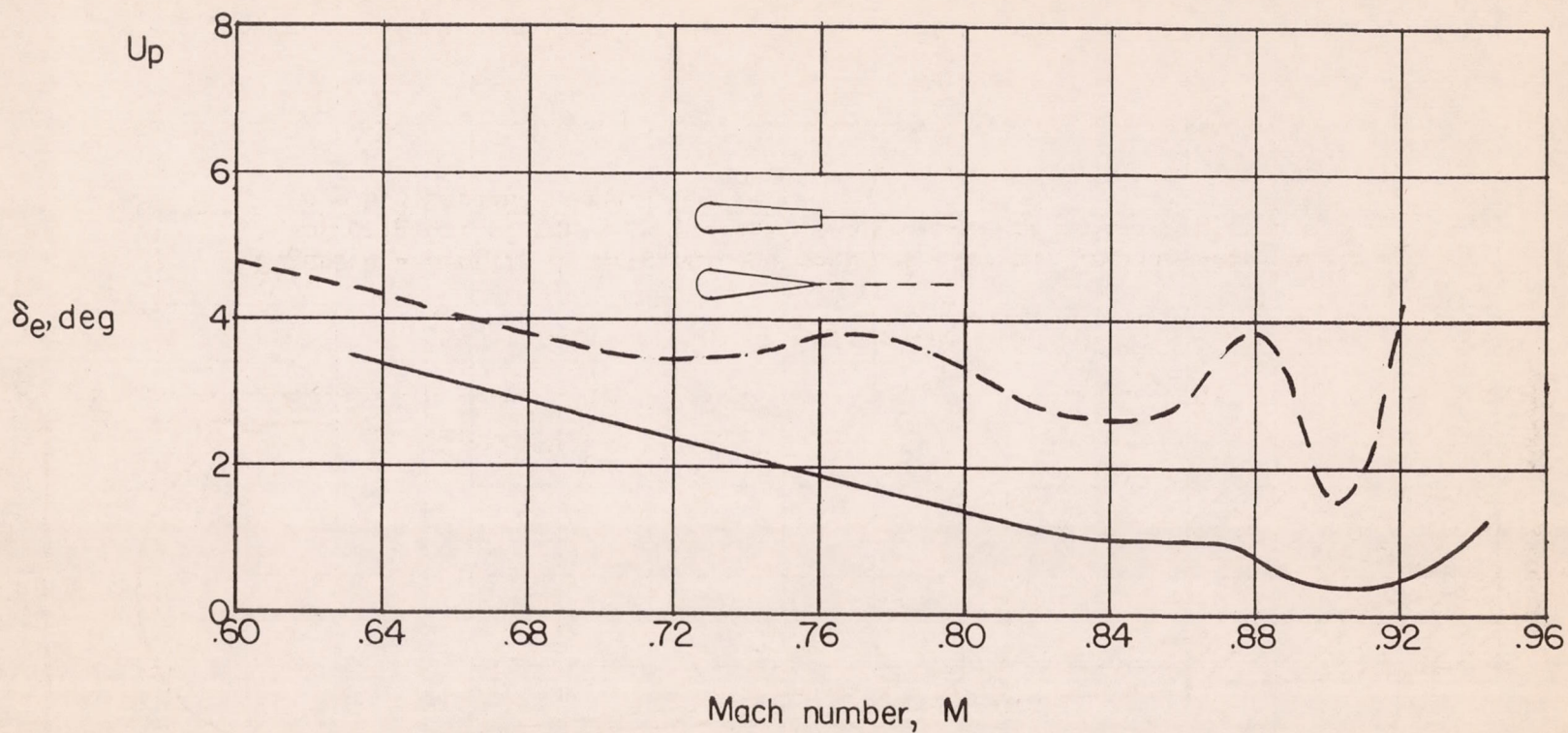
Figure 5.- Variation with Mach number of the longitudinal control deflection required for trim in level flight. h_p \approx 30,000 feet; c.g. at 17 to 18 percent M.A.C.
