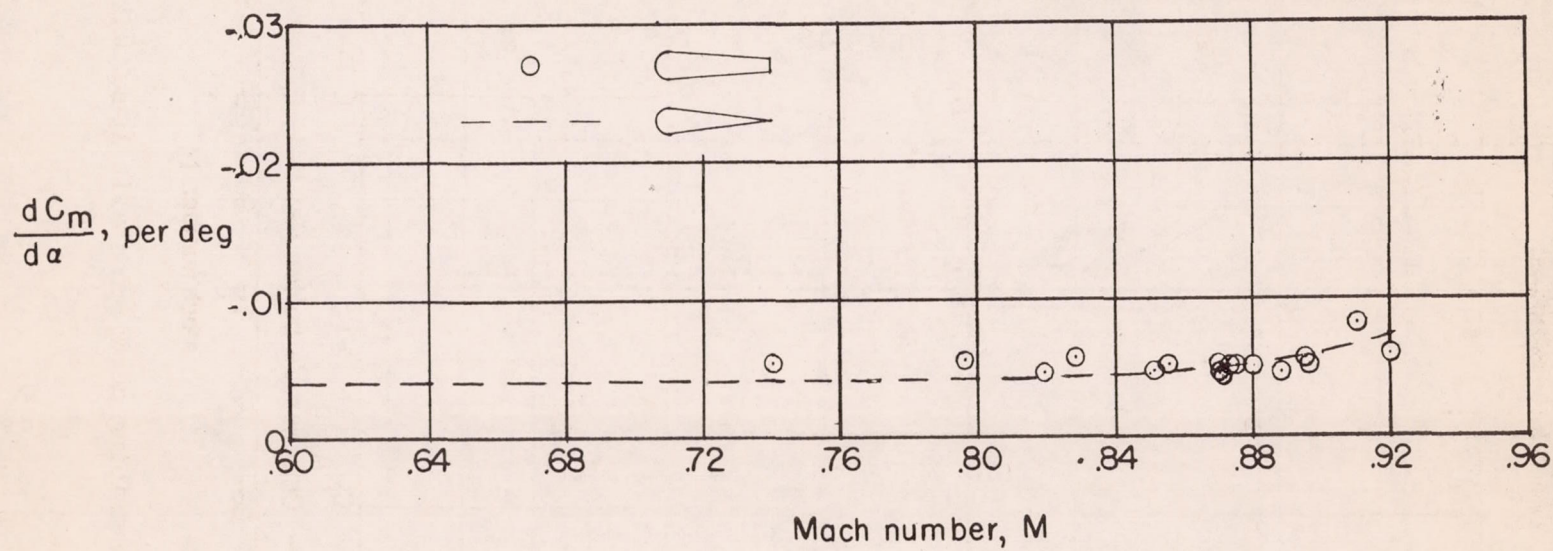
Figure 9.- The variation of static longitudinal stability with Mach number near level flight. h_p \approx 30,000 feet.
