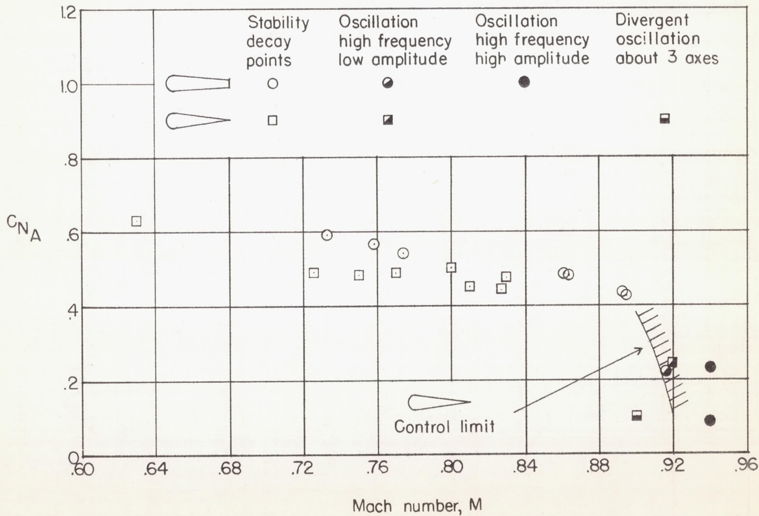
Figure 13.- Usable flight envelope for the X-4 airplane.
