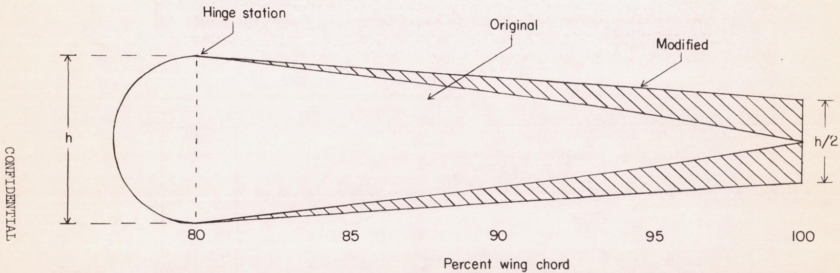
Figure 4.- Profile of original and modified elevon. Trailing-edge angle of original elevon \approx 19^\circ ; trailing-edge angle of modified elevon \approx 8^\circ . h \approx 5.5 percent chord.
