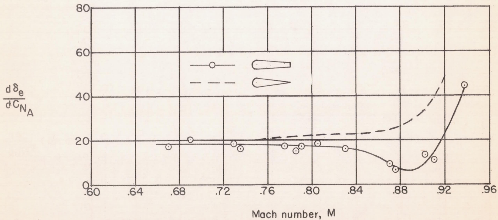
Figure 10.- The variation of the apparent static longitudinal stability parameter d\delta_e/dC_{N_A} with Mach number near level flight. h_p \approx 30,000 feet.
