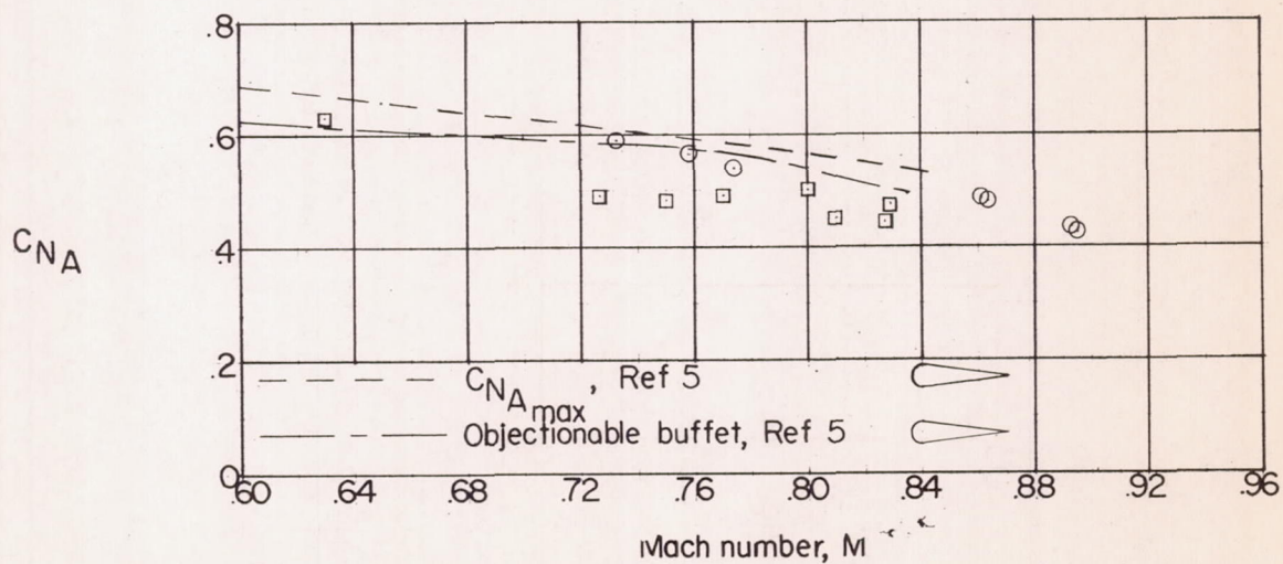
Figure 8.- Boundary describing decay of static longitudinal stability.
