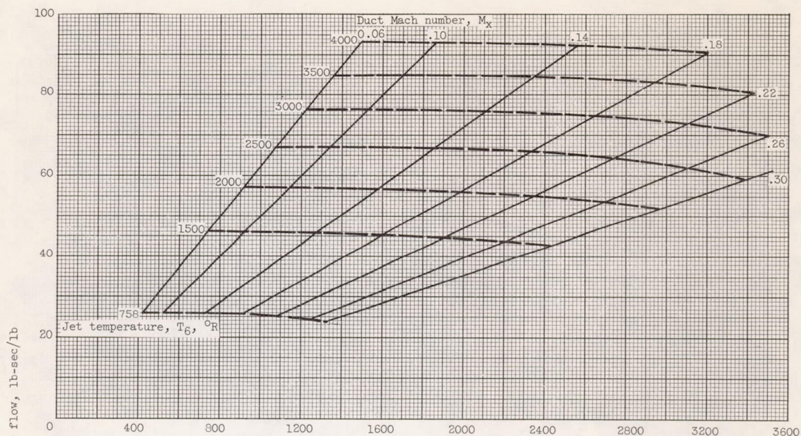
(k) Variable-area tip-jet nozzle; pressure ratio, 3.0; tip speed, 700 feet per second; \Delta P_f = 2.5q_x ; burner area/duct area, 1.5.
