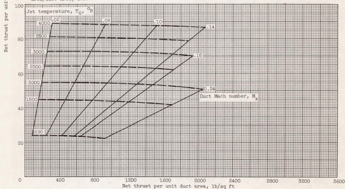
(d) Variable-area tip-jet nozzle; pressure ratio, 2.5; tip speed, 600 feet per second; \Delta P_f = 2.5q_x ; burner area/duct area, 1.5.
