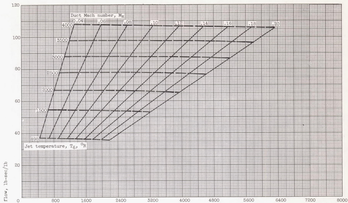
(m) Variable-area tip-jet nozzle; pressure ratio, 5.0; tip speed, 700 feet per second; \Delta P_f = 2.5q_x ; burner area/duct area, 1.5.
