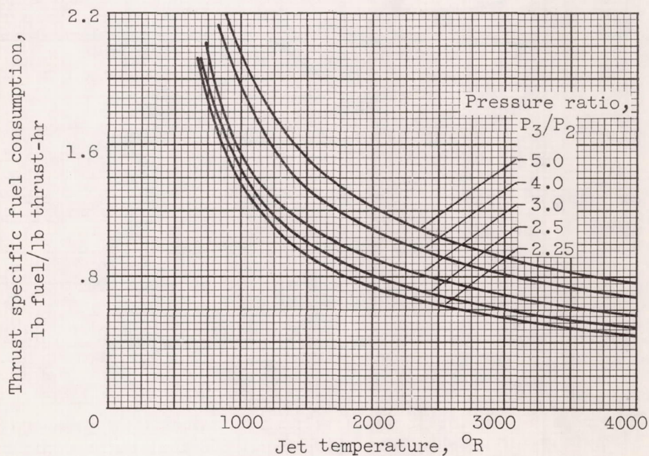
(b) Specific fuel consumption.
