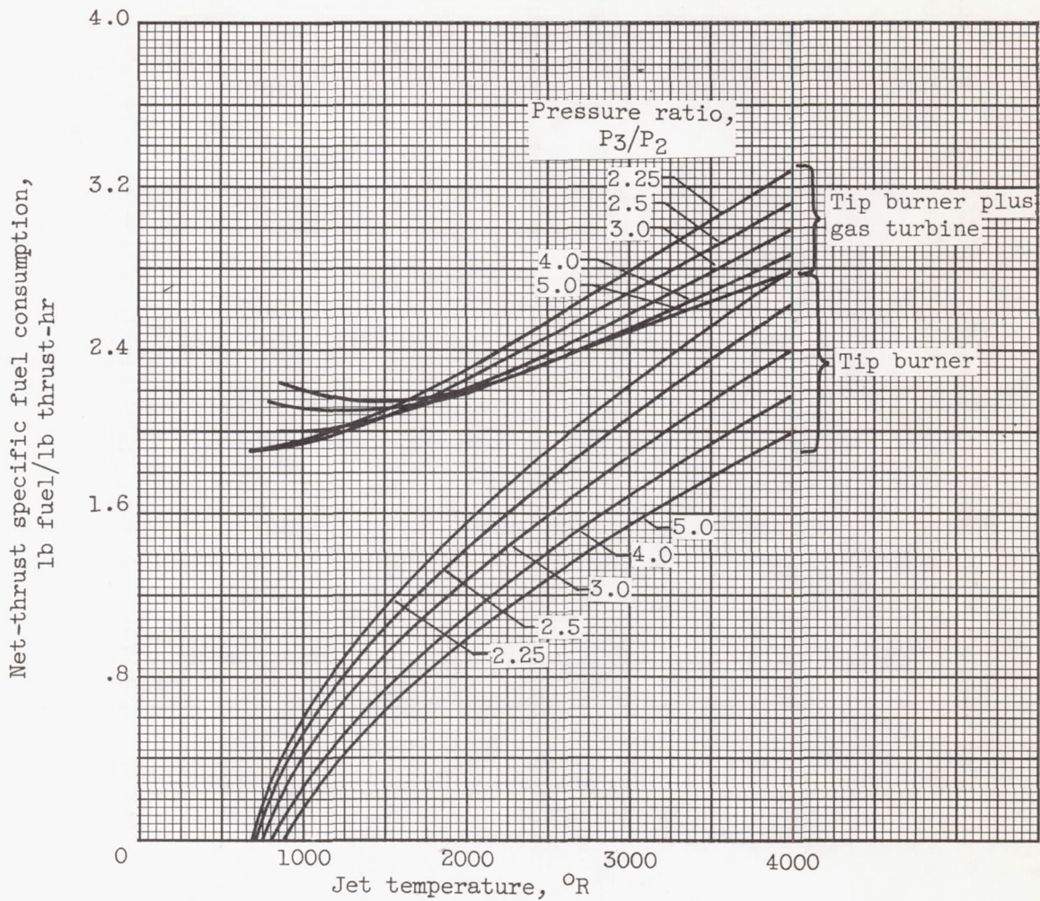
Figure 9. - Net-thrust specific fuel consumption of pressure jet. Variable-area jet nozzle; tip speed, 700 feet per second; burner area/duct area, 1.5; duct Mach number, 0.1.
