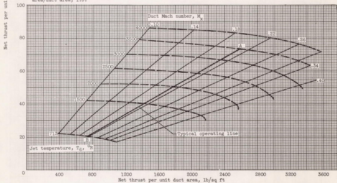
(h) Variable-area tip-jet nozzle; pressure ratio, 2.5; tip speed, 700 feet per second; \Delta P_r = 2.5q_x ; burner area/duct area, 1.5.
