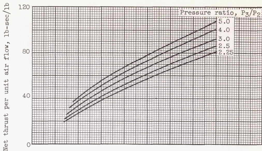
(a) Specific thrust.
