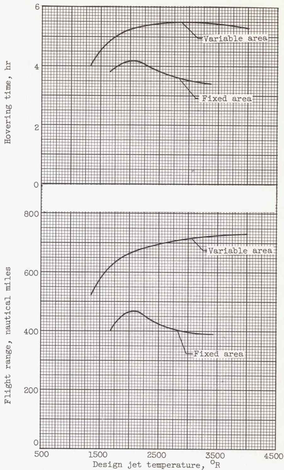
Figure 17. - Comparison of flight performance with variable- and fixed-area tip-jet nozzles. Design pressure ratio, 3.0; tip speed, 700 feet per second.
