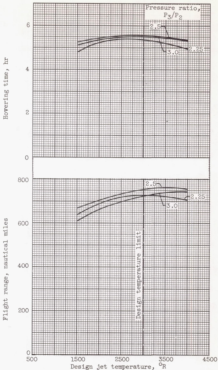
Figure 15. - Flight performance as function of design jet temperature and pressure ratio. Tip speed, 700 feet per second; duct area/section area, 0.50; burner area/section area, 0.75.
