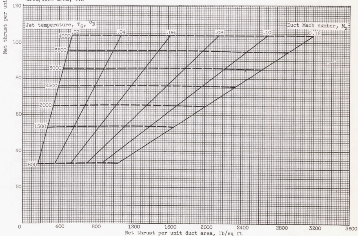
Figure 5. - Continued. Power-available chart.
