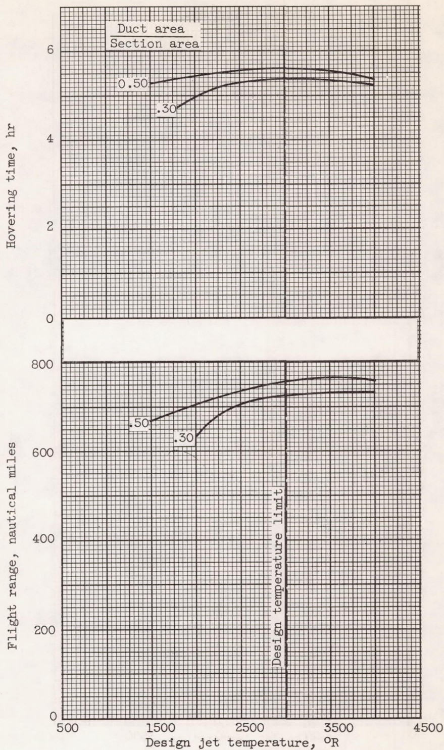
Figure 14. - Effect of duct area on flight performance. Design pressure ratio, 2.5; tip speed, 700 feet per second; burner area/section area, 0.75.
