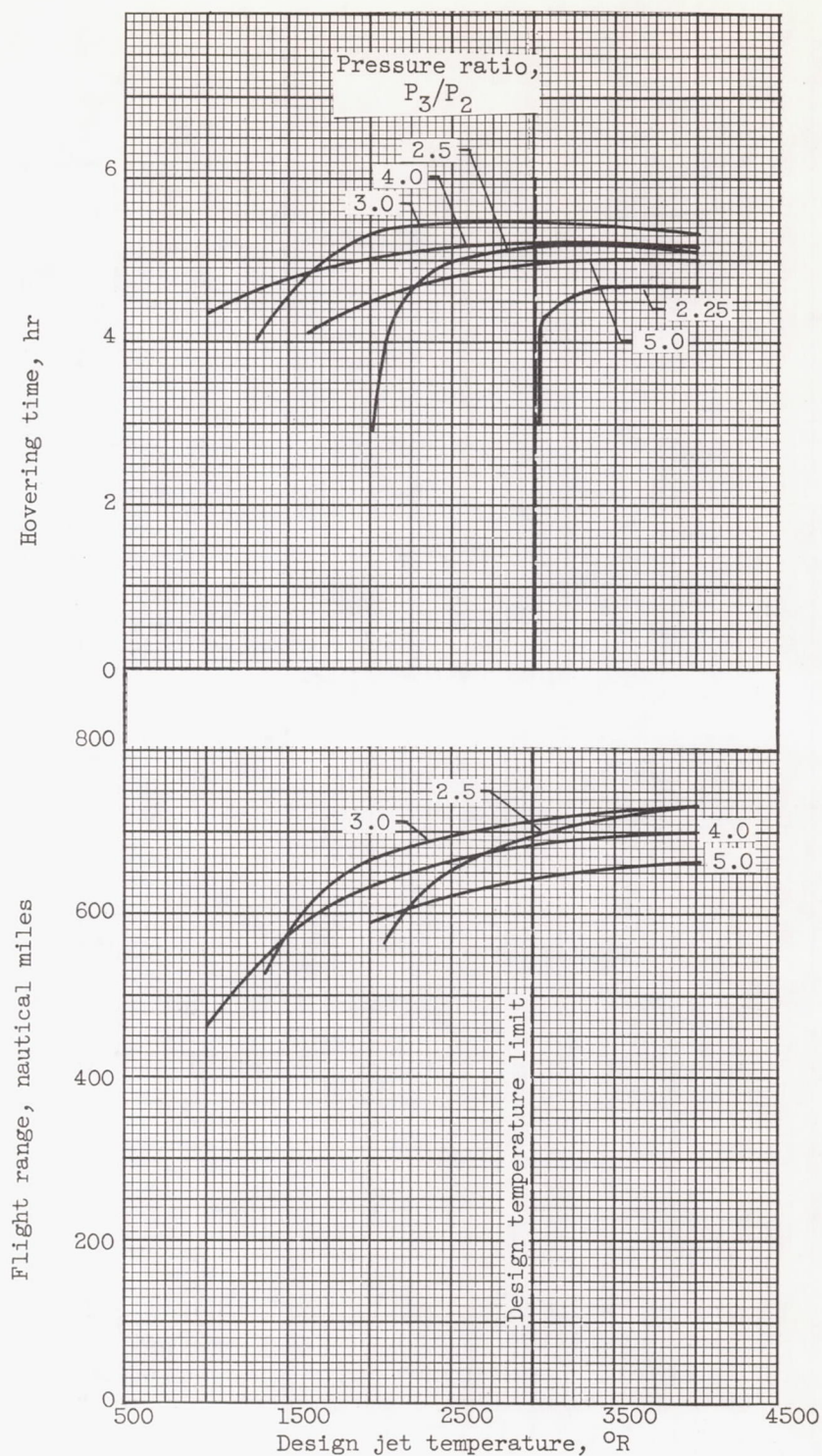
Figure 11. - Flight performance as function of design jet temperature and pressure ratio. Tip speed, 700 feet per second; duct area, 0.3 \times section area; burner area, 0.45 \times section area.
