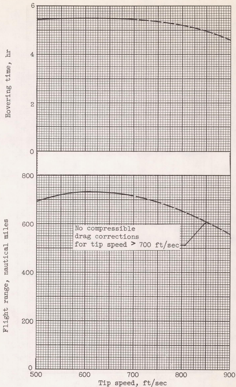
Figure 16. - Flight performance as function of rotor tip speed. Variable-area tip-jet nozzle; duct area/section area, 0.3; burner area/section area, 0.45.
