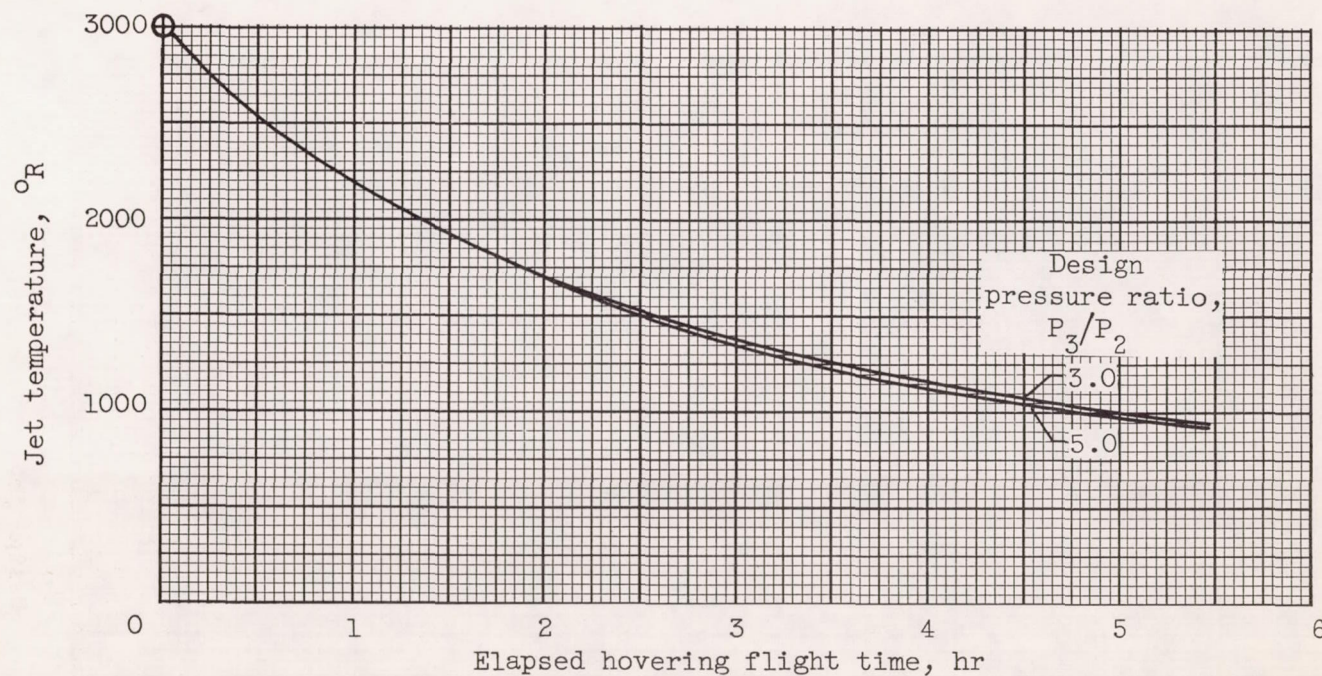
Figure 12. - Jet temperature as function of elapsed hovering time. Design jet temperature, 3000° R; tip speed, 700 feet per second; duct area/section area, 0.3; burner area/section area, 0.45.
