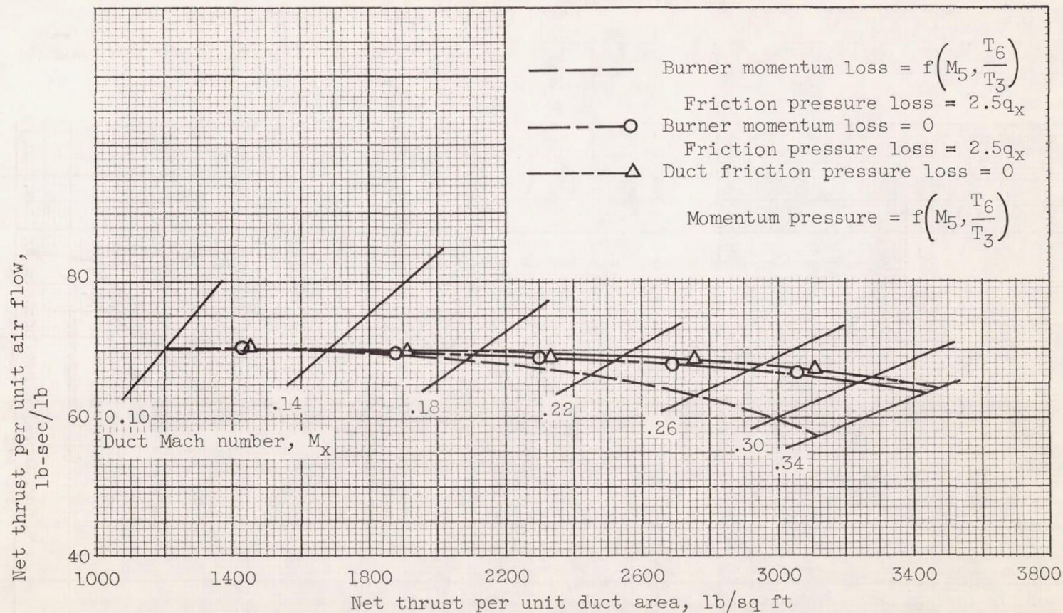
Figure 6. - Effect of duct friction pressure loss and burner momentum pressure loss on specific thrust. Pressure ratio, 2.5; tip speed, 700 feet per second; burner area/duct area, 1.5; jet temperature, 3000^\circ \text{R} .
