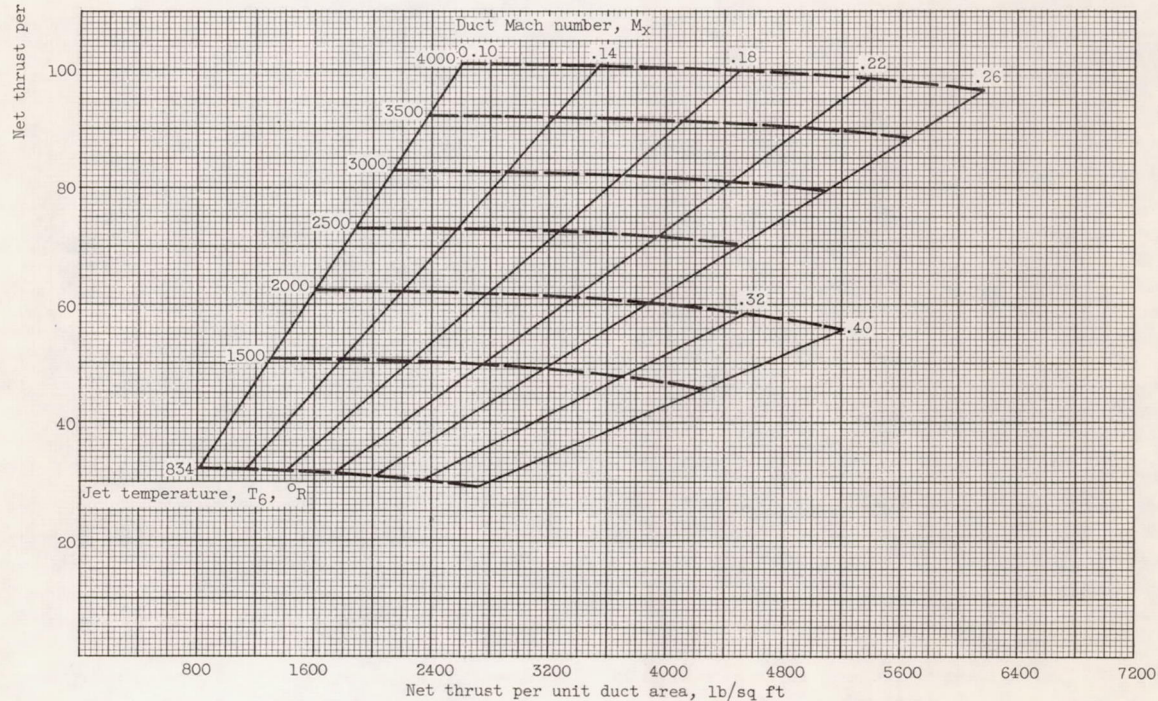
(l) Variable-area tip-jet nozzle; pressure ratio, 4.0; tip speed, 700 feet per second; \Delta P_f = 2.5q_x ; burner area/duct area, 1.5.
