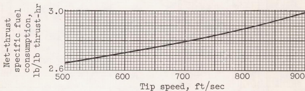
(c) Specific fuel consumption for gas turbine plus tip burner.
