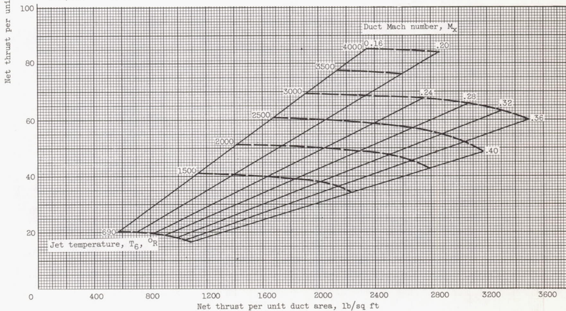
Figure 5. - Continued. Power-available chart.
