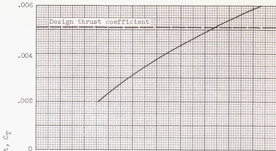
(a) Hovering performance.
