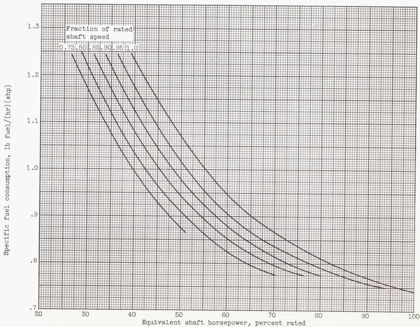
Figure 3. - Specific fuel consumption of gas turbine as function of equivalent shaft horsepower and shaft speed.
