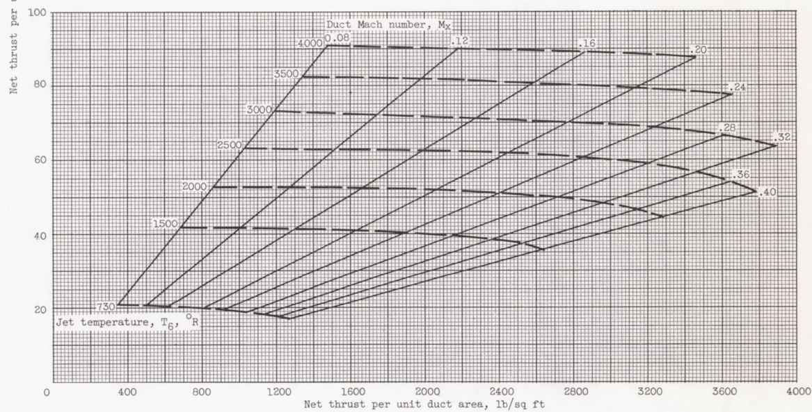
(n) Variable-area tip-jet nozzle; pressure ratio, 3.0; tip speed, 900 feet per second; \Delta P_f = 2.5q_x ; burner area/duct area, 1.5.
