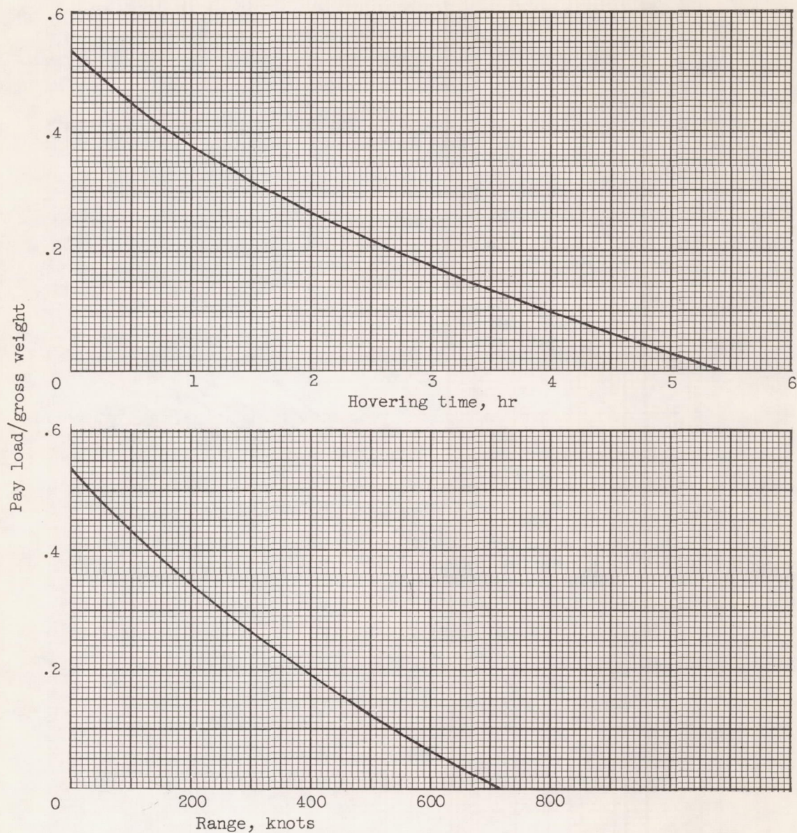
Figure 18. - Flight performance as function of pay load. Pressure ratio, 3.0; design jet temperature, 3000^{\circ} R; tip speed, 700 feet per second; duct area/section area, 0.3; burner area/section area, 0.45.
