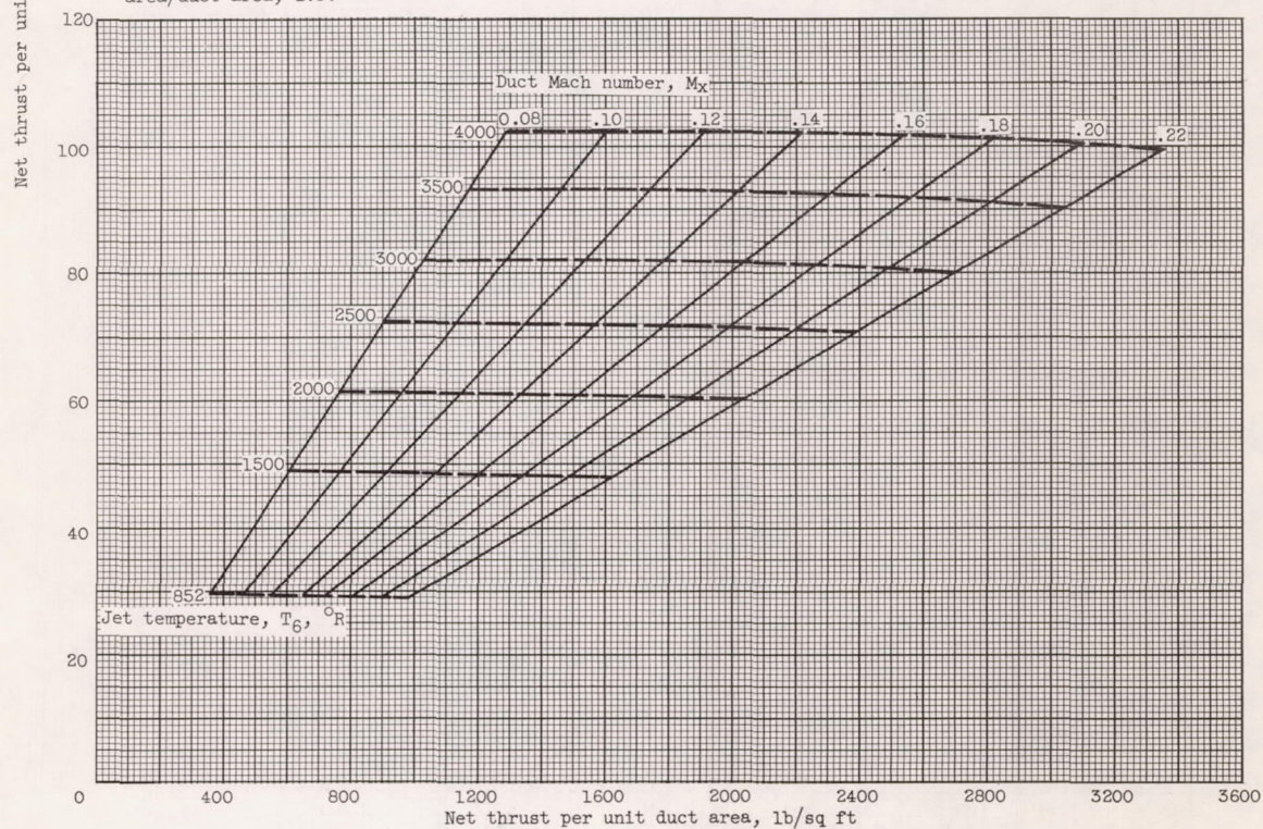
Figure 5. - Continued. Power-available chart.
