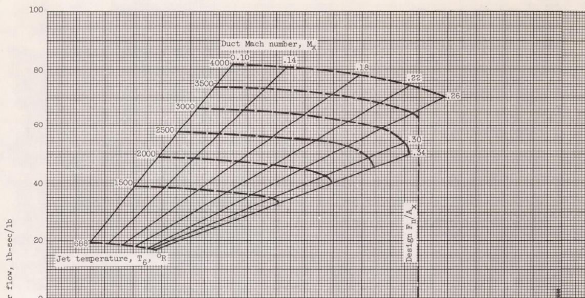
(g) Variable-area tip-jet nozzle; pressure ratio, 2.25; tip speed, 700 feet per second; \Delta P_r = 2.5q_x ; burner area/duct area, 1.5.
