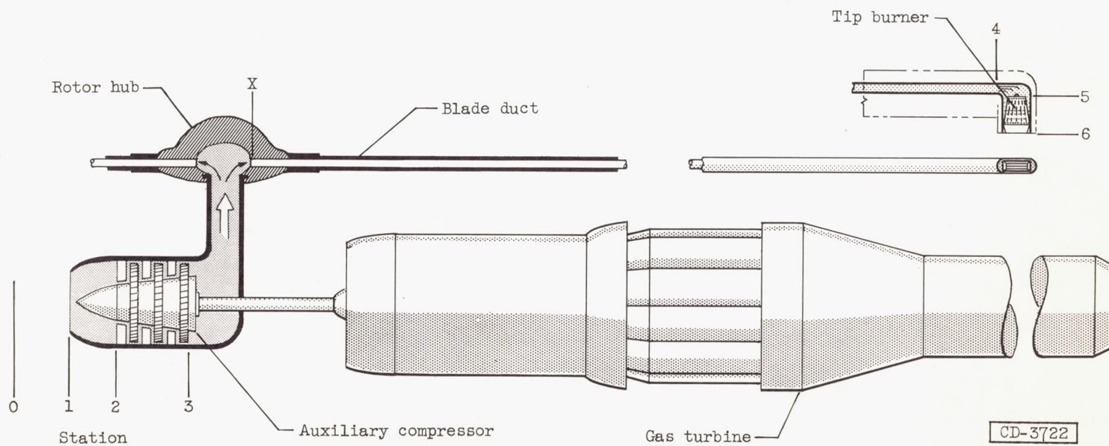
Figure 1. - Schematic of pressure-jet components.
