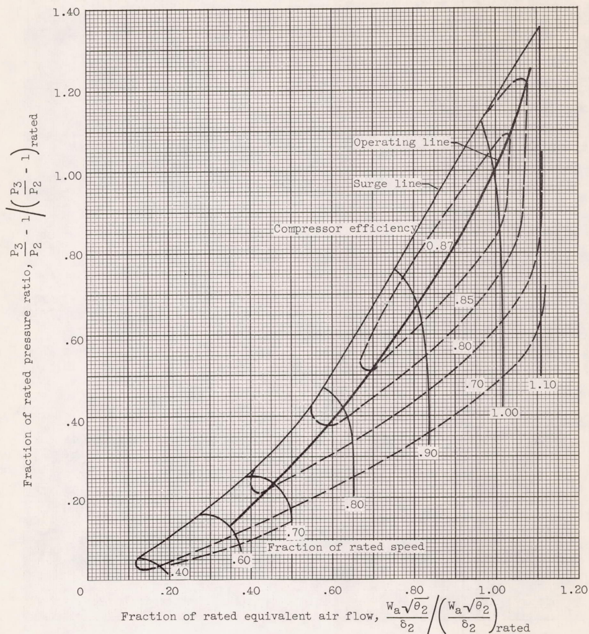
Figure 4. - Performance map for pressure-jet auxiliary compressor.
