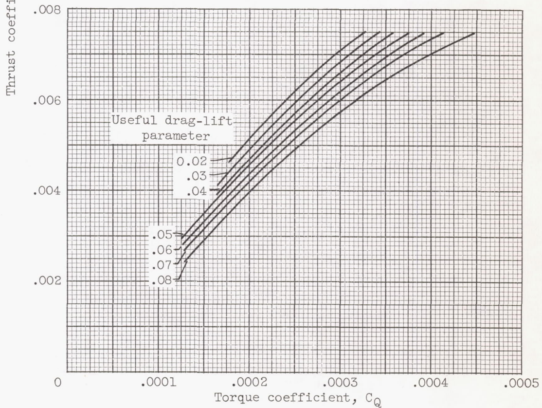
(b) Forward flight performance.
