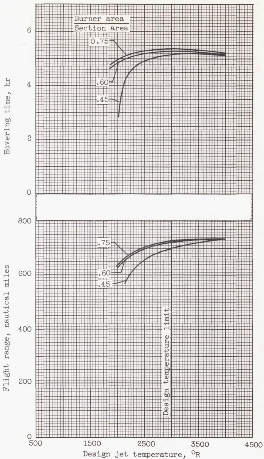
Figure 13. - Effect of burner area on flight performance. Design pressure ratio, 2.5; tip speed, 700 feet per second; duct area/section area, 0.3.
