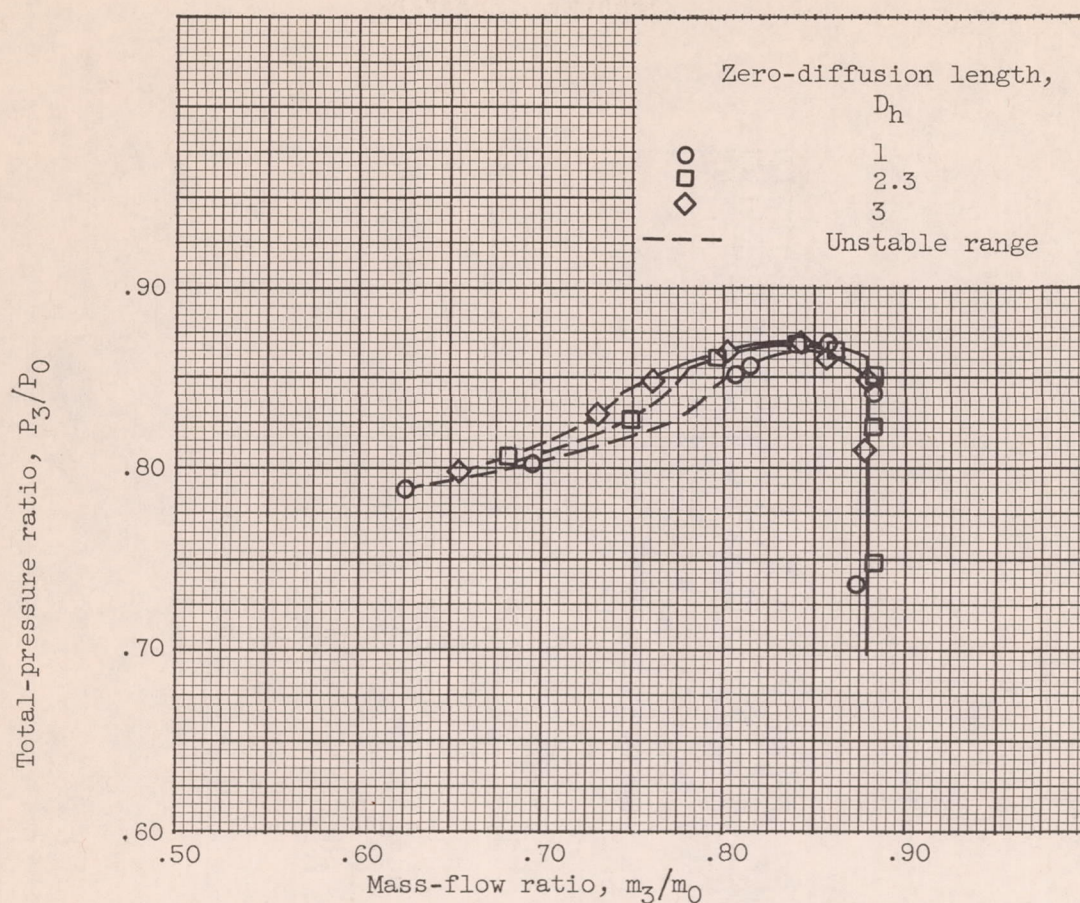
(a) Over-all performance.
