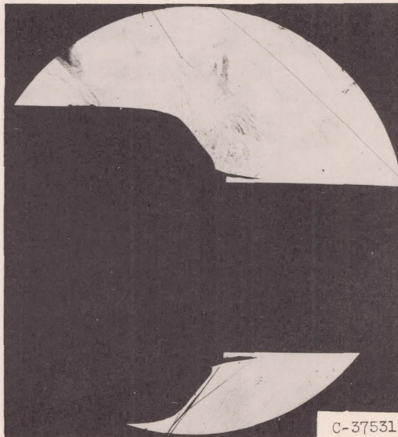
(d) Mass-flow ratio m_3/m_0 , 0.373; total-pressure ratio P_3/P_0 , 0.571.
