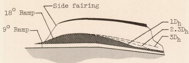
(a) Variations to subsonic diffuser.
