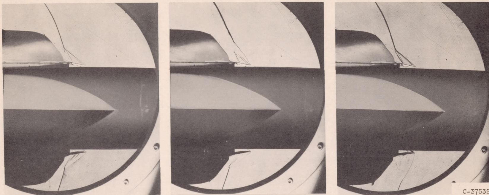
(b) Mass-flow ratio m_3/m_0 , 0.519; total-pressure ratio P_3/P_0 , 0.762.
