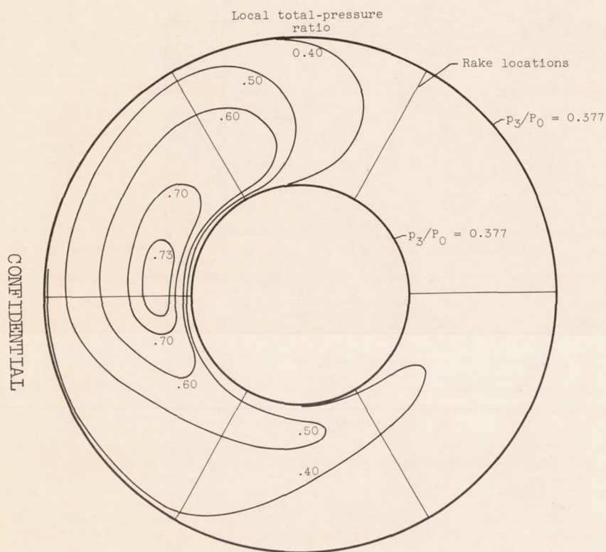
(a) Zero-degree second-ramp inlet; mass-flow ratio m_3/m_0 , 0.338; total-pressure ratio P_3/P_0 , 0.393.
