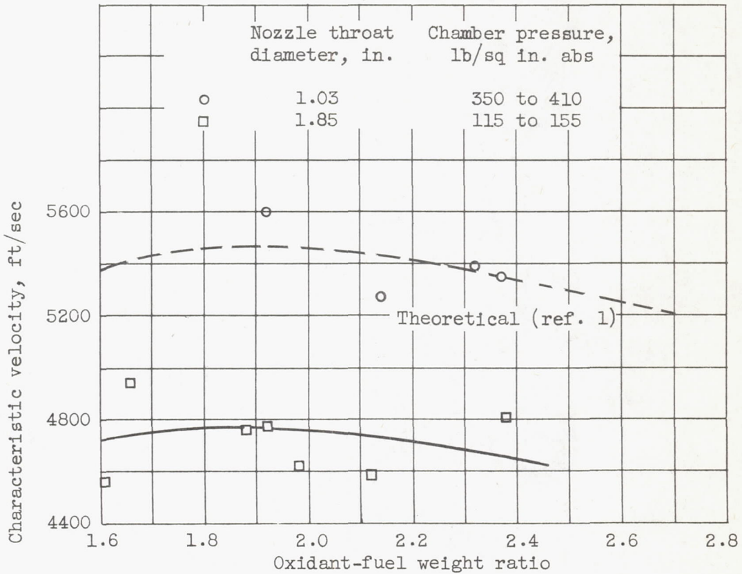
Figure 13. - Experimental characteristic velocity of mixed oxides of nitrogen and ammonia for two ranges of chamber pressure. Thrust, 200 to 480 pounds; two-entry swirl-cup injector.
