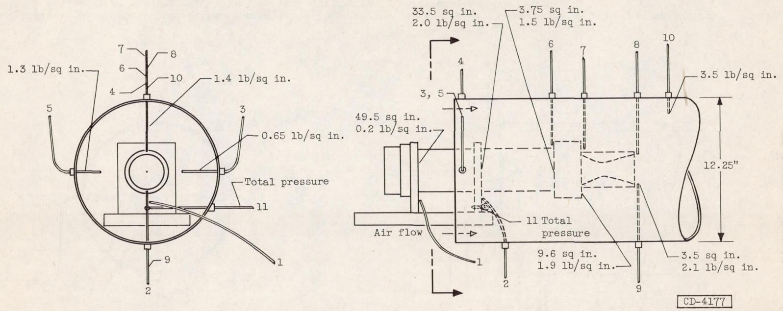
Figure 7. - Open-entrance exhaust duct and engine assembly showing locations of pressure measurements. Values given for typical partial vacuums and for areas affected.
