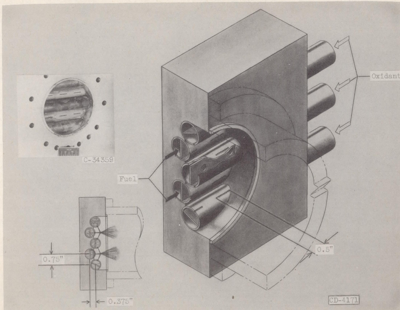
Figure 3. - Triplet impinging jet injector.
