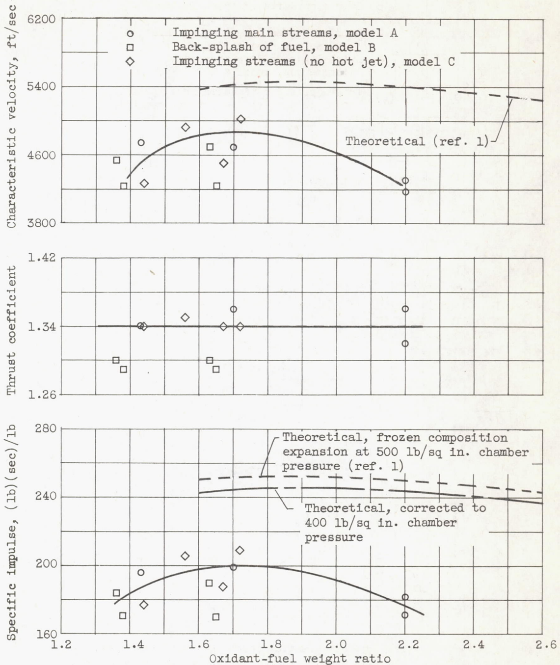
Figure 11. - Theoretical and experimental performance of mixed oxides of nitrogen and ammonia. Thrust, 1400 pounds; chamber pressure, 400 pounds per square inch absolute; hot-jet mixing injector; thrust data corrected for exhaust-duct effects (see appendix).
