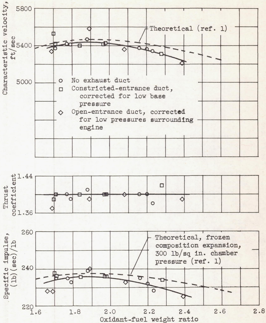
Figure 9. - Concluded. Theoretical and experimental performance of mixed oxides of nitrogen and ammonia. Thrust, 1100 pounds; chamber pressure, 300 pounds per square inch absolute; four-entrancy swirl-cup injector.
