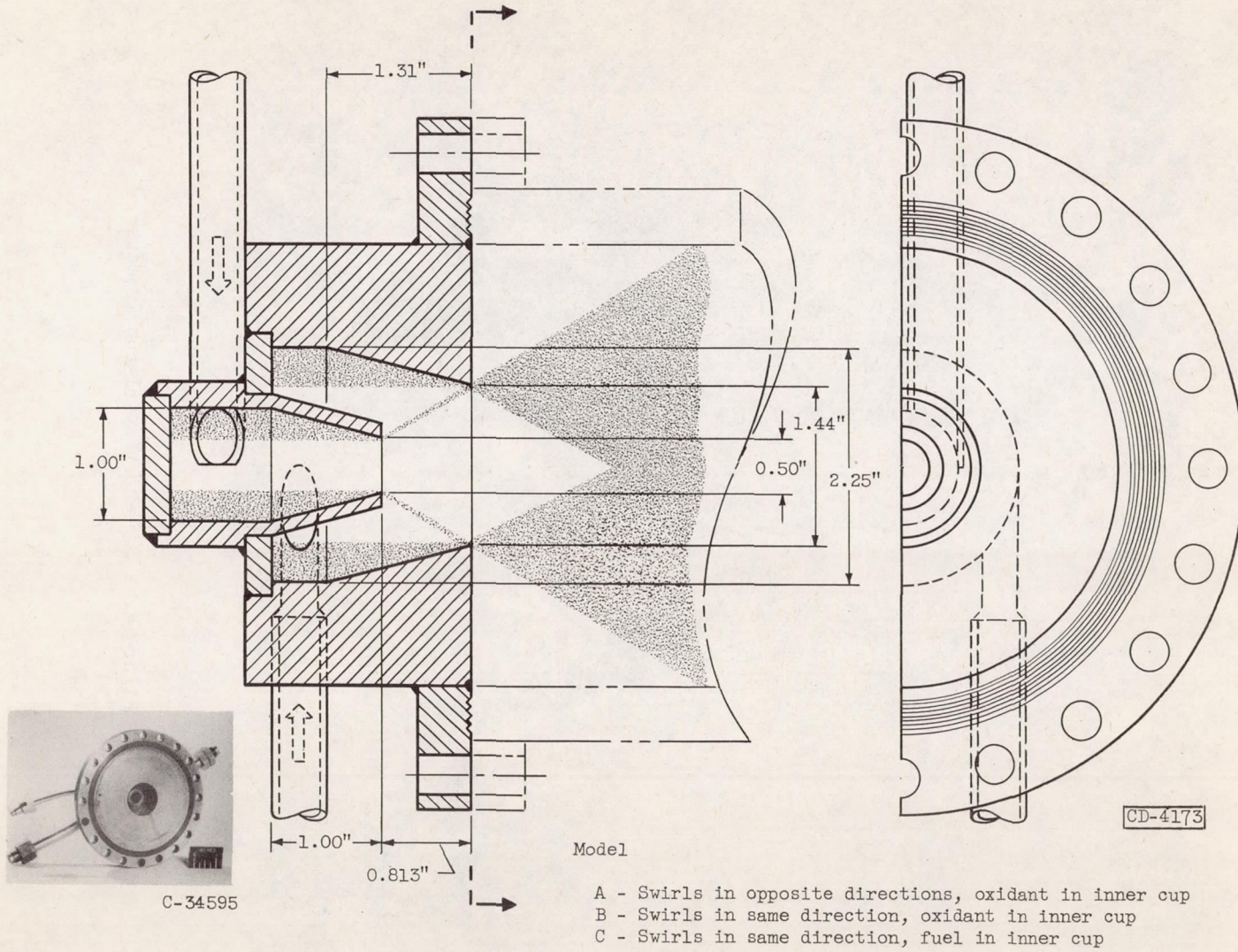
Figure 5. - Concentric swirl injector.
