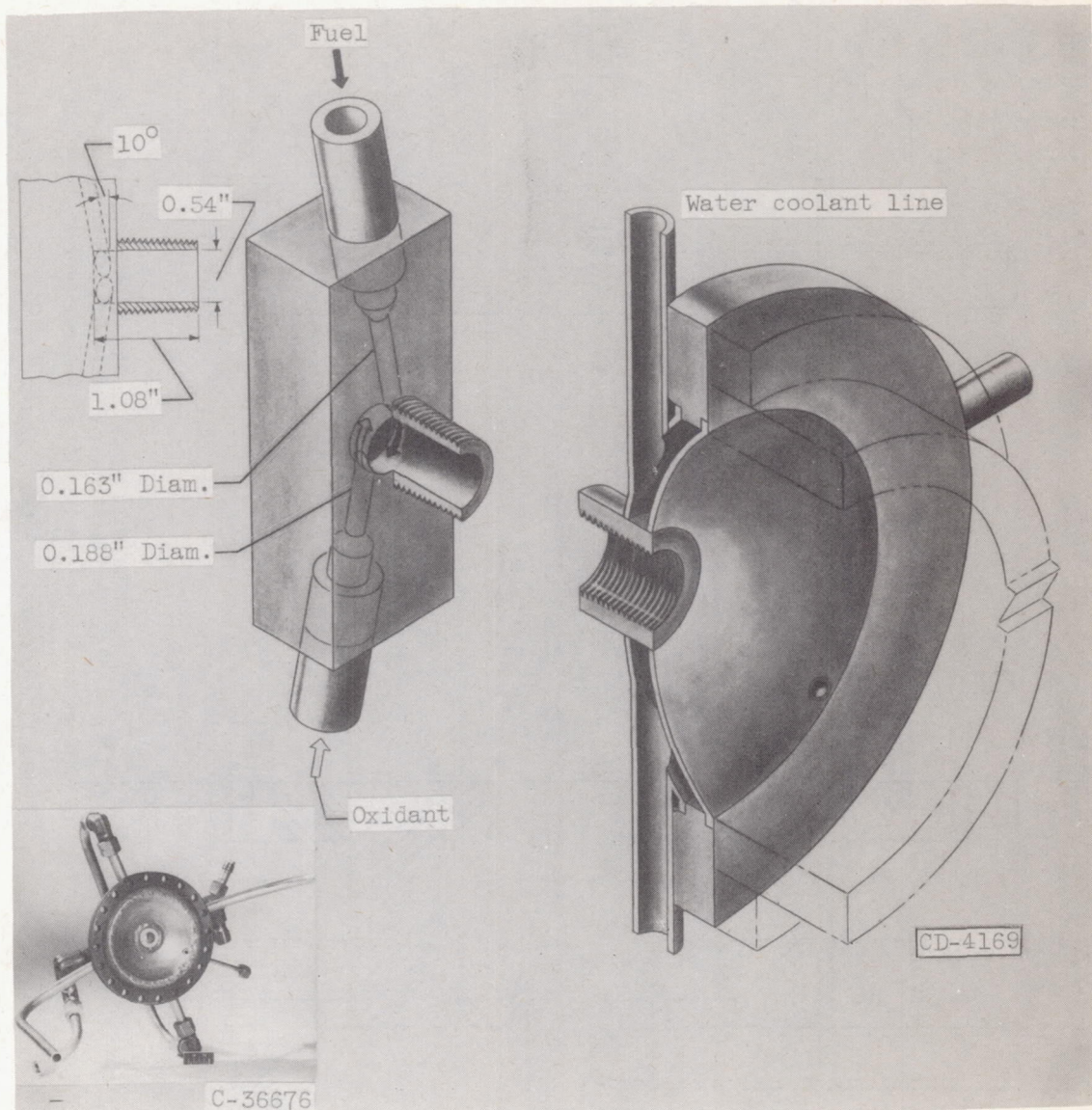
Figure 6. - Two-entry swirl-cup injector.
