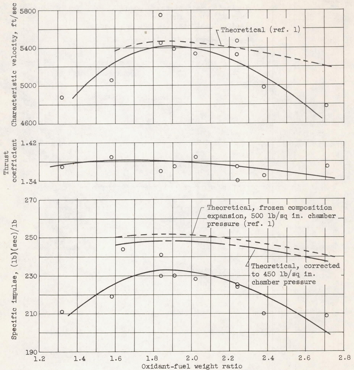
Figure 10. - Theoretical and experimental performance of mixed oxides of nitrogen and ammonia. Thrust, 1600 pounds; chamber pressure, 450 pounds per square inch absolute; triplet impinging jet injector; thrust data corrected for exhaust-duct effects (see appendix).
