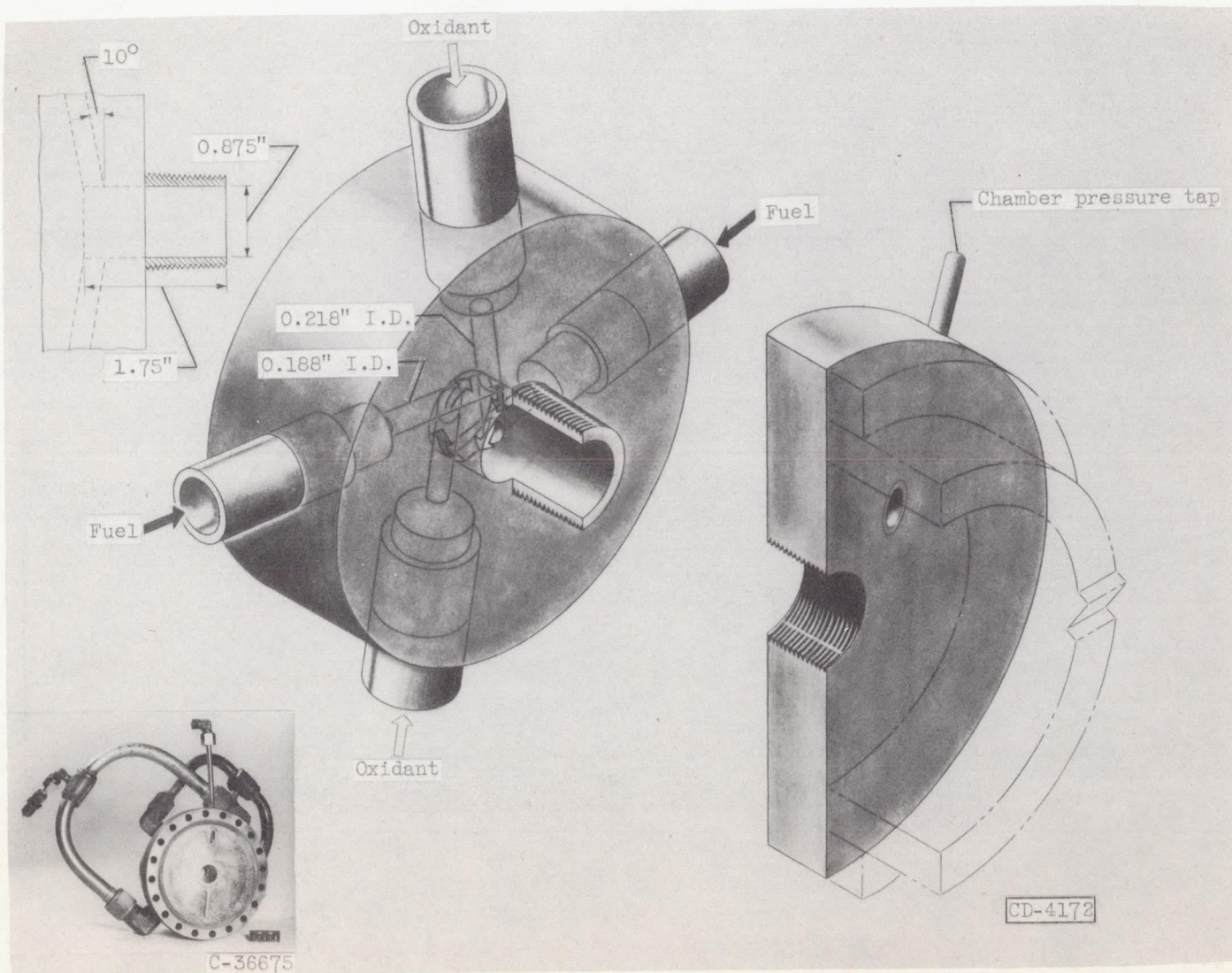
Figure 2. - Four-entry swirl-cup injector.
