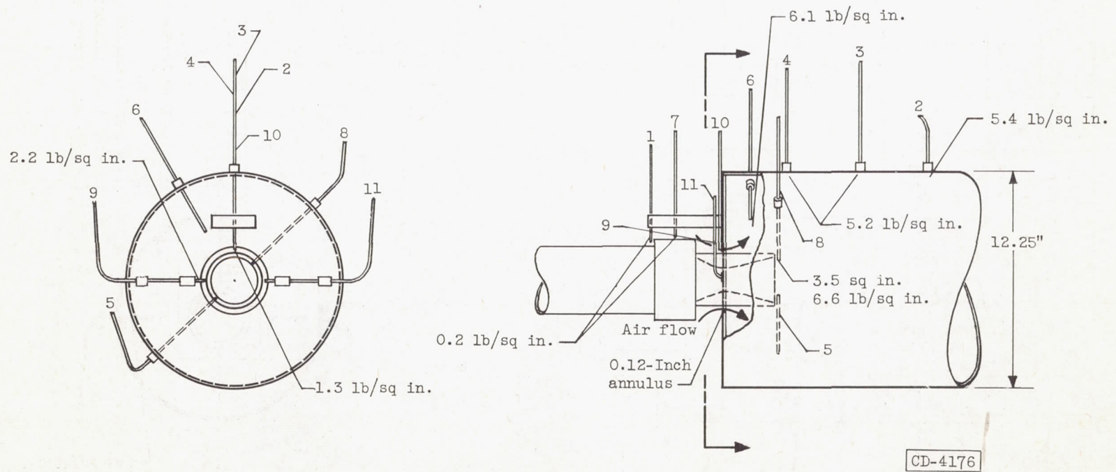
Figure 8. - Constricted-entrance exhaust duct and engine assembly showing locations of pressure measurements. Values given for typical partial vacuums and for areas affected.
