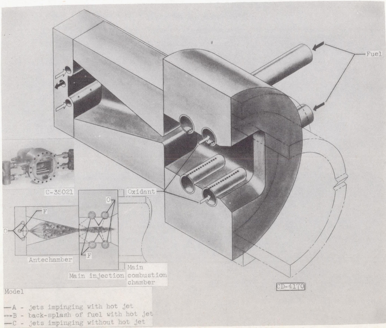
Figure 4. - Hot-jet mixing injector.
