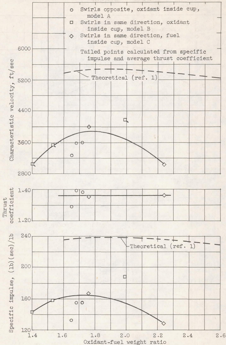
Figure 12. - Theoretical and experimental performance of mixed oxides of nitrogen and ammonia. Thrust, 1000 pounds; chamber pressure, 300 pounds per square inch absolute; concentric swirl injector; thrust data corrected for exhaust-duct effects (see appendix).
