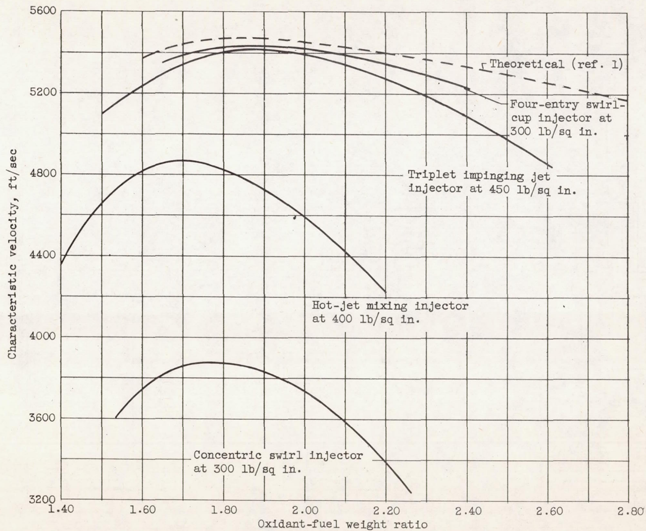
Figure 14. - Theoretical and experimental characteristic velocity of mixed oxides of nitrogen and ammonia for several injectors over a range of conditions.
