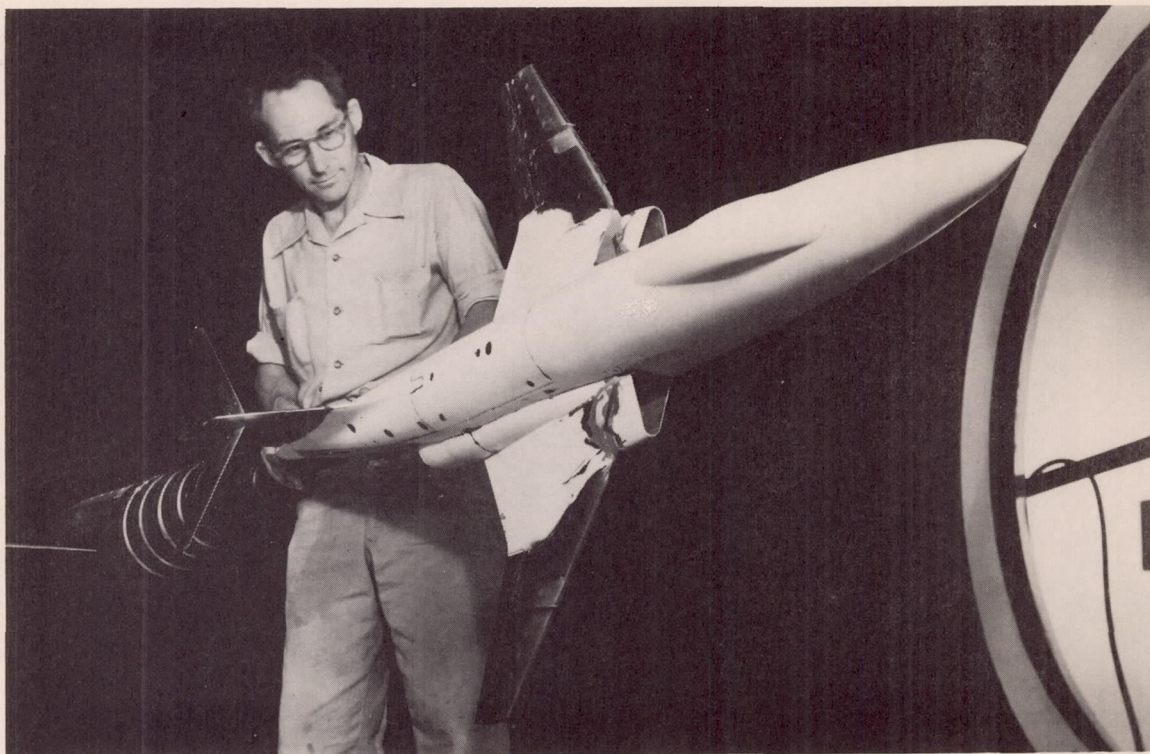
Figure 1.- The air-induction model in the Ames 6- by 6-foot supersonic wind tunnel.
