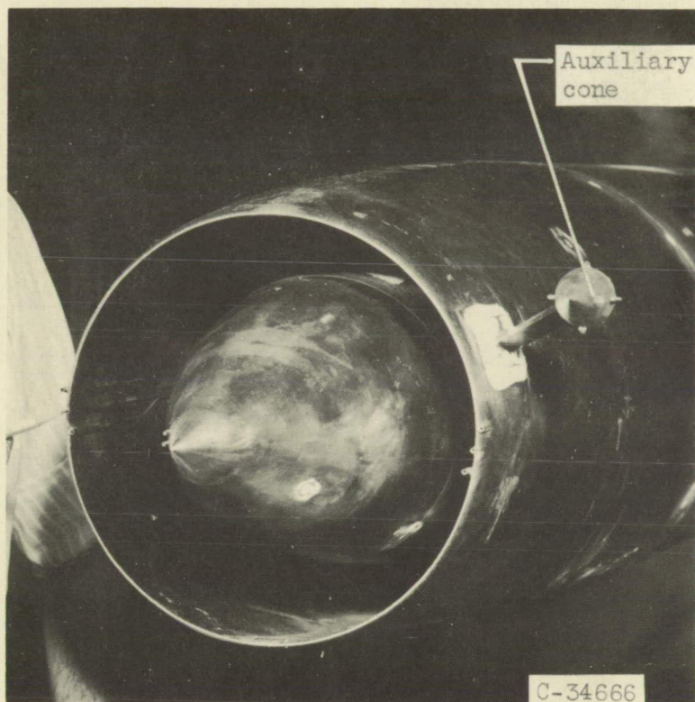
Figure 11. - Front view of 16-inch ram-jet engine showing auxiliary cone.
