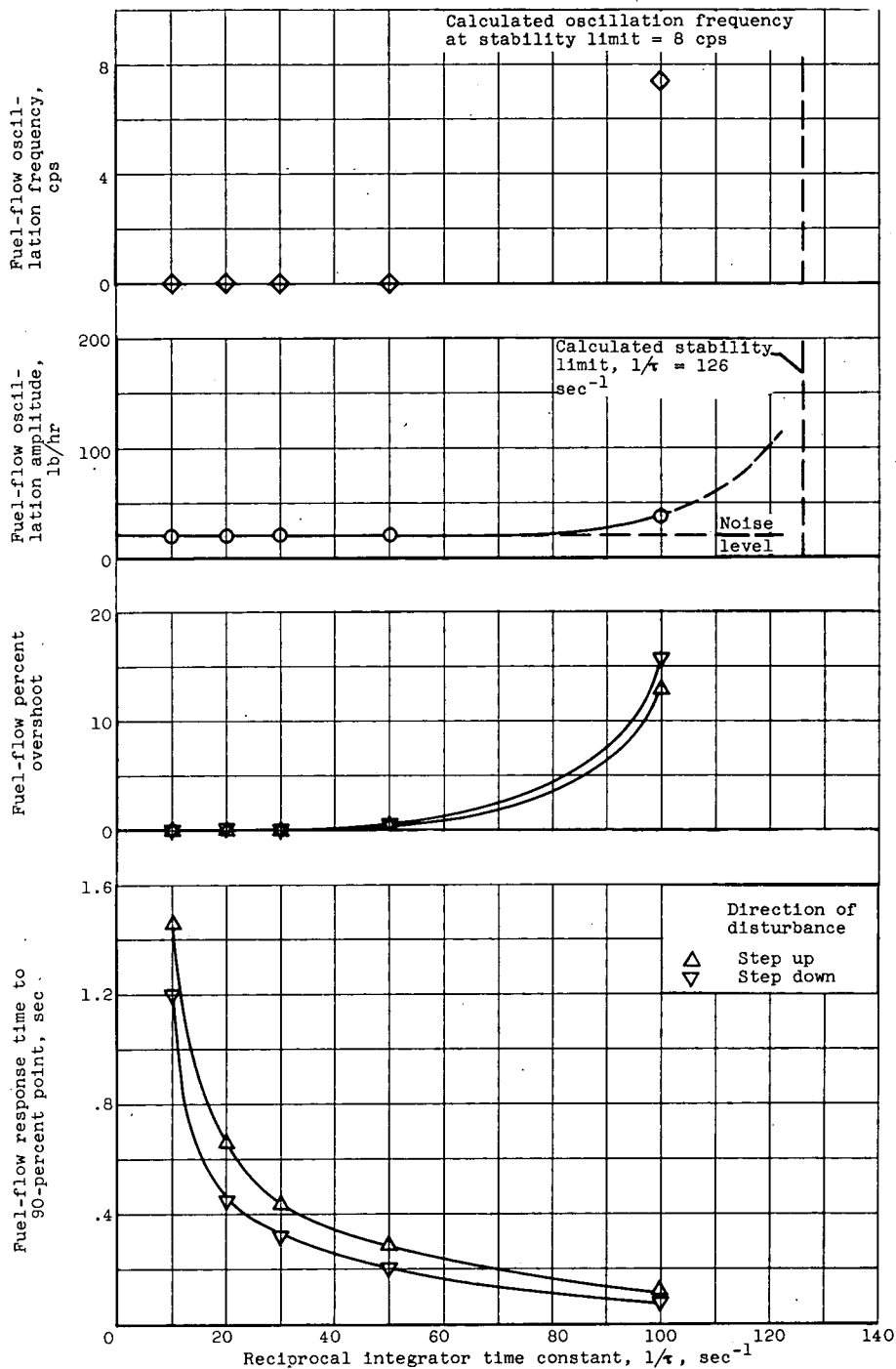
Figure 18. - Concluded. System response characteristic to step disturbance in input voltage to fuel servo of \pm 2 volts (i.e., fuel-flow step, \pm 556 \text{ lb/hr} ). Flight Mach number, 1.5; zero angle of attack; 0.9 P_{ac} schedule.
