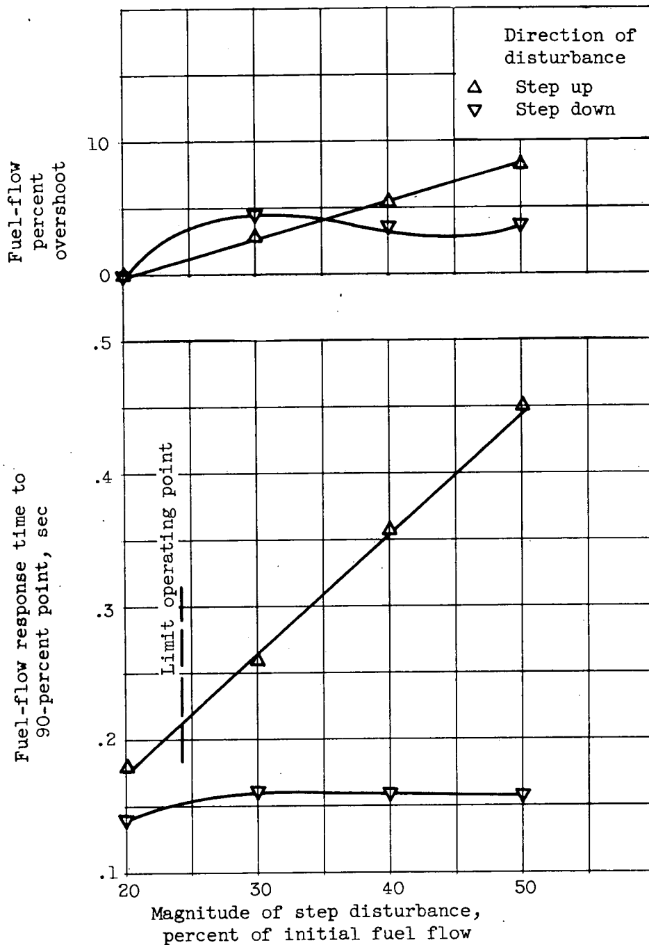
Figure 23. - Control-system response as function of magnitude of disturbance with fixed maximum fuel-flow limit. Flight Mach number, 1.7; zero angle of attack; 0.9 P_{ac} schedule; loop gain, 0.337; 1/\tau , 50 \text{sec}^{-1} ; initial fuel flow, 2793 pounds per hour.
