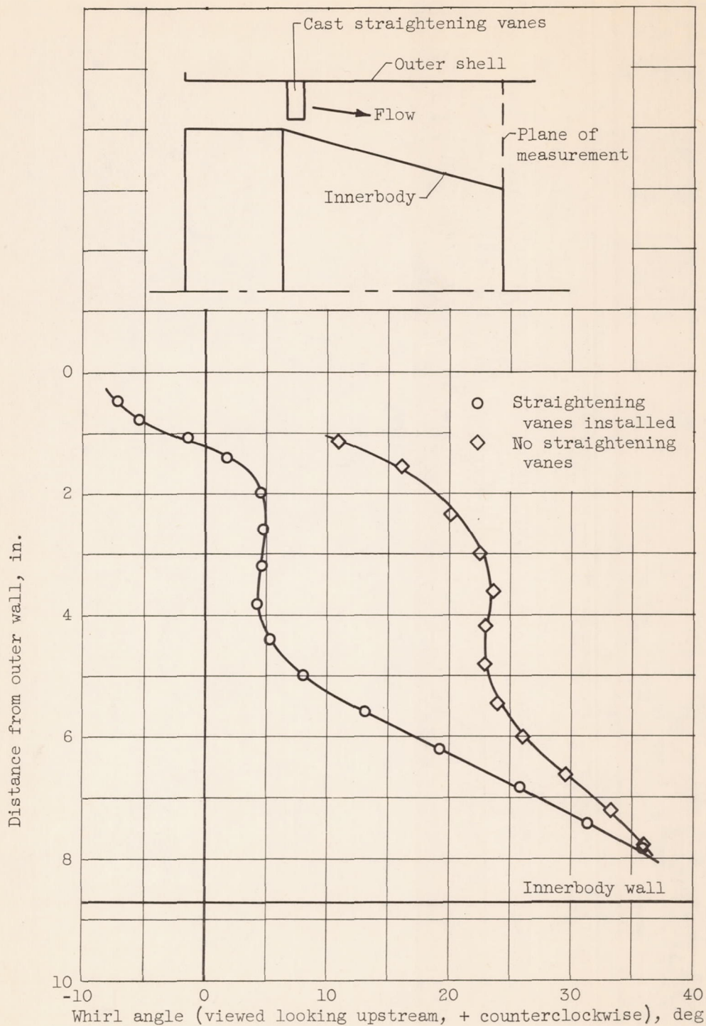
(a) Whirl profiles at diffuser outlet.
