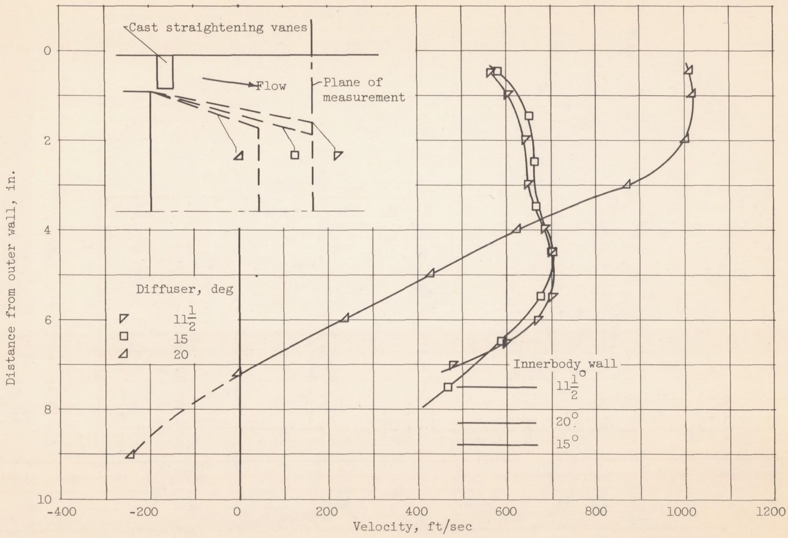
Figure 10. - Comparison of velocity profiles of three diffusers with cast straightening vanes installed.
