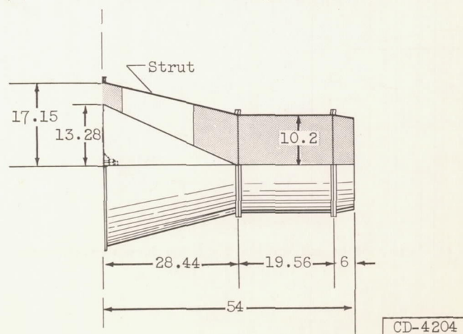
(c) Standard tail pipe.
