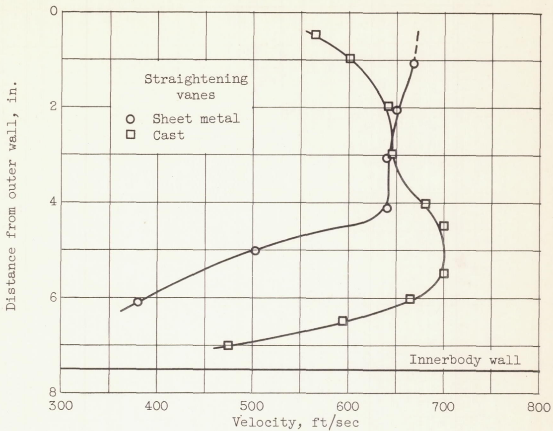
(b) Velocity profiles.
