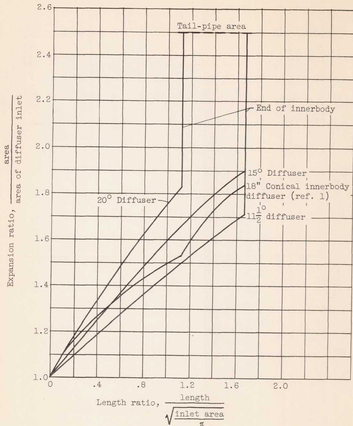
Figure 8. - Variation of diffuser area with length ratio.
