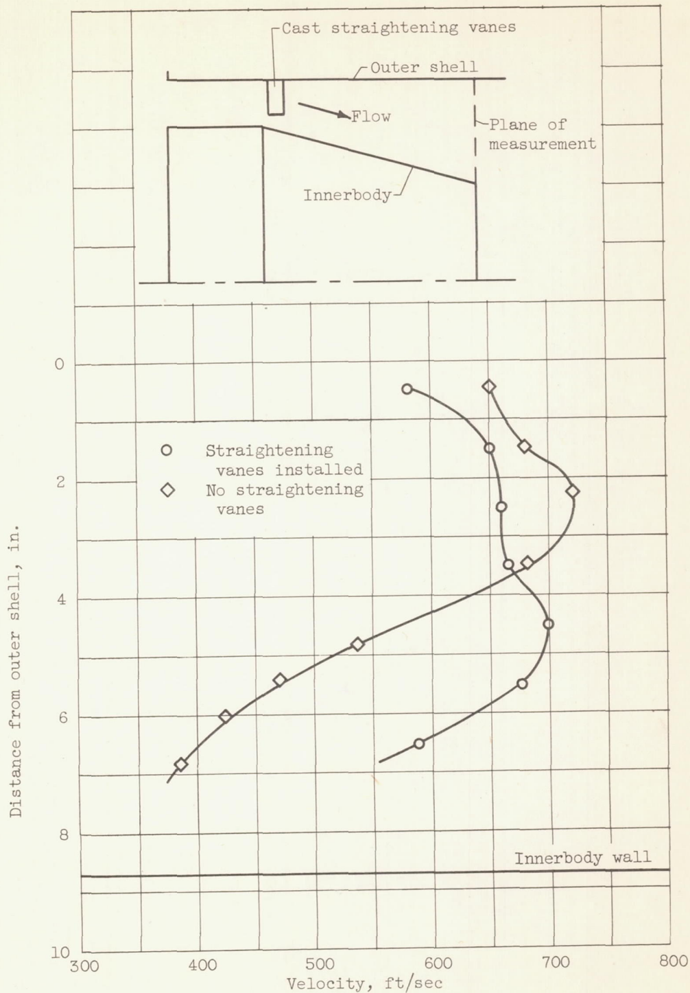
(b) Velocity profiles at diffuser outlet.
