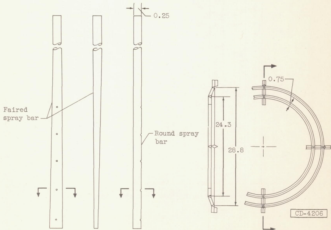
(a) Afterburner assembly details.
