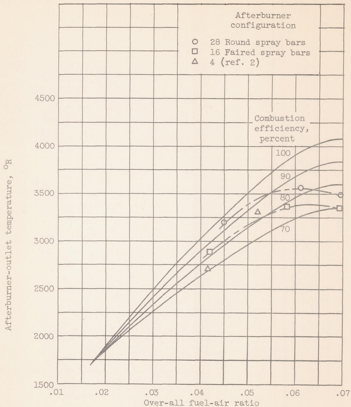
(a) Afterburner-outlet temperature and combustion efficiency.
