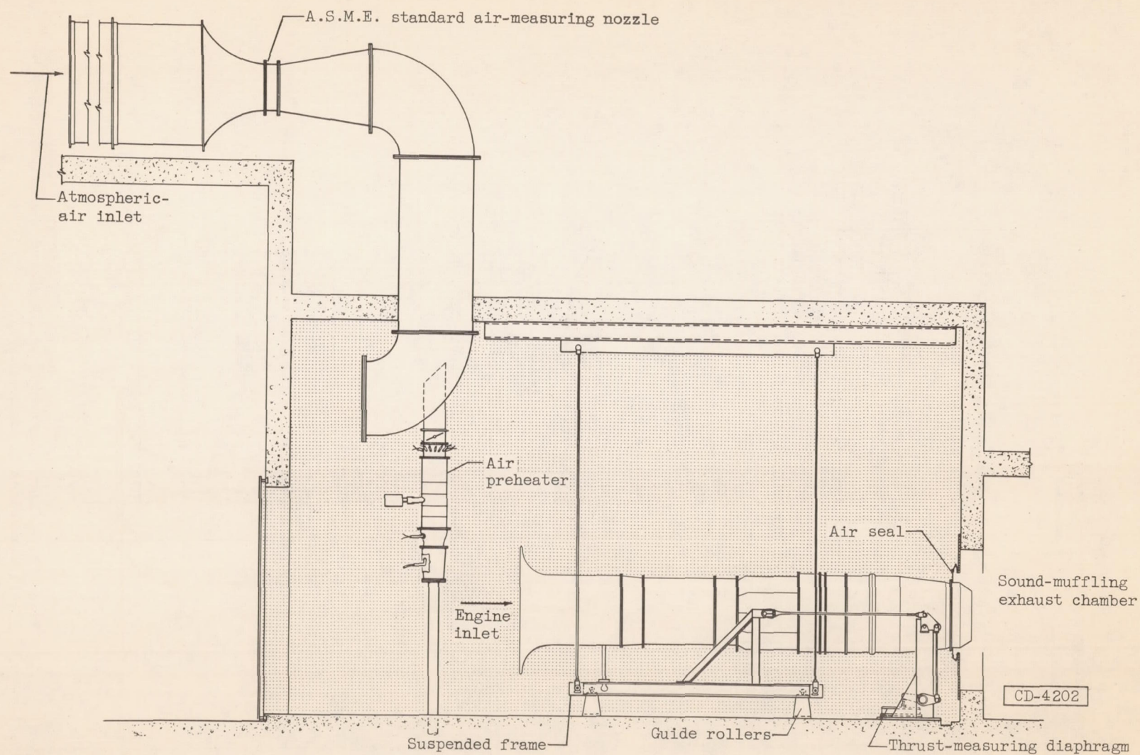
Figure 2. - Schematic diagram of installation of engine in test cell.
