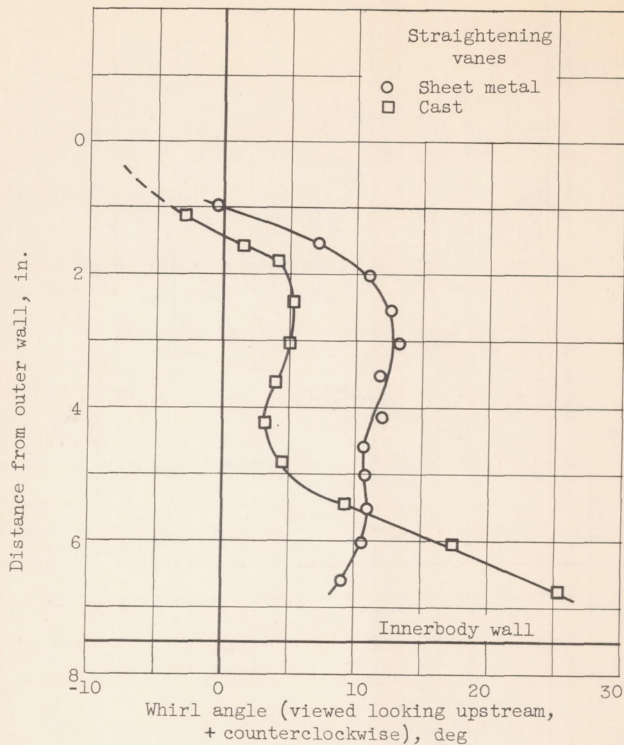
(a) Whirl profile.
