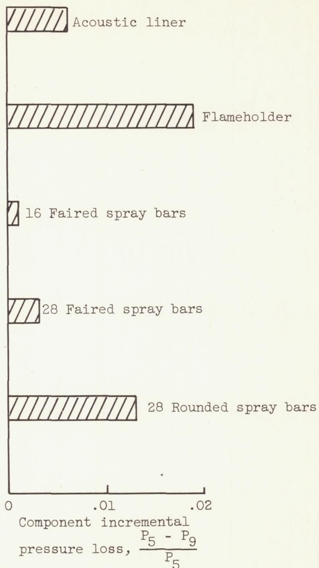
Figure 11. - Afterburner-component pressure losses.
