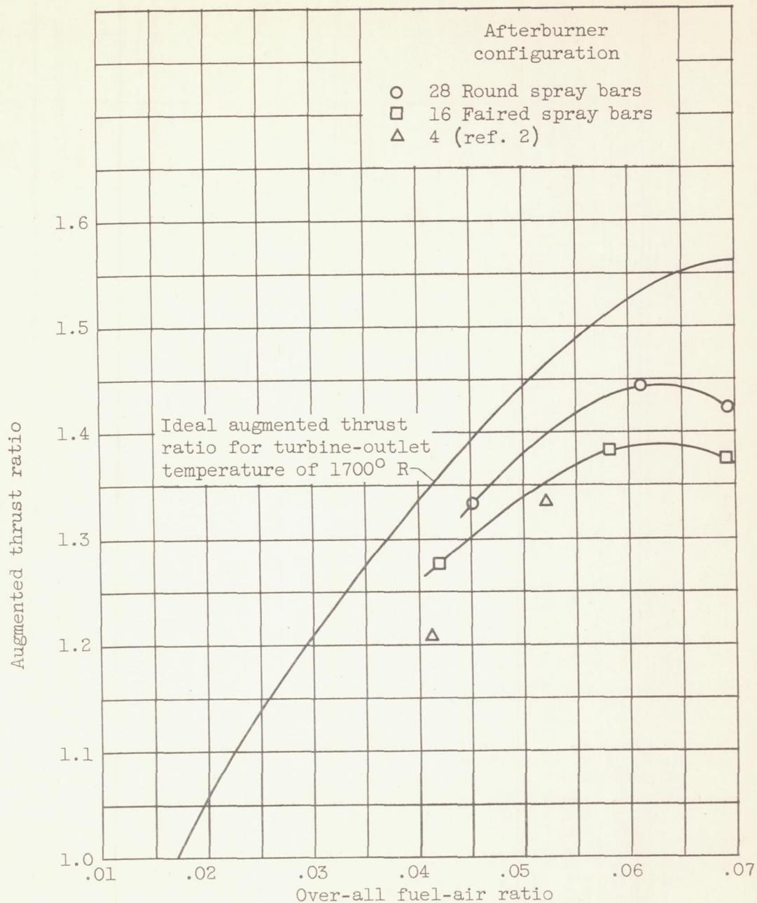
(b) Augmented thrust ratios.
