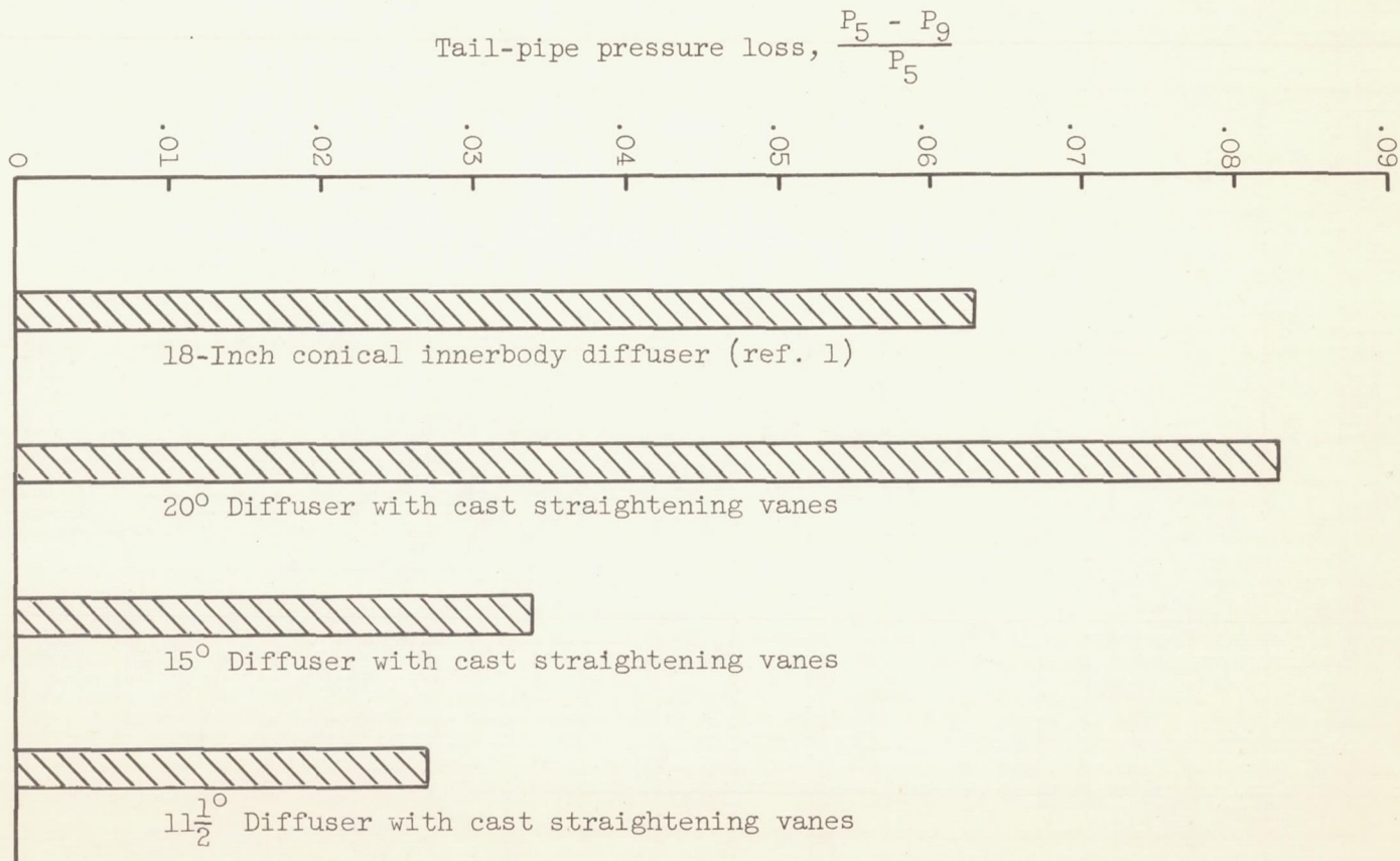
Figure 9. - Comparison of tail-pipe pressure losses of four diffusers.
