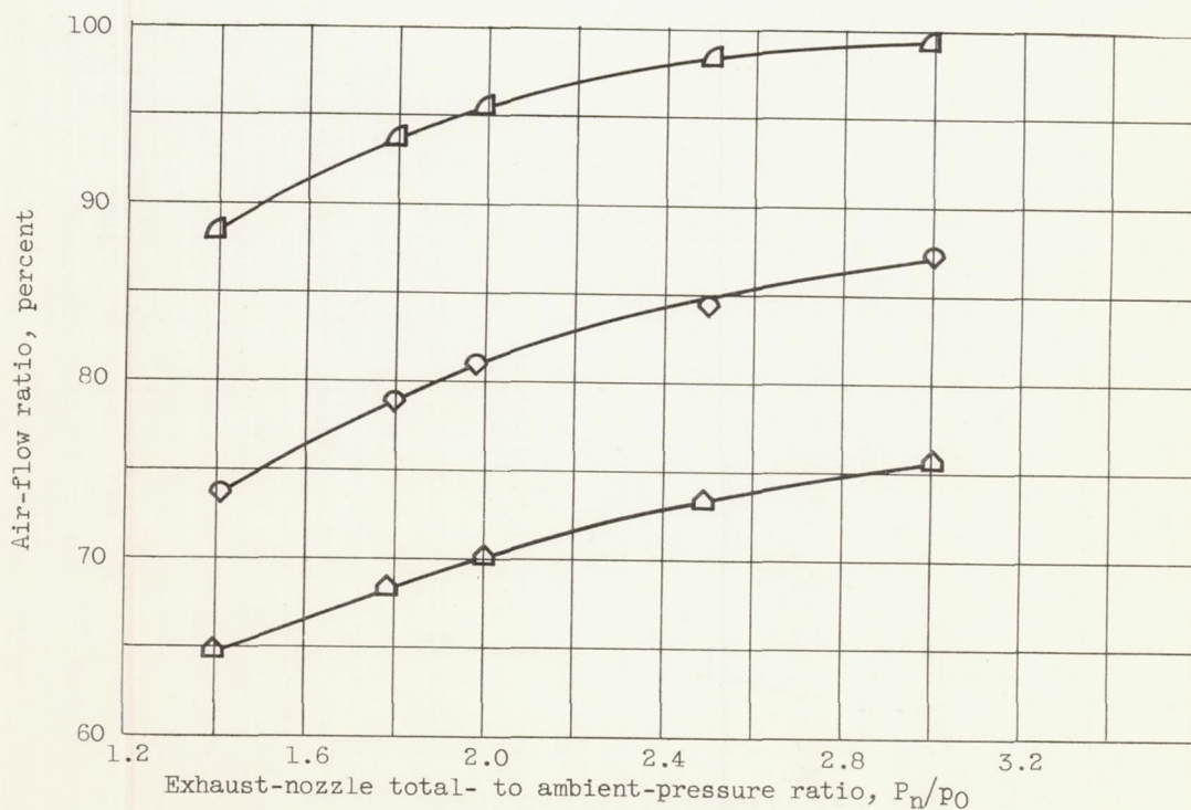
(d) Basic hemisphere diameter, 1.67 basic nozzle diameter; flat-plate-location parameter, 0.50.
