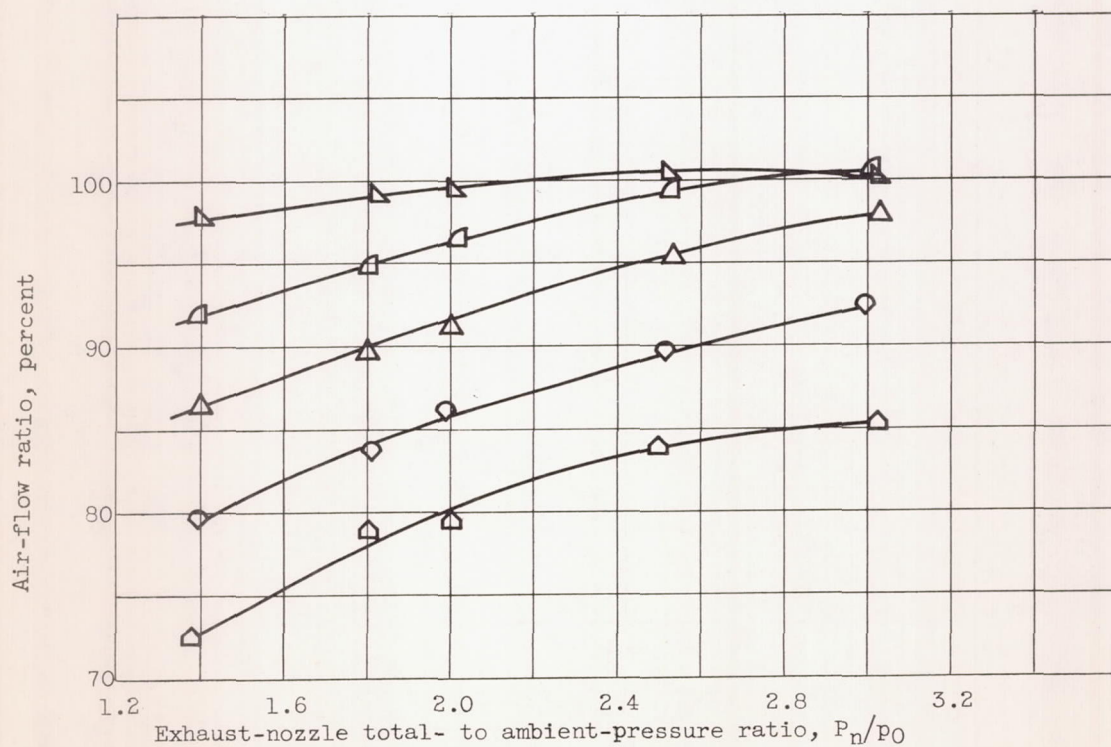
Figure 14. - Continued. Performance of hemispherical thrust reverser.
