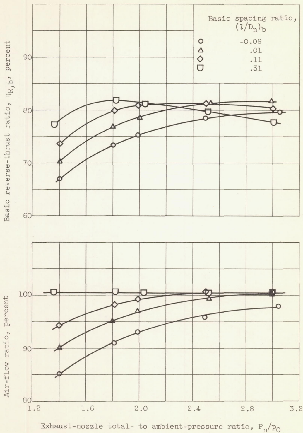
Figure 14. - Continued. Performance of hemispherical thrust reverser.
