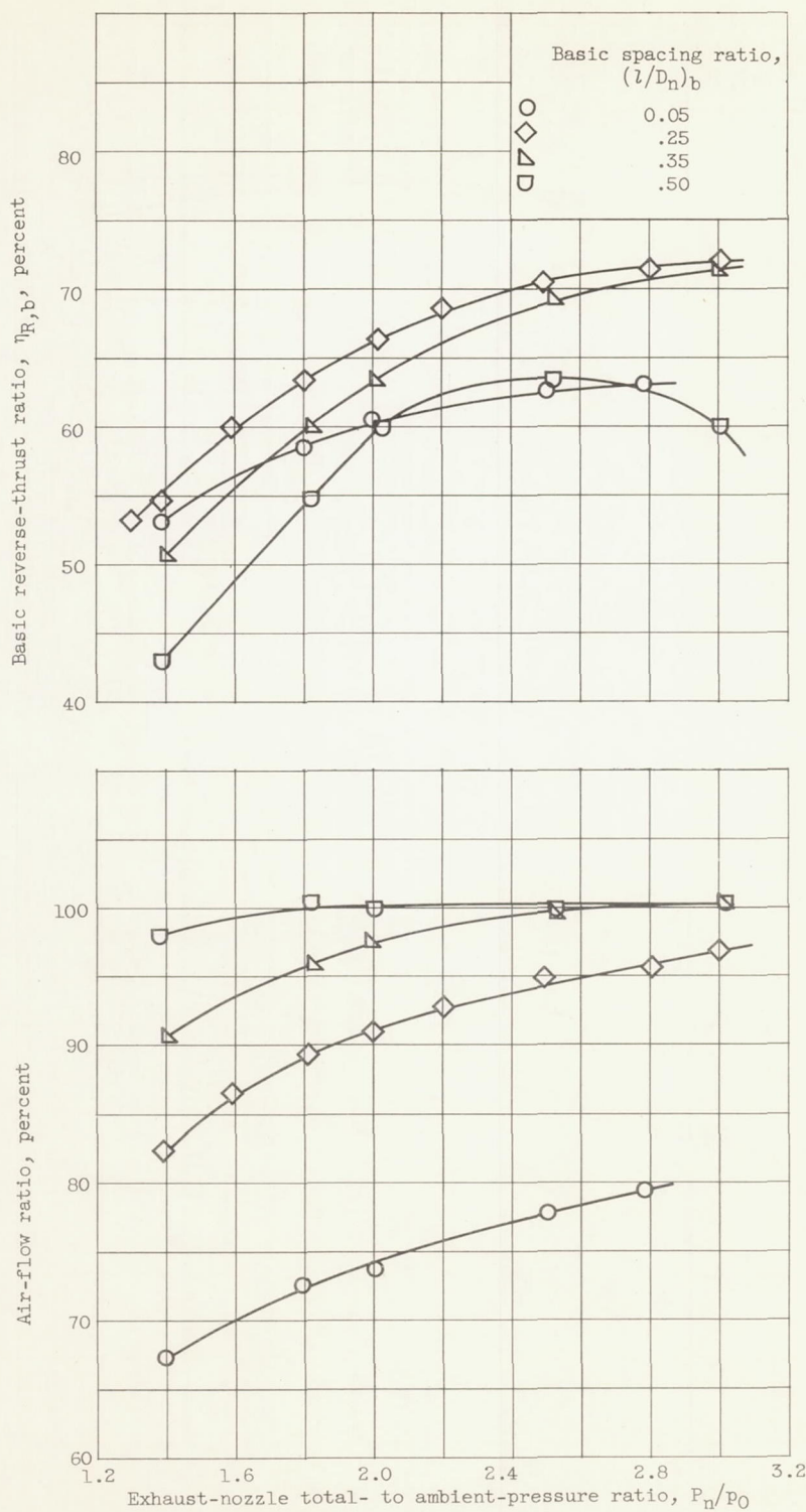
Figure 14. - Continued. Performance of hemispherical thrust reverser.
