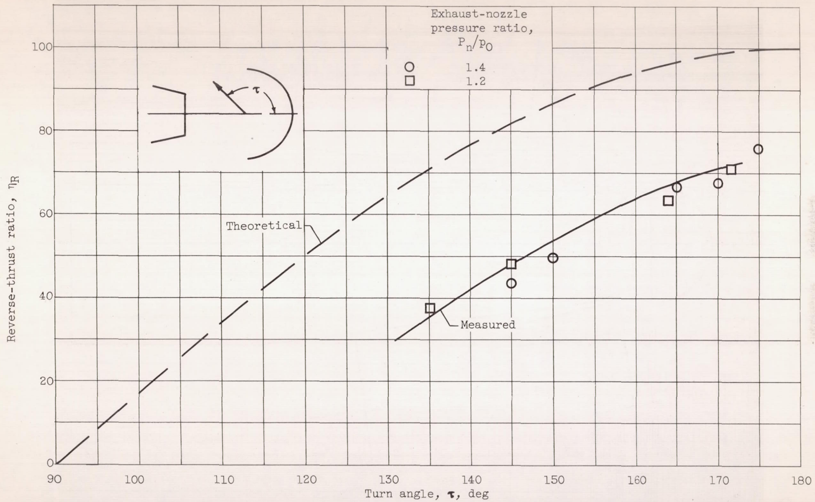
Figure 9. - Relation of reverse-thrust ratio to turn angle.
