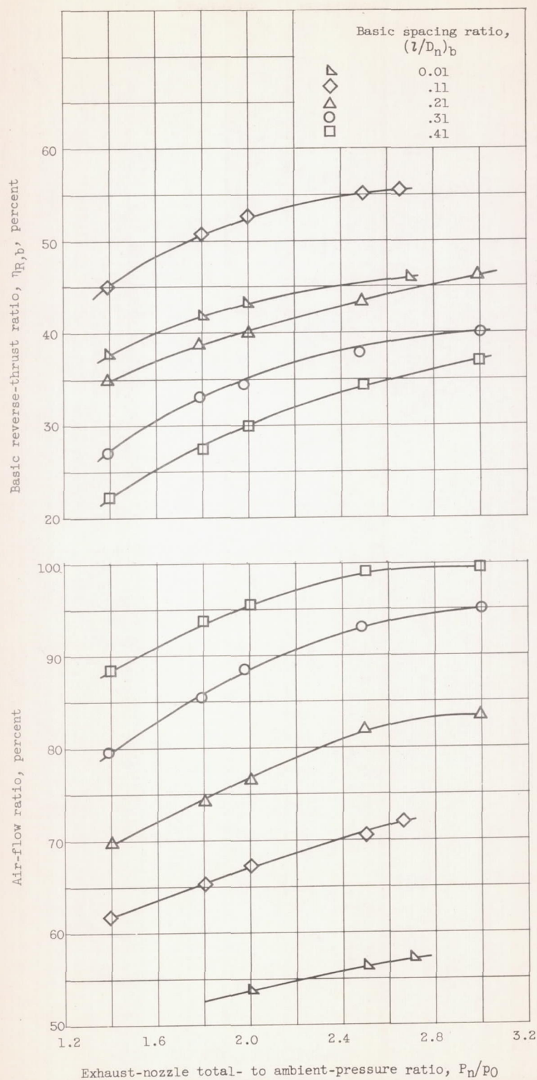
Figure 14. - Performance of hemispherical thrust reverser.
