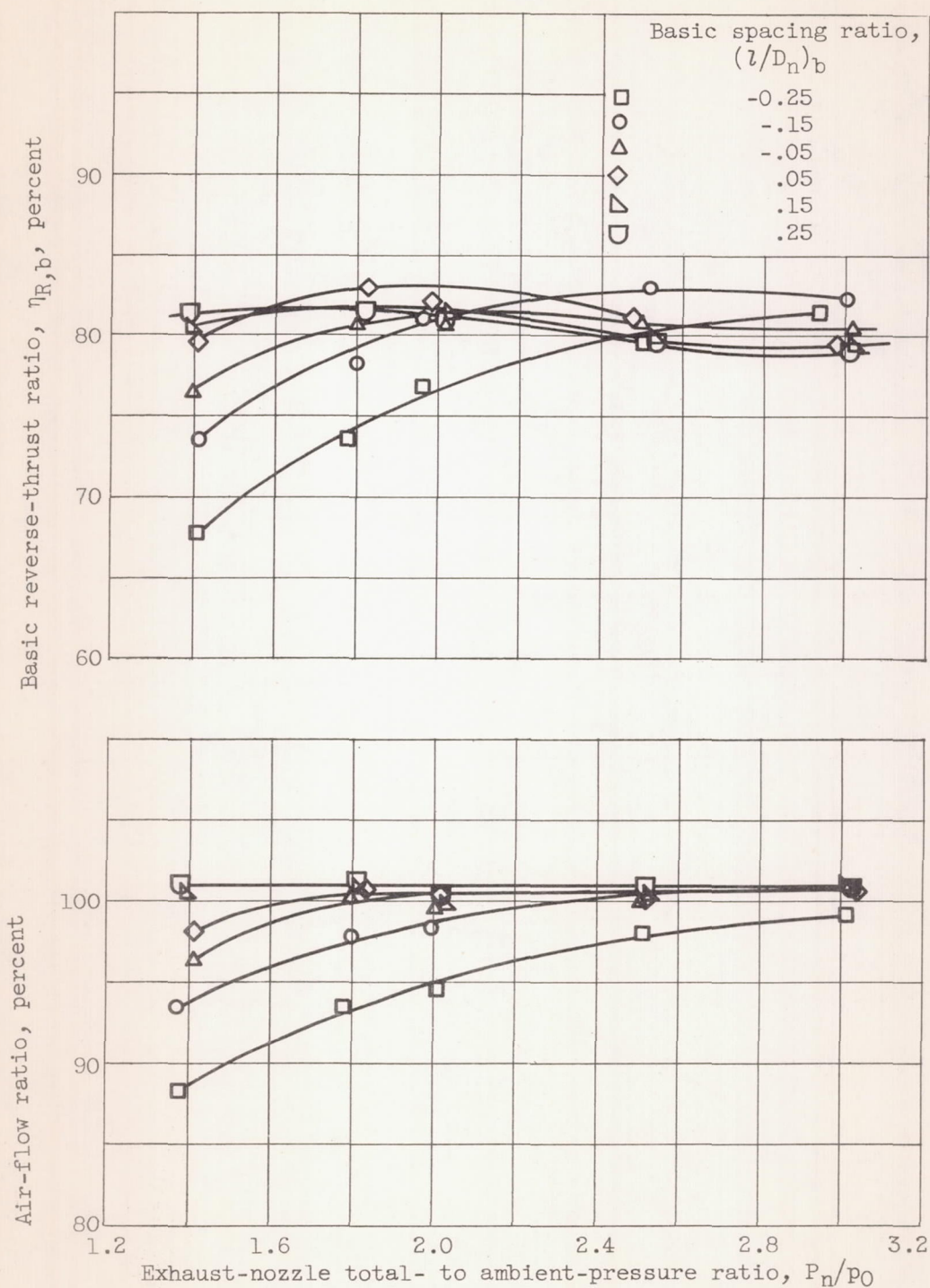
Figure 14. - Continued. Performance of hemispherical thrust reverser.
