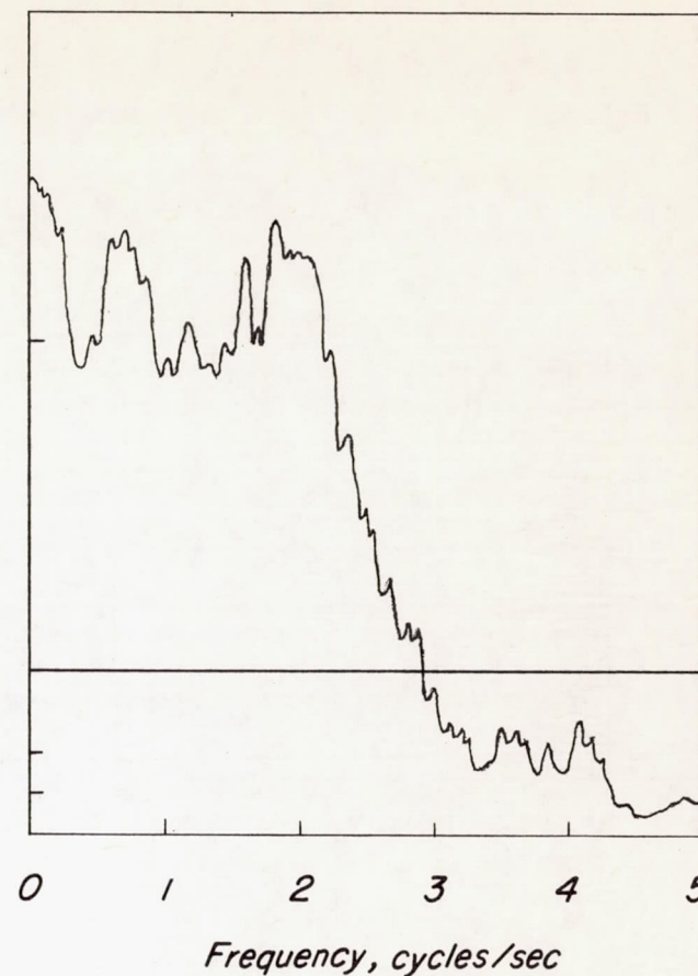
(b) V = 296 ft/sec; K_{\psi'} = 0.5 ; K_{\phi} = 3.5 ; K_{\dot{\psi}} = 0.30 ; K_{\theta'} = 2.2 ; K_{\dot{\theta}} = 0.60 .
