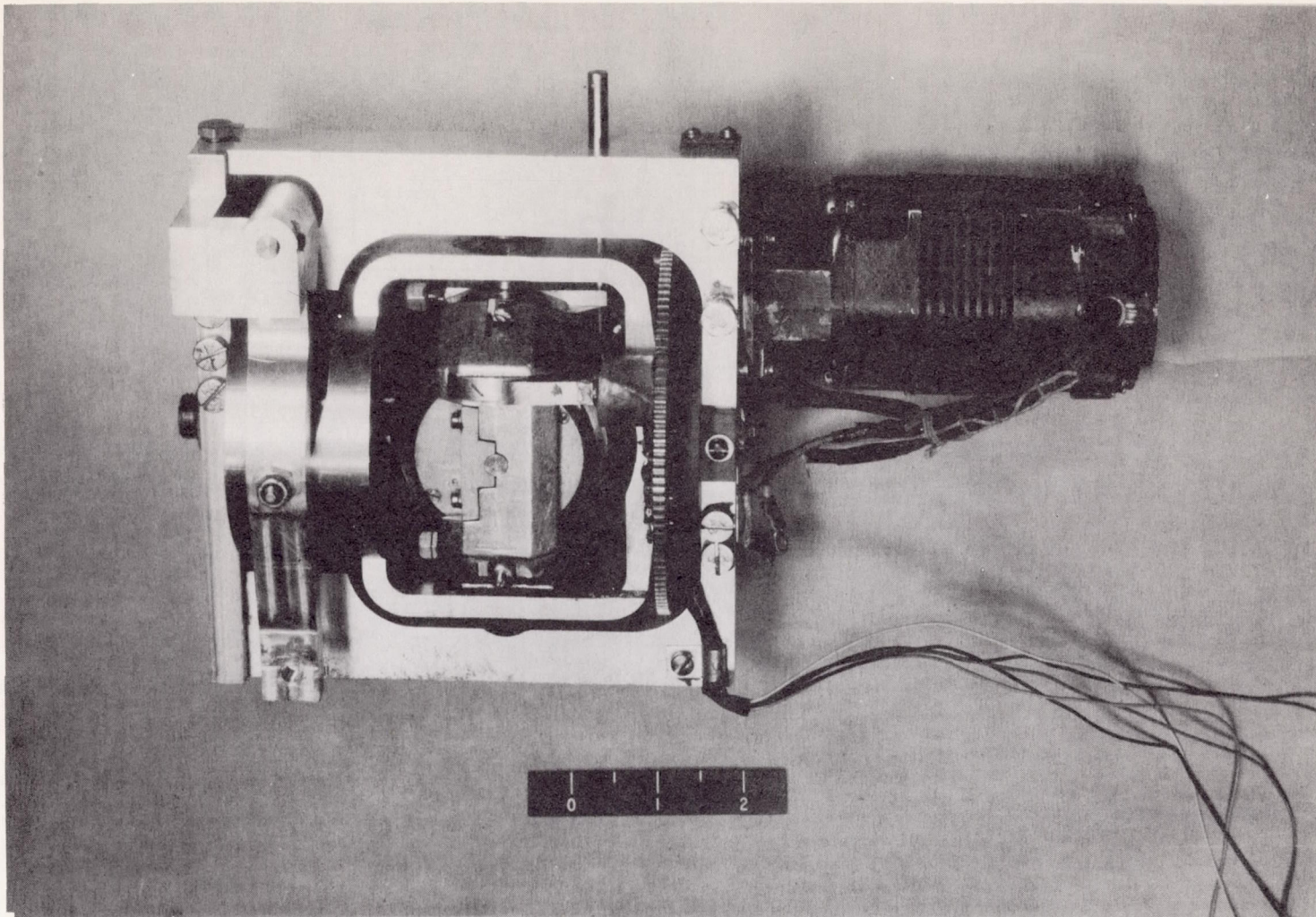
Figure 3.- Photograph of the roll-control autopilot component used in the towed model.
