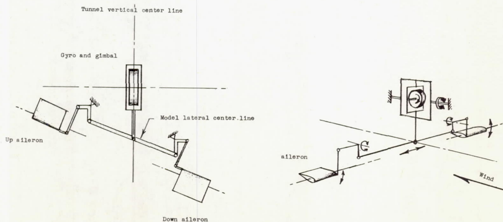
Roll Control
