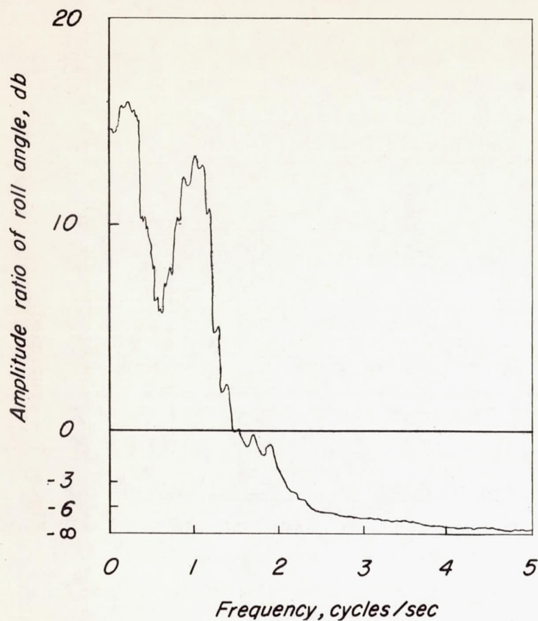
(a) V = 145 ft/sec; K_{\psi'} = 1.0 ; K_{\phi} = 4.0 ; K_{\dot{\psi}} = 0.48 ; K_{\theta'} = 2.6 ; K_{\dot{\theta}} = 0 .
