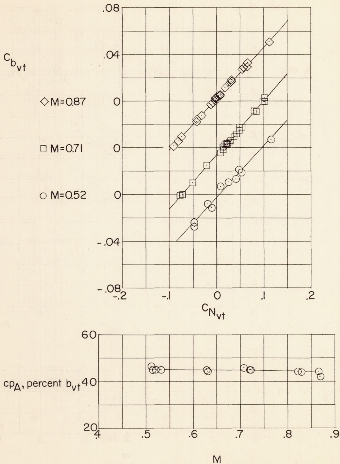
Figure 6.- Variation of vertical-tail bending-moment coefficient with normal-force coefficient and the variation with Mach number of the center of pressure of the additional air load during rudder-fixed oscillations.
