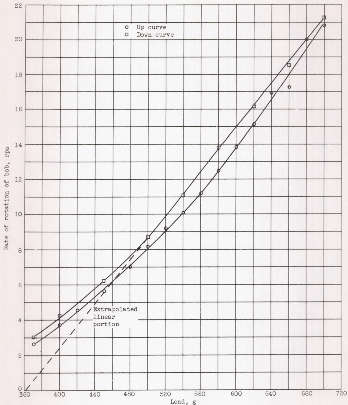
Figure 3. - Continued. Effect of concentration of additive on flow curve of vapor-process-magnesium slurry.
