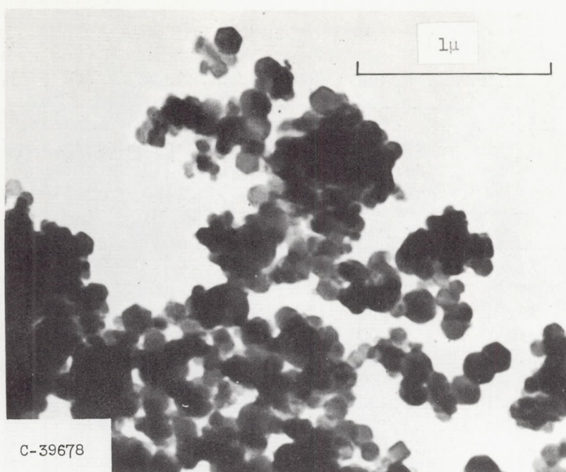
Figure 1. - Electron micrograph of vapor-process magnesium in FP-1.
