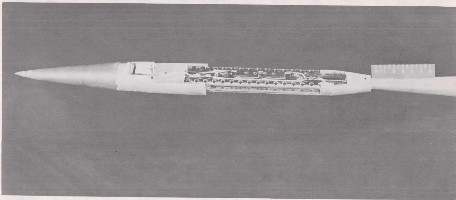
Figure 4.- Strain-gage balance mounted in the body.
