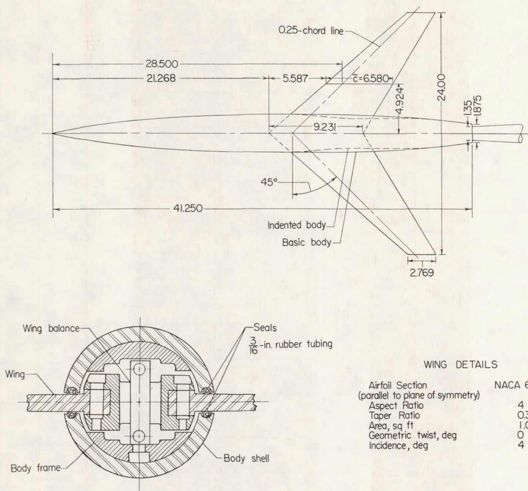
Section showing details of wing balance and seals
