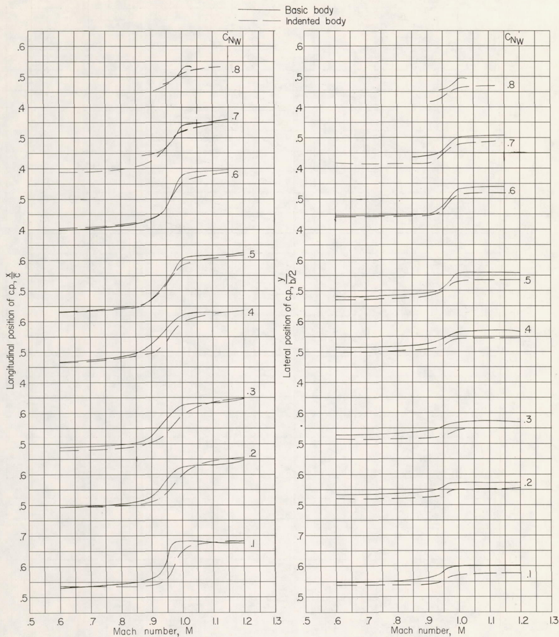
Figure 9.- Effect of body indentation on the variation of the longitudinal and lateral location of the center of pressure with Mach number. Wing incidence 4^\circ .
