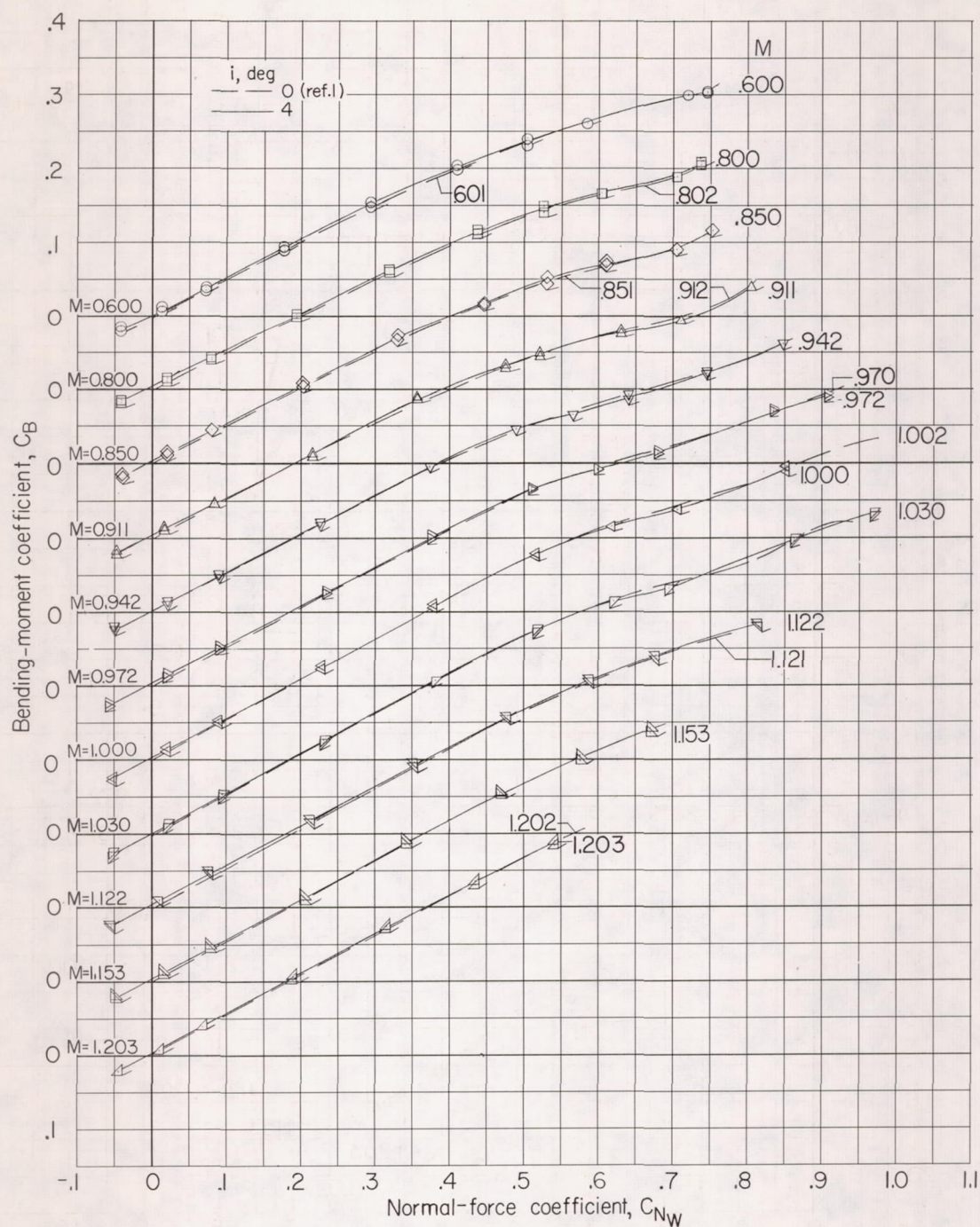
(c) Variation of C_B with C_{N_W} for right- and left-wing panels. Flagged symbols indicate left-wing panel.
