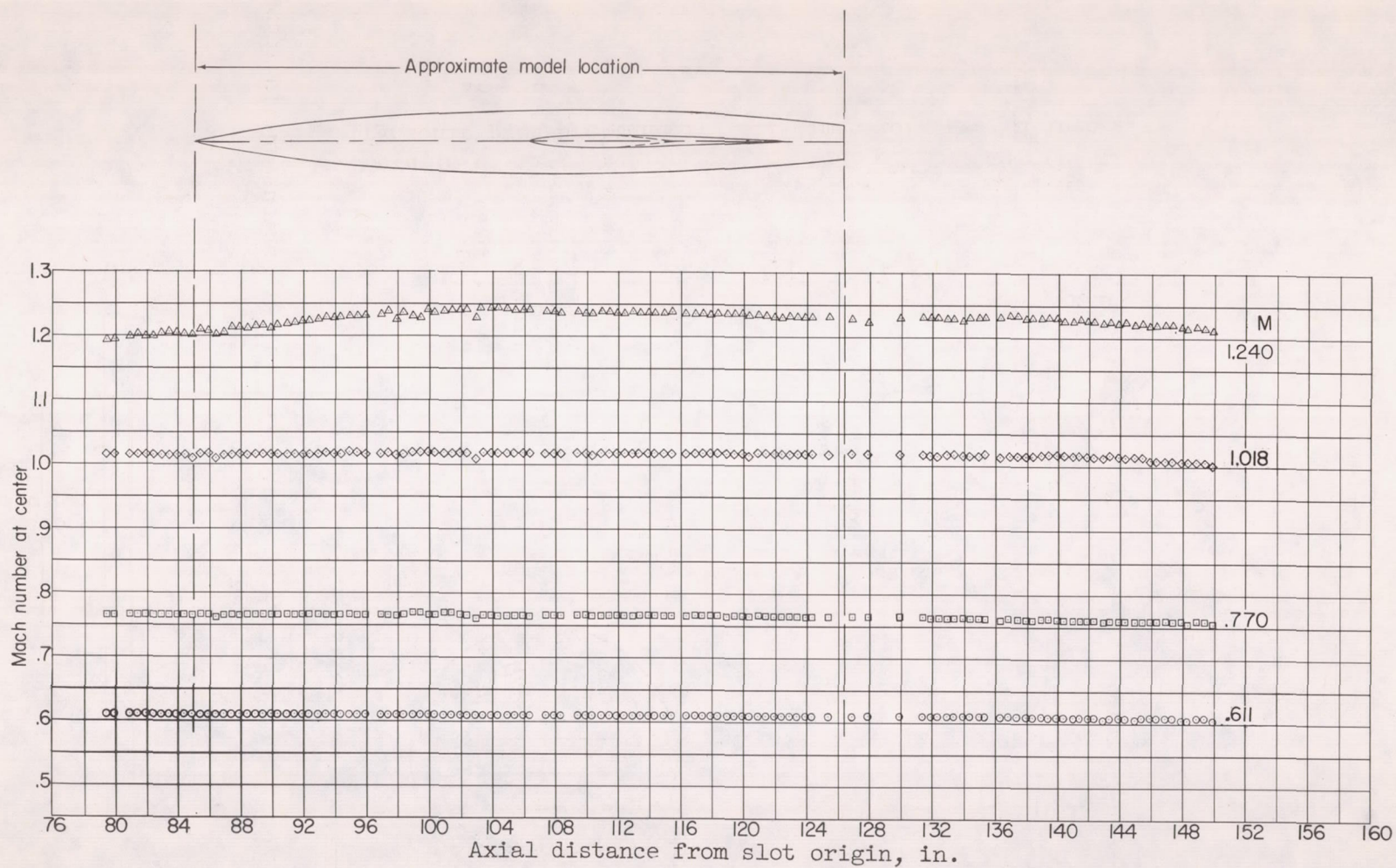
Figure 2.- Typical Mach number distributions in the test section of the Langley 8-foot transonic pressure tunnel during this investigation.
