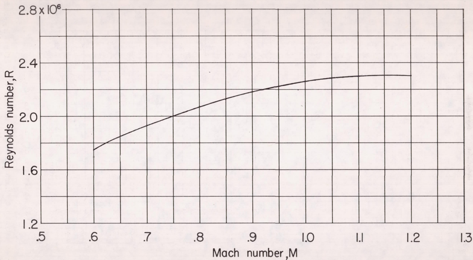
Figure 6.- Variation of Reynolds number with Mach number.
