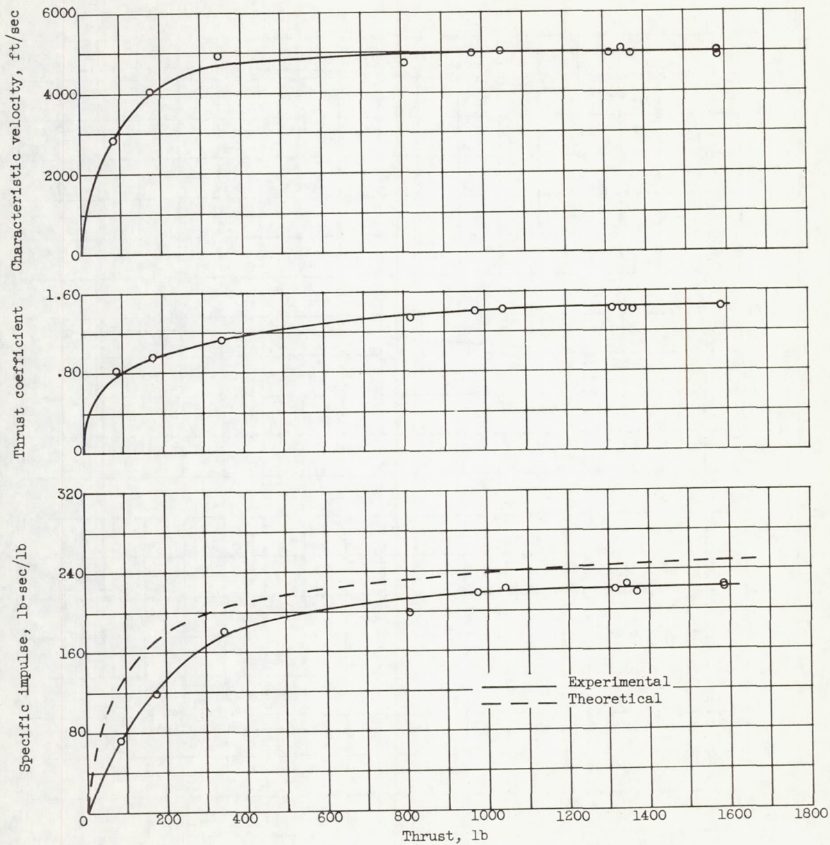
Figure 6. - Performance over wide range of thrust for swirl-cup injector using mixed oxides of nitrogen and ammonia. Nominal full thrust, 1585 pounds.
