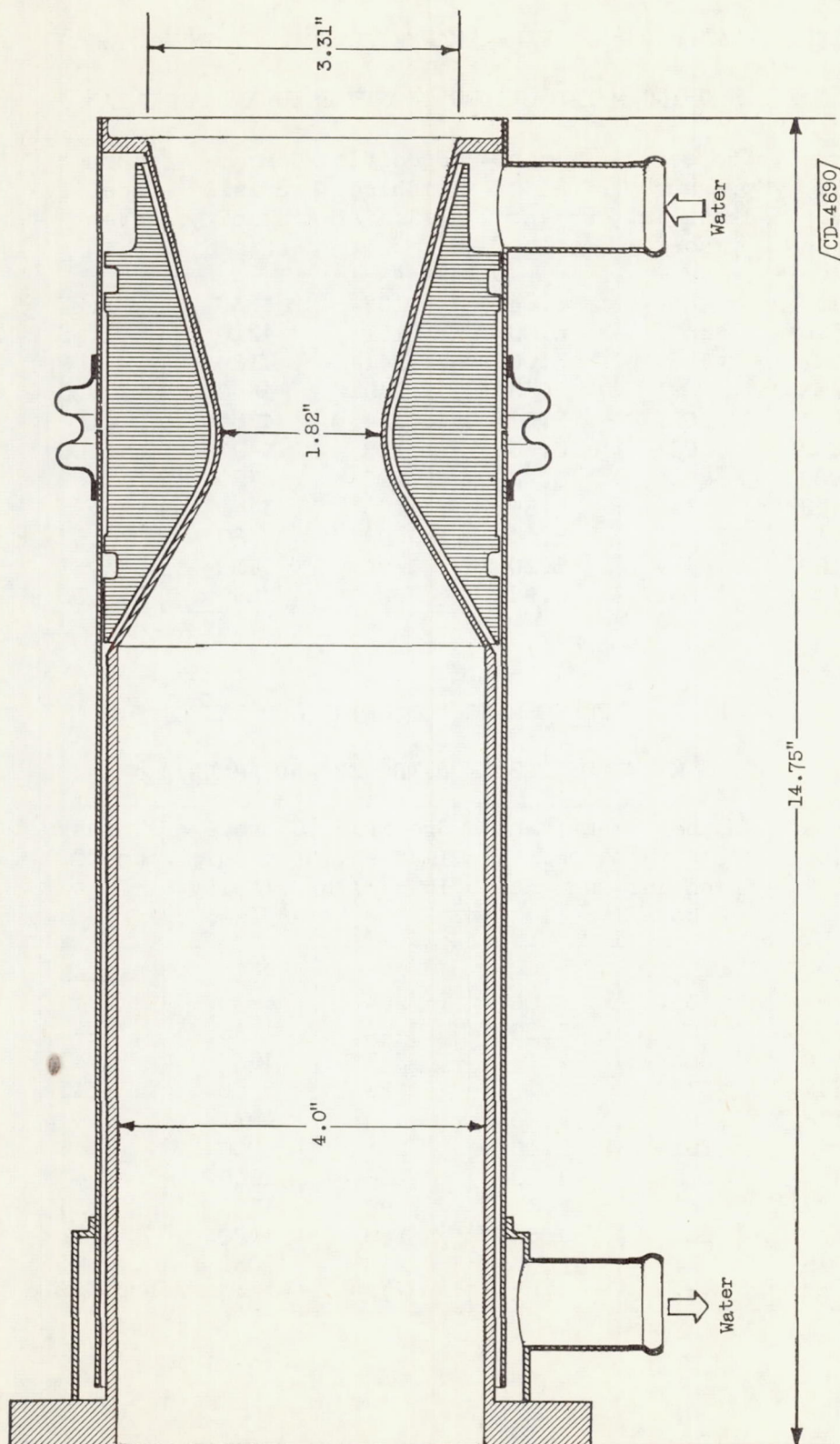
Figure 1. - Water-cooled thrust chamber.
