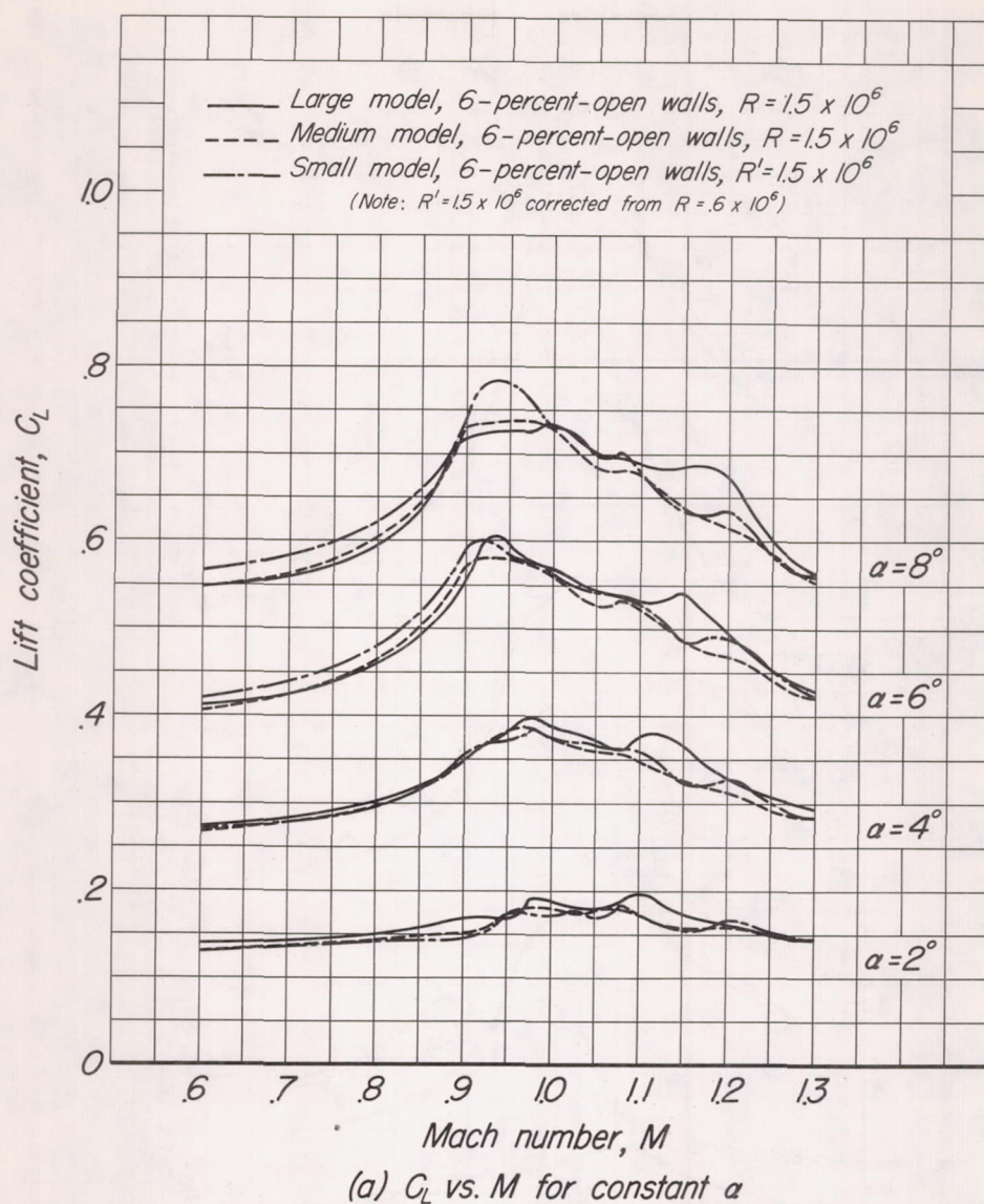
Figure 21.- Variation of aerodynamic characteristics with model size as a function of Mach number.
