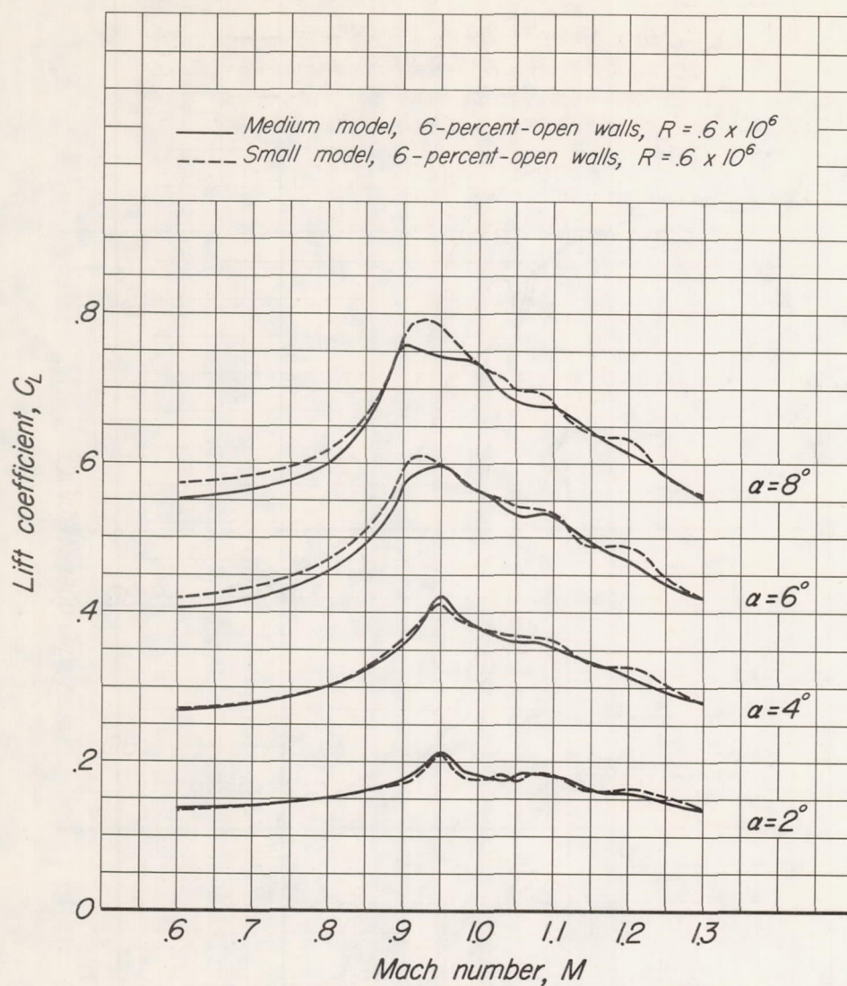
(a) C_L vs. M for constant \alpha
