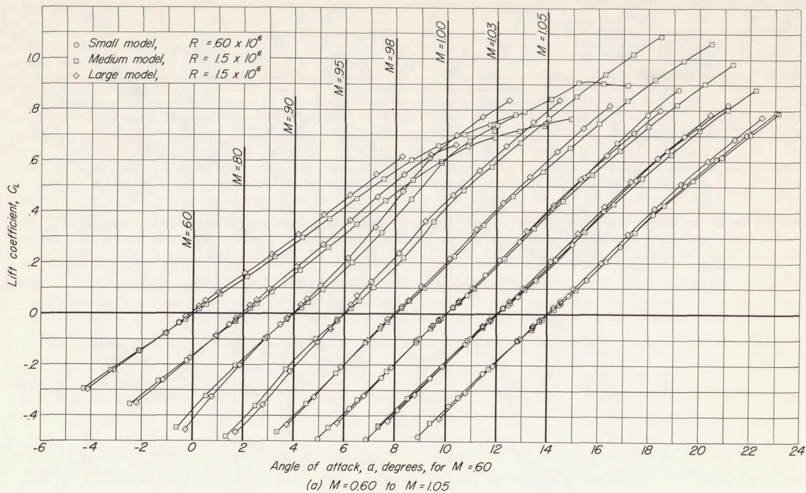
Figure 15.- Variation of lift coefficient with angle of attack at constant Mach numbers; quasi-solid walls.
