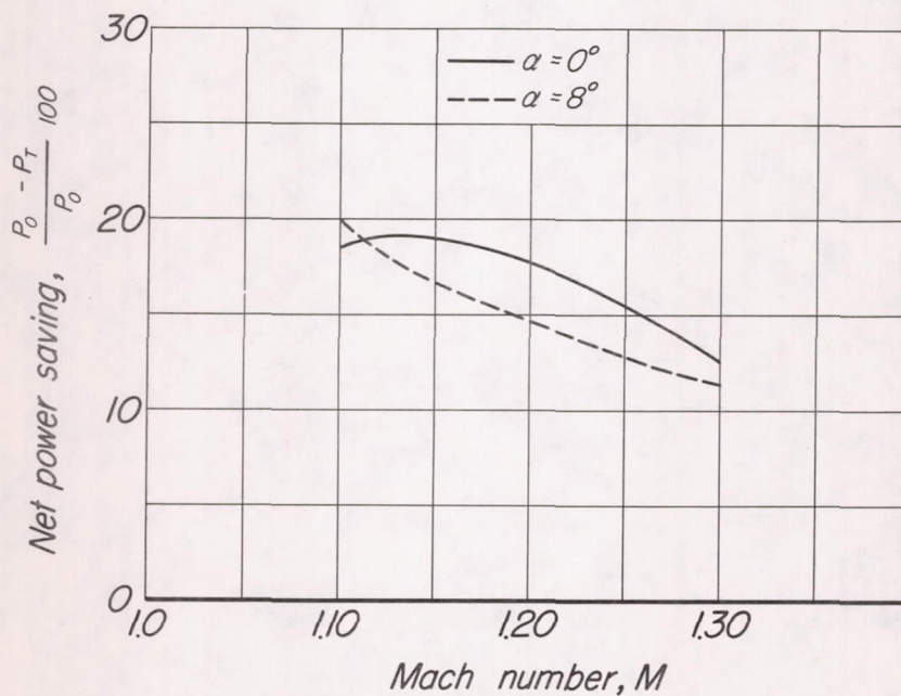
Figure 26.- Net power saving by use of auxiliary suction ( \eta = 100 percent).
