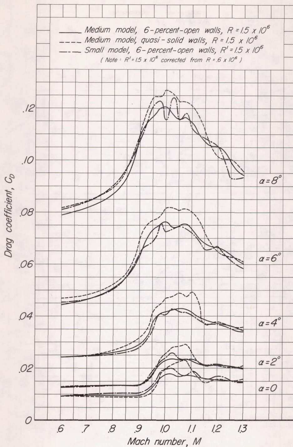
(b) C_D vs. M for constant \alpha
