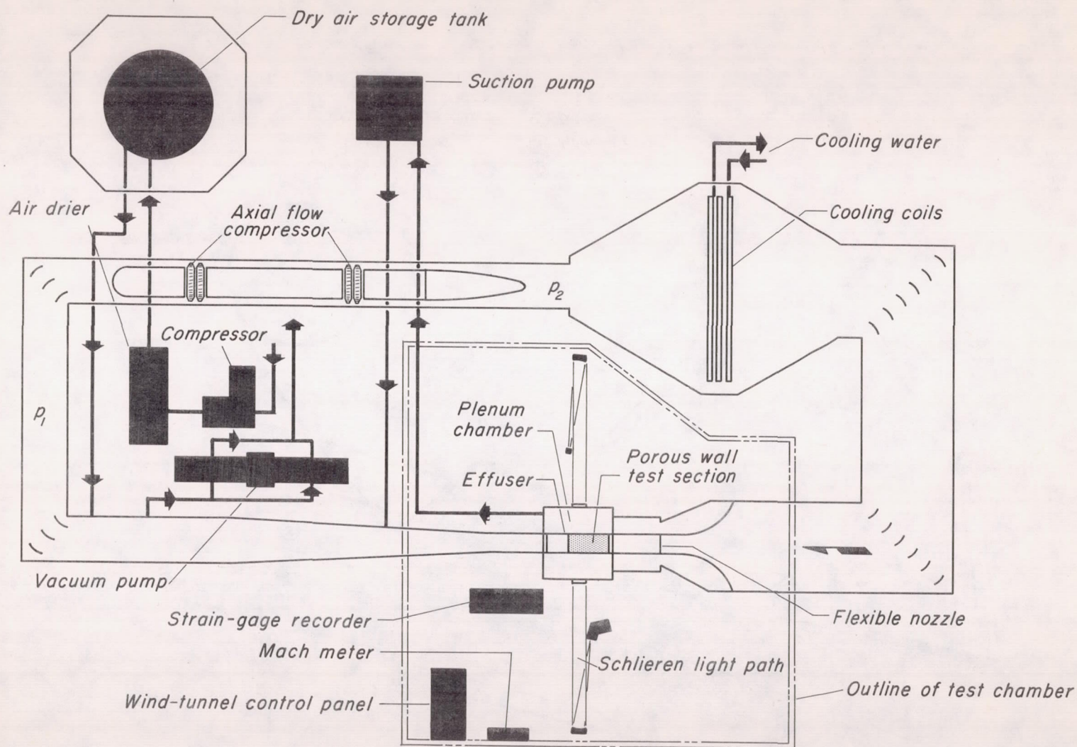
Figure 1.—Schematic drawing of the 2-by 2-foot transonic wind tunnel showing tunnel layout with auxiliary equipment.
