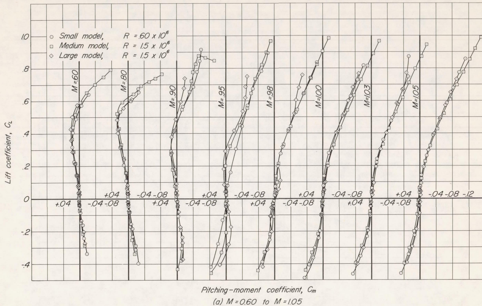
Figure 14.- Variation of lift coefficient with pitching-moment coefficient at constant Mach numbers; 6-percent-open walls.
