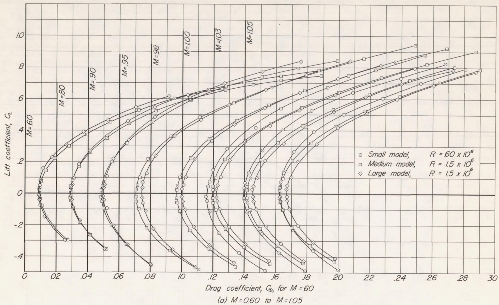
Figure 16.- Variation of lift coefficient with drag coefficient at constant Mach numbers; quasi-solid walls.
