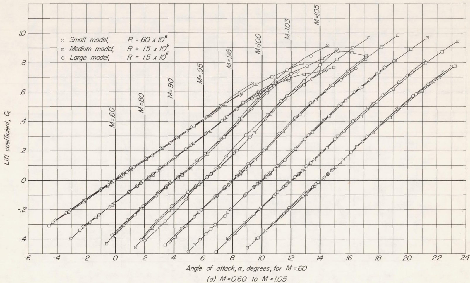
Figure 12.- Variation of lift coefficient with angle of attack at constant Mach numbers; 6-percent-open walls.
