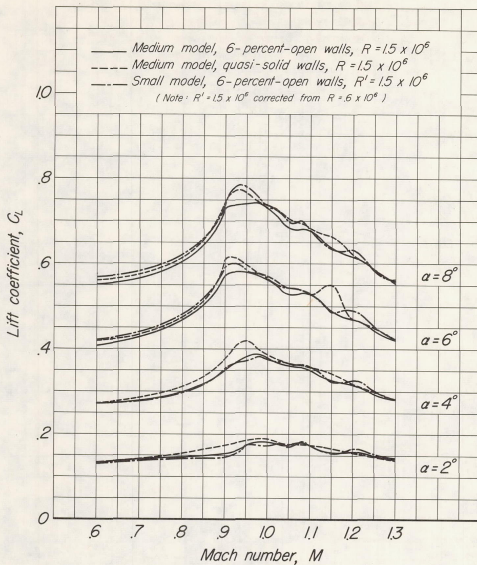
(a) C_L vs. M for constant \alpha
