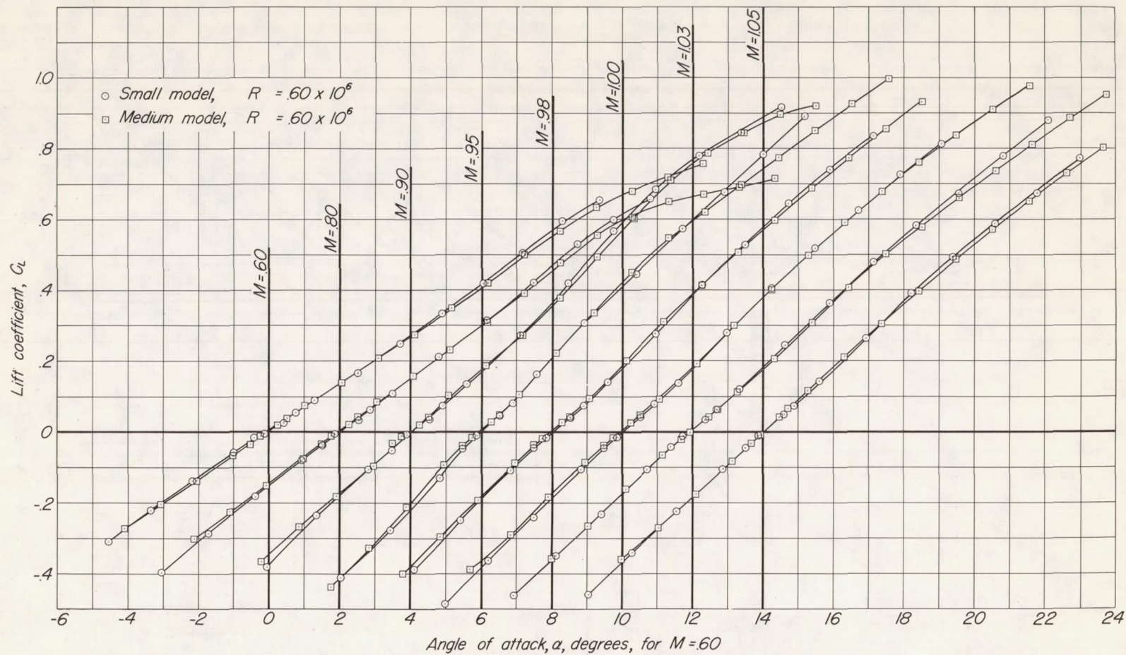
Figure 9.-Variation of lift coefficient with angle of attack at constant Mach numbers for comparison of small model to medium model at R = 0.60 \times 10^6 ; 6-percent-open walls.
