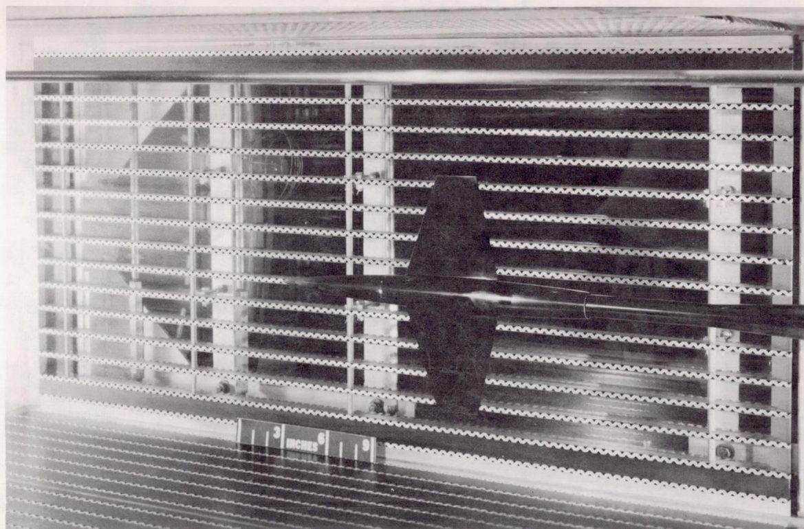
Figure 3.- Typical model installation in perforated test section.
