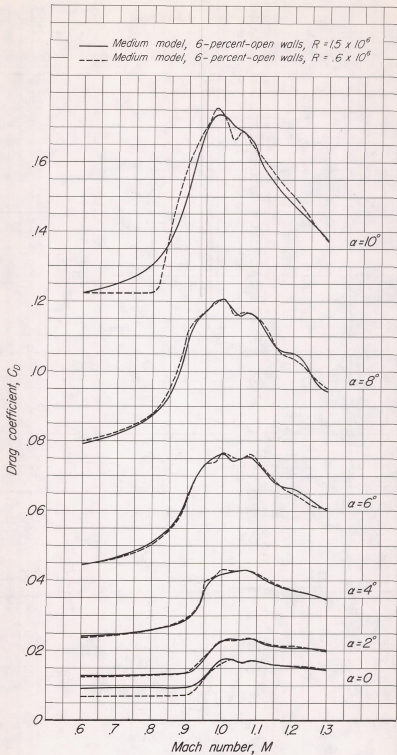
(b) C_D vs. M for constant \alpha
