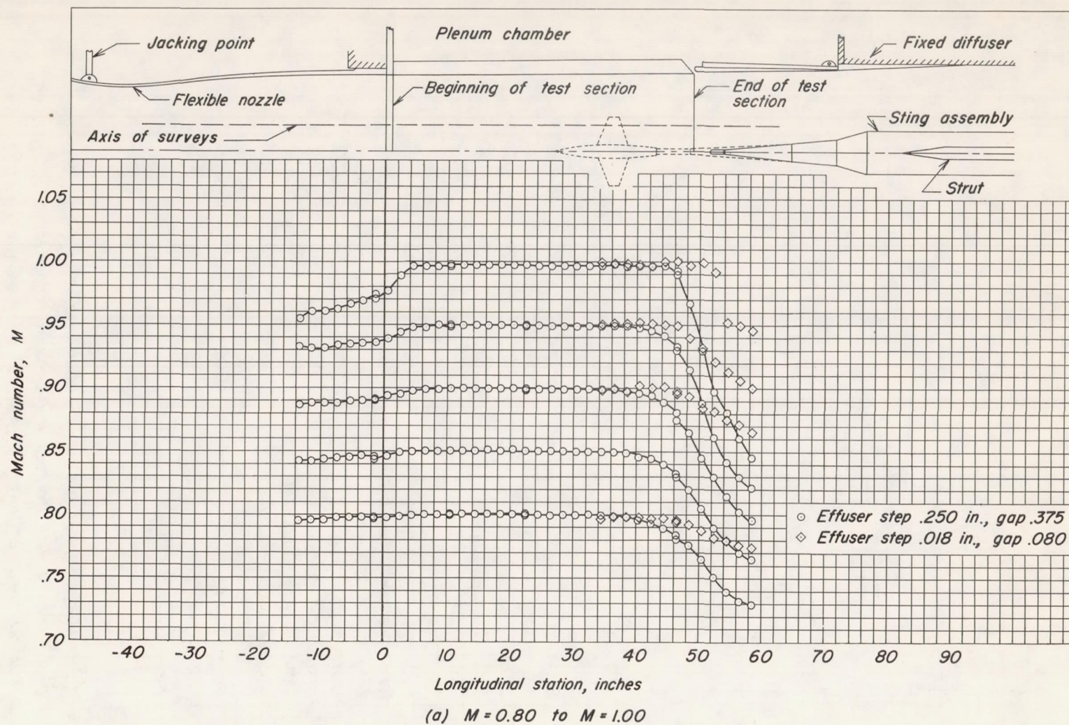
Figure 8.- Mach number distribution as obtained by axial survey on the vertical center line 4 inches above horizontal center line. (Tunnel empty)
