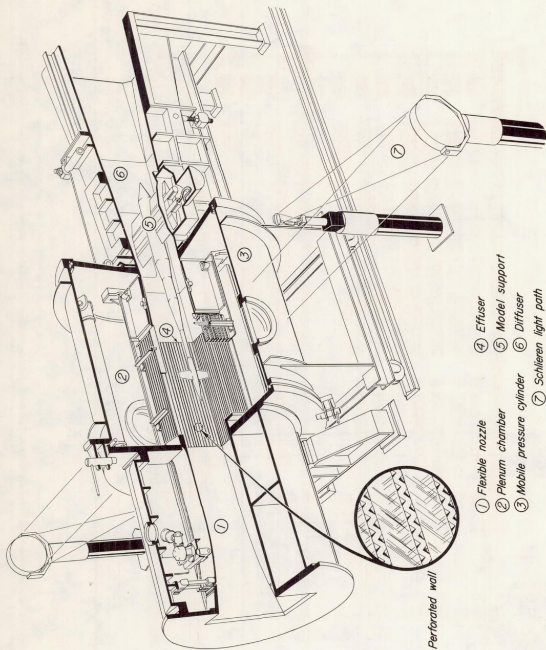
Figure 2.- Sectional view of the high-speed region of the 2-by 2-foot transonic wind tunnel.
