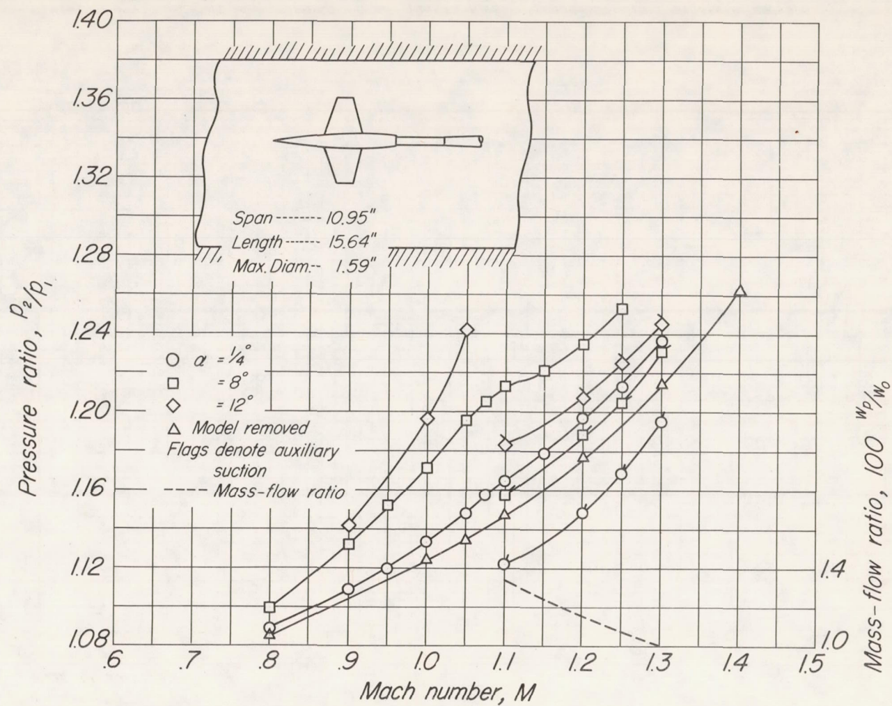
Figure 24.- Pressure-ratio requirements across main-drive compressor ( P_2/P_1 , fig. 1.)
