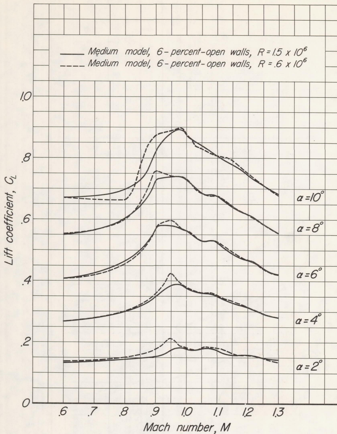
(a) C_L vs. M for constant \alpha
