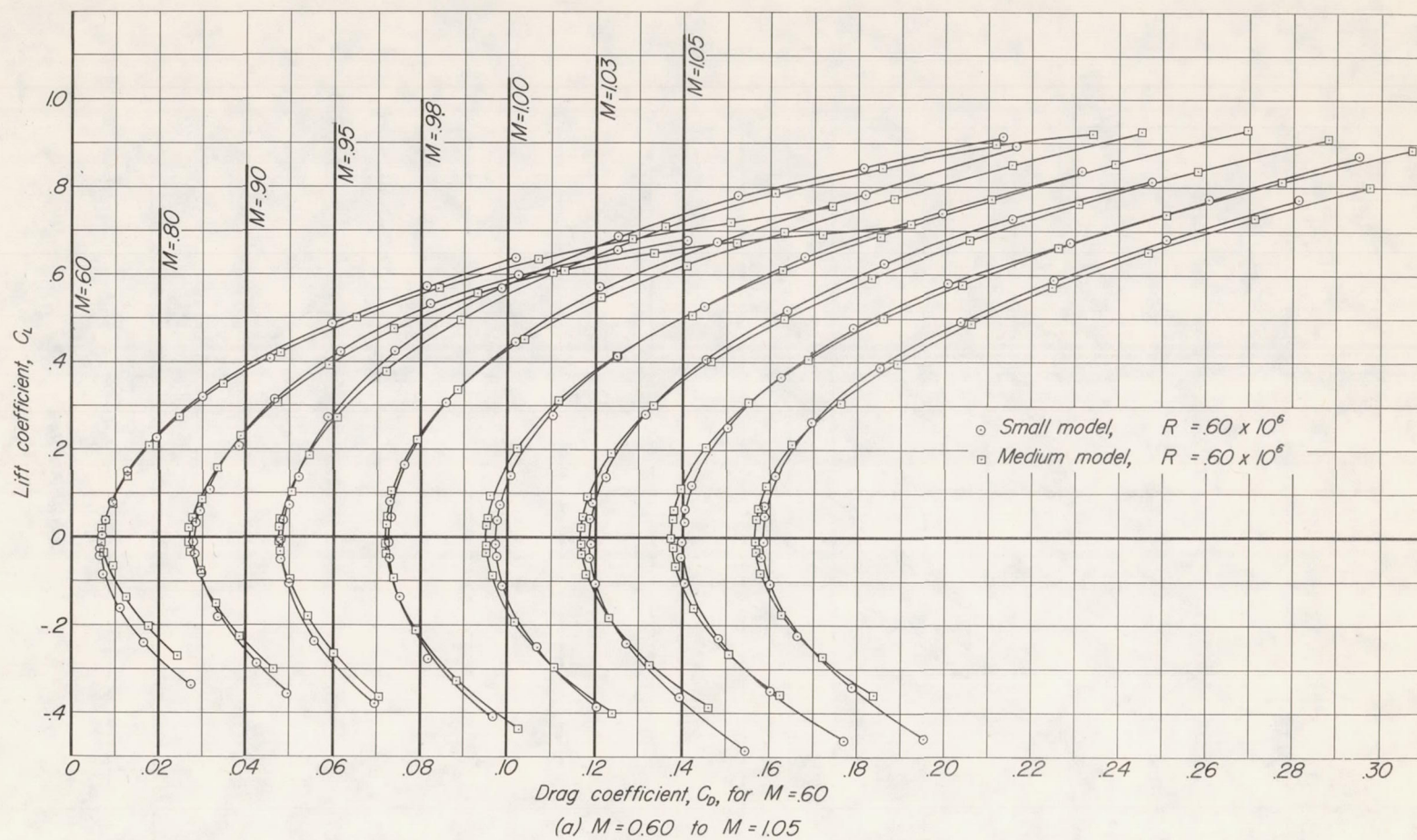
Figure 10.-Variation of lift coefficient with drag coefficient at constant Mach numbers for comparison of small model to medium model at R = 0.60 \times 10^6 ; 6-percent-open walls.
