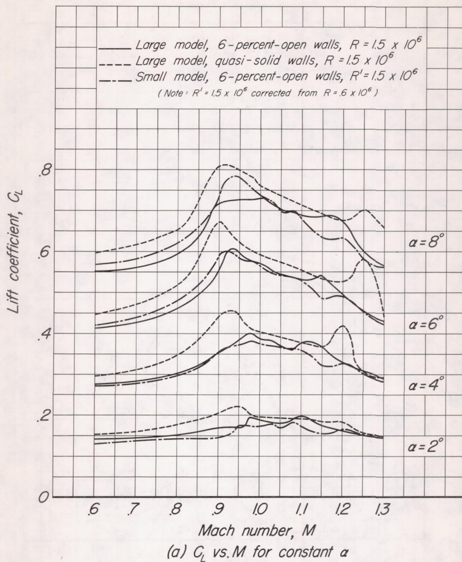
Figure 19.- Effect of test-section-wall solidity on aerodynamic characteristics as a function of Mach number; large model.
