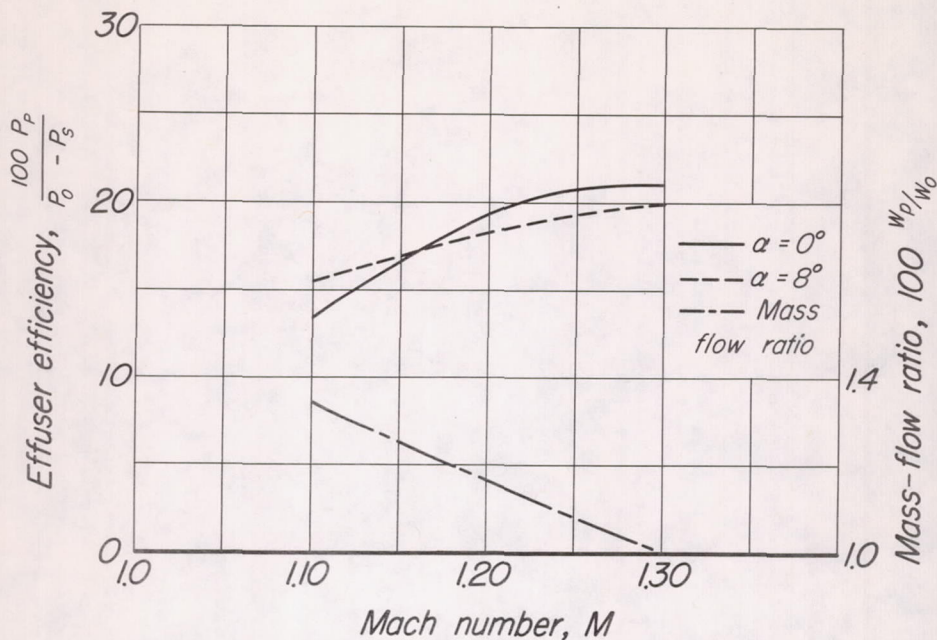
Figure 25.-Effuser efficiency based on auxiliary suction power ( \eta = 100 percent).
