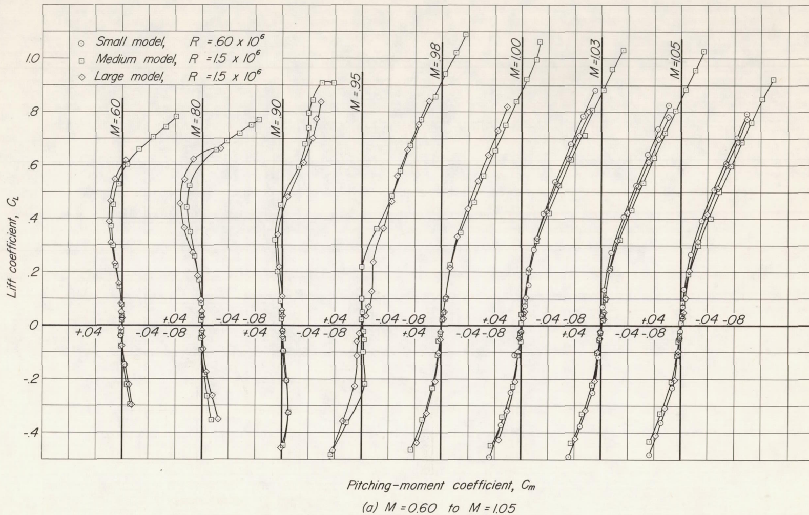
Figure 17.-Variation of lift coefficient with pitching-moment coefficient at constant Mach numbers; quasi-solid walls.
