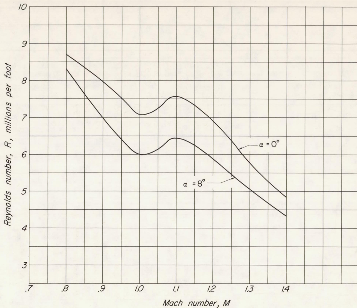
Figure 6.- Variation of the maximum Reynolds number with Mach number for the 2-by-2-foot transonic wind tunnel.
