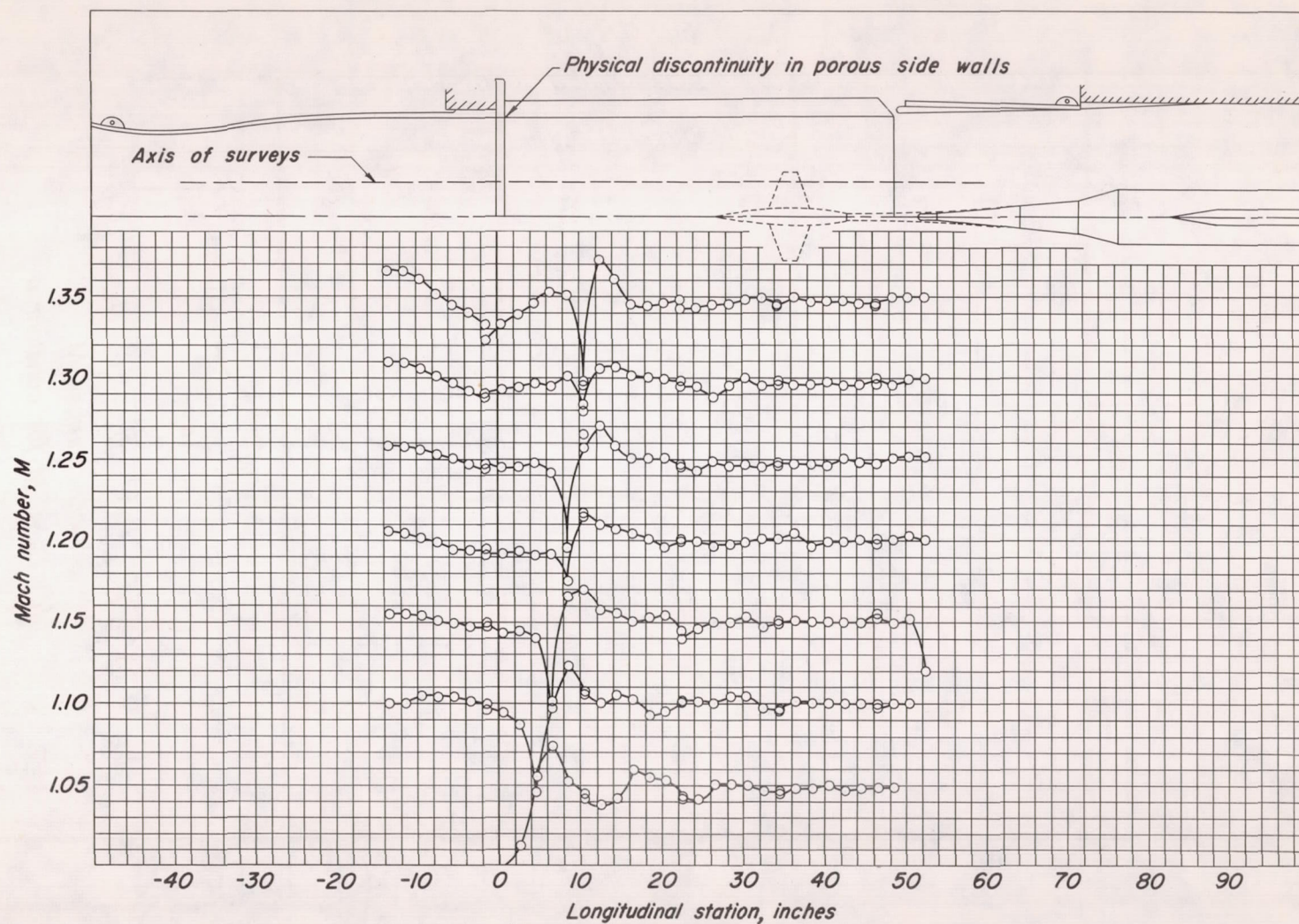
Figure 23.- Indication of shock-wave attenuation from pressure surveys.
