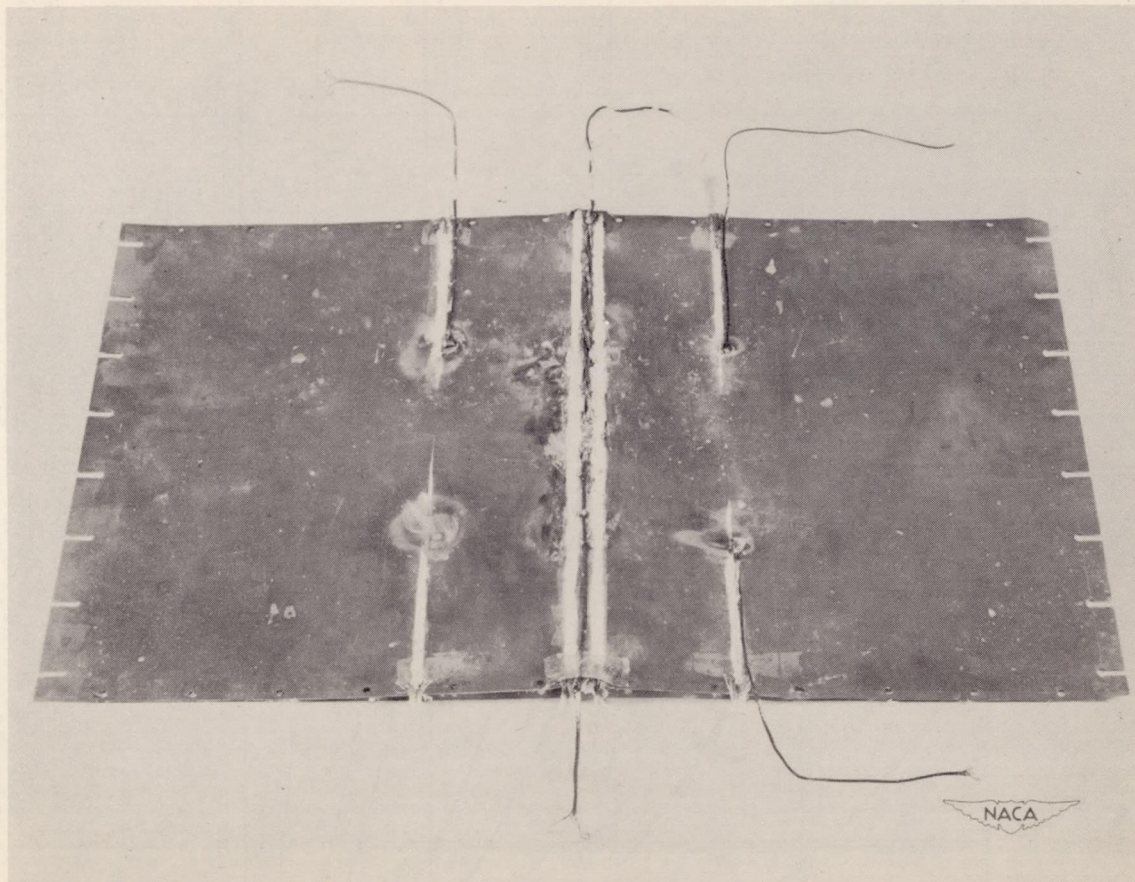
Figure 2.- Insulated iron-constantan and Chromel-Alumel thermocouples mounted in "laid-on-plate" position. Leads were tied down to plate at 1-inch intervals. White streaks indicate position of embedded thermocouples.
