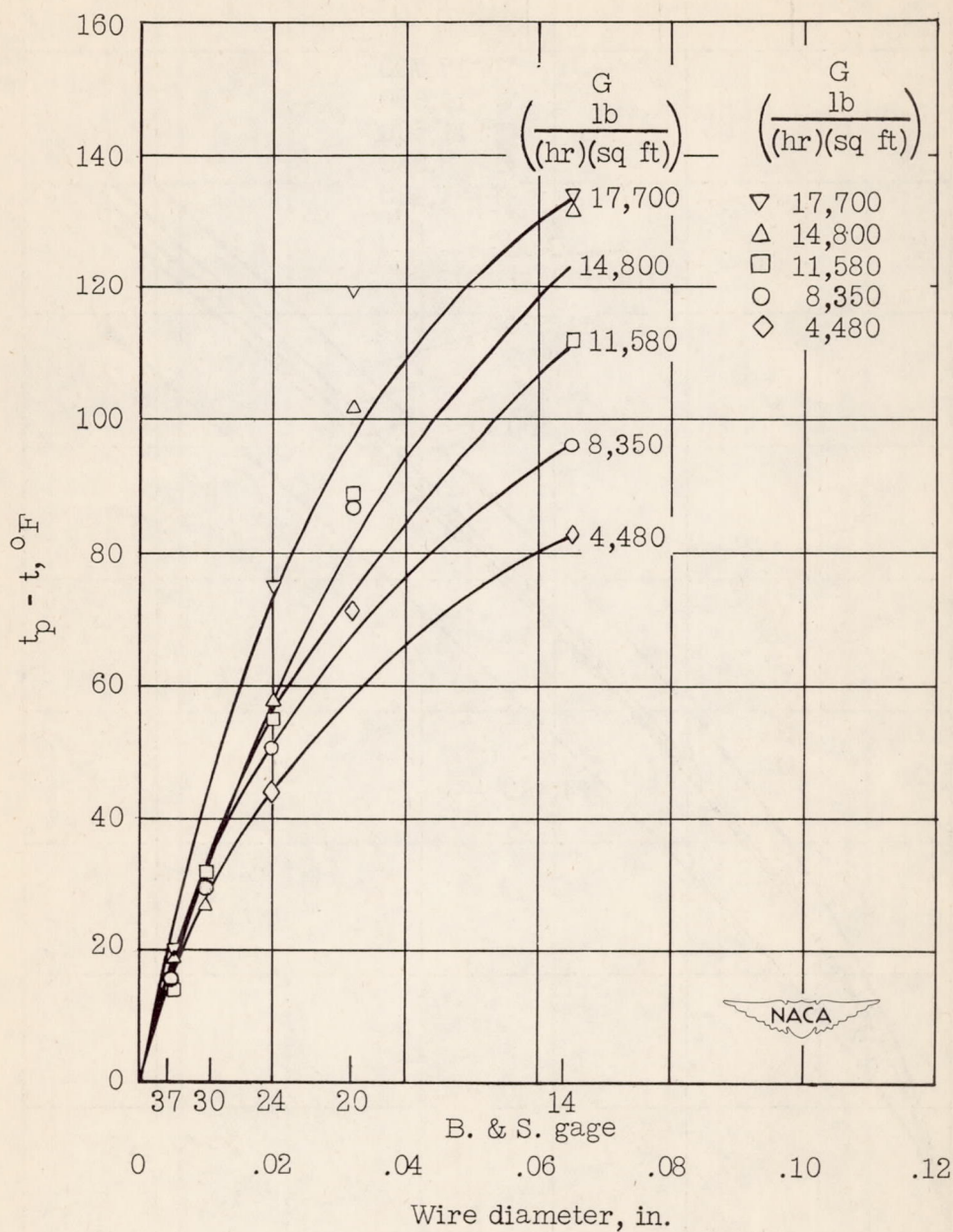
Figure 6.- Thermocouple-error curves for bare iron-constantan thermocouple wire mounted in vertical position. Temperature of test plate t_p , 475^{\circ}\text{F} .
