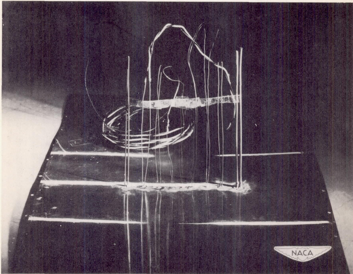
Figure 1.- Bare iron-constantan and Chromel-Alumel thermocouples mounted in vertical position. (Note how the weld beads were cut to test plate wherever possible.) White streaks indicate position of embedded thermocouples. (Three more were added before data were recorded.)
