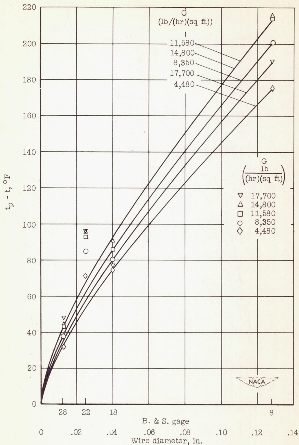
Figure 9.- Thermocouple-error curves for bare Chromel-Alumel thermocouple wire mounted in vertical position. Temperature of test plate t_p , 600^\circ\text{F} .
