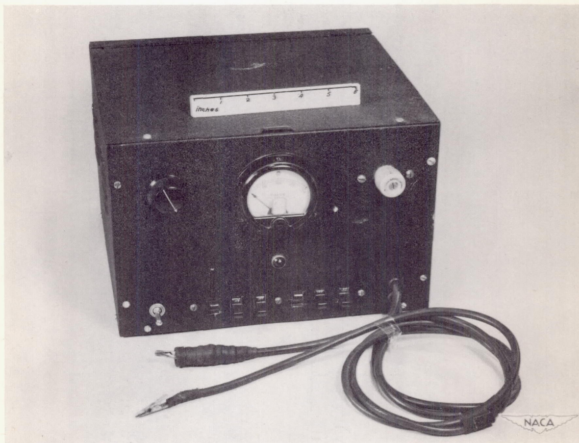
Figure 15.- Condenser-discharge spot welder.
