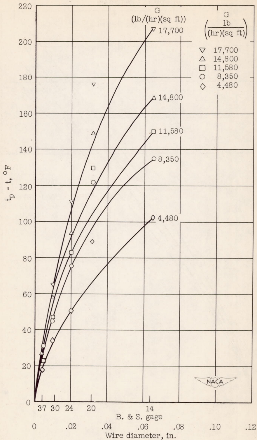
Figure 8.- Thermocouple-error curves for bare iron-constantan thermocouple wire mounted in vertical position. Temperature of test plate t_p , 600^\circ\text{F} .
