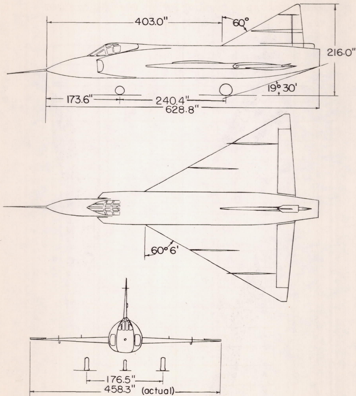
Figure 1.- Three-view drawing of the airplane.
