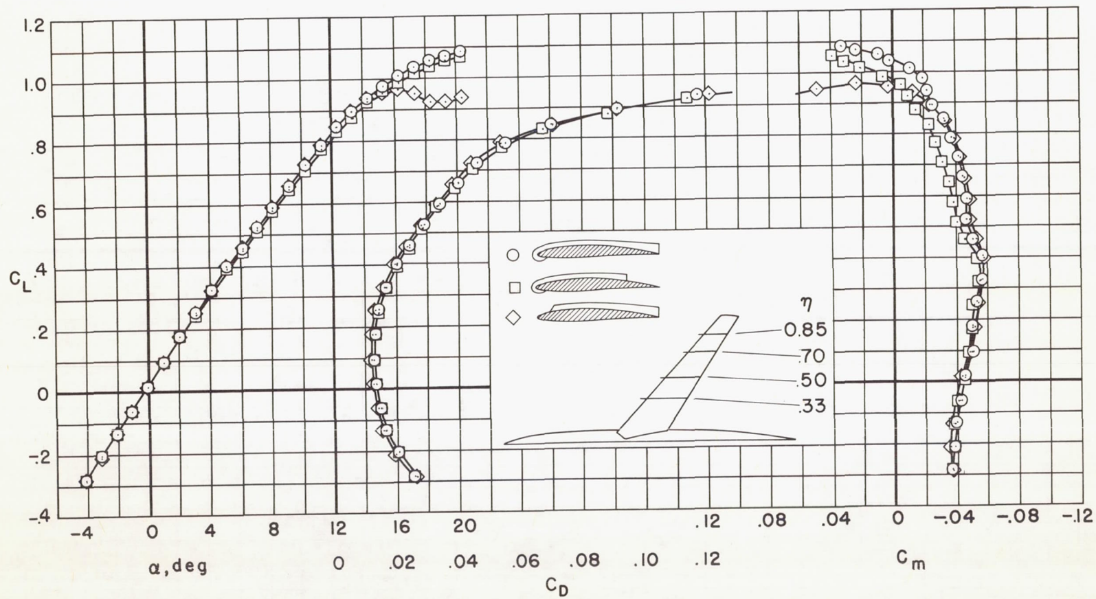
Figure 7.- The effect of complete- and partial-chord fences on the longitudinal characteristics of the wing-fuselage combination; M = 0.417 , R = 3,600,000 .
