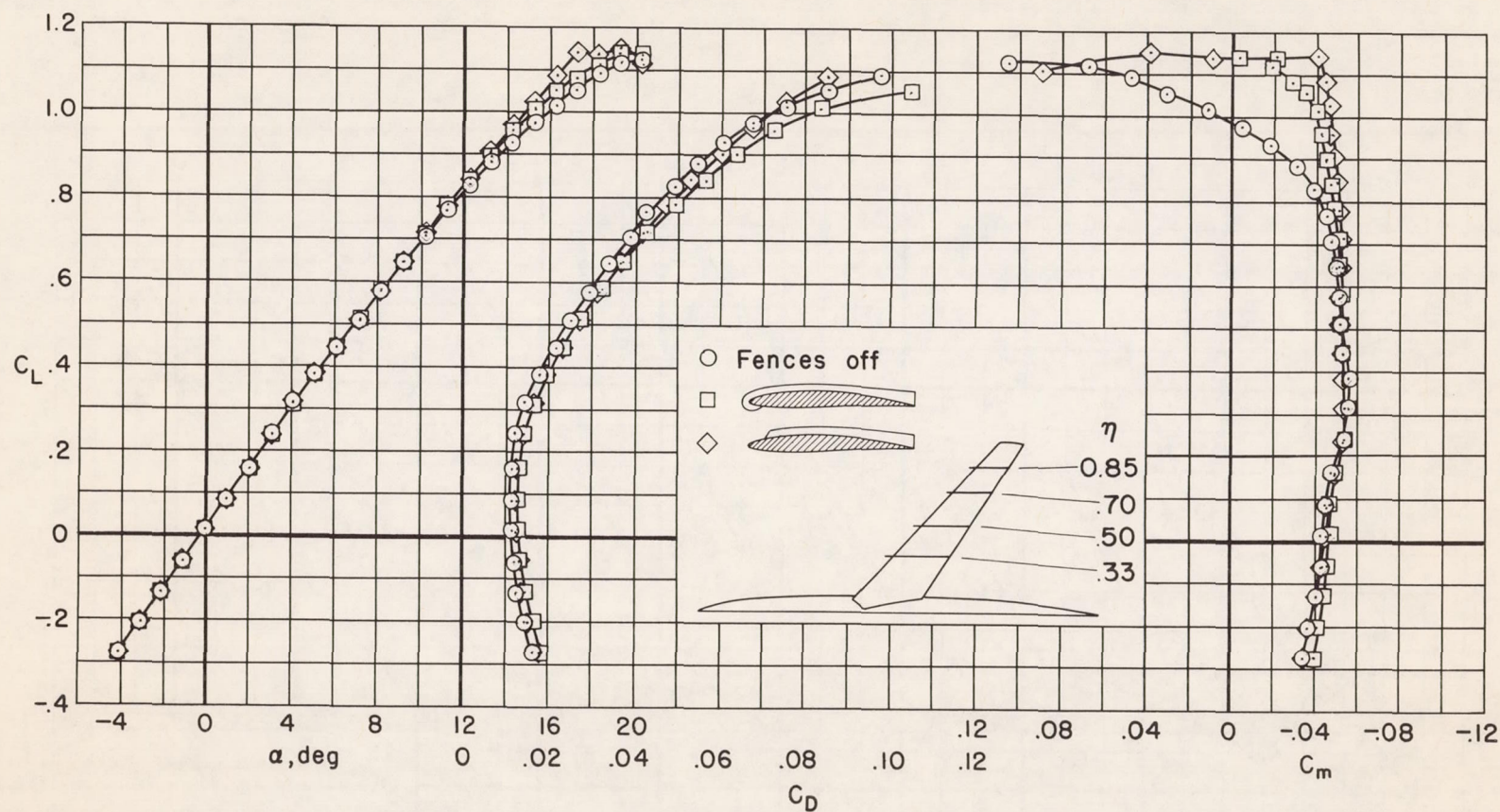
Figure 8.- The effect of complete- and partial-chord fences on the longitudinal characteristics of the wing-fuselage combination; M = 0.25 , R = 8 \times 10^6 .
