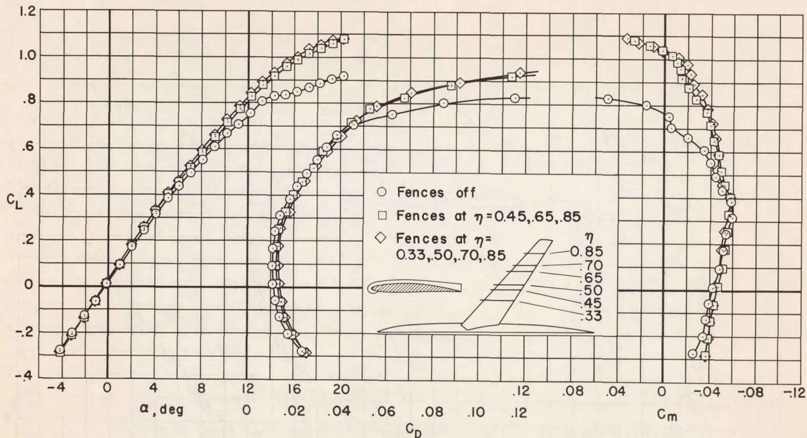
Figure 6.- The effect of three and four fences on the longitudinal characteristics of the wing-fuselage combination; M = 0.417 , R = 3,600,000 .
