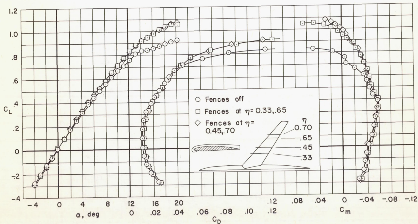
Figure 5.- The effect of two fences at various spanwise locations on the longitudinal characteristics of the wing-fuselage combination; M = 0.417 , R = 3,600,000 .
