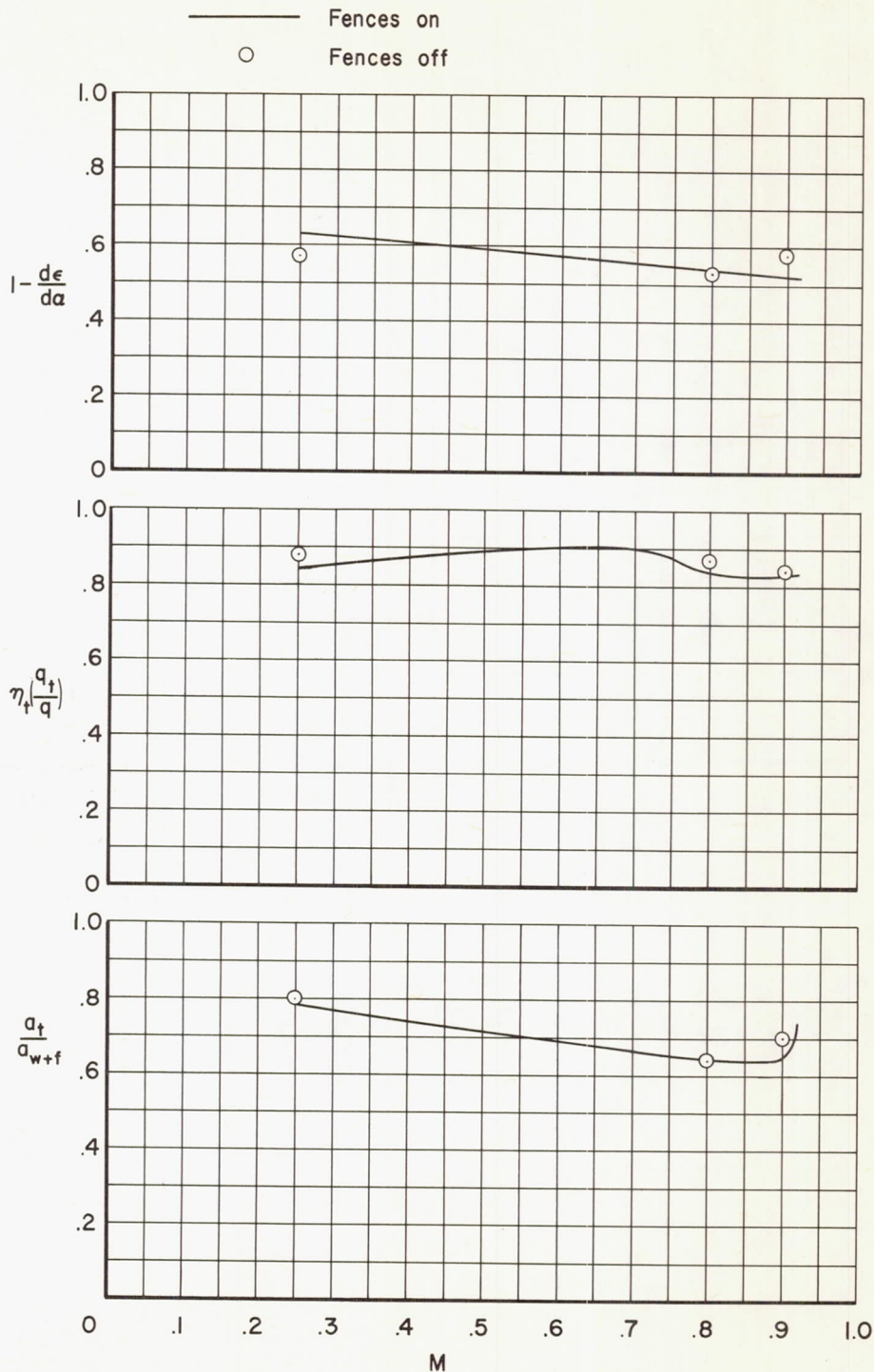
Figure 24.- The variation with Mach number of the factors affecting the stability contribution of the horizontal tail; \alpha = 4^\circ , R = 2,000,000 .
