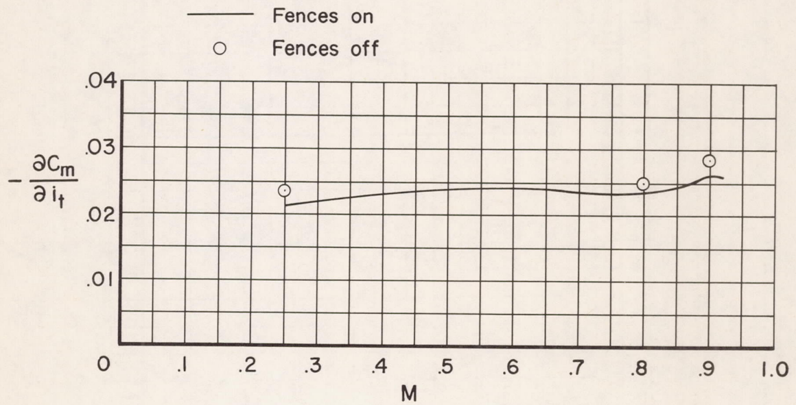
Figure 23.- The variation with Mach number of the control-effectiveness of the horizontal tail; \alpha = 4^\circ , R = 2,000,000 .
