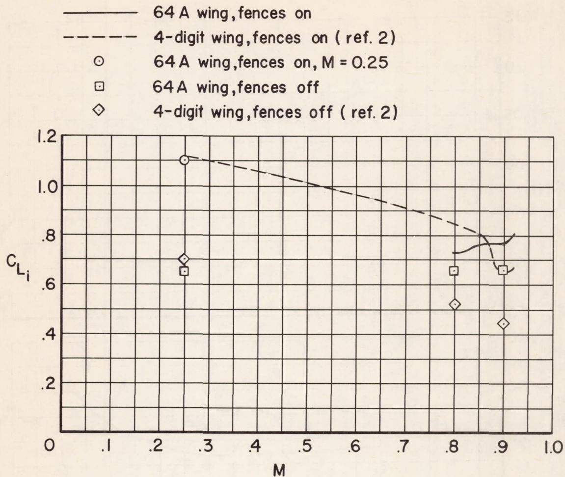
Figure 19.- The variations with Mach number of the inflection lift coefficients of the 64A and four-digit wing-fuselage-tail combinations with and without wing fences; i_t = -8^\circ , R = 2,000,000 .
