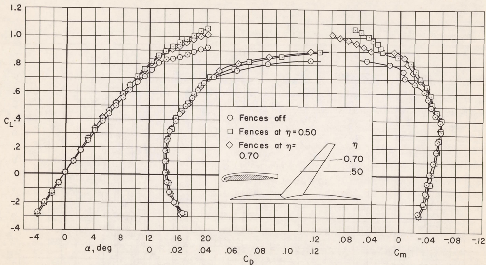
Figure 4.- The effect of a single wing fence at various spanwise locations on the longitudinal characteristics of the wing-fuselage combination; M = 0.417 , R = 3,600,000 .
