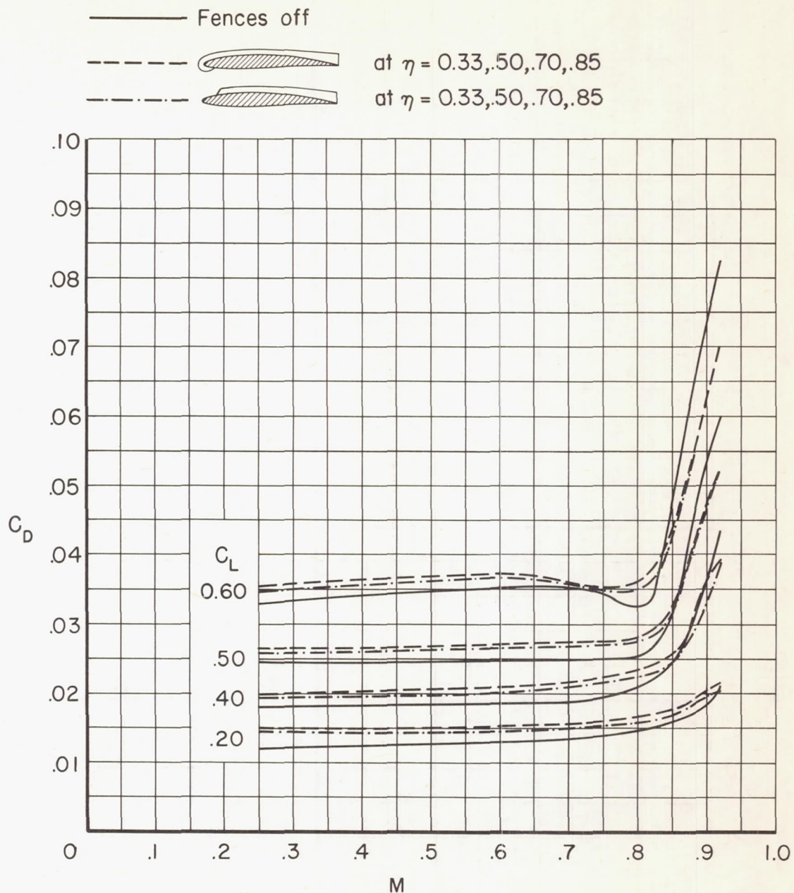
Figure 14.- The variation with Mach number of the drag coefficients of the wing-fuselage combination with and without wing fences at several constant lift coefficients; R = 2,000,000 .
