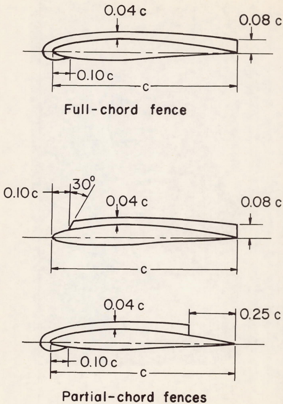
Figure 2.- Fence details.
