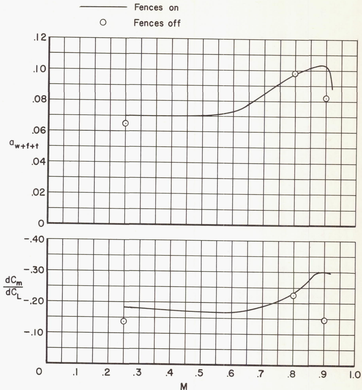
Figure 20.- The variations with Mach number of the slopes of the lift and pitching-moment curves of the wing-fuselage-tail combination with and without wing fences; i_t = -8^\circ , C_L = 0.40 , R = 2,000,000 .
