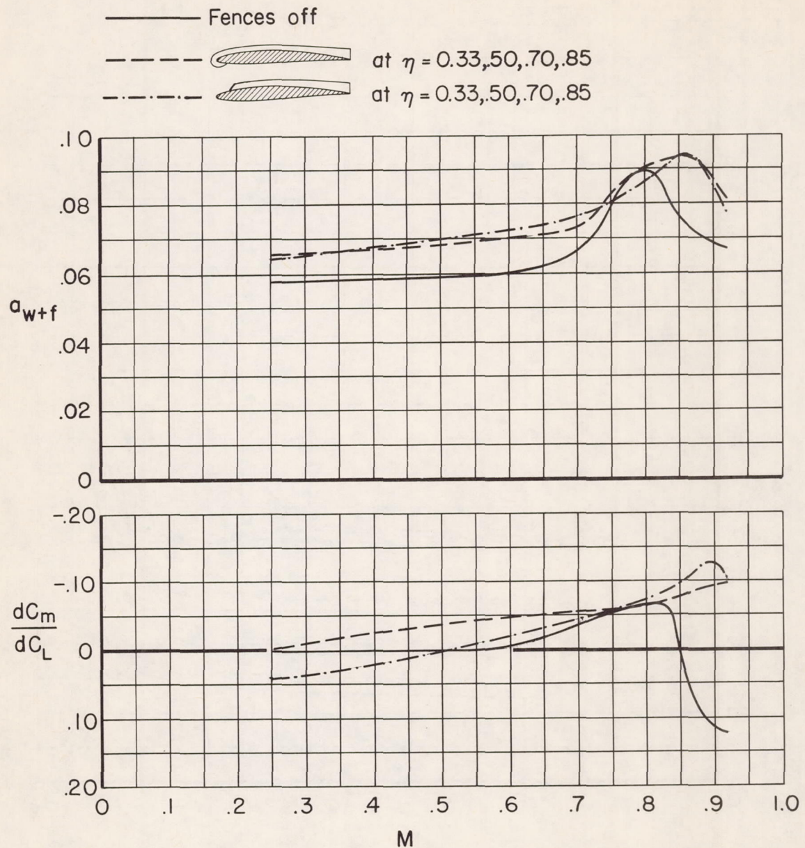
Figure 13.- The variation with Mach number of the slopes of the lift and pitching-moment curves of the wing-fuselage combination with and without wing fences; C_L = 0.40 , R = 2,000,000 .
