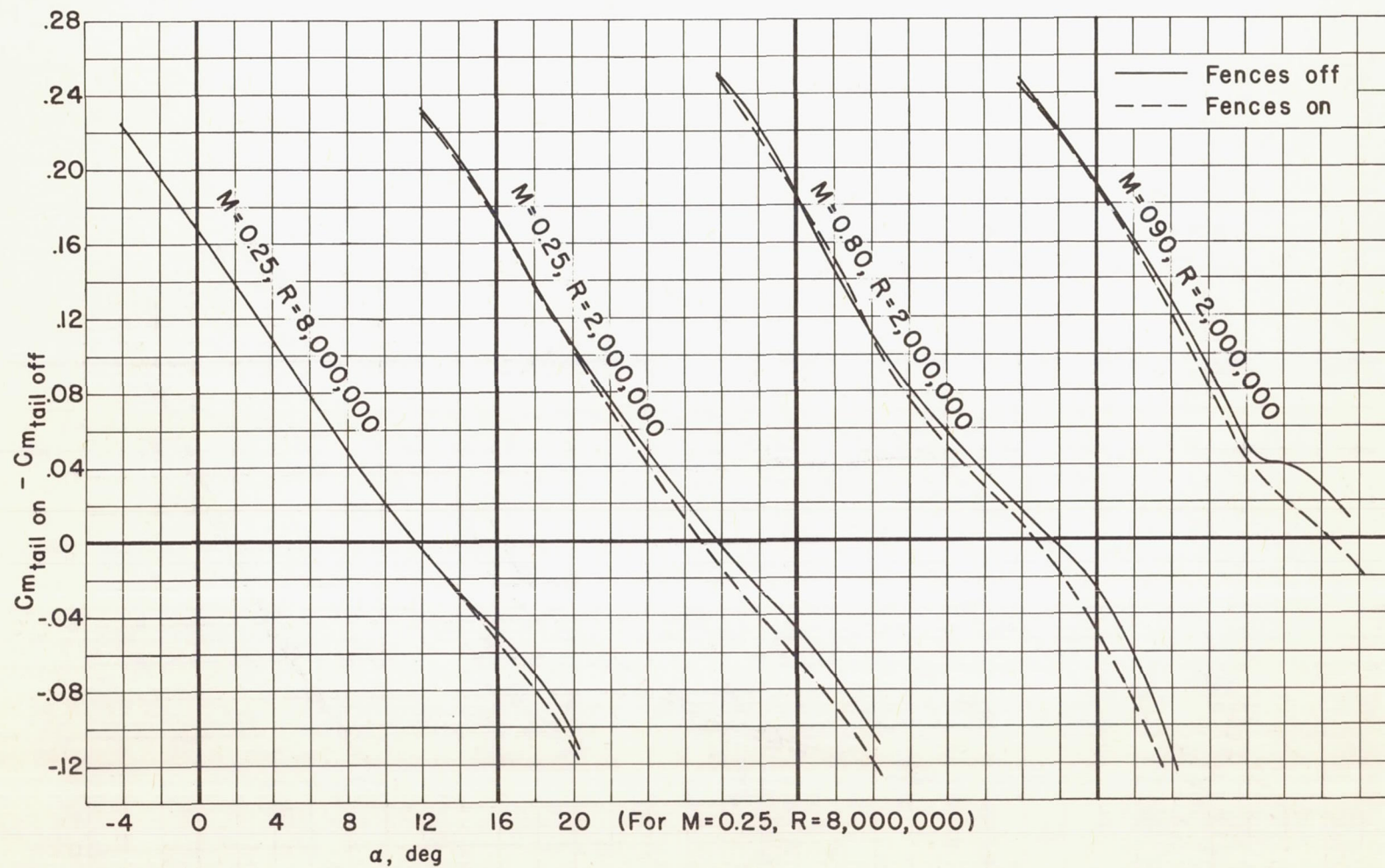
Figure 18.- Pitching-moment coefficient due to the horizontal tail; i_t = -8^\circ .
