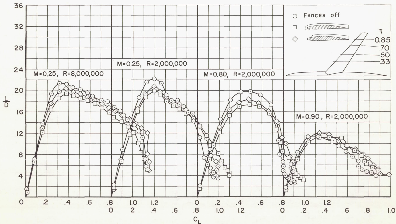
Figure 12.- The effect of complete- and partial-chord fences on the lift-drag ratios of the wing-fuselage combination.
