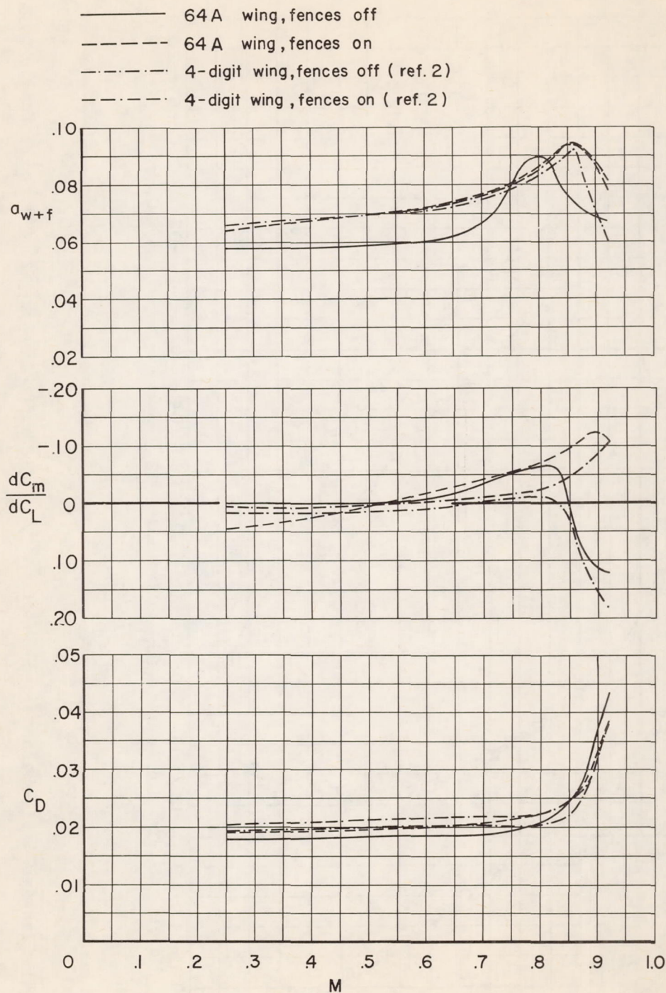
Figure 15.- Comparison of the longitudinal characteristics of the 64A and four-digit wing-fuselage combinations with and without partial-chord fences; C_L = 0.40 , R = 2,000,000 .
