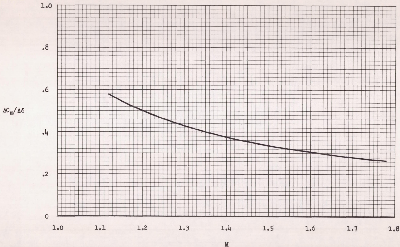
Figure 13.- Variation of control-surface pitching effectiveness with Mach number.
