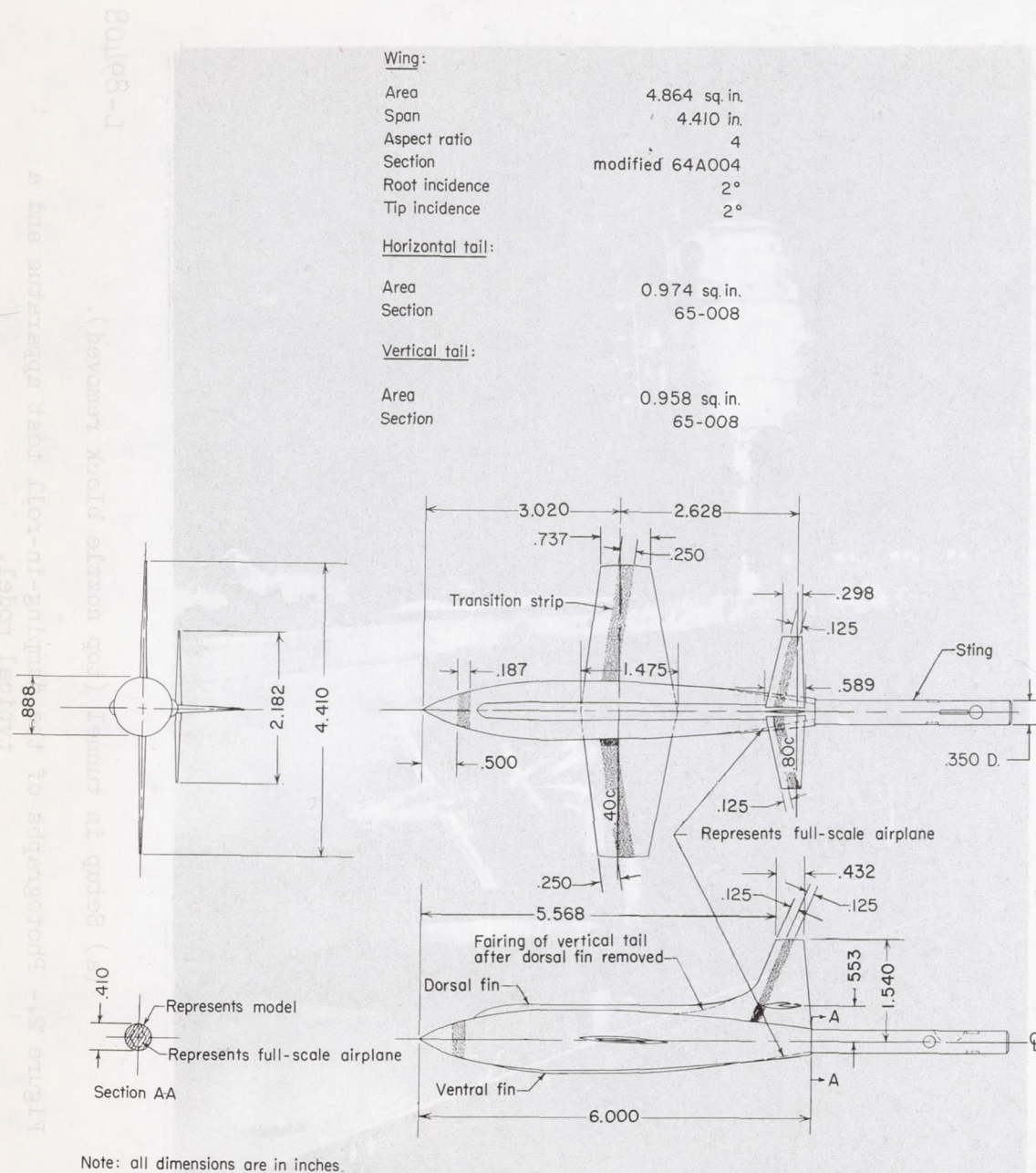
Figure 1.- Drawing of the complete model.
