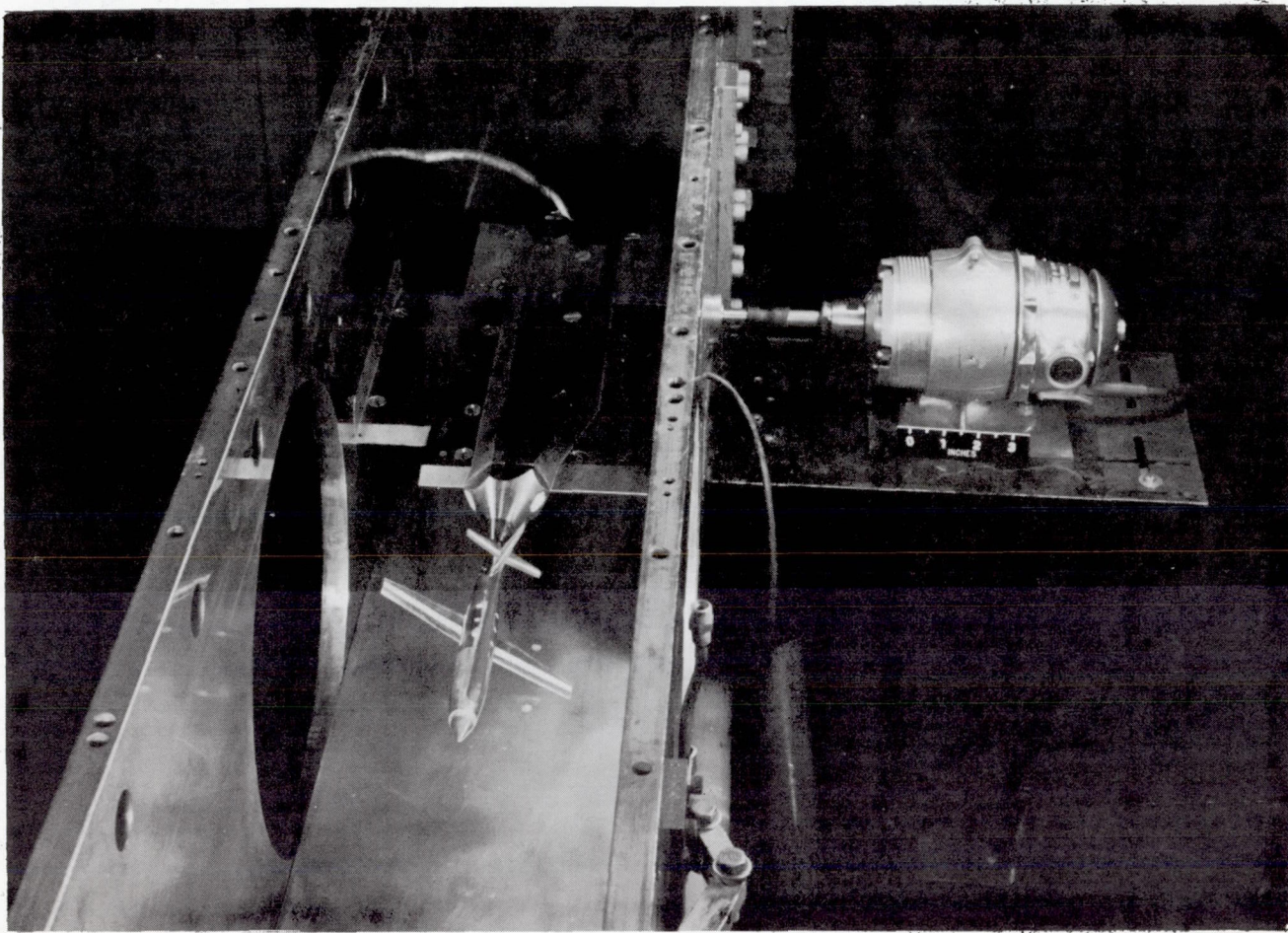
(a) Setup in tunnel (top nozzle block removed).
