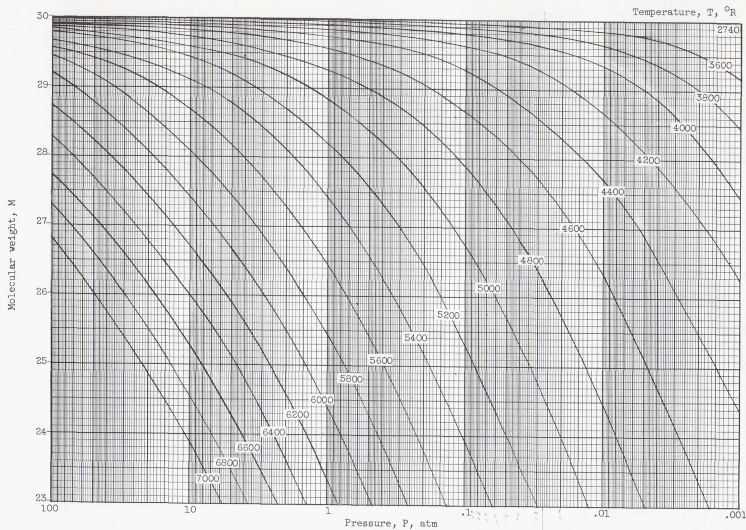
Figure 3. - Concluded. Thermodynamic data for pentaborane \text{B}_5\text{H}_9 , including effects of dissociation. Fuel-air ratio (stoichiometric), 0.07645.
