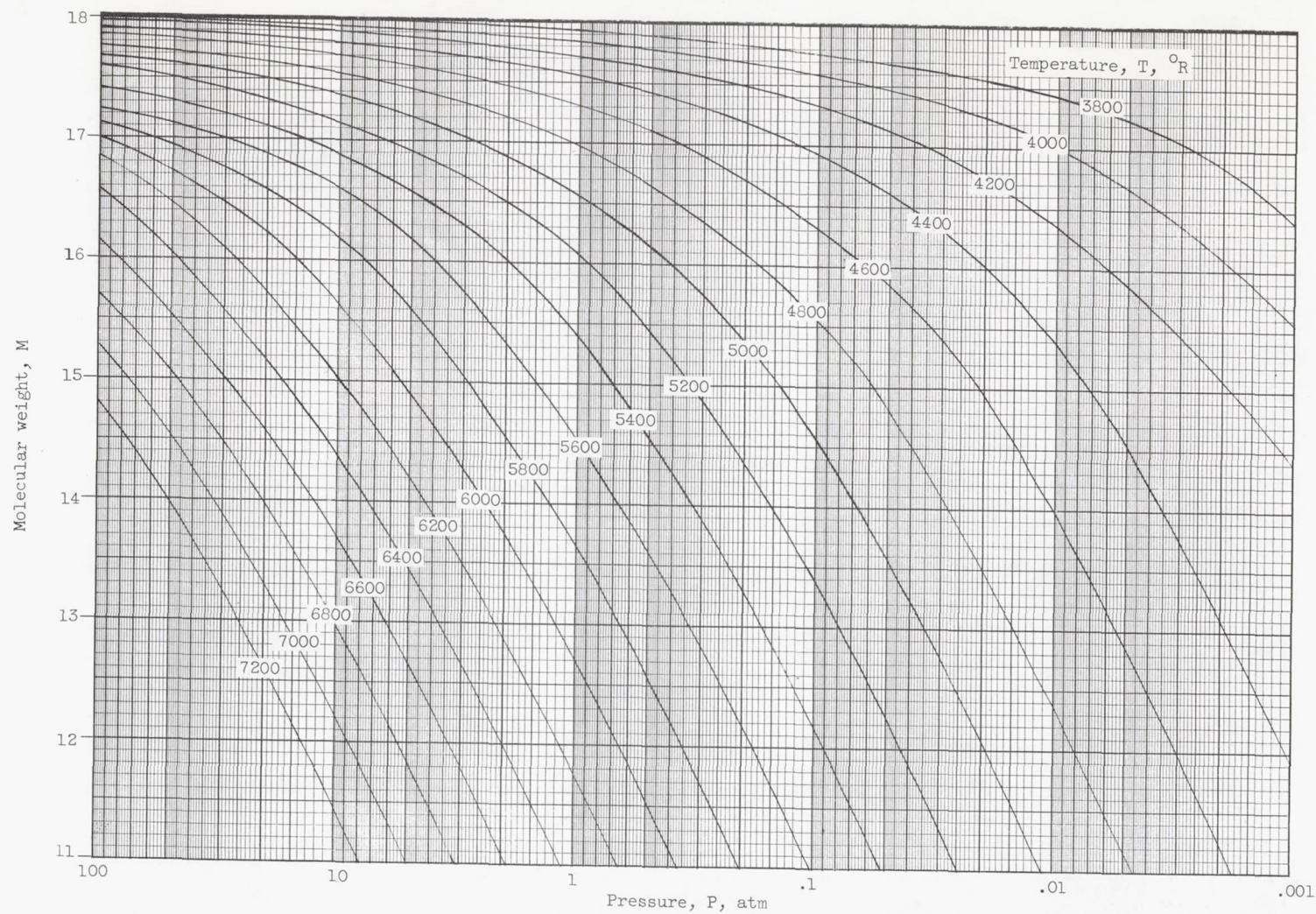
Figure 2. - Concluded. Thermodynamic data for water vapor, including effects of dissociation.
