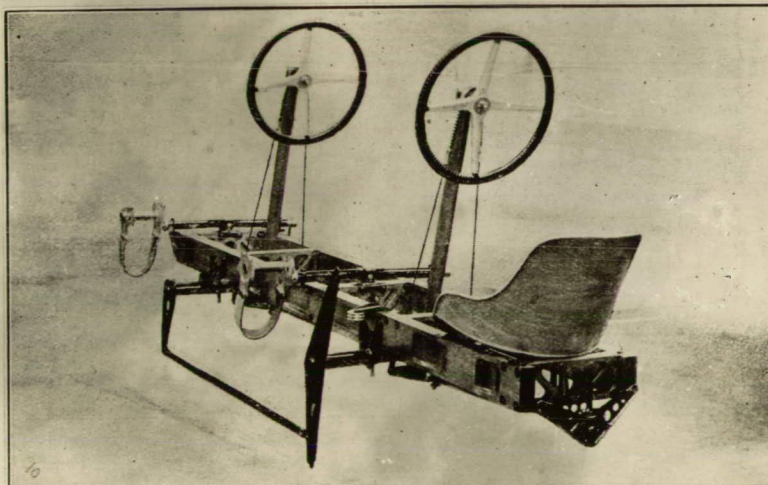
Fig.10 The controls are built up in the form of complete units, one of which is shown.
