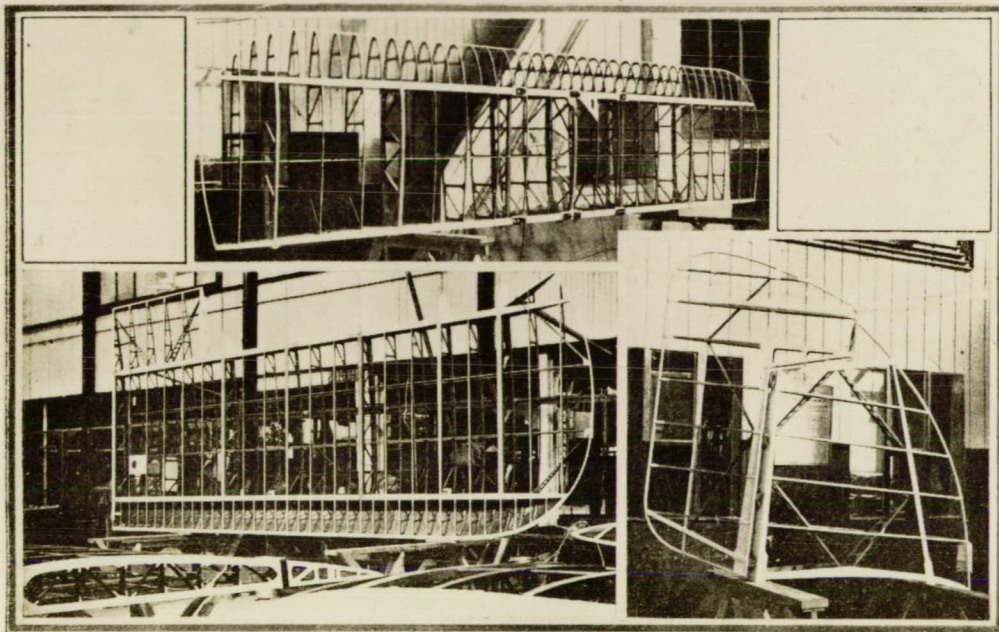
Fig.4 Skeleton of stabilizer, wing, and rudder.
