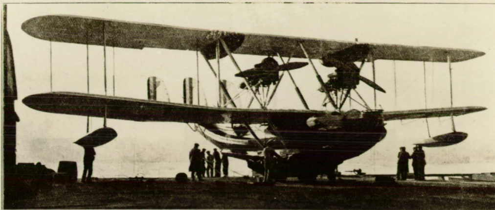
Fig.1 Three-quarter view of "Southampton" seaplane on the slipway, giving a good idea of the somewhat unusual arrangement of the interplane struts. The Napier "Lion" engines are mounted on struts independent of the wing structure and can be removed without interfering with the wing bracing.
