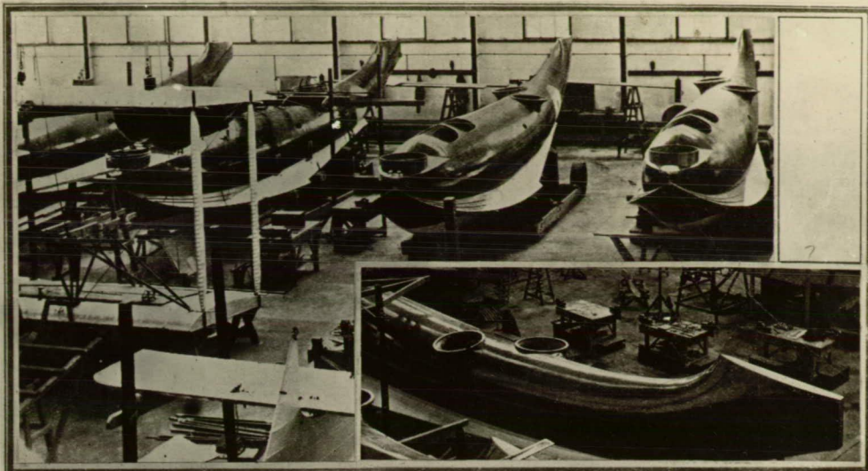
Fig.7 Hulls of the Supermarine "Southampton". Note the staggered cockpits for the rear gunners.
