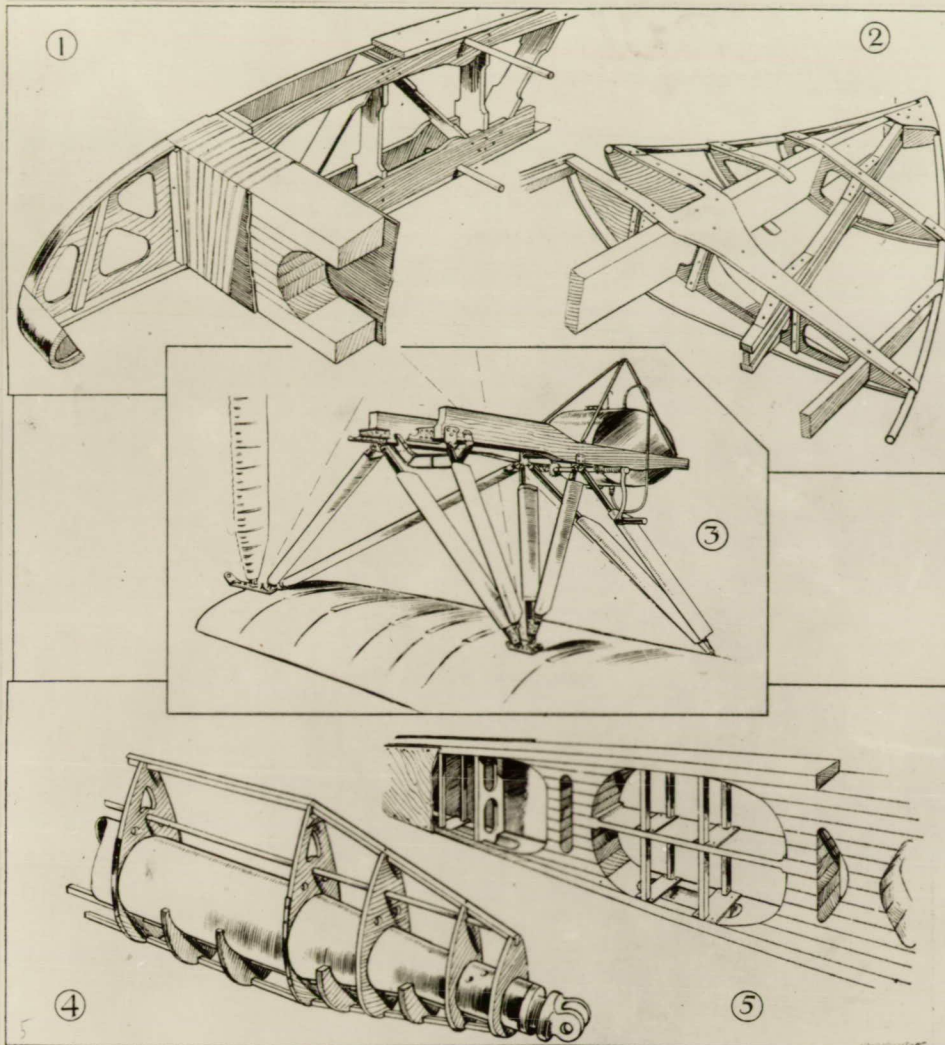
Fig. 5 Some constructional details.
