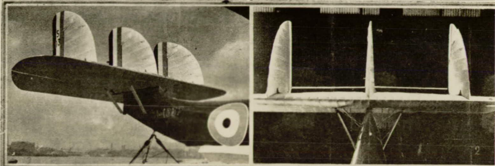
Fig.3 Two views of the cantilever tail, illustrating how little the field of fire is interfered with by the tail.
