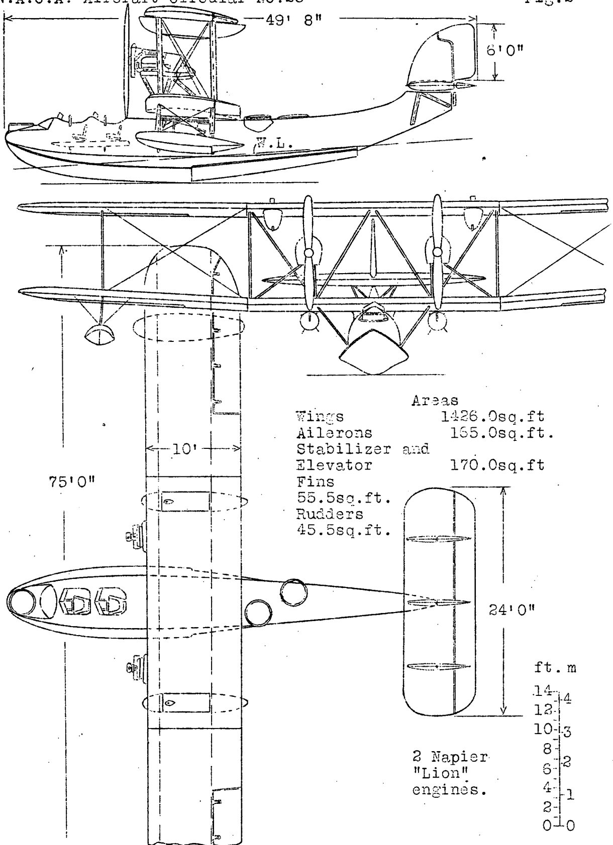
Fig.2 Supermarine "Southampton" seaplane.
