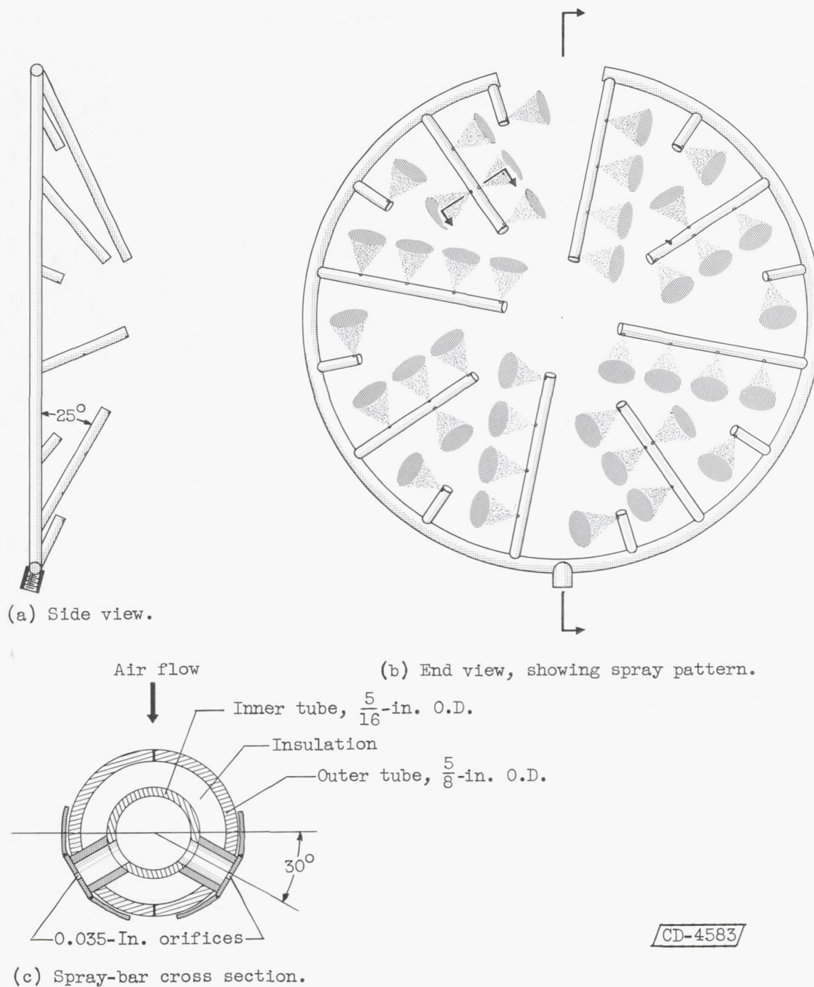
Figure 3. - Pentaborane fuel injector.
