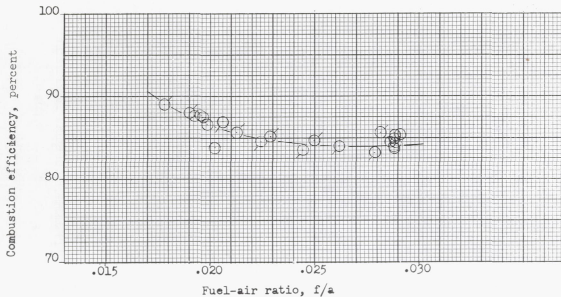
(a) First test; combustor length, 8 feet.
