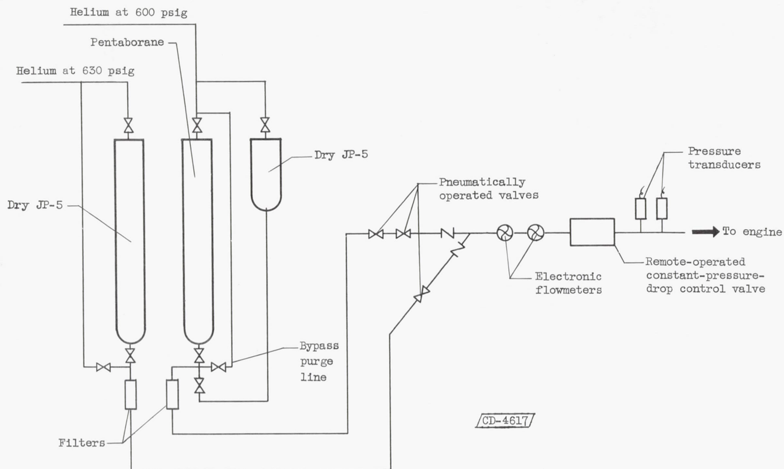
Figure 4. - Fuel system for pentaborane combustion tests.
