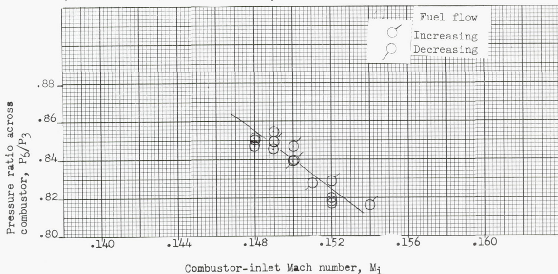
(b) Second test; combustor length, 6 feet (free-jet air flow broken down).
