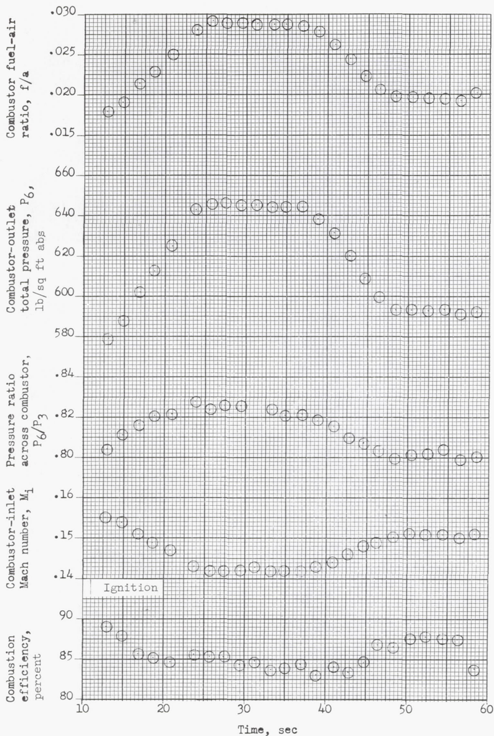
Figure 6.- Performance of pentaborane combustor in first test as indicated by fast-response instrumentation. Combustor length, 8 feet.
