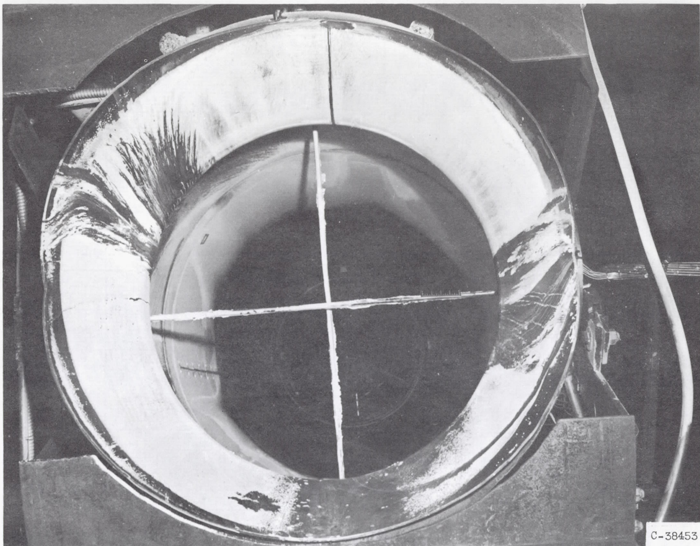
Figure 10. - Oxide deposits on 48-inch-diameter ram-jet engine after 1 minute of pentaborane combustion.
