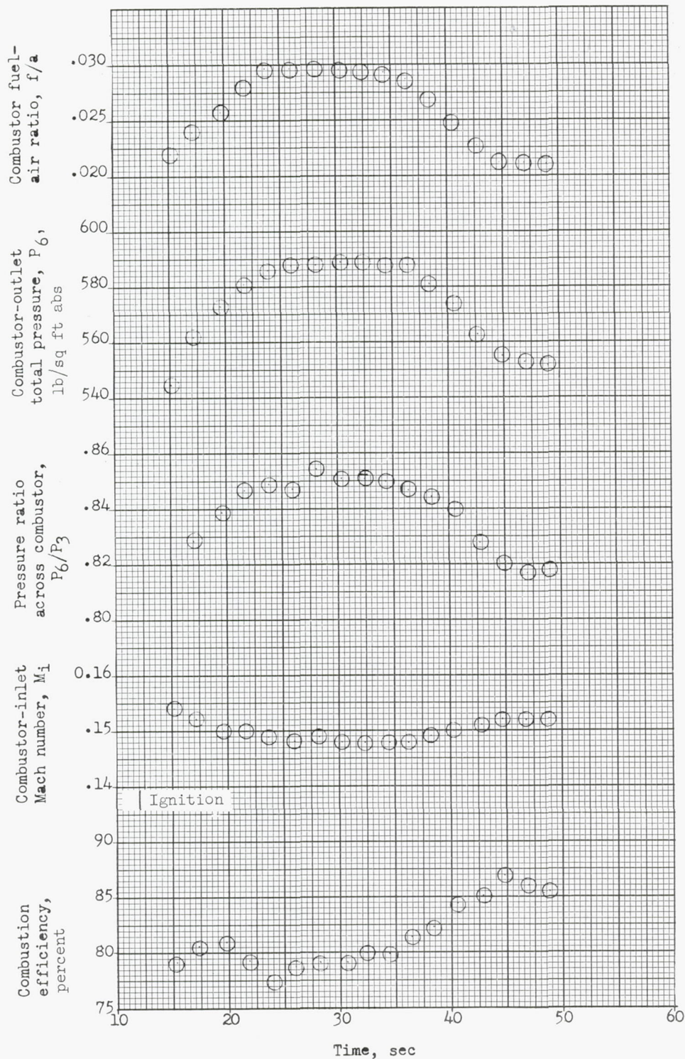
Figure 7. - Performance of pentaborane combustor in second test as indicated by fast-response instrumentation. Combustor length, 6 feet.
