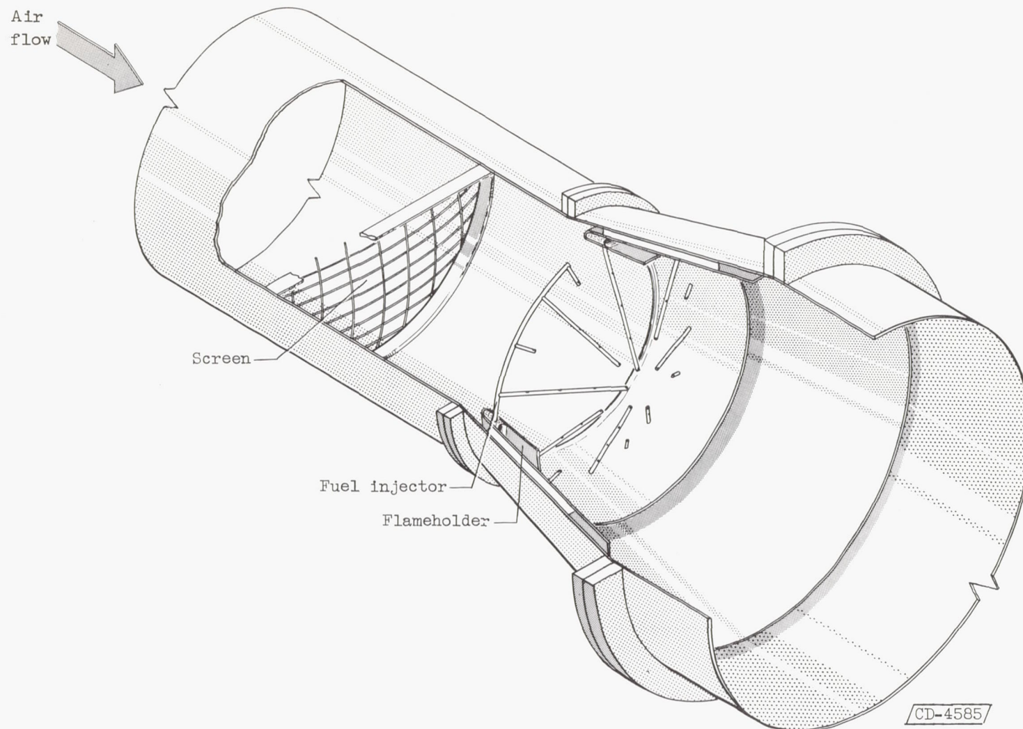
Figure 2. - Cutaway view of 48-inch-diameter ram-jet engine showing flameholder and fuel injector.
