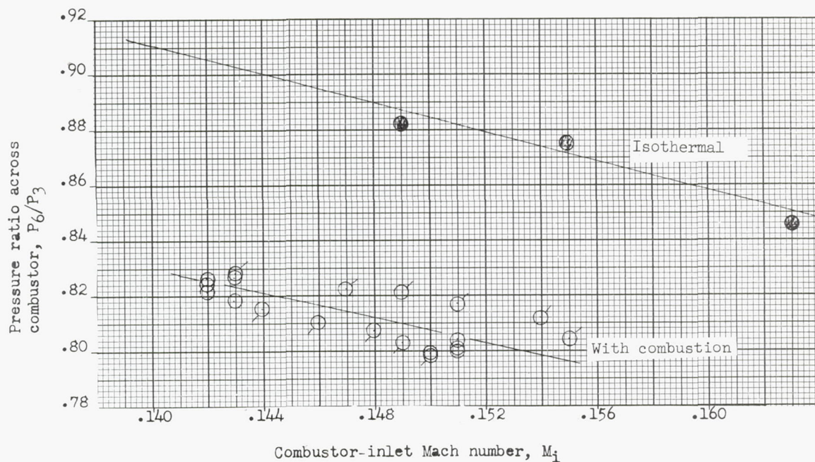
(a) First test; combustor length, 8 feet.
