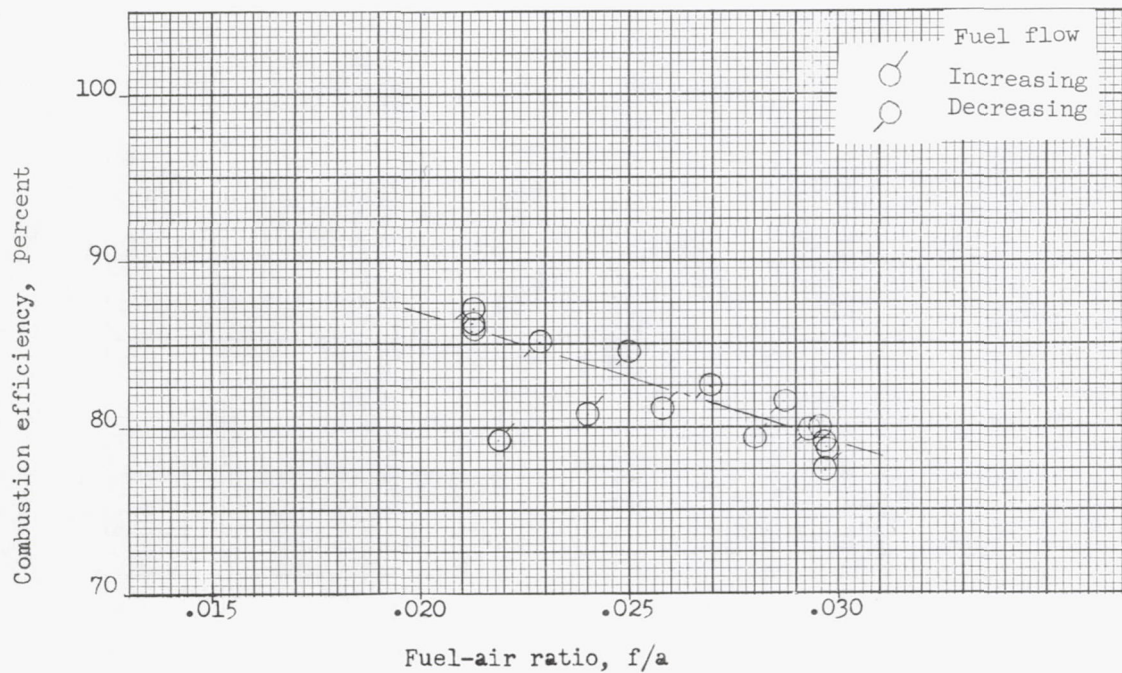
(b) Second test; combustor length, 6 feet (free-jet air flow broken down).
