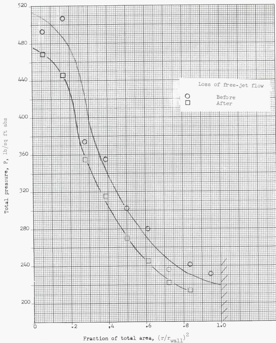
Figure 11.- Pressure profiles at ram-jet-engine outlet before and after loss of free-jet flow.
