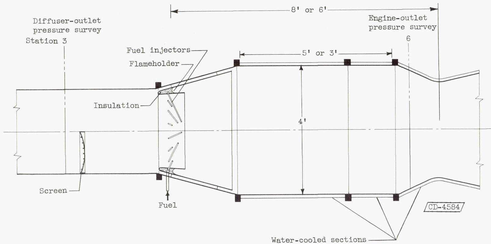
Figure 1. - Ram-jet engine used to study pentaborane combustion.
