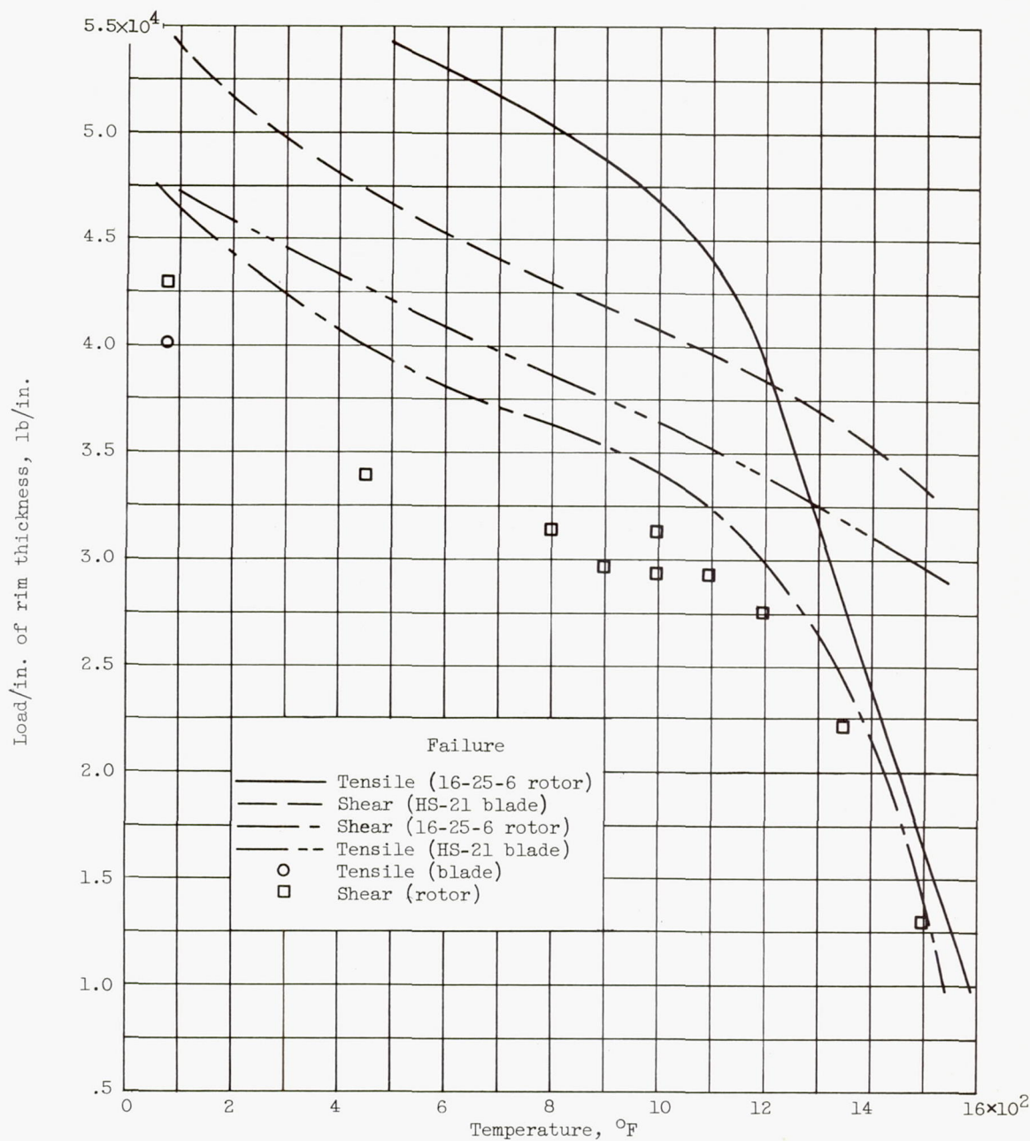
Figure 12. - Continued. Mechanism of short-time failure as result of variations in temperature.
