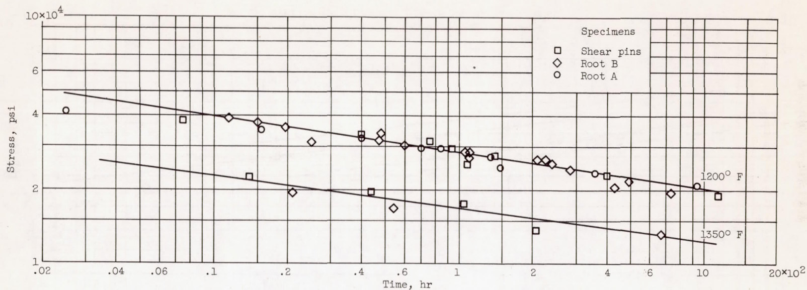
(c) Shear properties of Timken 16-25-6 at 1200° and 1350° F.
