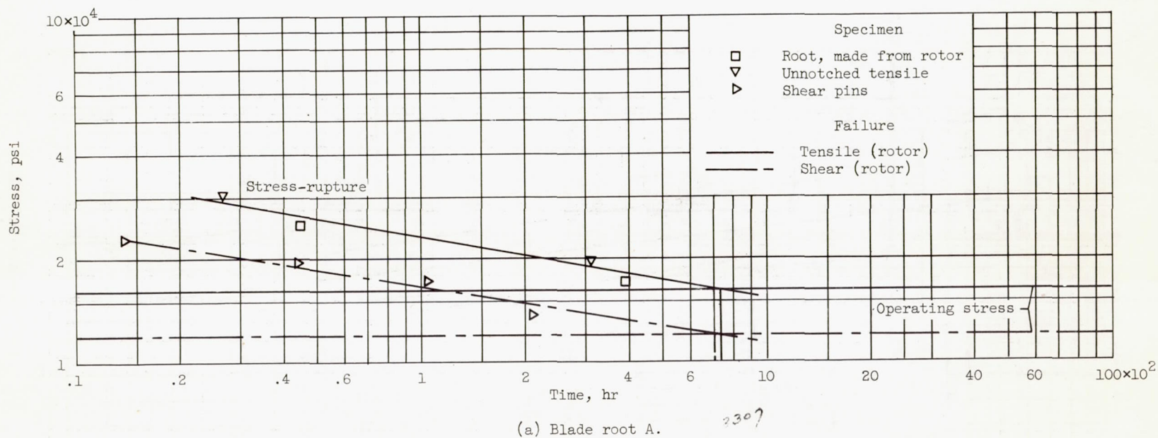
Figure 15. - Stress-rupture data for turbine rotor at 1350° F. Specimens of Timken 16-25-6.
