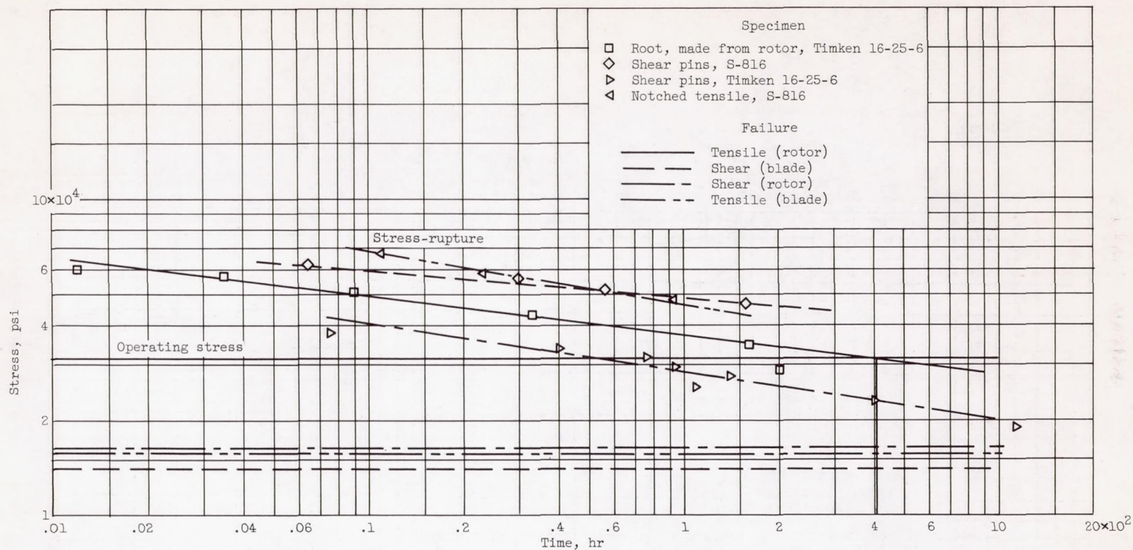
Figure 14. - Concluded. Stress-rupture results determined at 1200° F.
