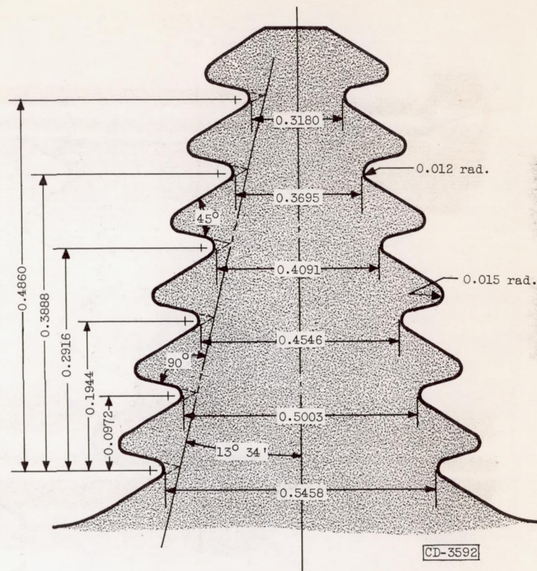
(b) Turbine rotor segment A.
