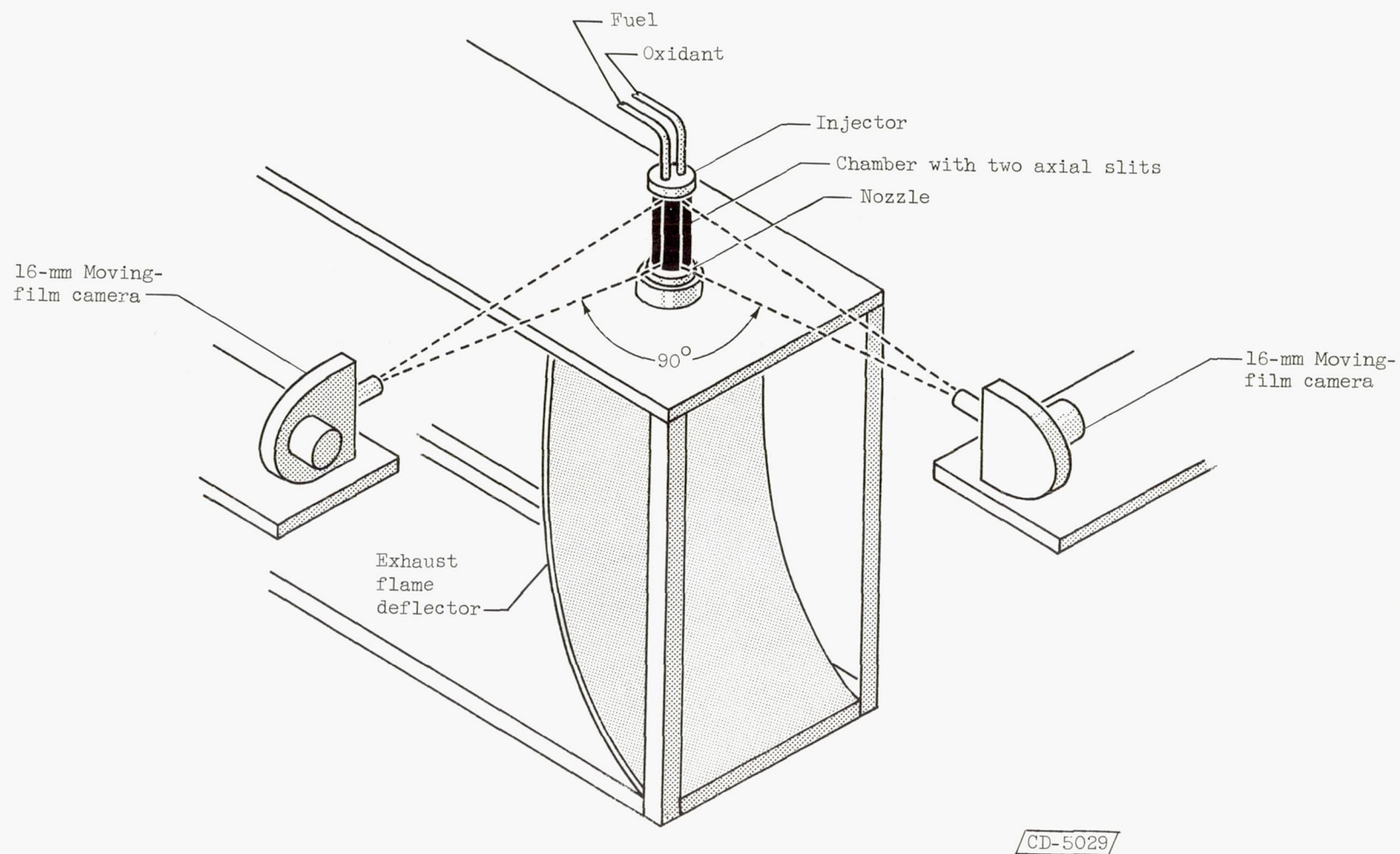
Figure 3. - Rocket engine and photographic arrangement.
