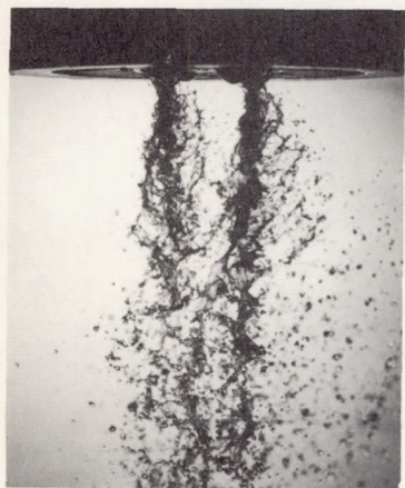
(a) Impinging-jets injector; parallel orientation of sprays.
