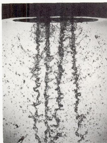
(h) Fuel-sheet - oxidant-jet injector; butt orientation of sprays.
