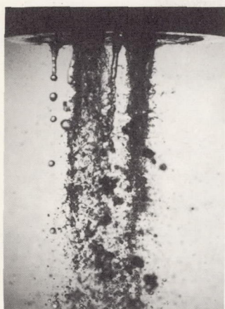
(e) Parallel-sheets injector; parallel orientation of sprays.
