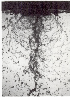
(f) Parallel-sheets injector; butt orientation of sprays.
