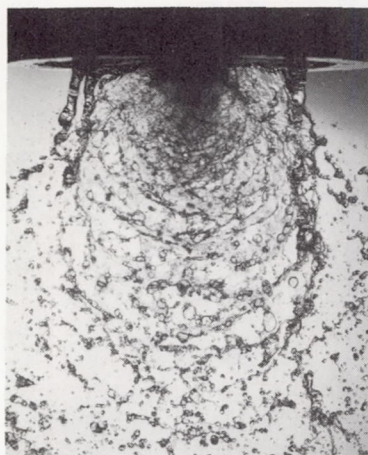
(c) Impinging-sheets injector; parallel orientation of sprays.
