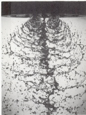
(b) Impinging-jets injector; butt orientation of sprays.
