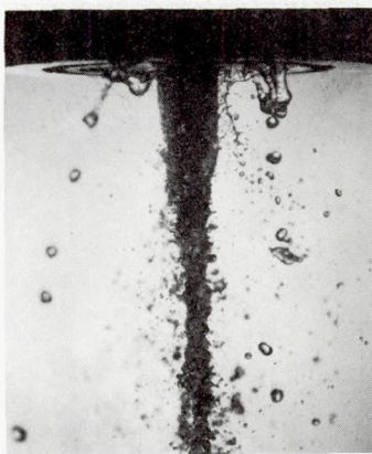
(f) Parallel-sheets injector; butt orientation of sprays.
