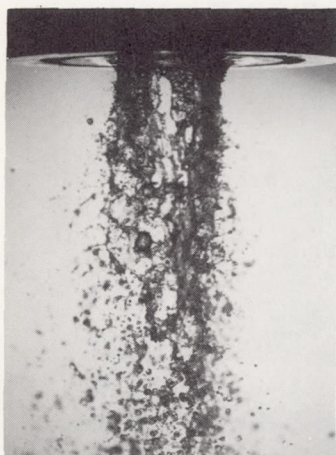
(c) Impinging-sheets injector; parallel orientation of sprays.
