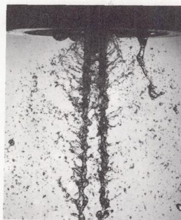
(g) Fuel-sheet - oxidant-jet injector; parallel orientation of sprays.
