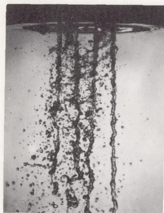
(g) Fuel-sheet - oxidant-jet injector; parallel orientation of sprays.
