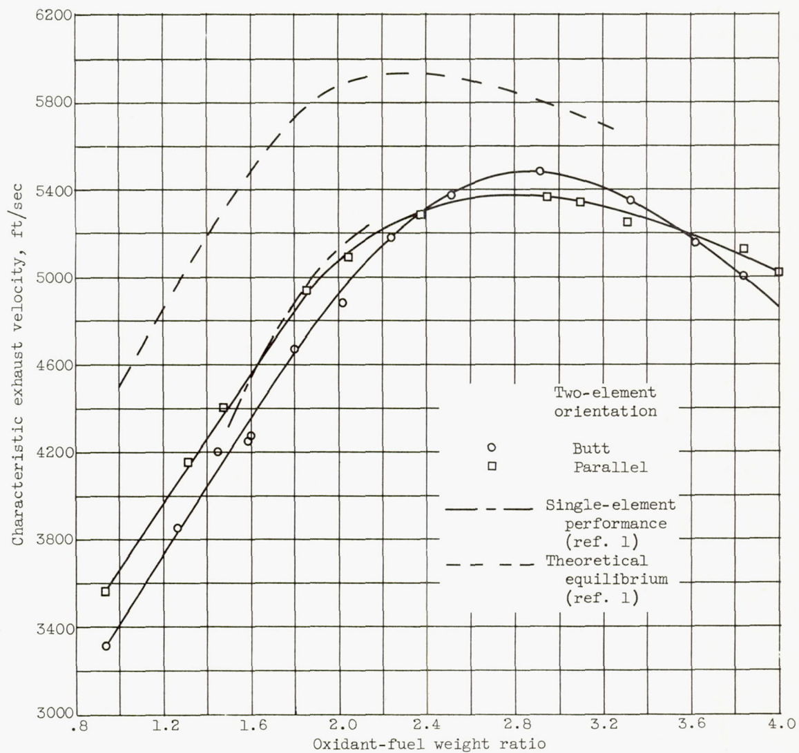
Figure 4. - Performance characteristics of several injection methods.
