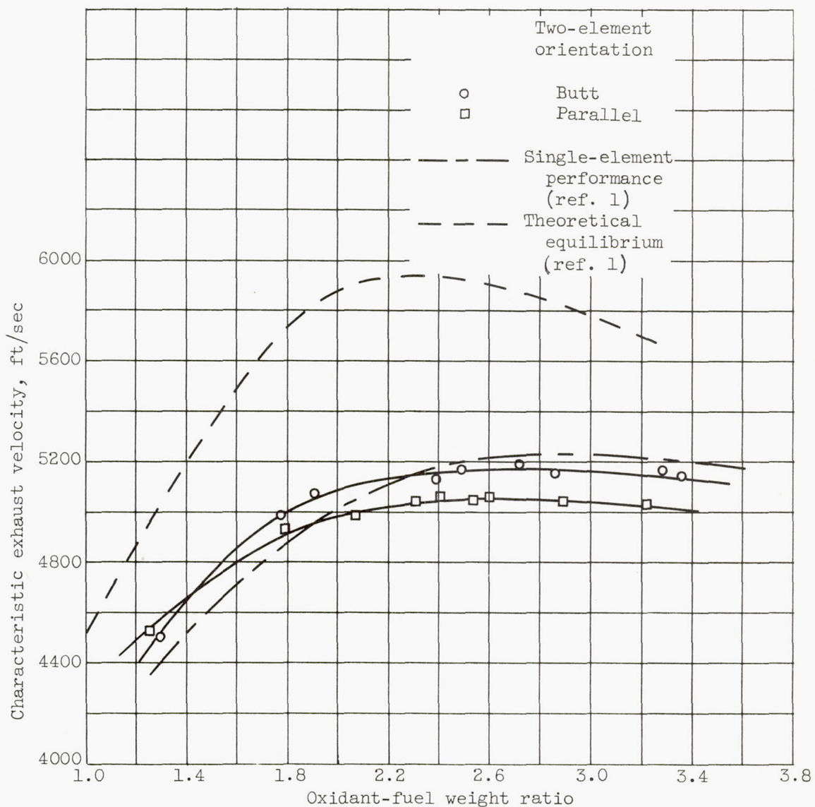
Figure 4. - Continued. Performance characteristics of several injection methods.
