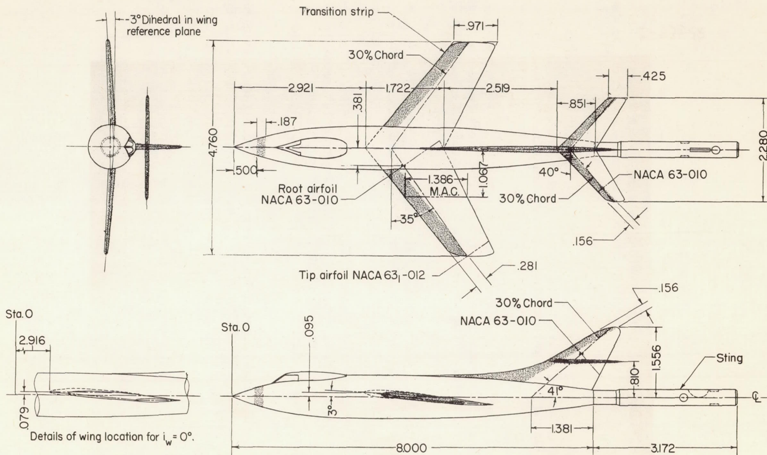
Figure 1.- Drawing of the complete model. All dimensions are in inches.
