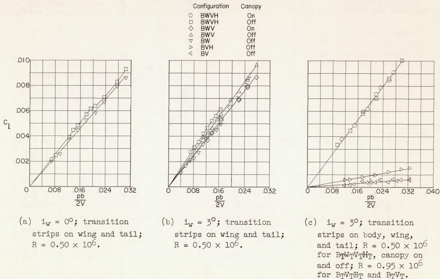
Figure 6.- Variations of rolling-moment coefficient with wing-tip helix angle for complete configuration and its components. With transition strips; M = 1.62 . Flagged symbols indicate check points.
