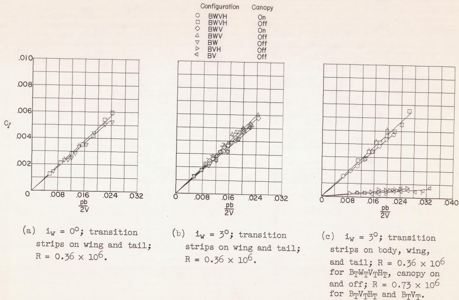
Figure 9.- Variations of rolling-moment coefficient with wing-tip helix angle for complete configuration and its components. With transition strips; M = 2.41 . Flagged symbols indicate check points.
