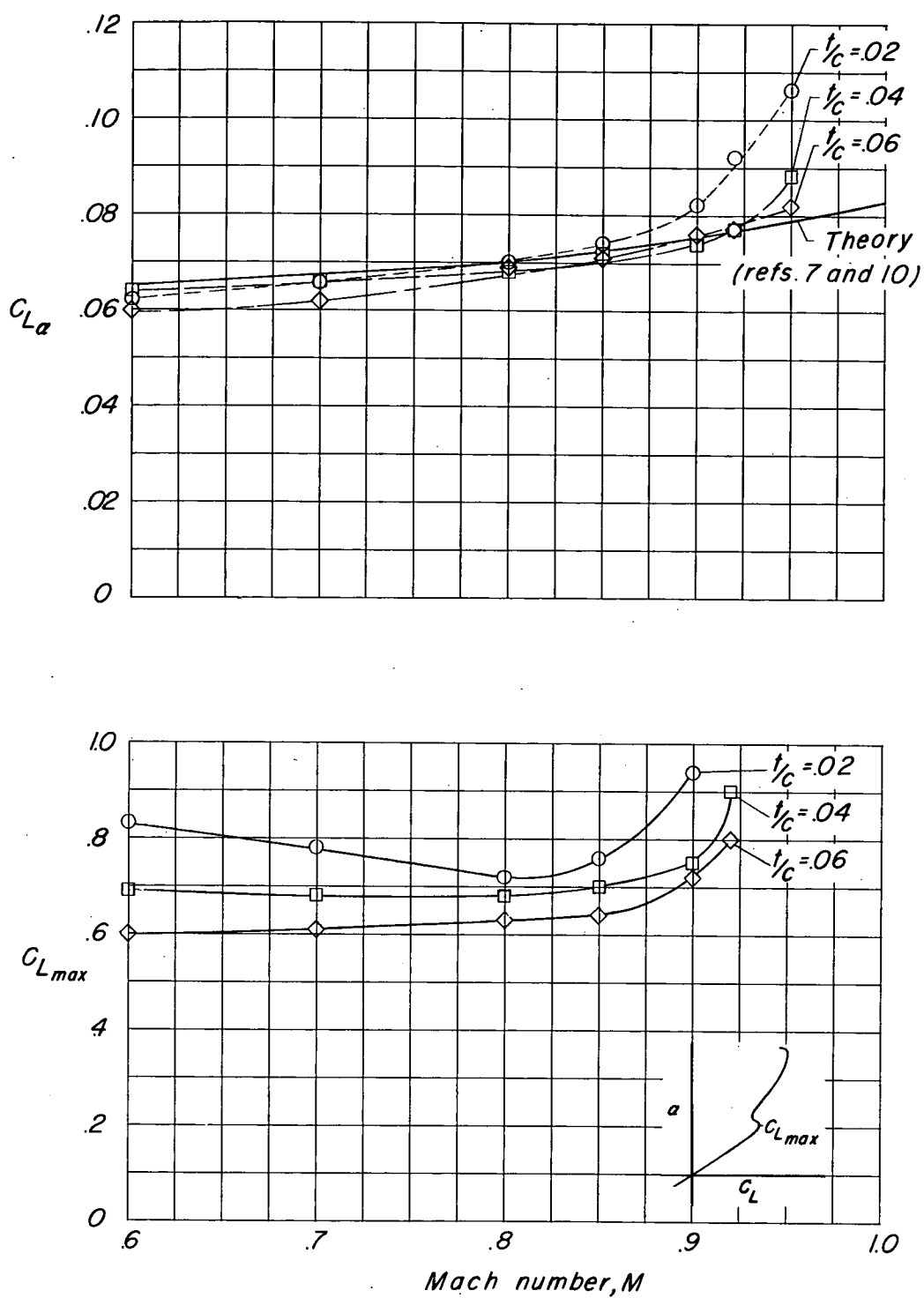
Figure 9.- Variation of lift-curve slope and maximum lift coefficient with Mach number.
