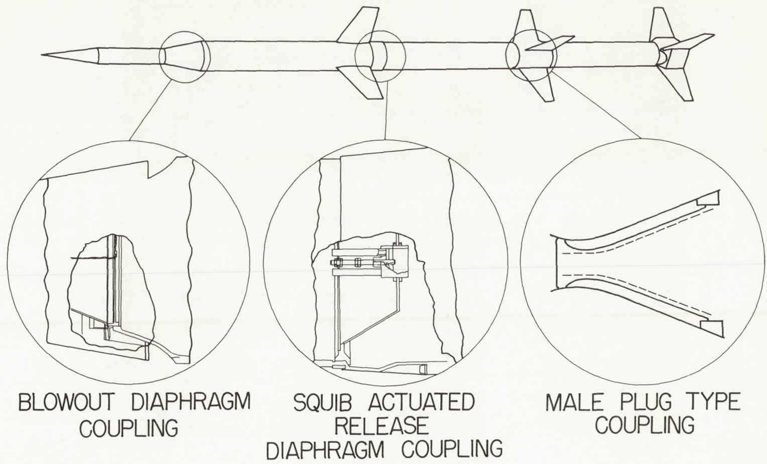
Figure 2.- Typical model-booster couplings.
