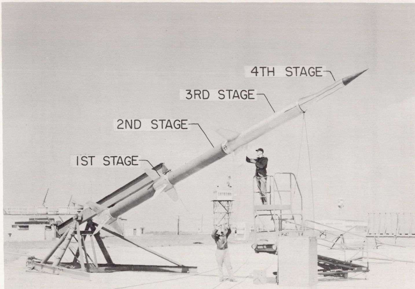
Figure 1.- Typical four-stage model.
