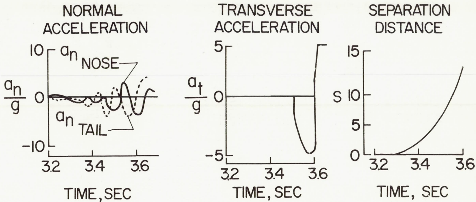
Figure 6.- Booster acceleration during separation.
