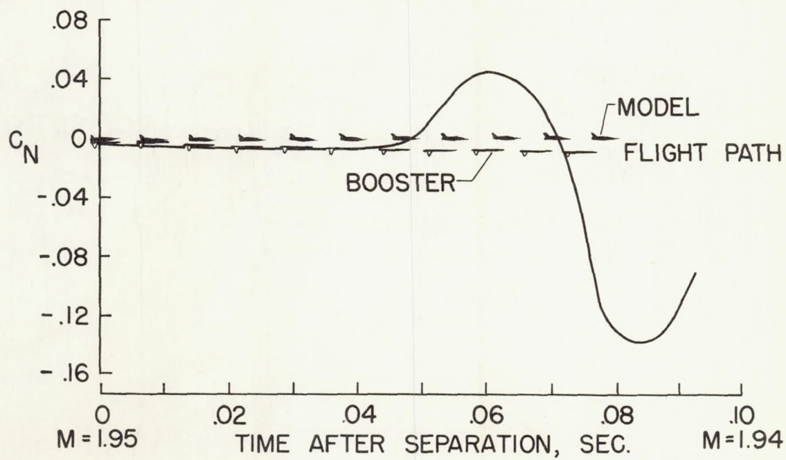
Figure 8.- Separation study of single underslung booster.
