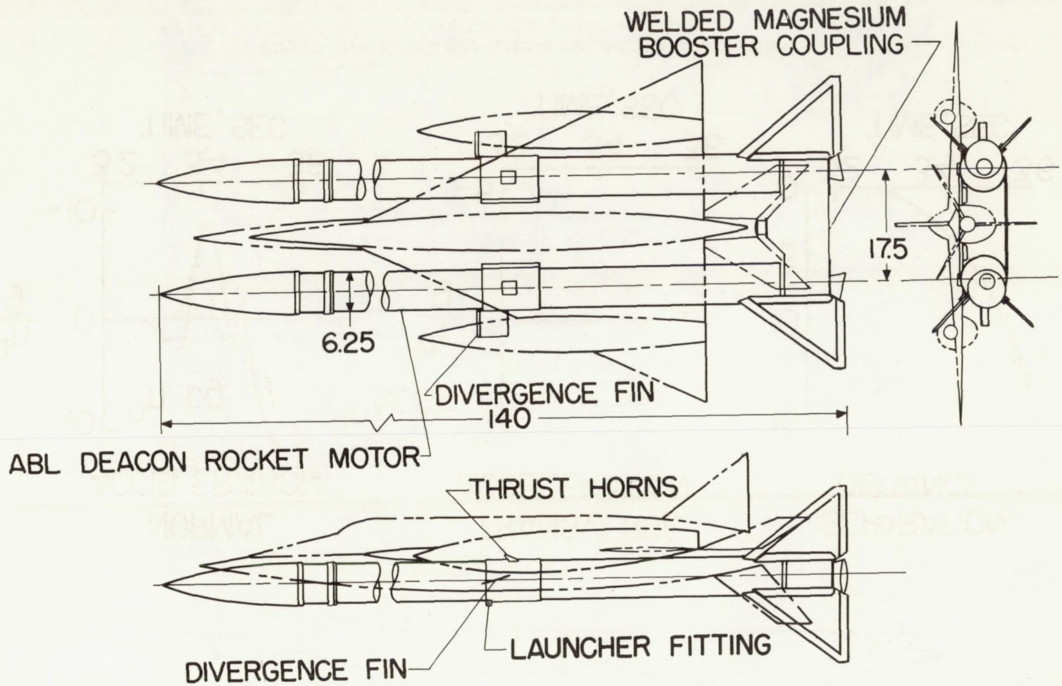
Figure 4.- Typical double underslung booster arrangement.
