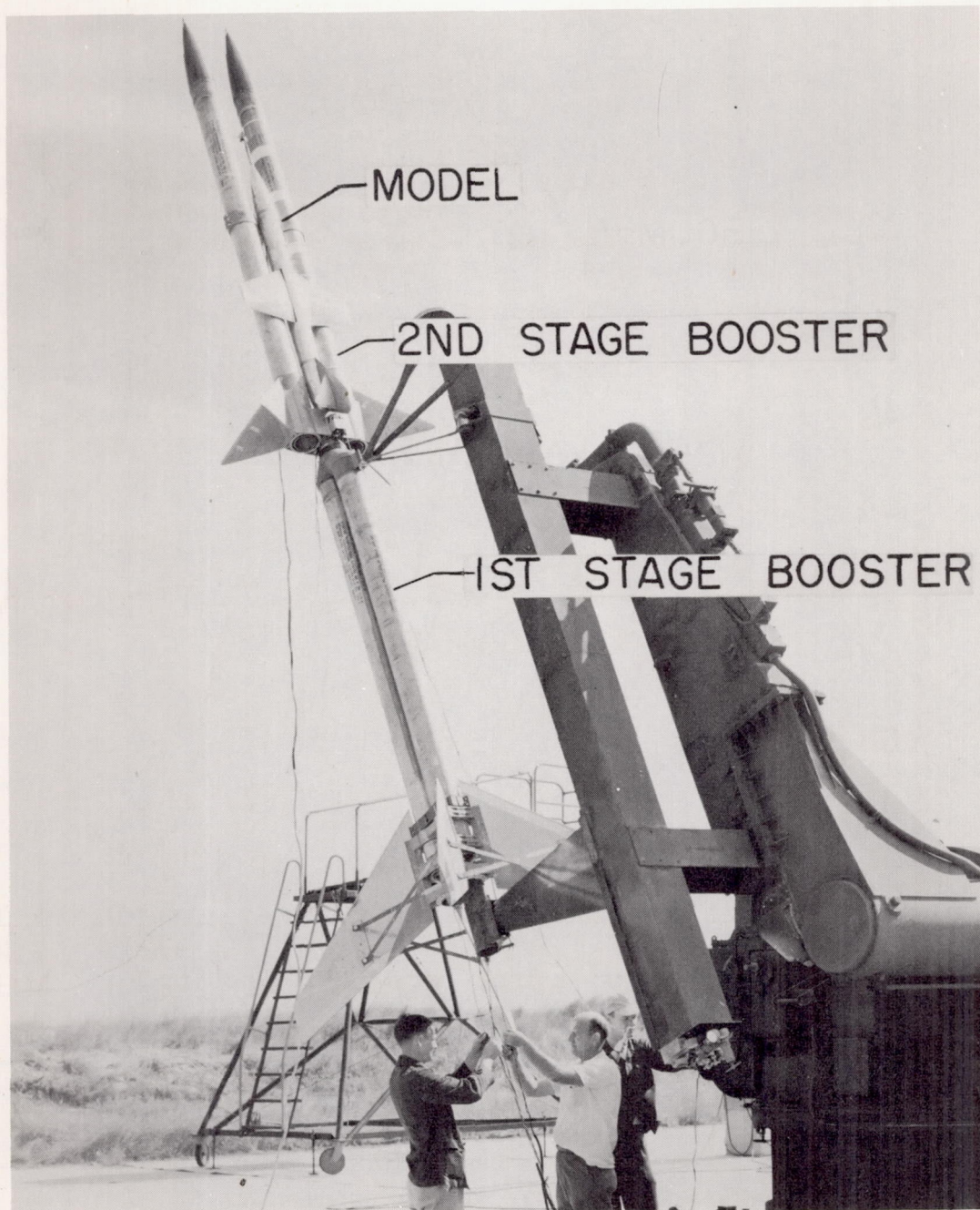
Figure 9.- Typical tandem-underslung boost arrangement.
