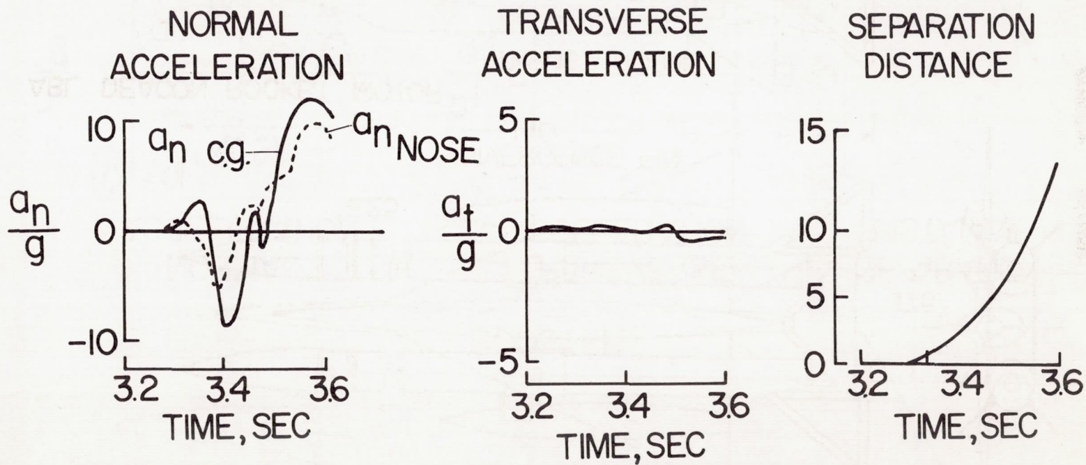
Figure 5.- Model accelerations during separation.
