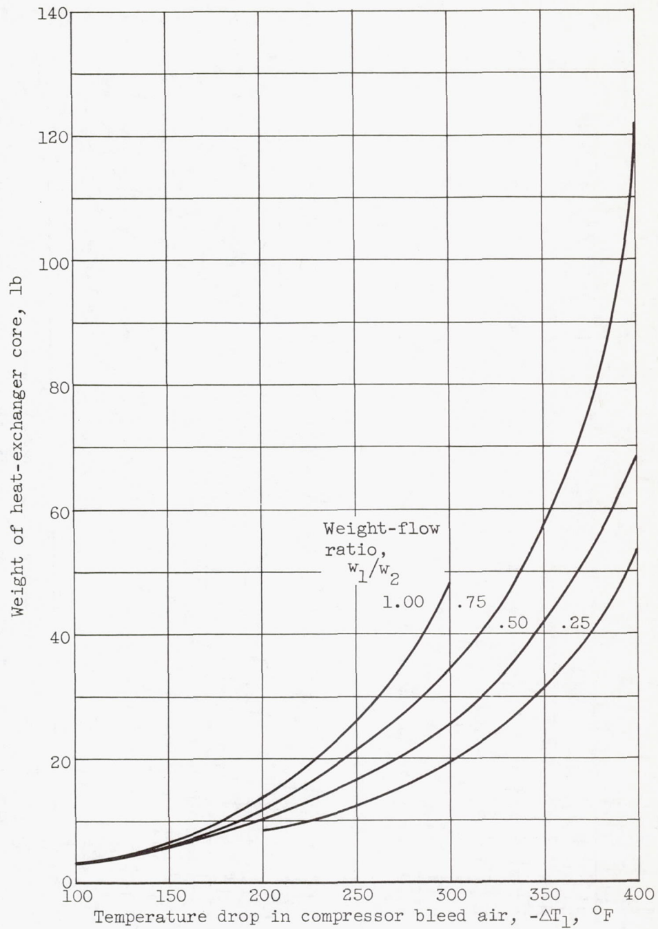
Figure 10. - Weight of heat-exchanger core against temperature drop in compressor bleed air. Compressor-bleed-air weight-flow rate, 2.70 pounds per second; metal thickness, 0.004 inch; density of metal, 0.300 pound per cubic inch.
