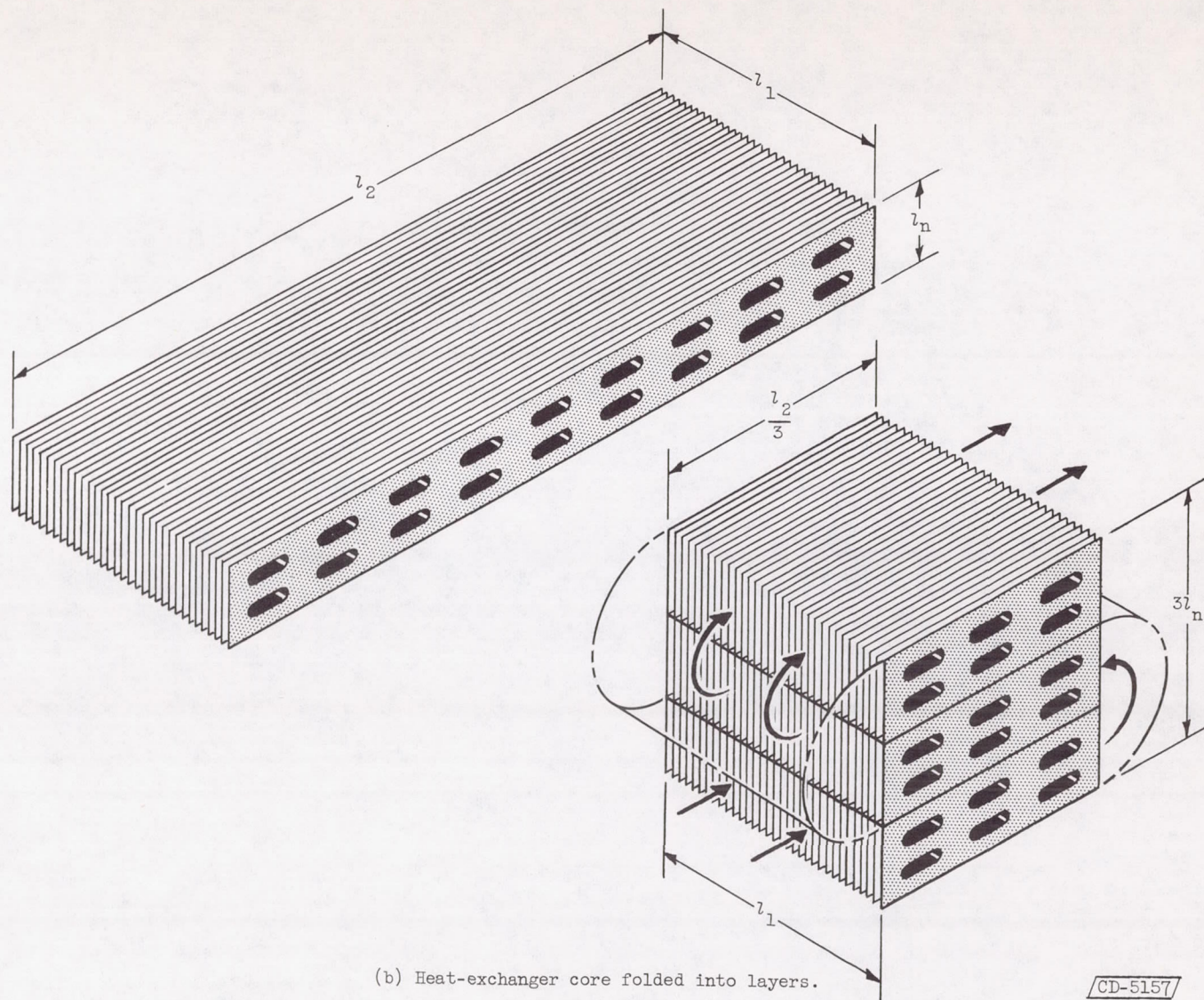
Figure 14. - Concluded. Heat-exchanger core arrangement.
