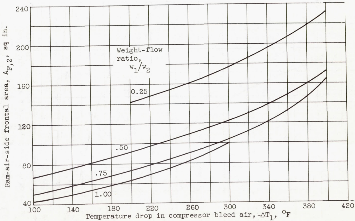
Figure 12. - Ram-air-side frontal area against temperature drop of compressor bleed air. Compressor-bleed-air weight-flow rate, 2.70 pounds per second; ratio of free-flow to frontal area, 0.697.
