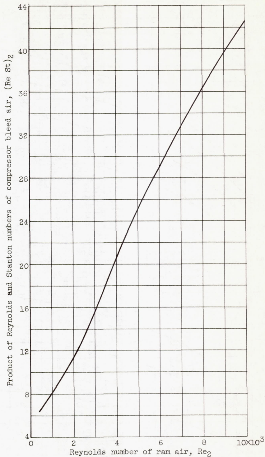
Figure 8. - Rearrangement of heat-transfer characteristics of finned-tube configuration. Prandtl number Pr^{2/3} = 0.75 .
