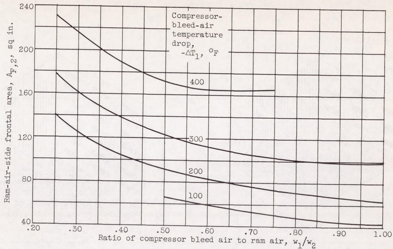
Figure 13. - Ram-air-side frontal area against ratio of compressor bleed air to ram air bleed. Compressor-bleed-air weight-flow rate, 2.70 pounds per second; ratio of free-flow to frontal area, 0.697.
