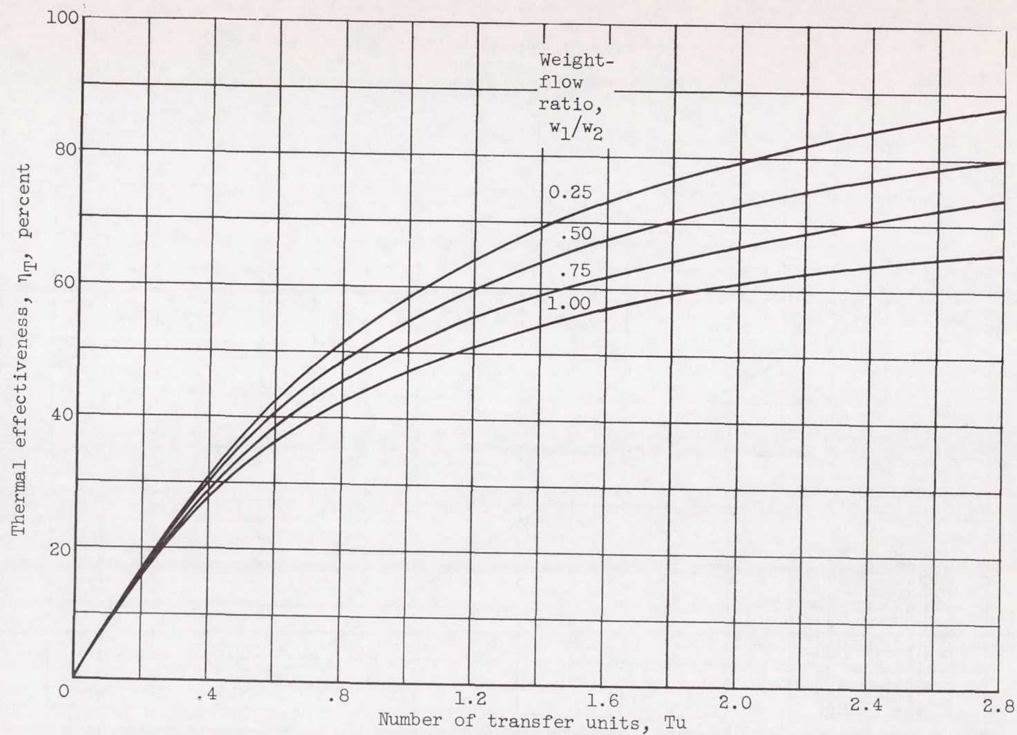
Figure 4. - Performance of crossflow heat exchanger with fluids unmixed. (Specific heat at constant pressure assumed constant.)
