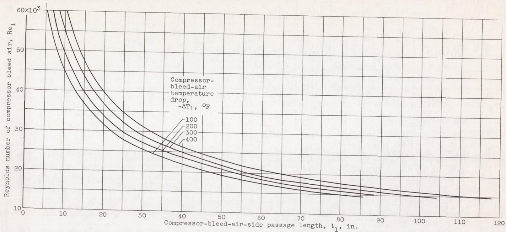
Figure 6. - Graphical representation of equation (3) for inlet state, temperature and pressure drops, and flow characteristics corresponding to compressor bleed air. Pressure drop, 1000 pounds per square foot; inlet pressure, 5300 pounds per square foot; inlet temperature, 1410^\circ R ; ratio of free-flow to frontal area, 0.219; hydraulic diameter, 0.018 foot.
