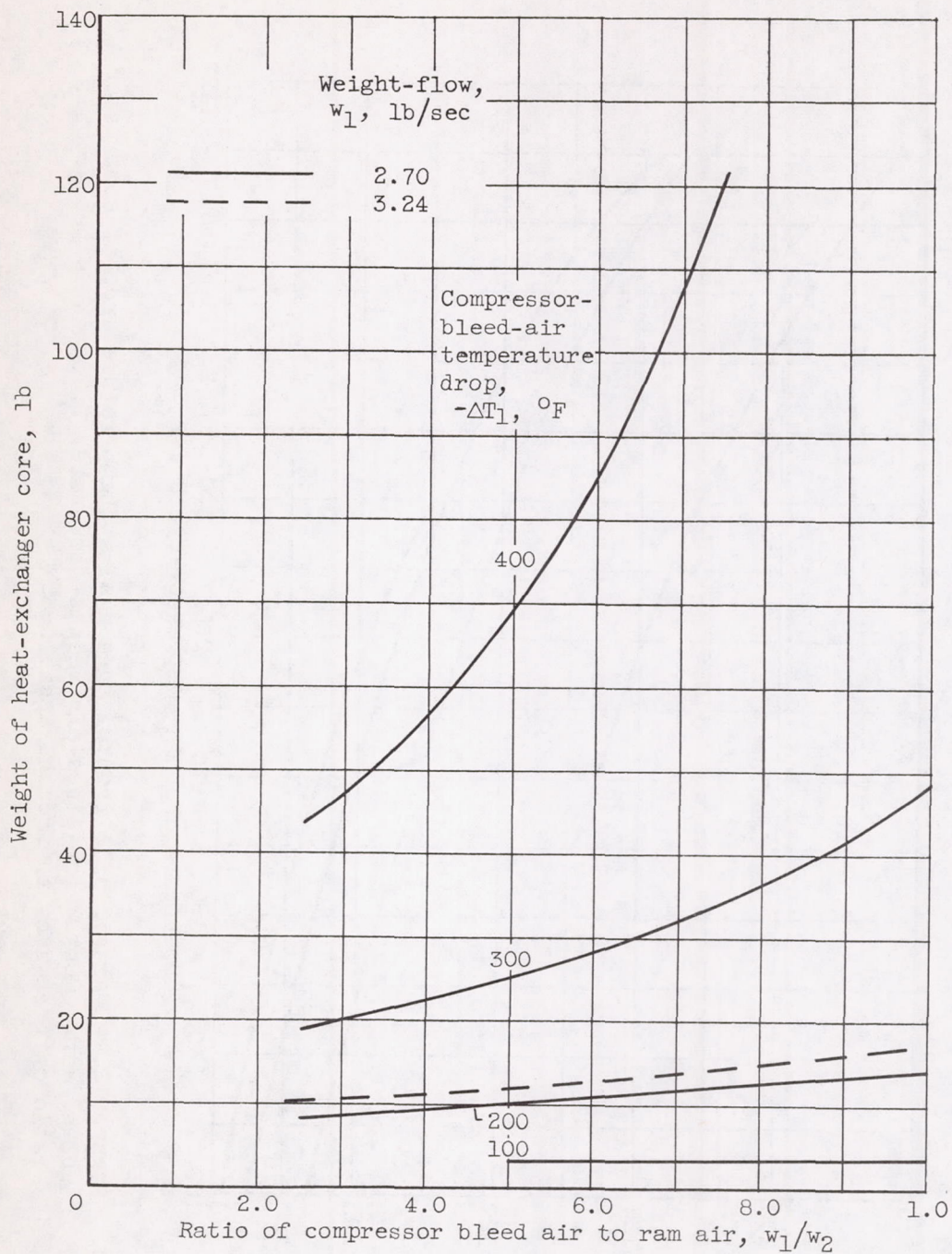
Figure 11. - Weight of heat-exchanger core against rate of compressor bleed air to ram bleed air. Compressor-bleed-air weight-flow rate, 2.70 pounds per second; metal thickness, 0.004 inch; density of metal, 0.300 pound per cubic inch.
