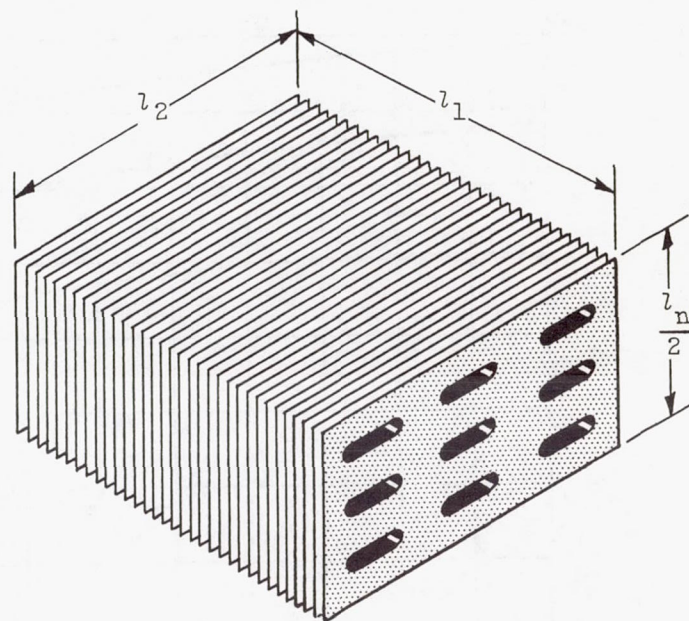
(a) Heat-exchanger core divided into segments.
