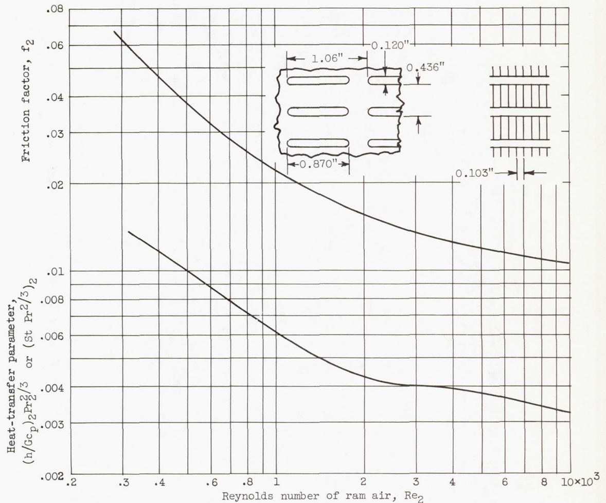
Figure 3. - Heat-transfer and friction data for finned-tube heat-exchanger core (ref. 5).
