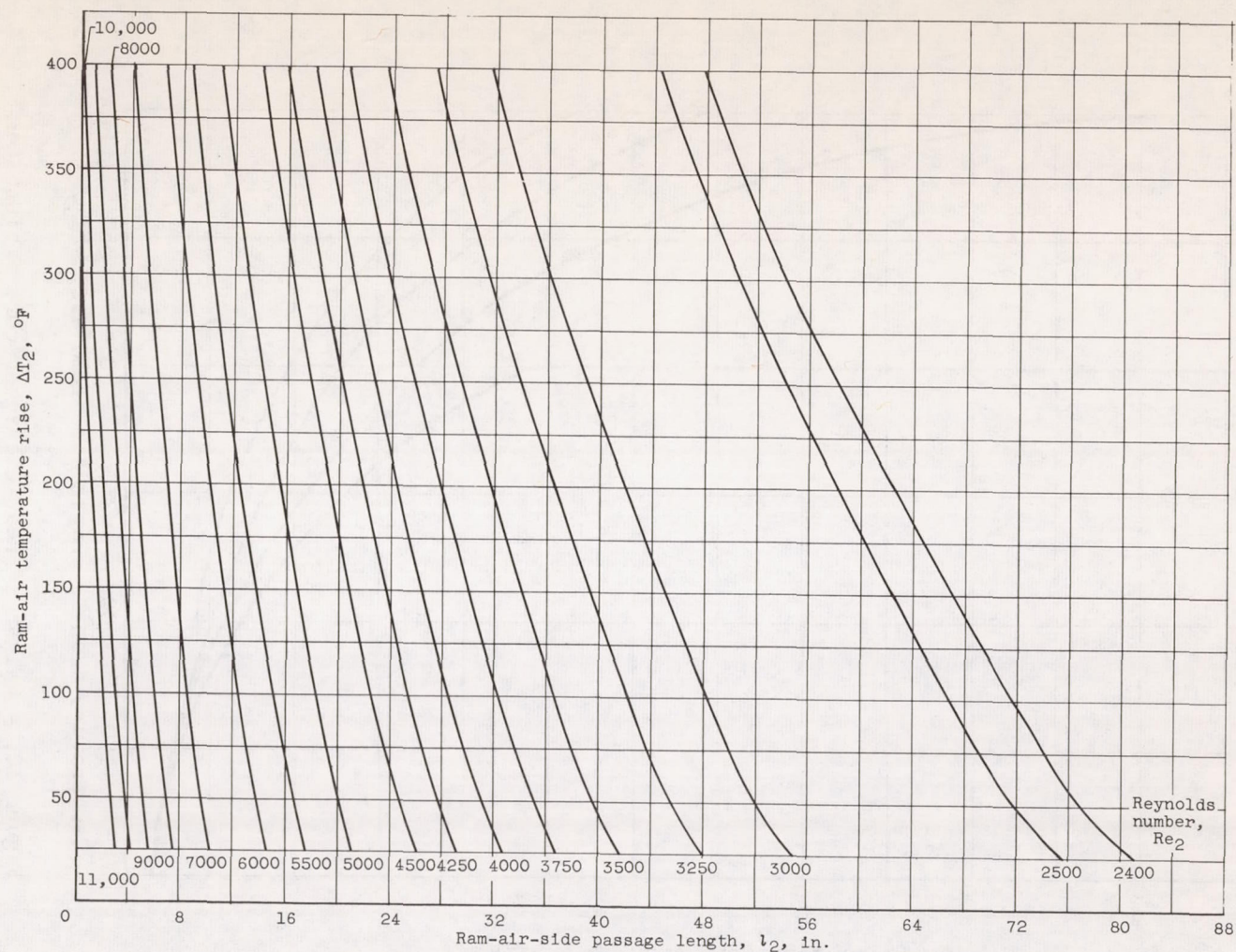
Figure 9. - Graphical representation of equation (3) for inlet-state; temperature and pressure drops and flow characteristics corresponding to ram air bleed. Ram-air pressure drop, 400 pounds per square foot; inlet pressure, 1080 pounds per square foot; inlet temperature, 880° R; ratio of free-flow to frontal area, 0.697; hydraulic diameter, 0.0118 foot.
