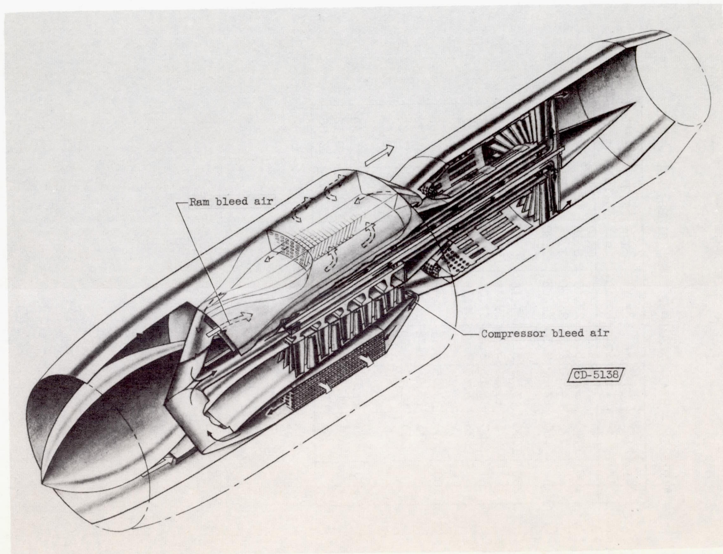
Figure 1. - Heat-exchanger installation on jet engine.
