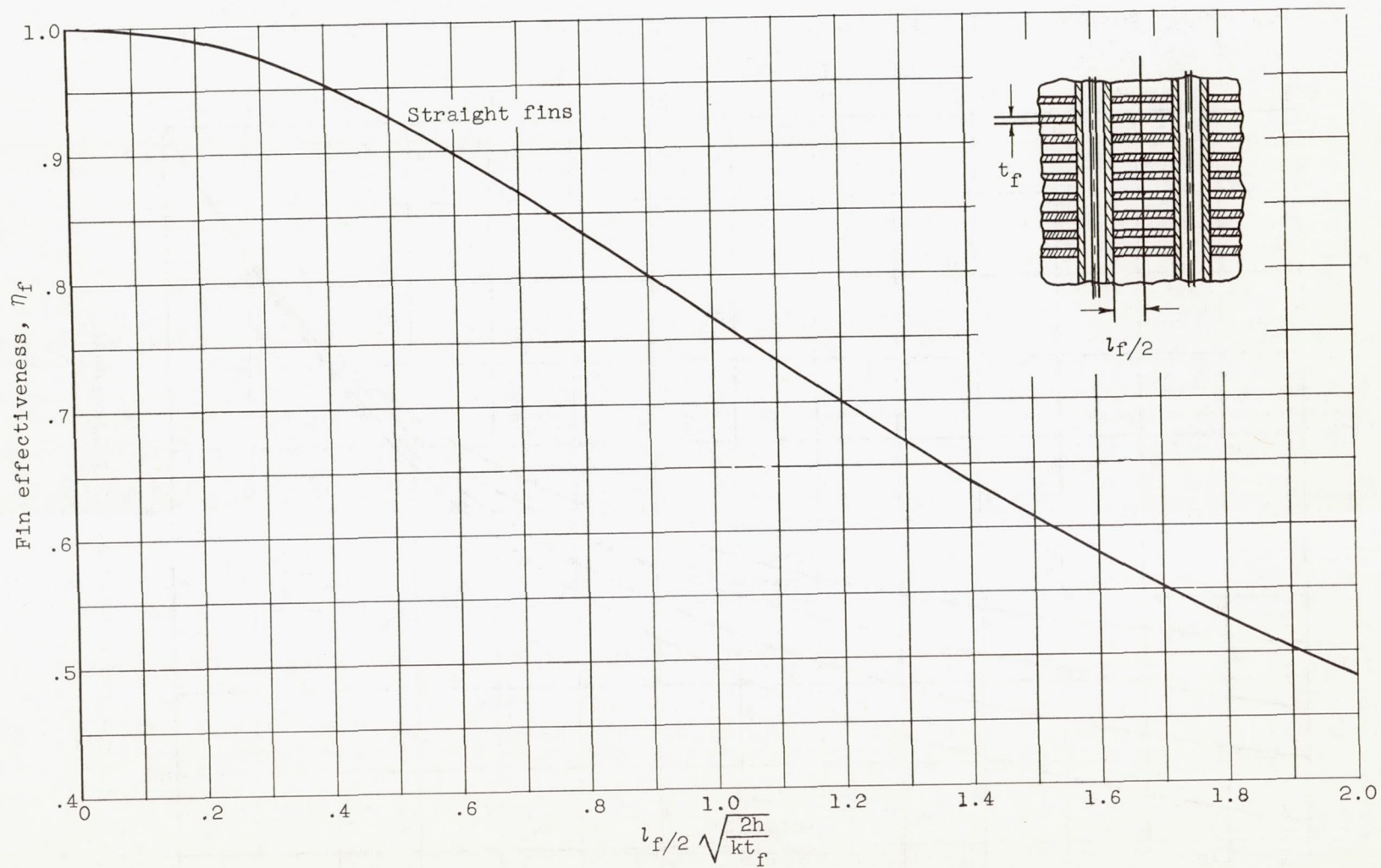
Figure 5. - Effectiveness for straight fins.
