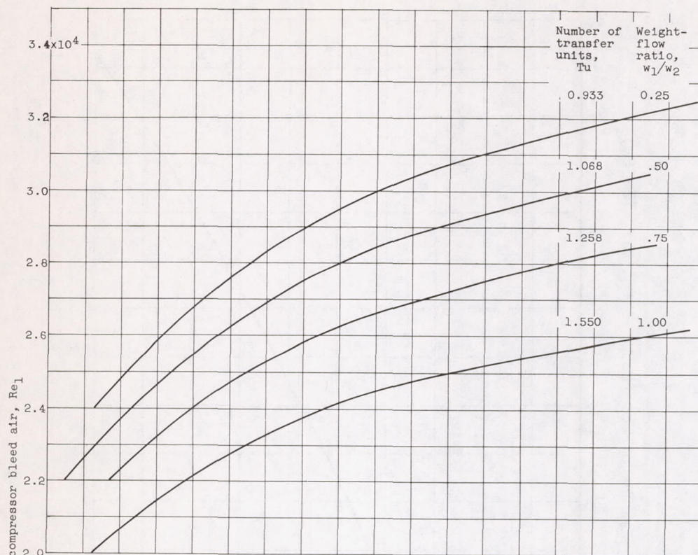
(c) Compressor-bleed-air temperature drop, \Delta T_1 = -300^\circ \text{F} .
