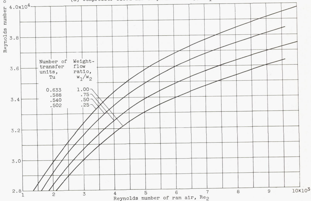
(b) Compressor-bleed-air temperature drop, \Delta T_1 = -200^\circ \text{ F.}
