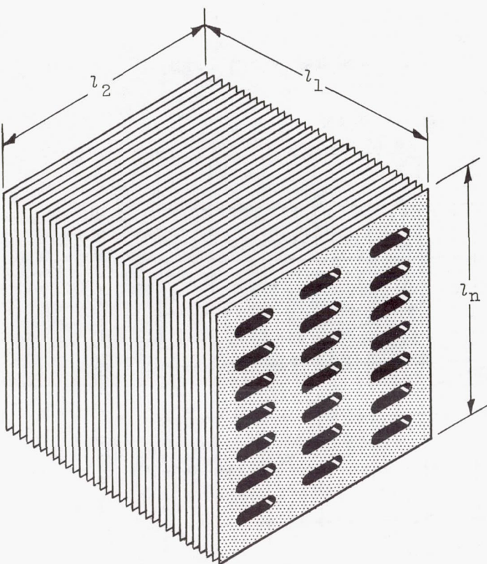
(a) Heat-exchanger core divided into segments.
