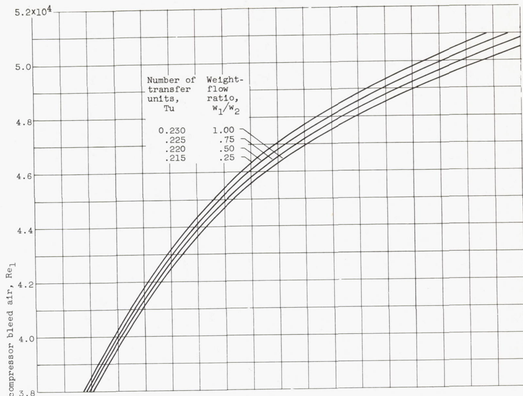
(a) Compressor-bleed-air temperature drop, \Delta T_1 = -100^\circ \text{ F.}
