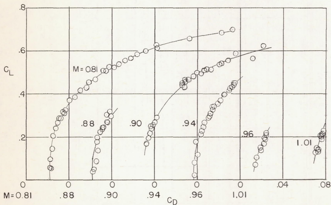
Figure 5.- Variation of lift coefficient with drag coefficient for several Mach numbers.
