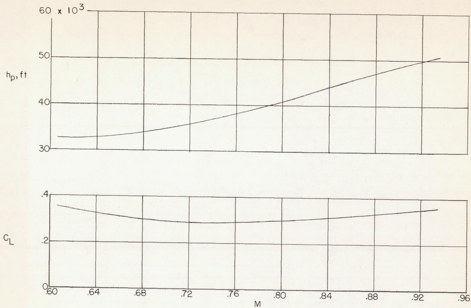
Figure 9.- Variation of C_L for (L/D)_{\max} and level flight altitude for (L/D)_{\max} with Mach number.
