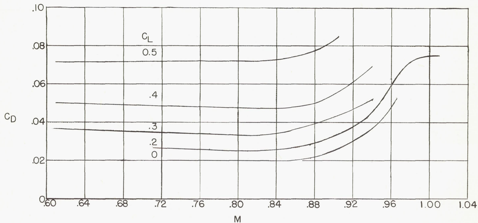
Figure 6.- Variation of drag coefficient with Mach number for several lift coefficients. ( 45^\circ configuration.)
