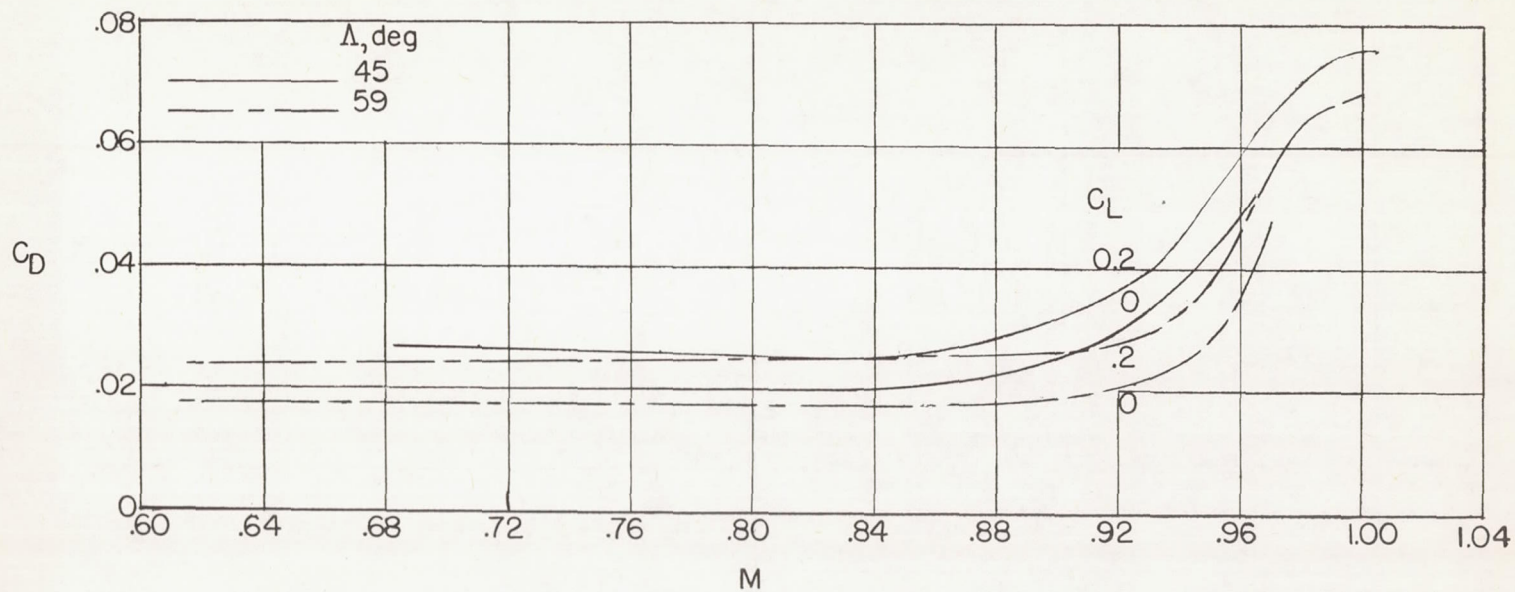
Figure 7.- Drag coefficient variation with Mach number for the 45^\circ and 59^\circ configurations.
