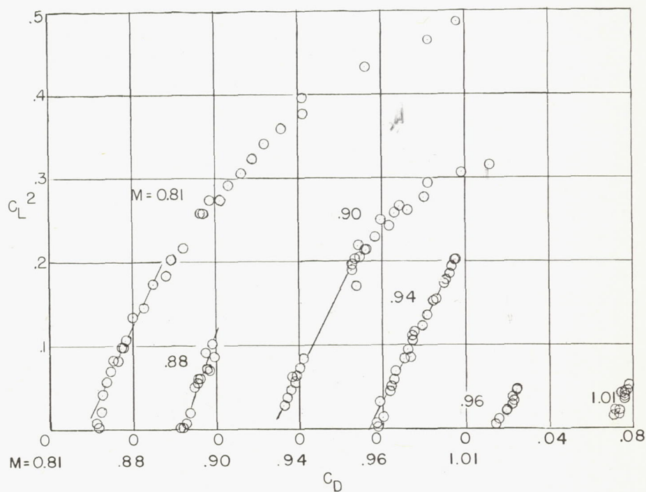
Figure 10.- Variation of drag coefficient with lift coefficient squared for several Mach numbers.
