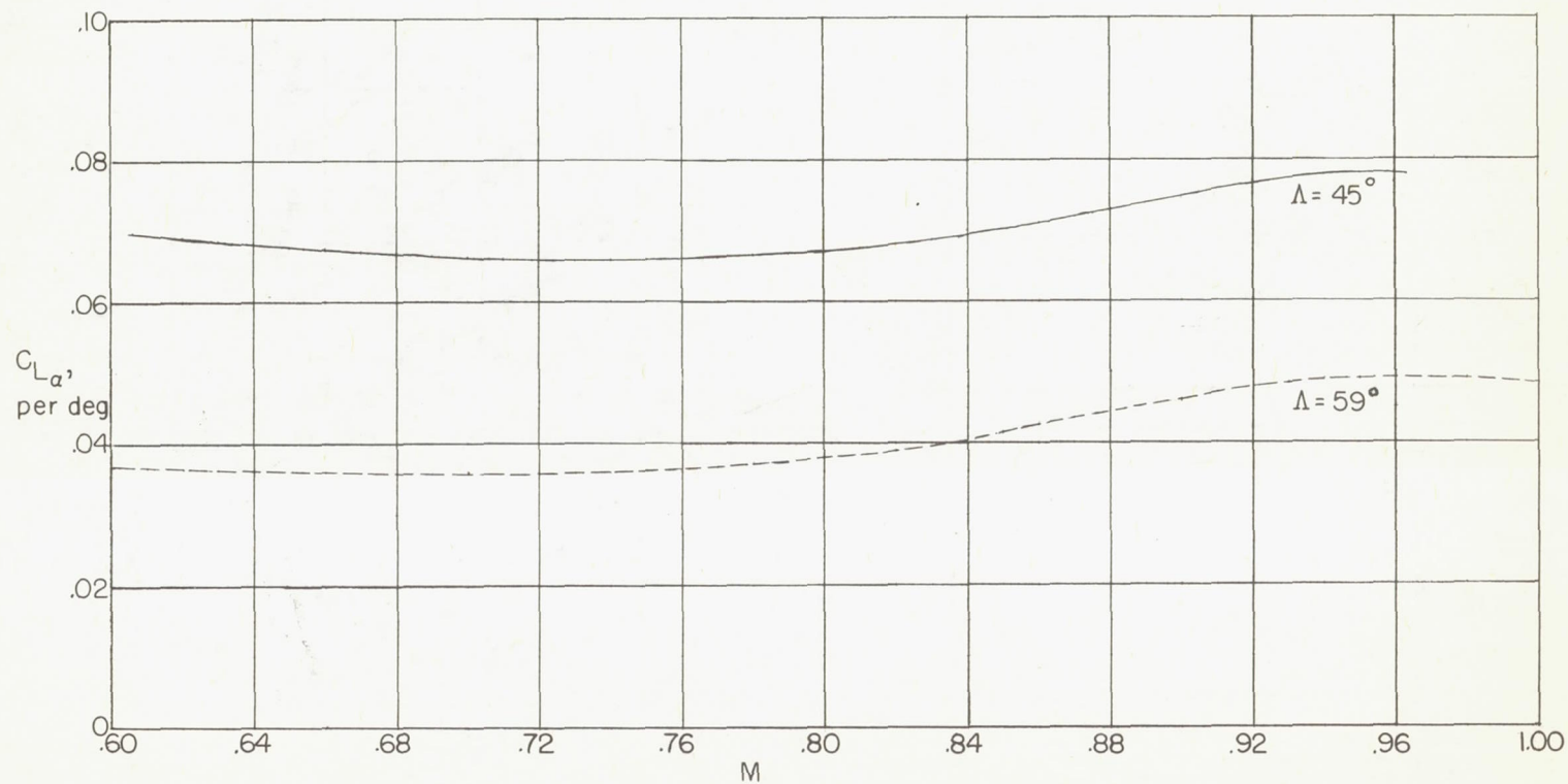
Figure 4.- Variation of lift-curve slope with Mach number.
