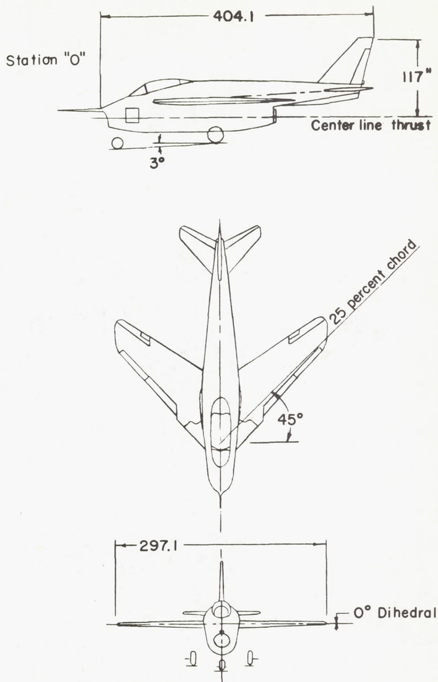
Figure 2.- Three-view drawing of Bell X-5 research airplane at 45^\circ sweepback.
