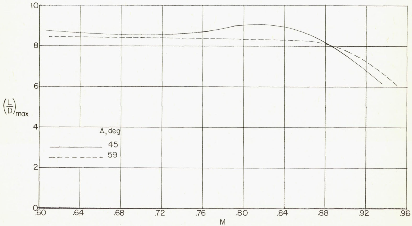
Figure 8.- Variation of (L/D)_{\max} with Mach number.
