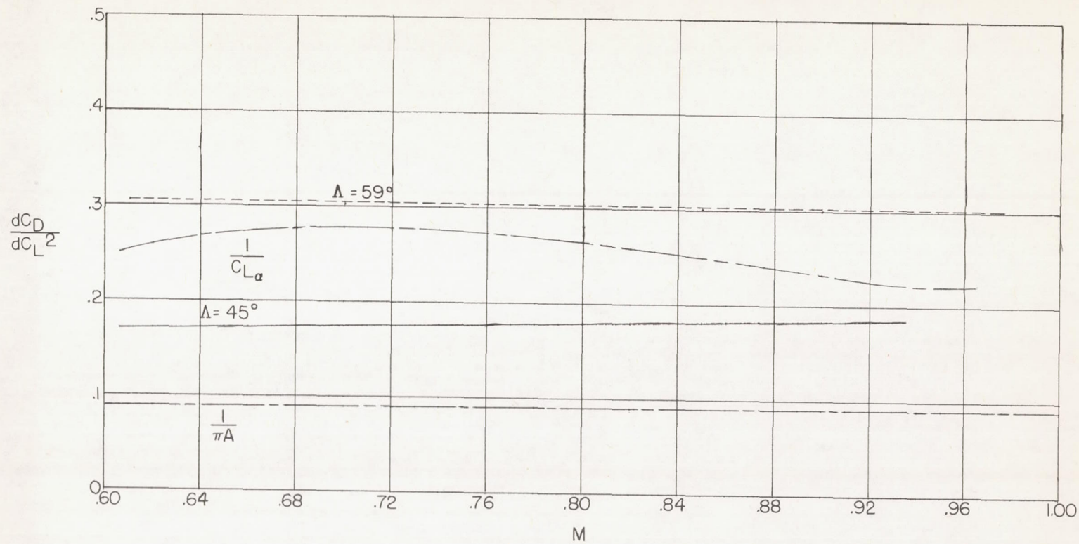
Figure 11.- Variation of drag-due-to-lift factor with Mach number.
