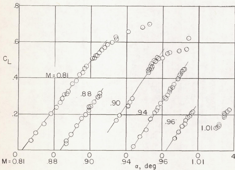
Figure 3.- Variation of lift coefficient with angle of attack for several Mach numbers.
