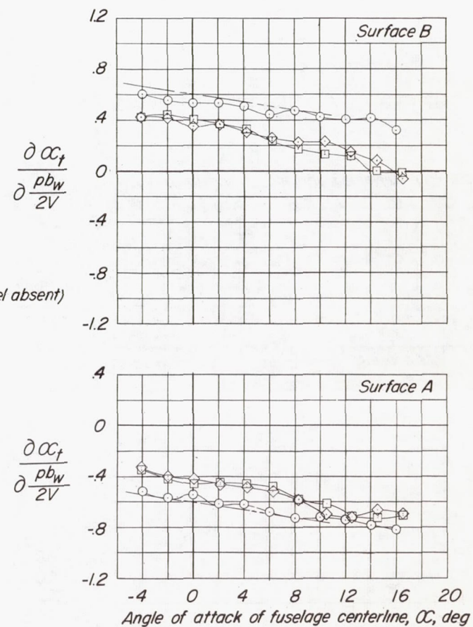
(h) Spanwise station, y = 10 inches.
