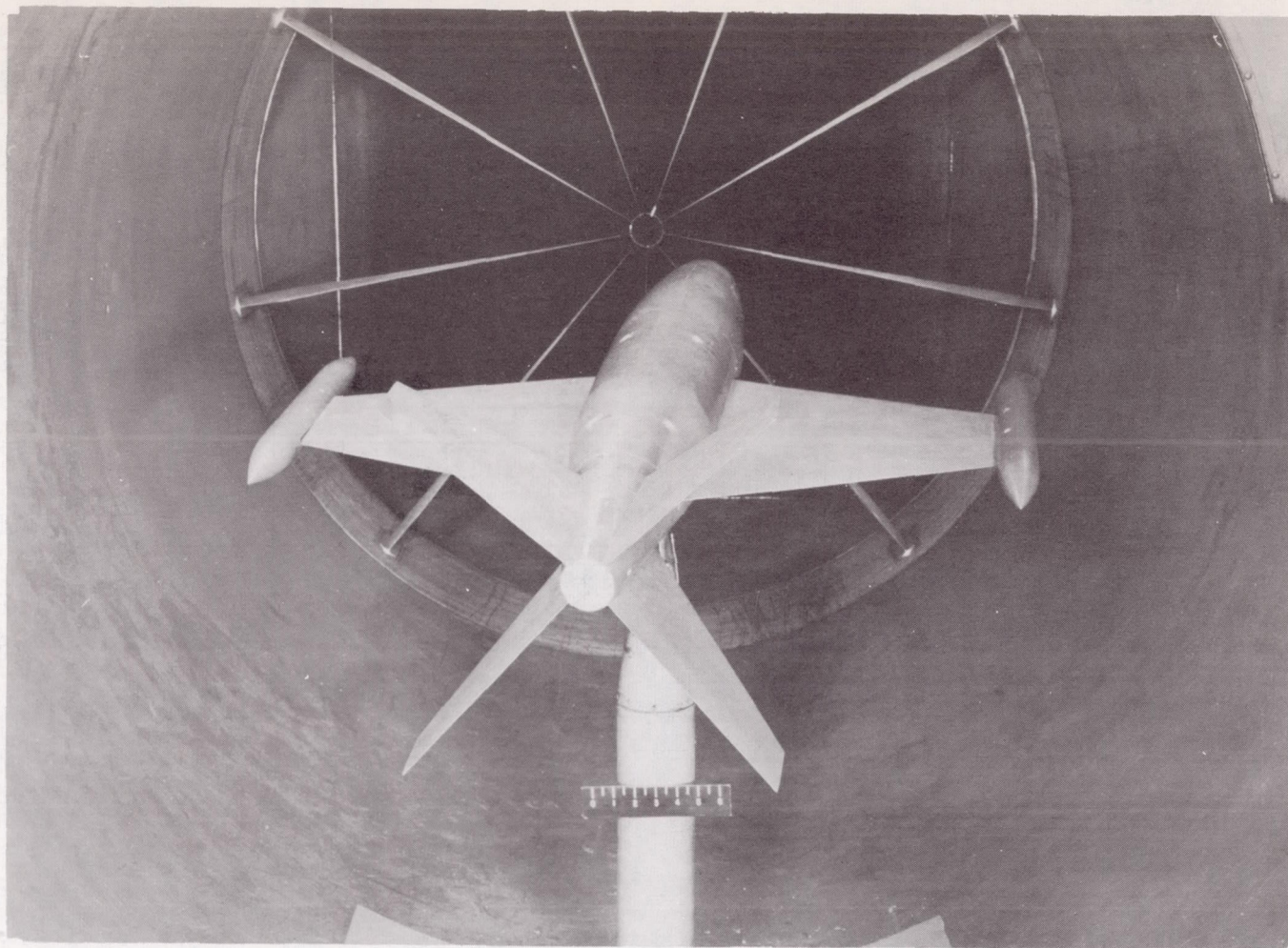
L-75328 Figure 4.- Rear view of the X-tail model shown at a slight angle of side-slip in the 6-foot-diameter rolling-flow test section of the Langley stability tunnel.
