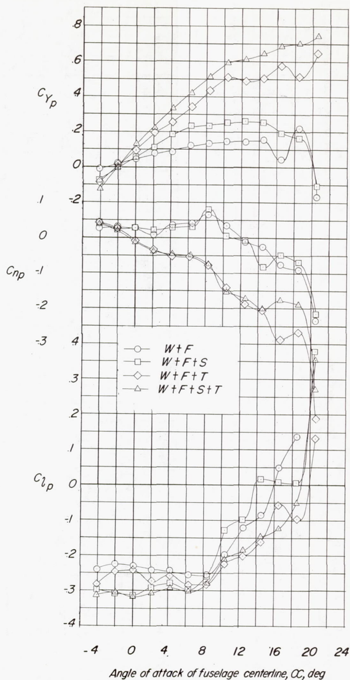
Figure 7.- Variation with angle of attack of C_{Yp} , C_{np} , and C_{lp} for the wing-fuselage combination with and without the wing-tip stores and X-tail.
