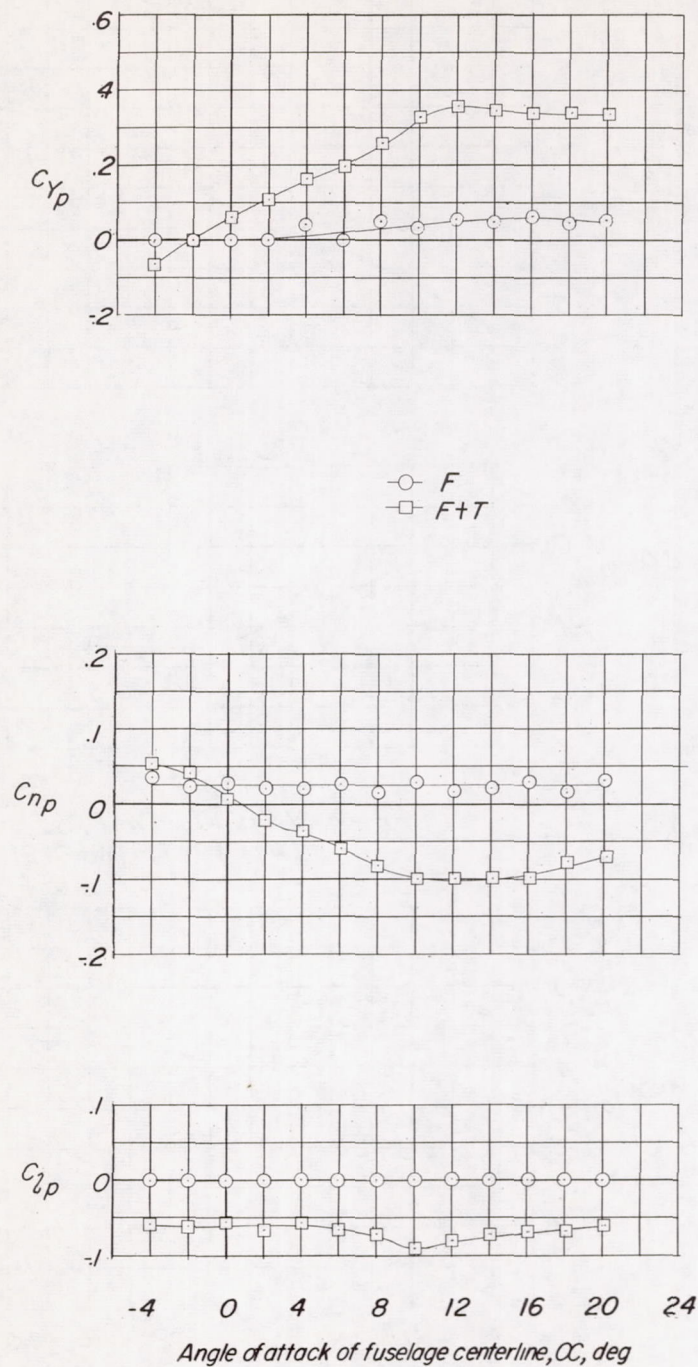
Figure 8.- Variation with angle of attack of C_{Yp} , C_{np} , and C_{lp} for the fuselage alone and with the X-tail.
