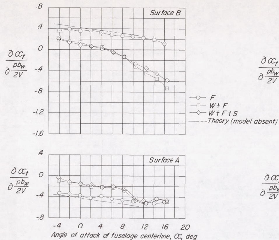
(e) Spanwise station, y = 7 inches.
