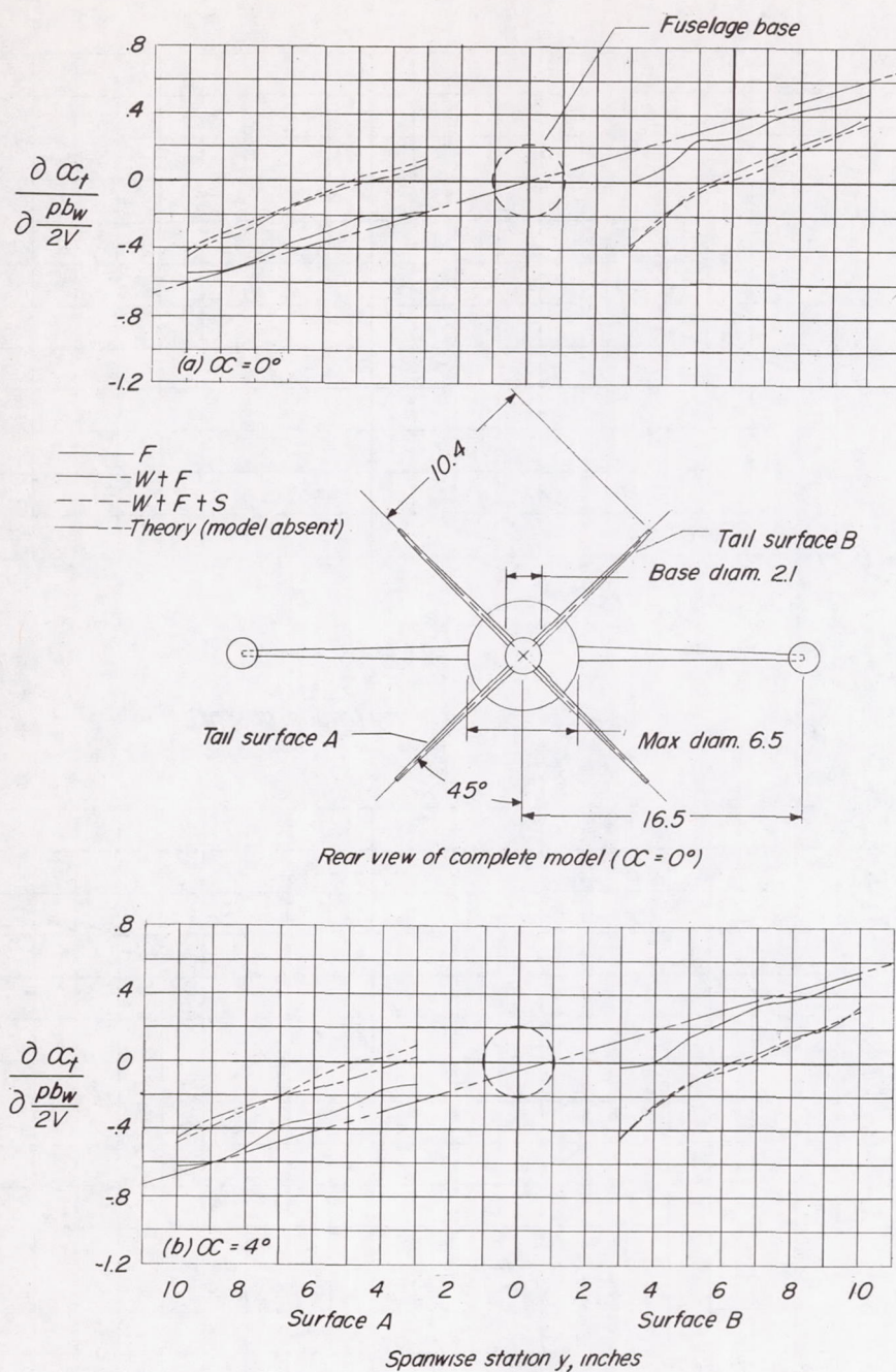
Figure 11.- Spanwise distributions of the airstream angularity derivative at the tail \frac{\partial \alpha_t}{\partial \frac{pb_w}{2V}} for tail surfaces A and B at several angles of attack of the model.
