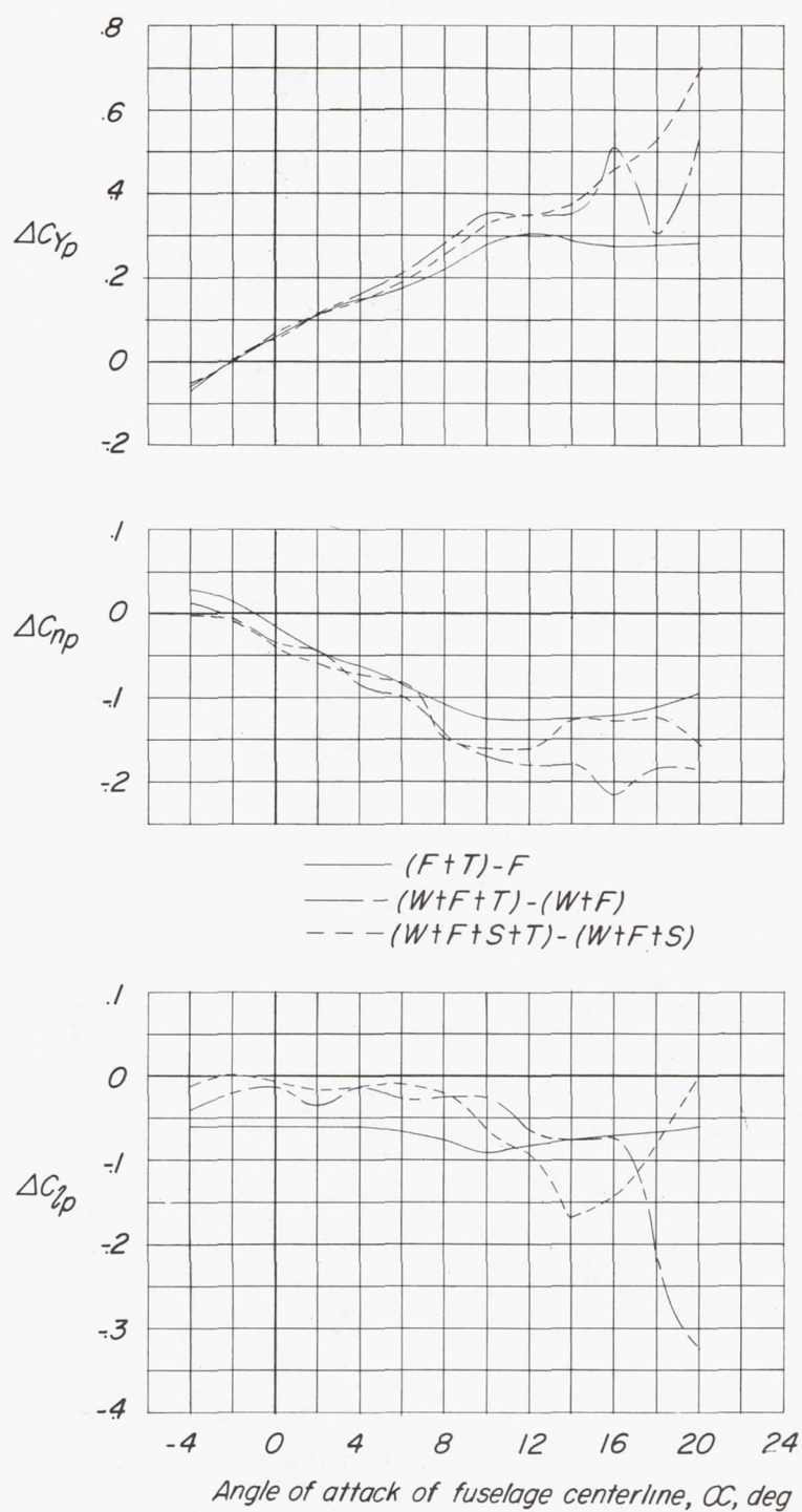
Figure 9.- Variation with angle of attack of the x-tail contribution to the rolling stability derivatives.
