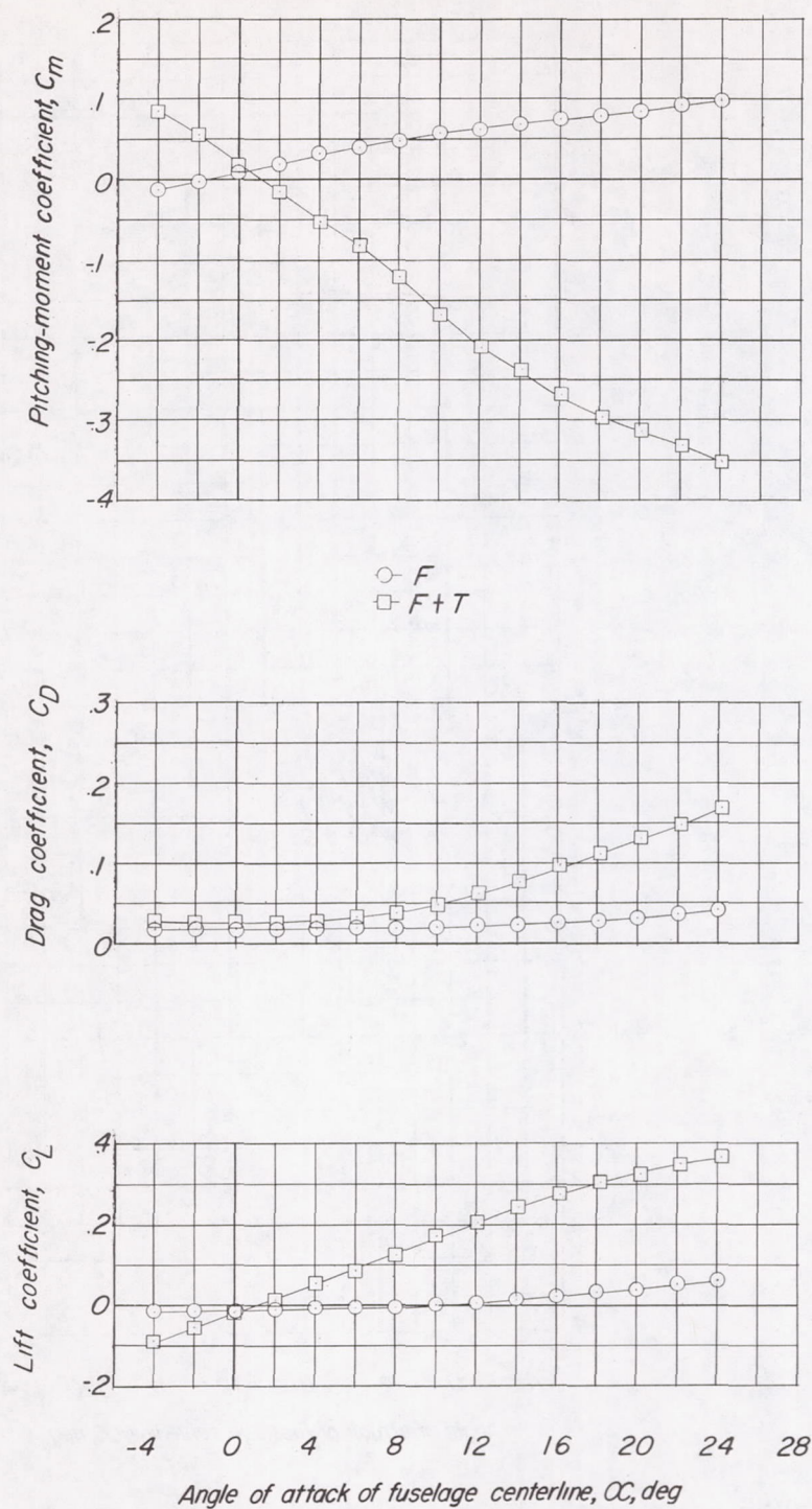
Figure 6.- The lift, drag, and pitching-moment characteristics for the fuselage alone and with the X-tail.
