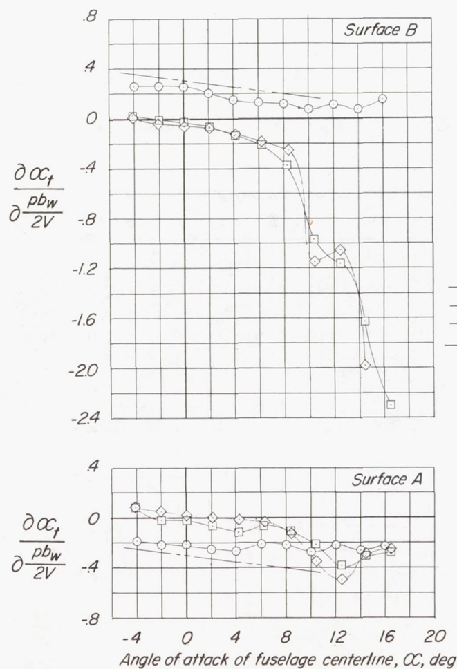
(c) Spanwise station, y = 5 inches.
