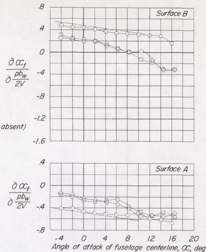
(f) Spanwise station, y = 8 inches.
