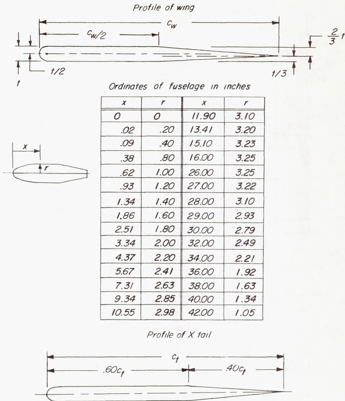
Figure 3.- Details of the wing and tail profiles and a table of ordinates for the fuselage.
