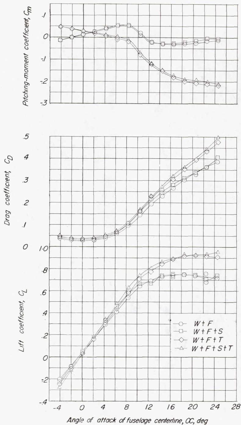
Figure 5.- The lift, drag, and pitching-moment characteristics for the wing-fuselage configuration with and without the wing-tip stores and x-tail.
