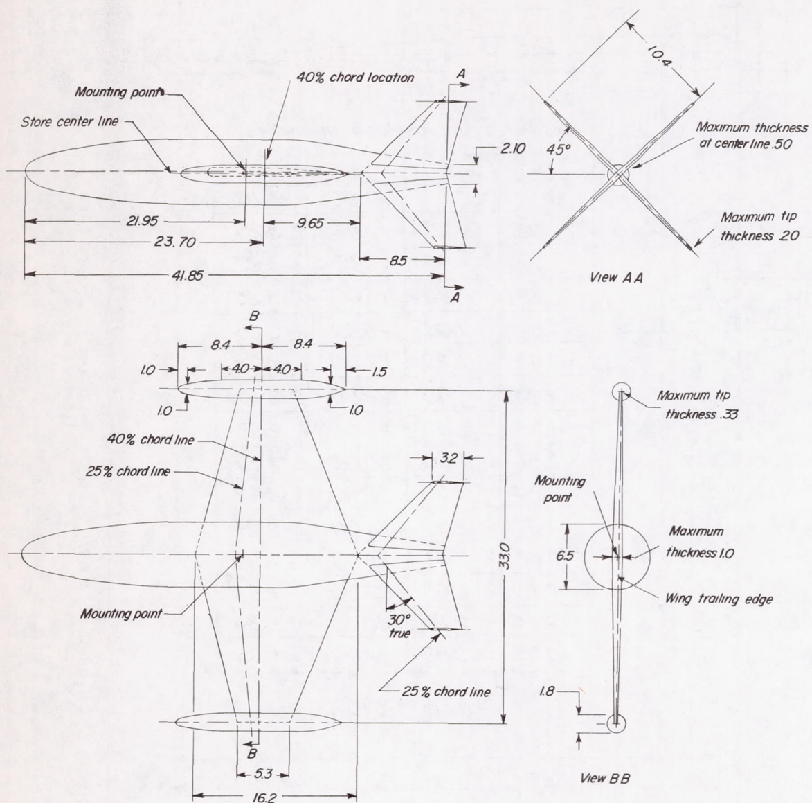
Figure 2.- A drawing of the complete X-tail model. All dimensions are in inches.
