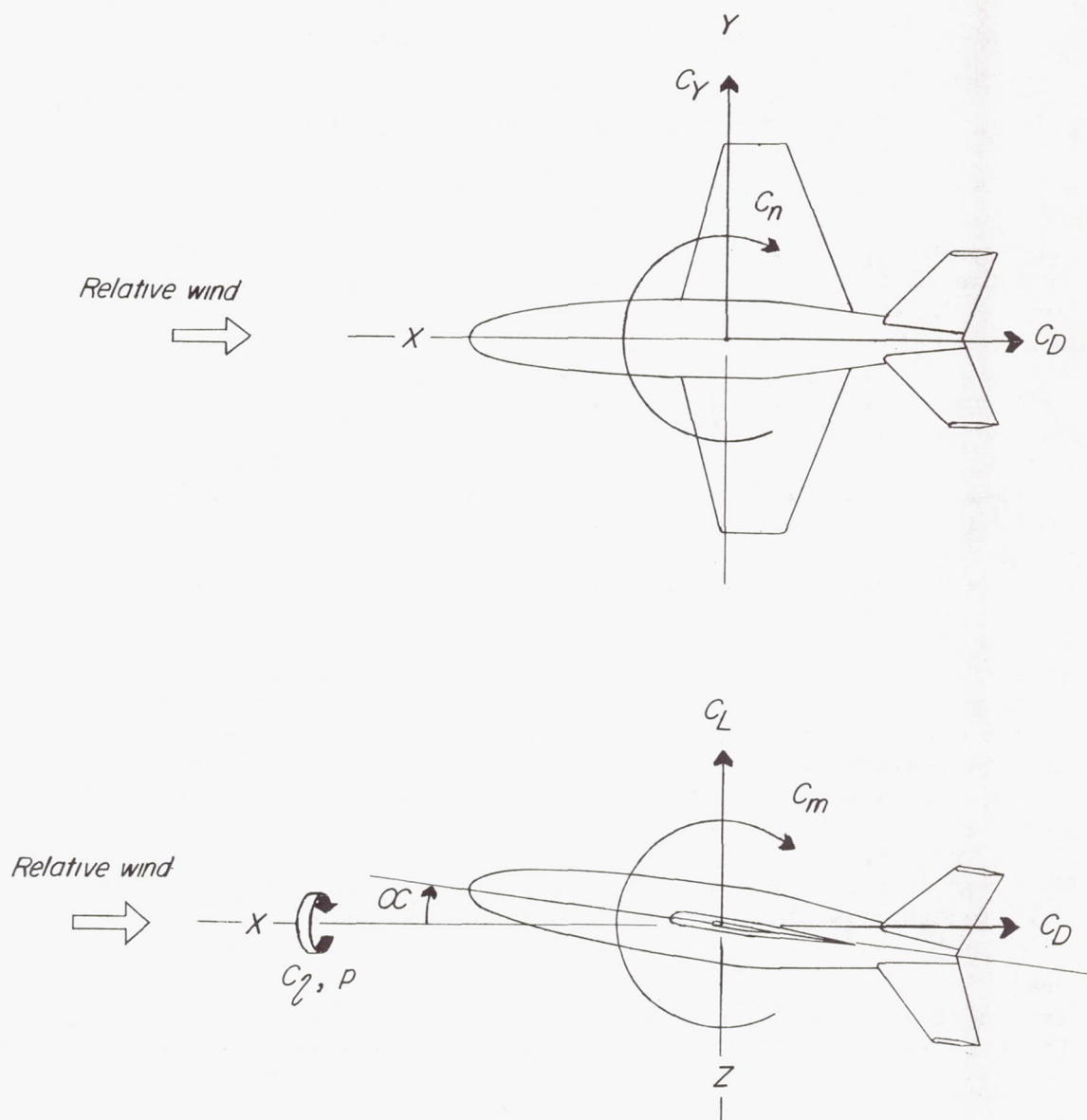
Figure 1.- System of axes used. Arrows indicate positive directions.
