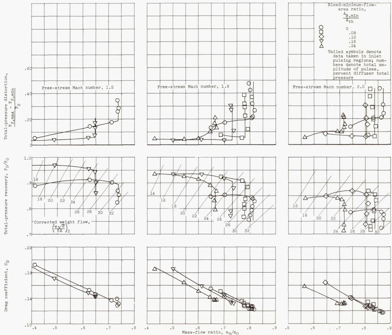
Figure 4. - Continued. Inlet performance characteristics of forward ram scoop having 14° ramp without side fairings (configuration A-1).
