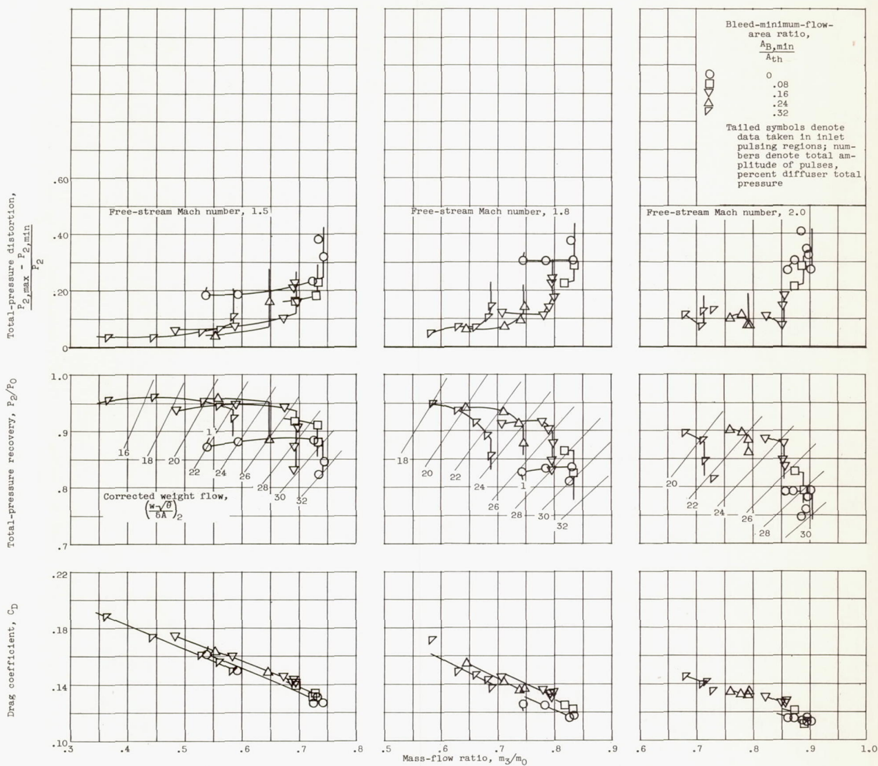
Figure 7. - Concluded. Inlet performance characteristics of aft ram scoop having 14° ramp with side fairings (configuration B-2).
