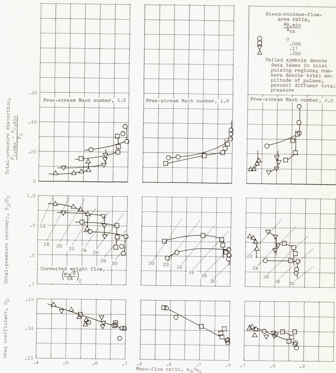
Figure 9. - Concluded. Inlet performance characteristics of forward ram scoop having 18° ramp with side fairings (configuration C-2).
