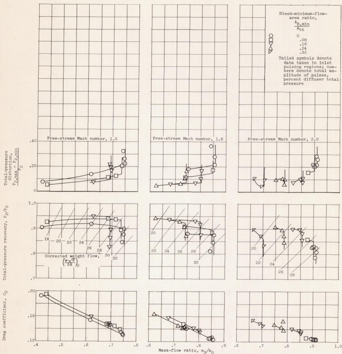
Figure 7. - Continued. Inlet performance characteristics of aft ram scoop having 14^\circ ramp with side fairings (configuration B-2).
