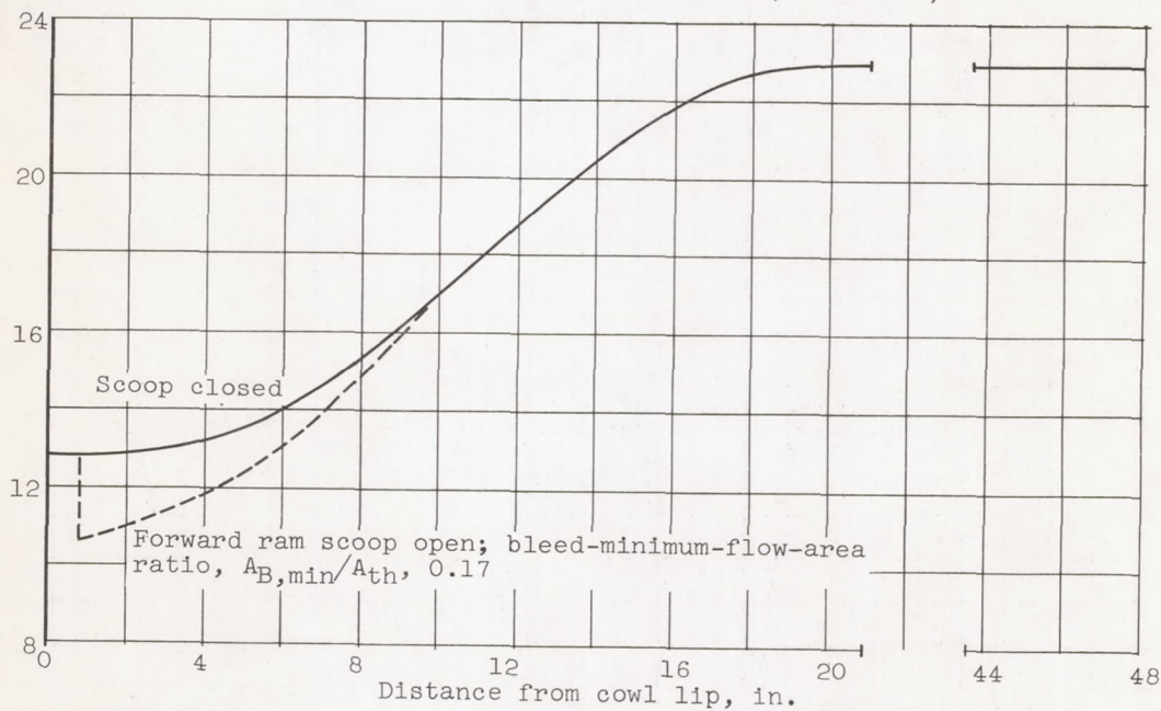
(b) 18° Ramp (inlet hydraulic diam., 3.35 in.).
