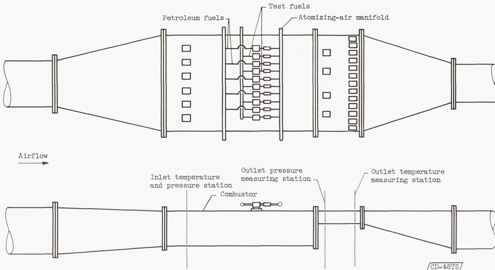
Figure 1. - Schematic diagram of test installation.
