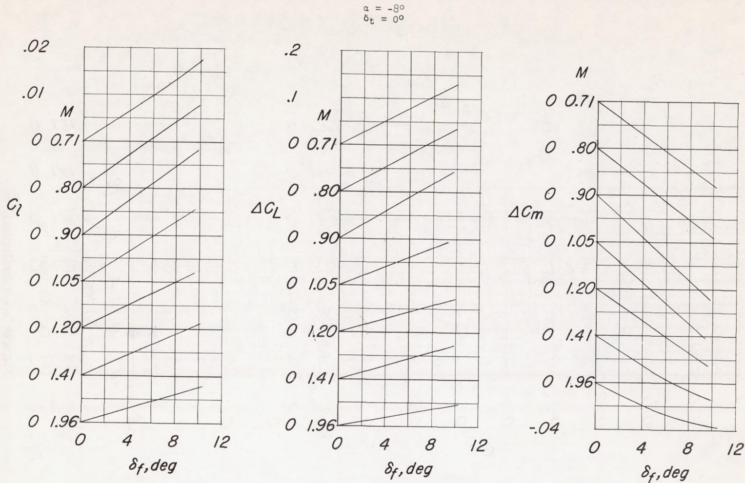
Figure 6.- Variation with flap deflection of rolling moment and increment in lift and pitching-moment coefficients due to flap deflection at various Mach numbers for three angles of attack. \delta_t = 0^\circ .
