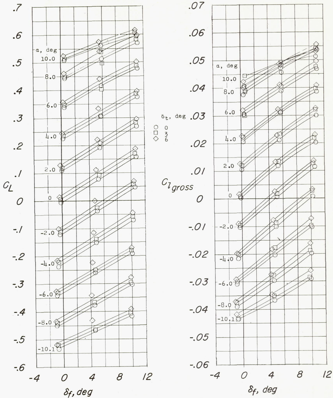
(a) C_L and C_l against \delta_f .
