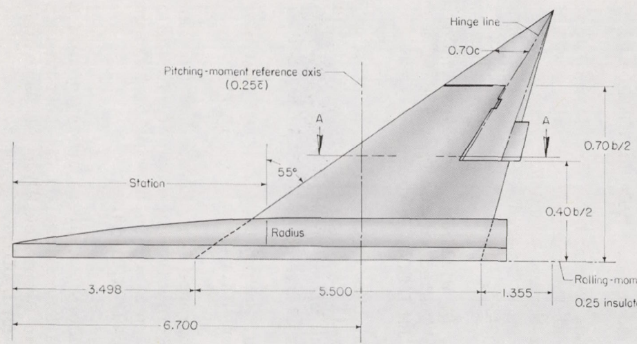
Figure 1.- Details of semispan-wing-fuselage combination. Aspect ratio, 3.5; mean aerodynamic chord, 3.667 inches; semispan-wing area, 13.20 square inches. (All dimensions are in inches unless otherwise indicated.)
