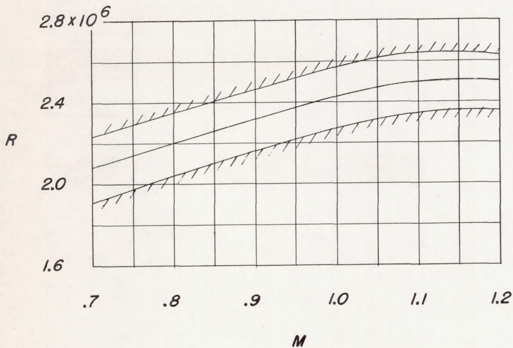
(b) Average test Reynolds number based on wing \bar{c} .
