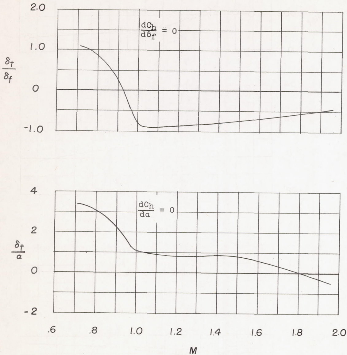
Figure 10.- Ratios of \delta_t/\delta_f and \delta_t/\alpha necessary to balance aerodynamically the control surface through the Mach number range.
