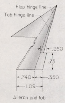
Figure 1.- Details of semispan-wing-fuselage combination. Aspect ratio, 3.5; mean aerodynamic chord, 3.667 inches; semispan-wing area, 13.20 square inches. (All dimensions are in inches unless otherwise indicated.)
