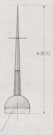
Figure 1.- Details of semispan-wing-fuselage combination. Aspect ratio, 3.5; mean aerodynamic chord, 3.667 inches; semispan-wing area, 13.20 square inches. (All dimensions are in inches unless otherwise indicated.)
