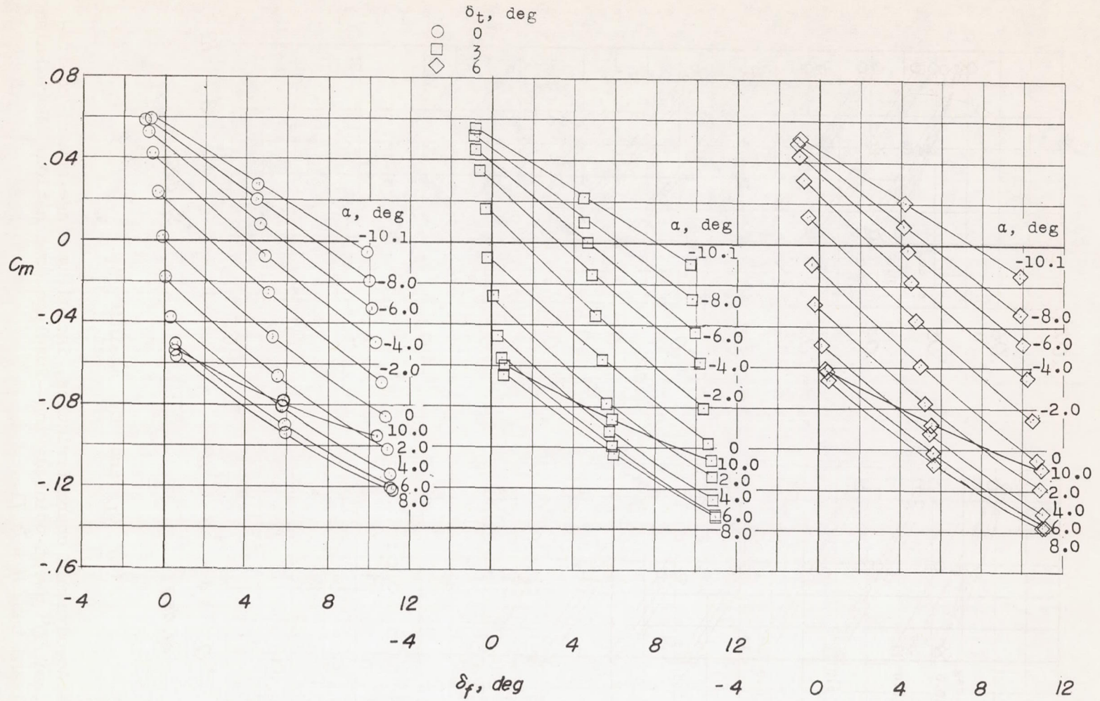
(b) C_m against \delta_f .
