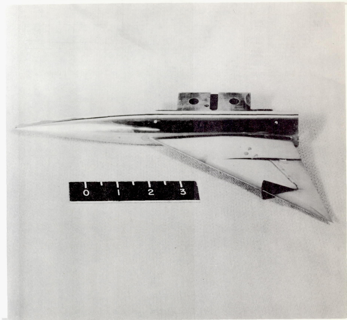
Figure 2.- Wing-fuselage model with fence and horn-balanced control without tab.
