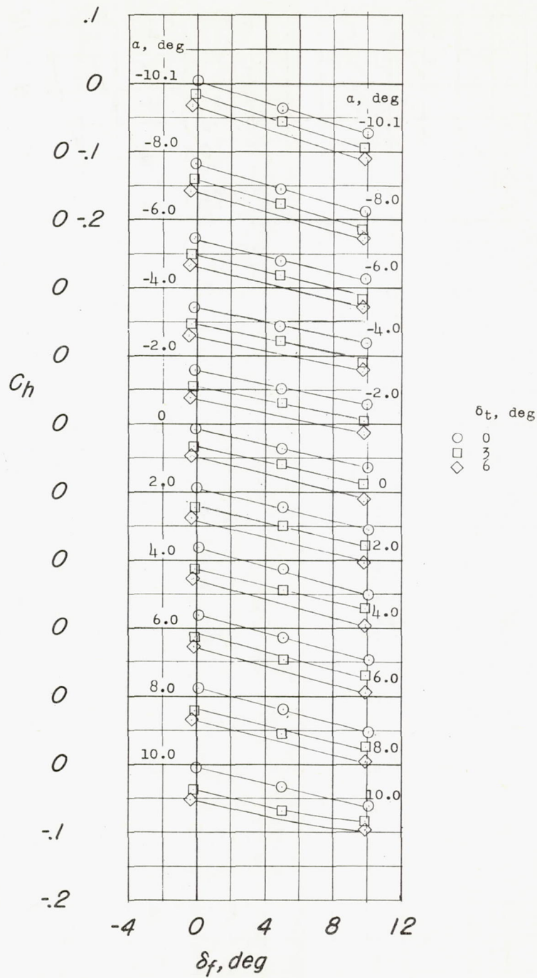
(b) C_h against \delta_f .
