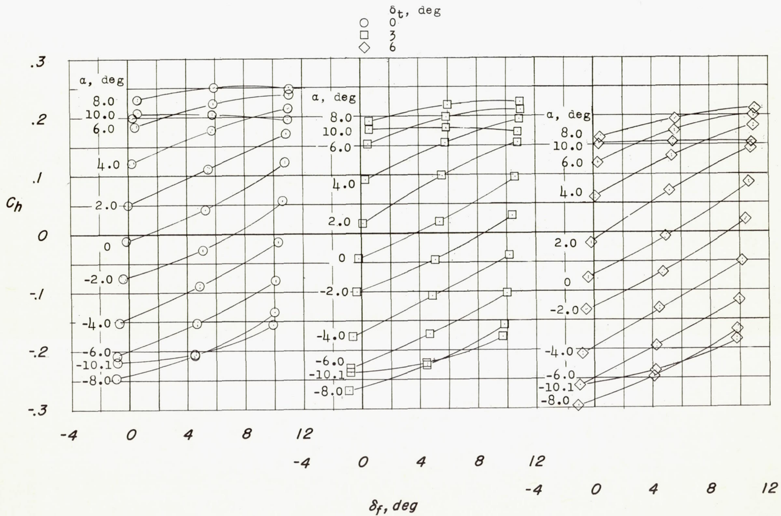
(c) C_h against \delta_f .
