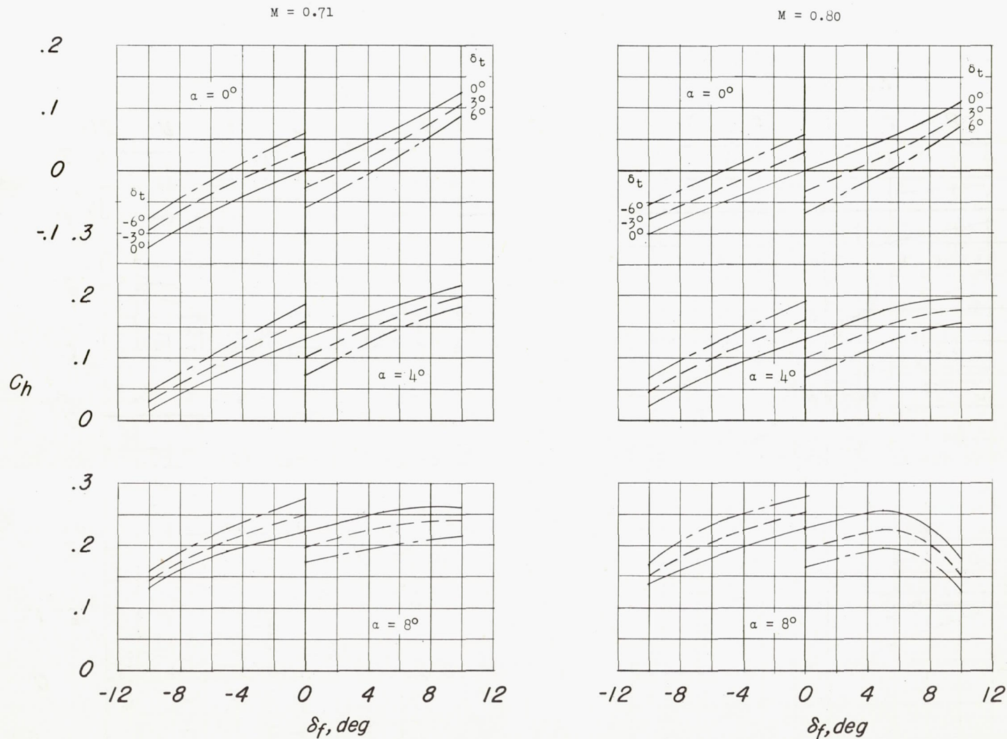
Figure 7.- Variation of hinge-moment coefficient with flap deflection for several tab deflections and angles of attack.
