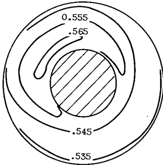
(a) Two-shock ramp; scoop-to-throat-height ratio, 0; critical operation.
