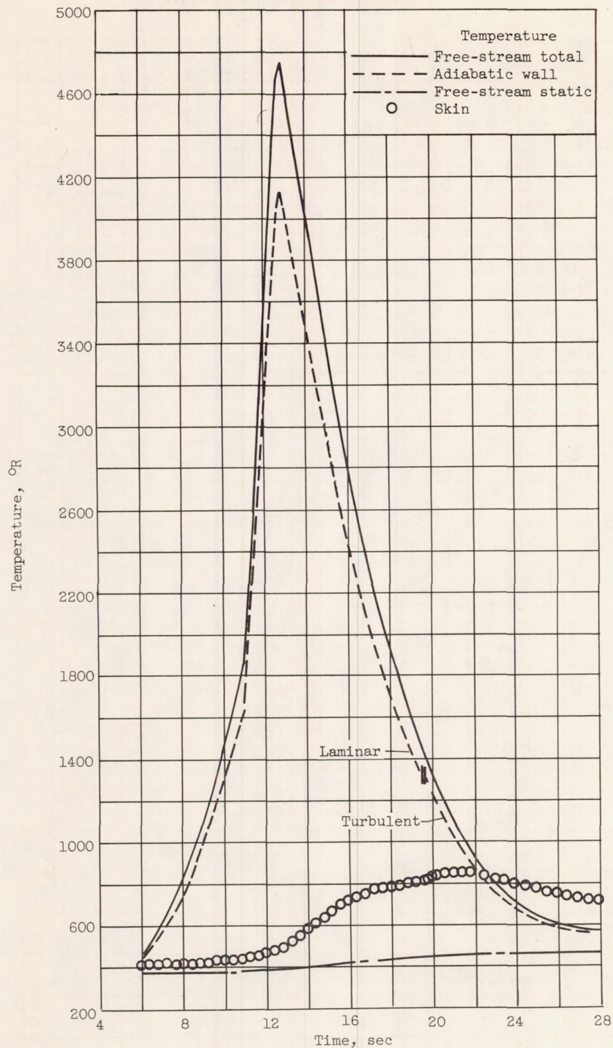
Figure 12. - Concluded. Variation of temperatures with time.
