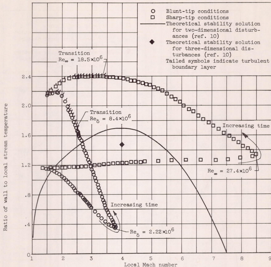
Figure 15. - Continued. Variation of ratio of wall to local stream temperature with Mach number. Re_{\infty} , Reynolds number for sharp-tip conditions; Re_{\delta} , Reynolds number for blunt-tip conditions.
