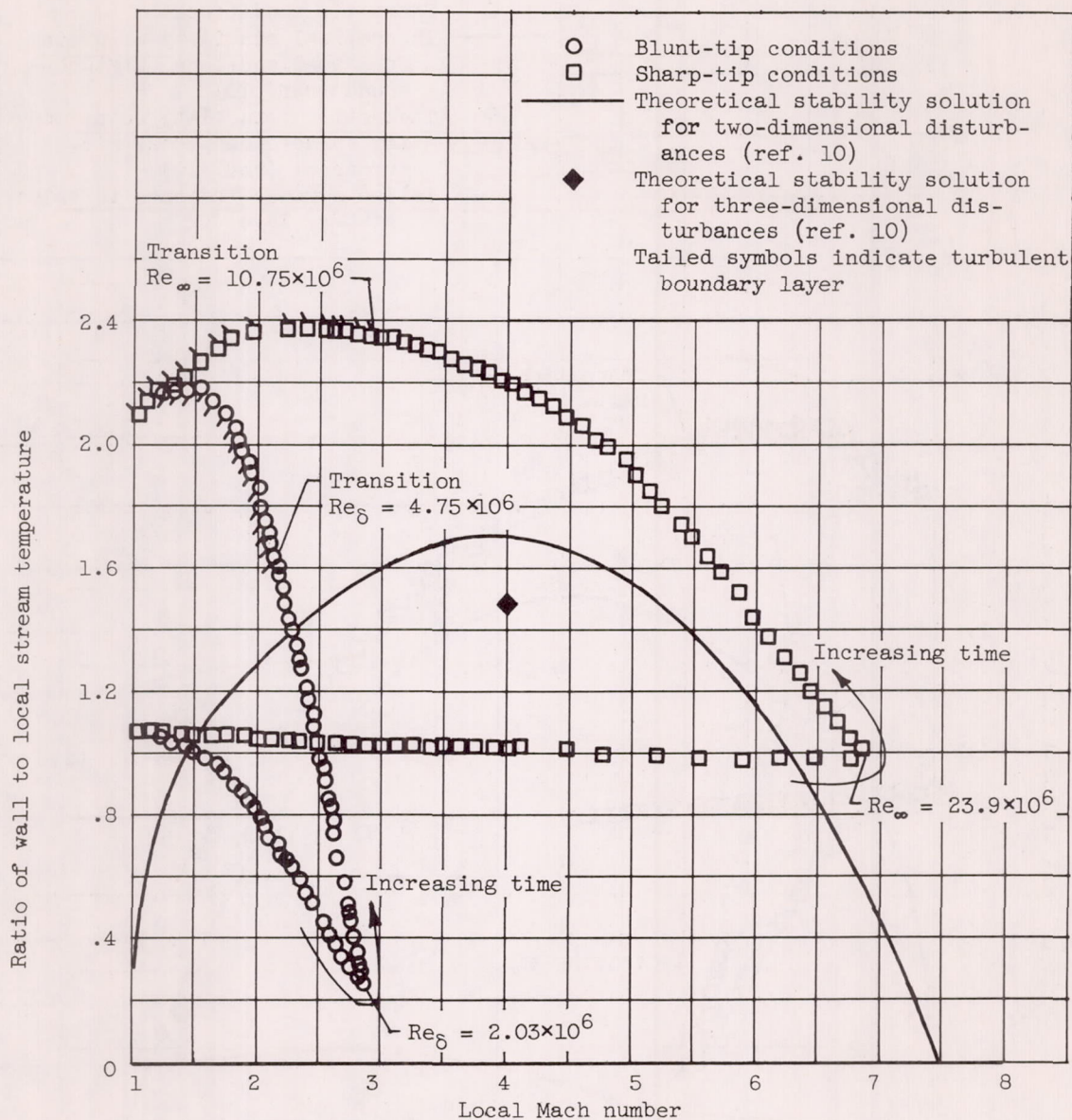
(a) Station 9.75.
