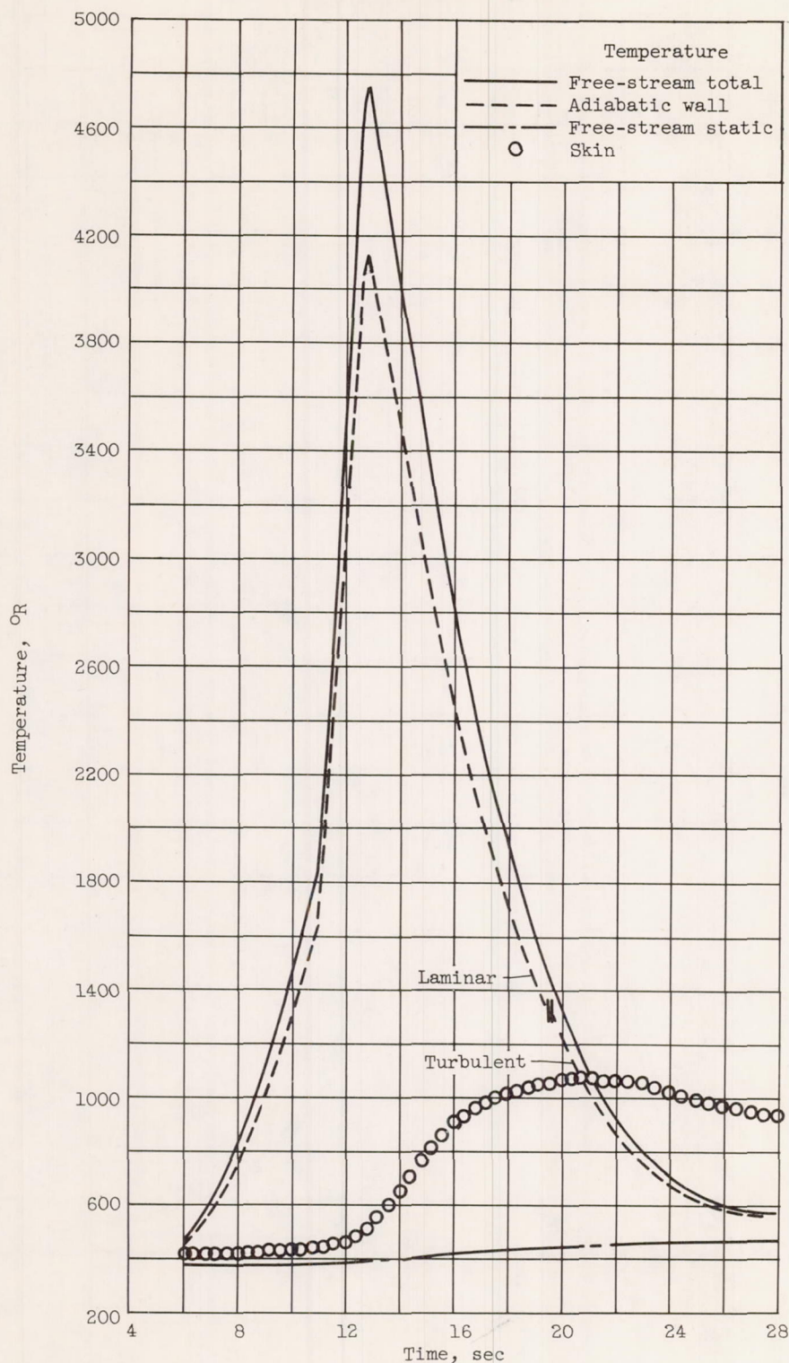
Figure 12. - Continued. Variation of temperatures with time.
