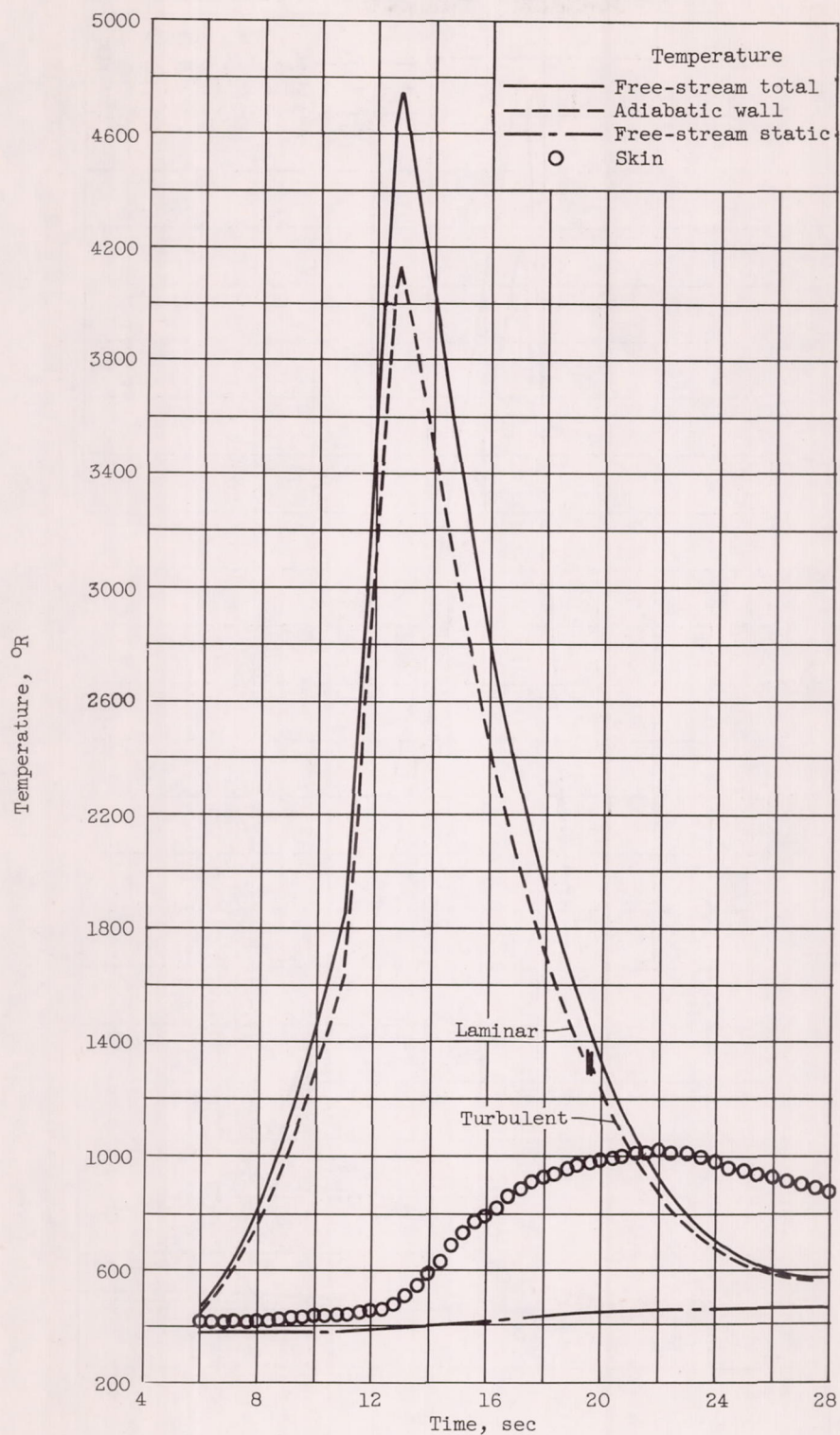
Figure 12. - Continued. Variation of temperatures with time.
