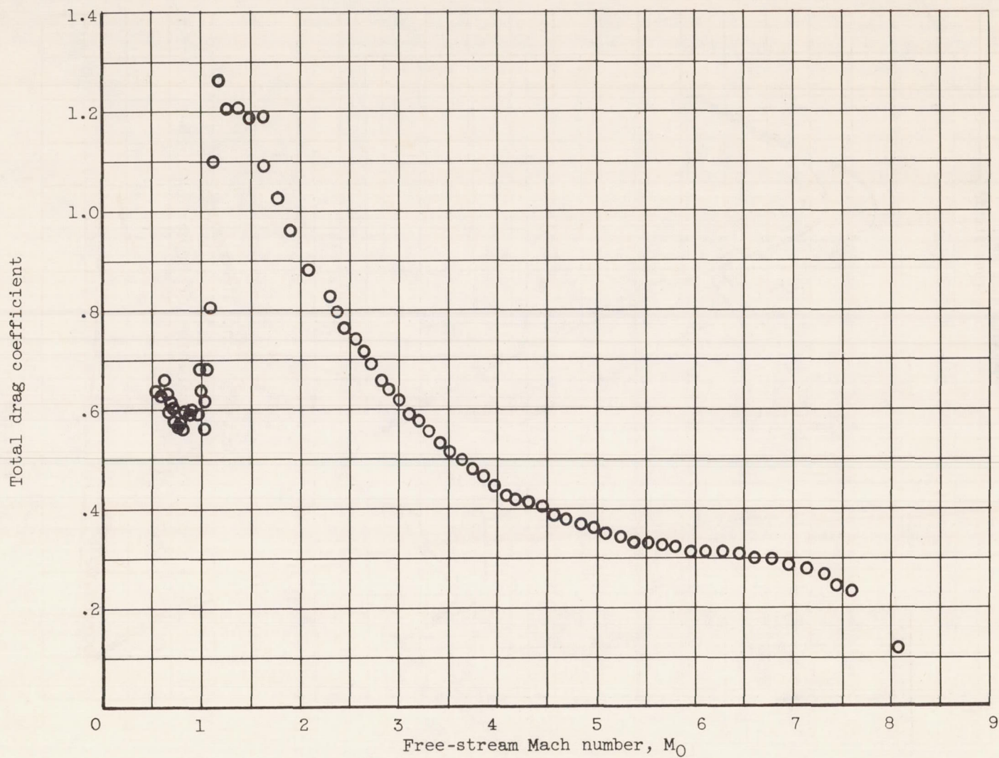
Figure 11. - Variation of total drag coefficient for sustainer stage with Mach number. Reference area, 0.196 square foot.
