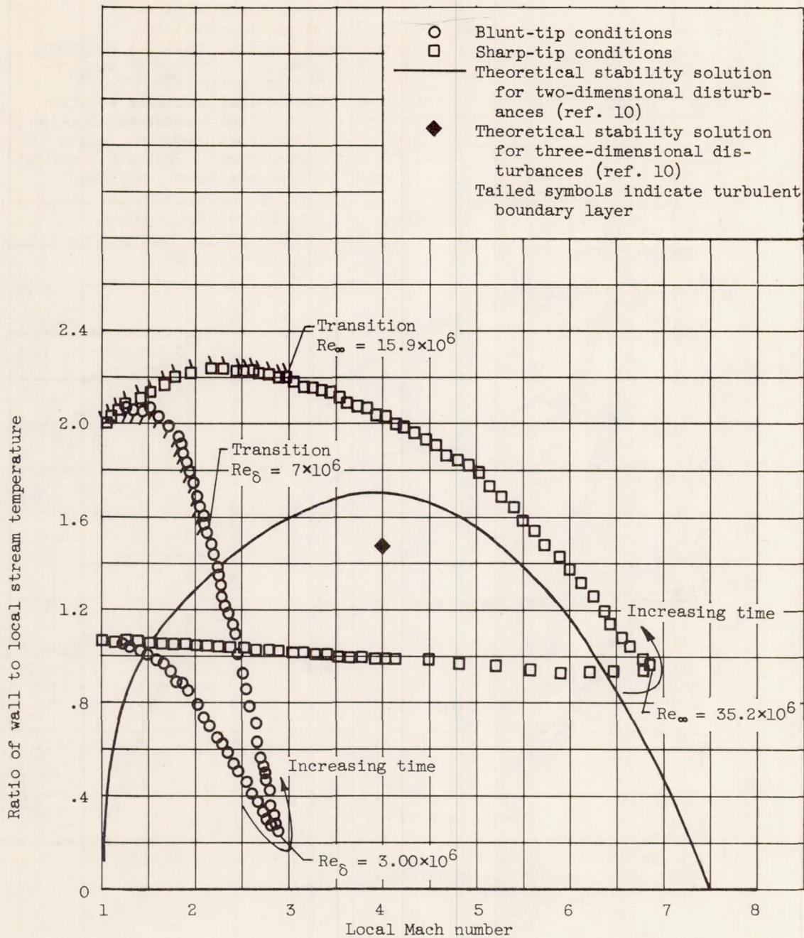
(b) Station 14.45.
