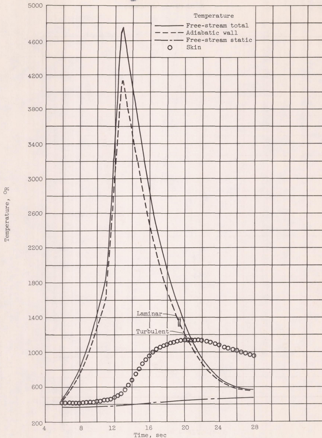
(a) Station 9.75.
