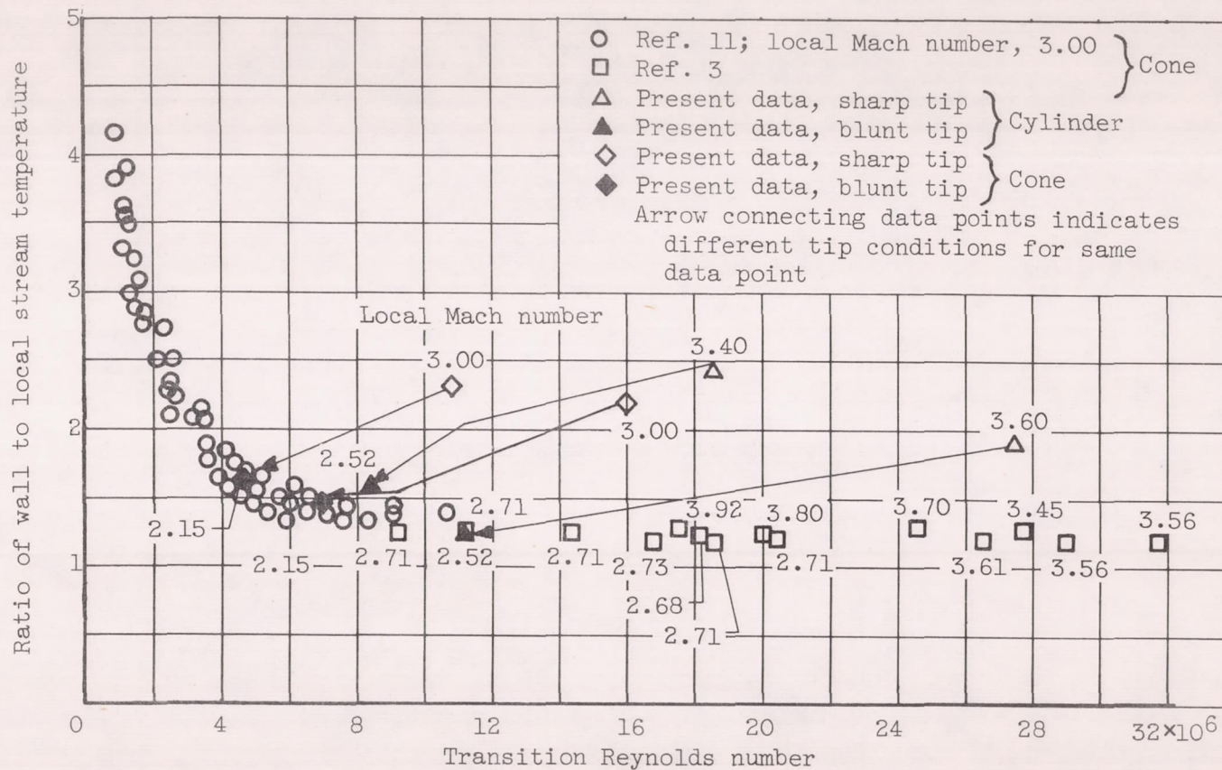
Figure 16. - Comparison of present data with previously obtained transition data for sharp-tipped cones.
