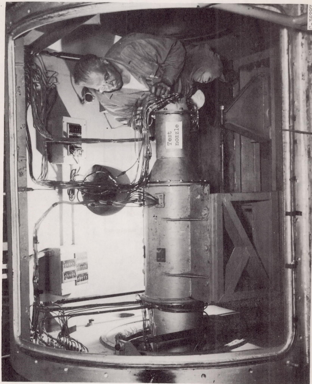
Figure 4. - Installation of nozzle in test chamber.
