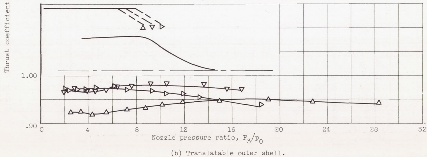
Figure 13. - Effect of varying throat area of contoured-plug nozzle with simulated iris and translatable outer shells.
