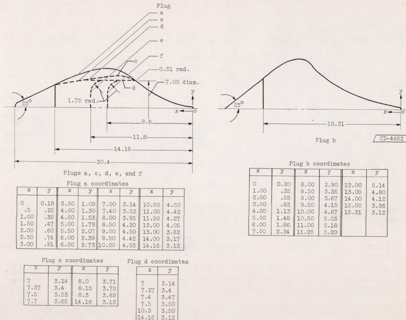
Figure 1. - Plug configurations (all dimensions in inches).
