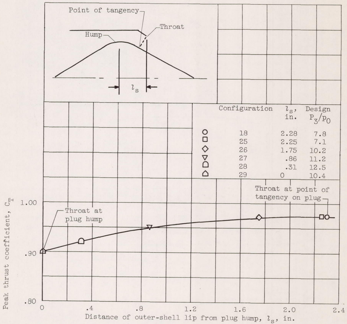
Figure 6. - Effect of outer-shell exit position on peak thrust coefficient.
