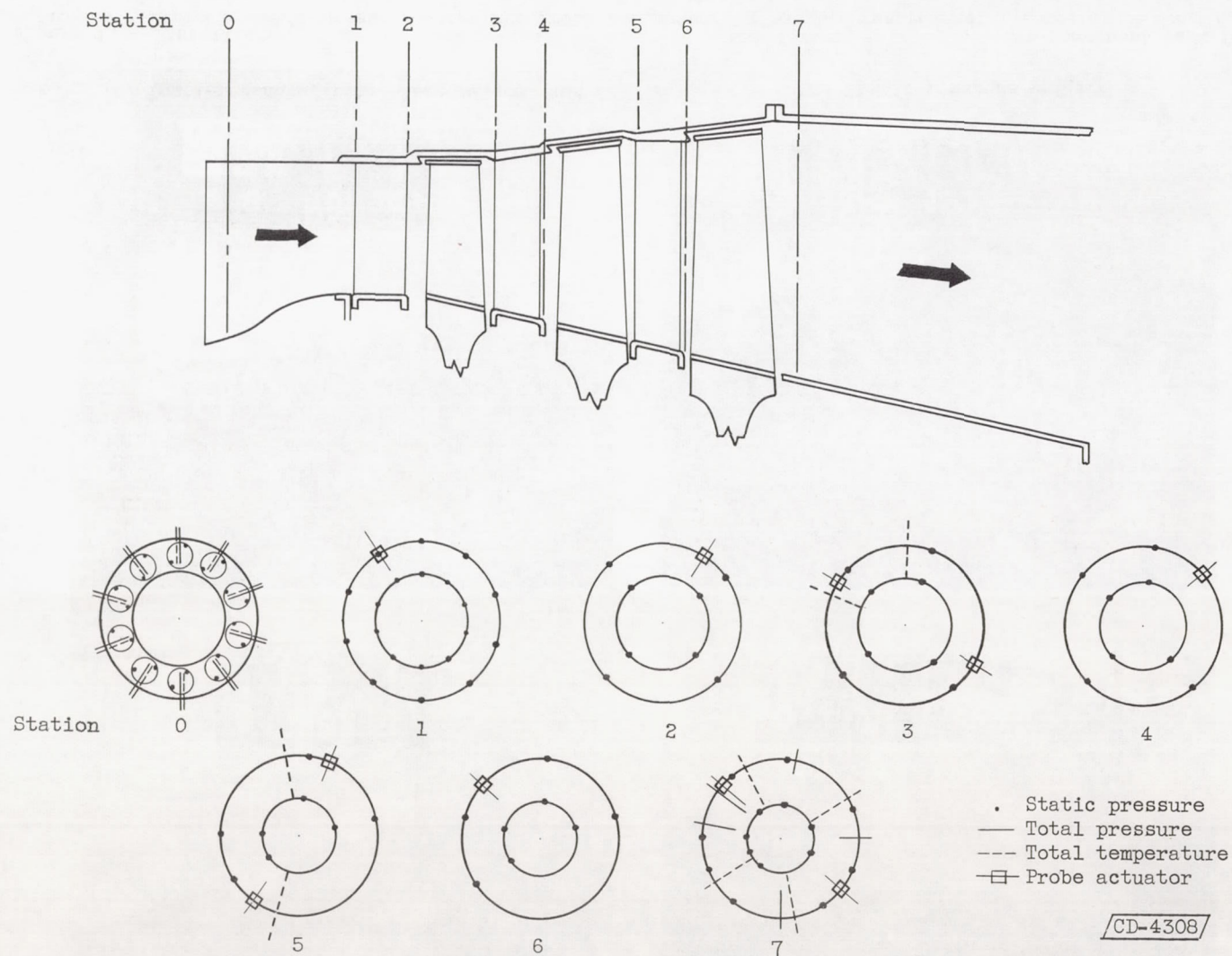
Figure 2. - Schematic diagram of J71-87 turbine showing instrumentation.
