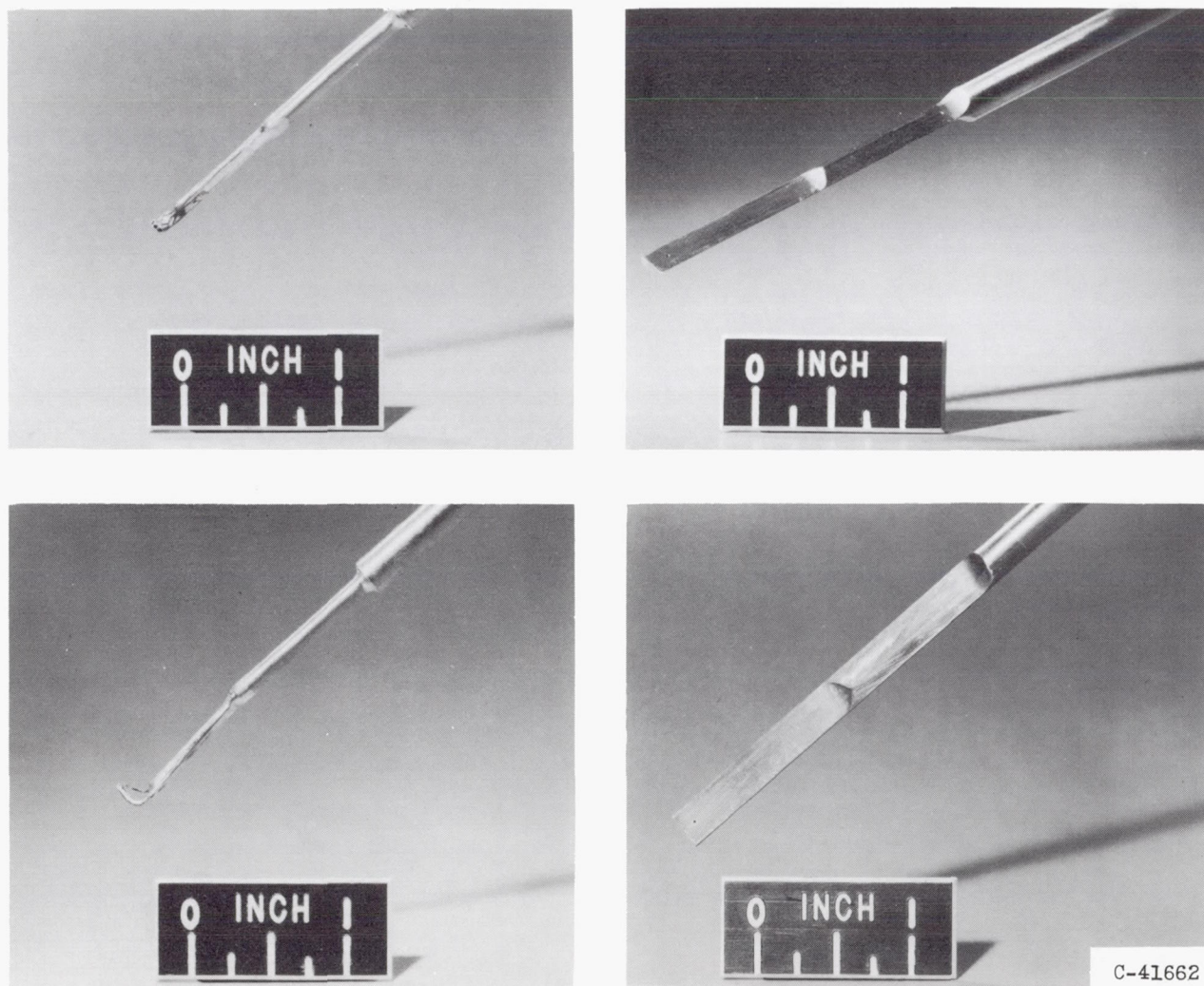
(a) Total-pressure, total-temperature, and angle probe.
