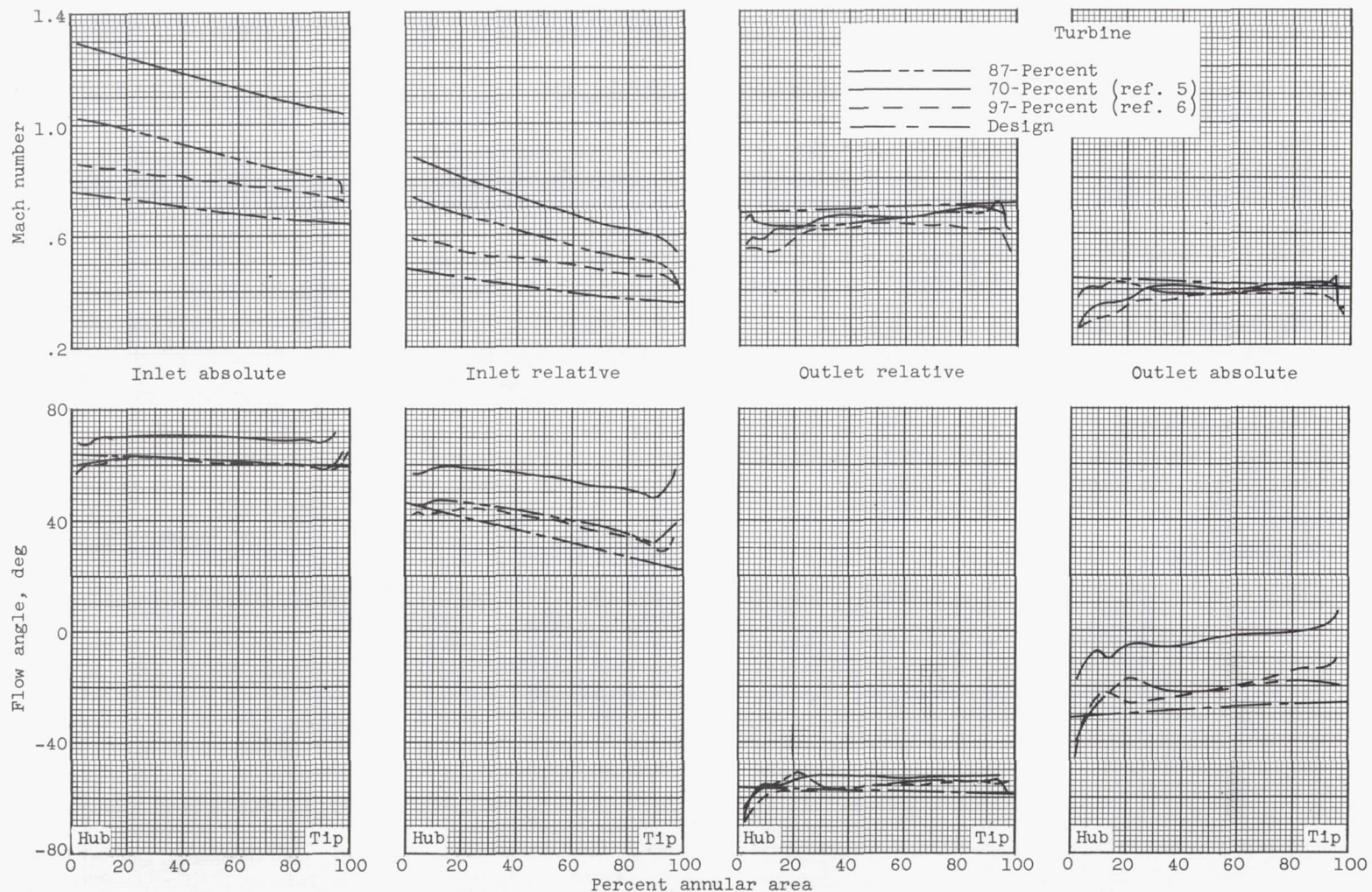
(a) First rotor.
