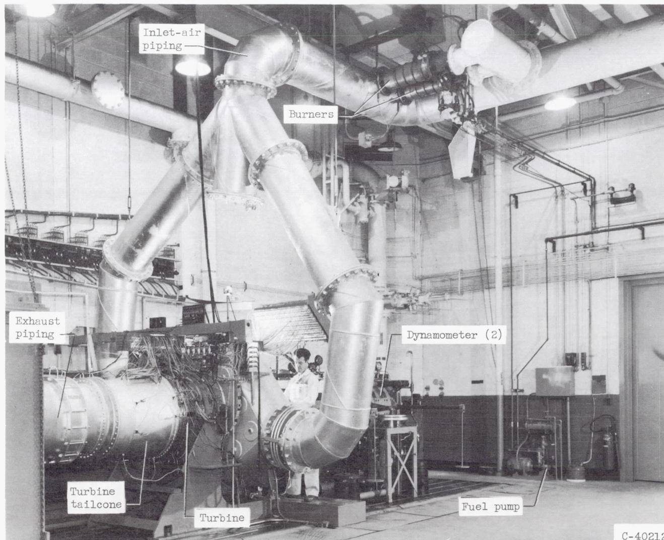
Figure 1. - Installation of J71-87 experimental three-stage turbine in full-scale turbine-component test facility.
