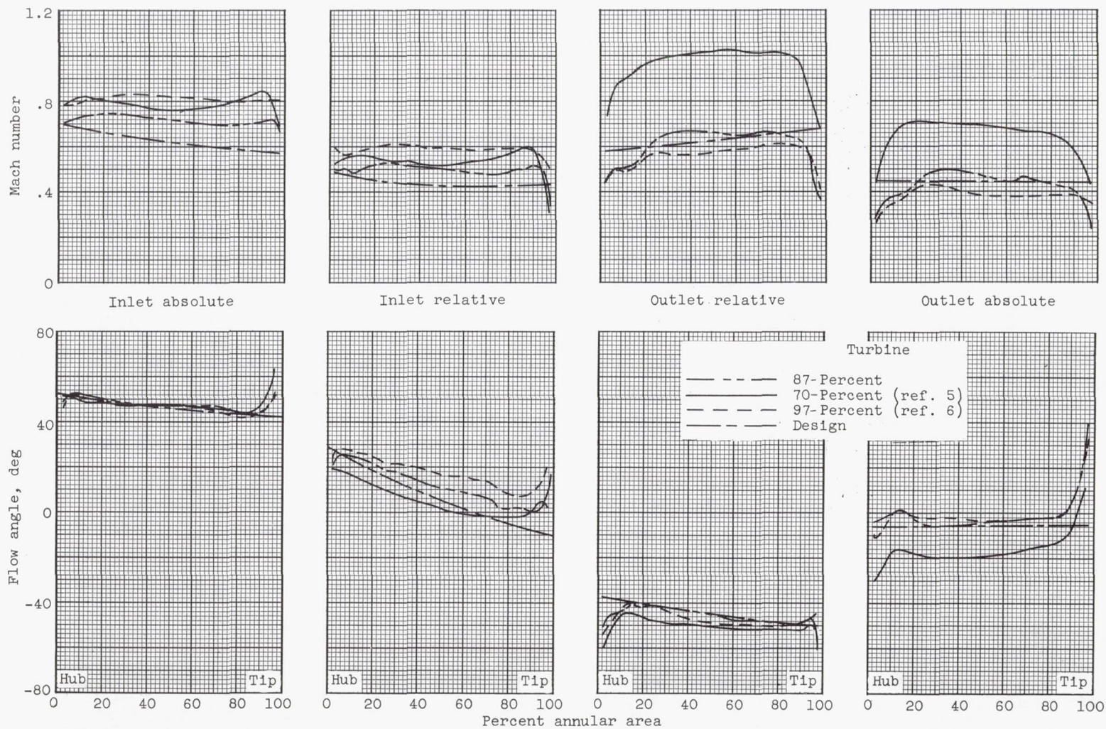
(c) Third rotor.
