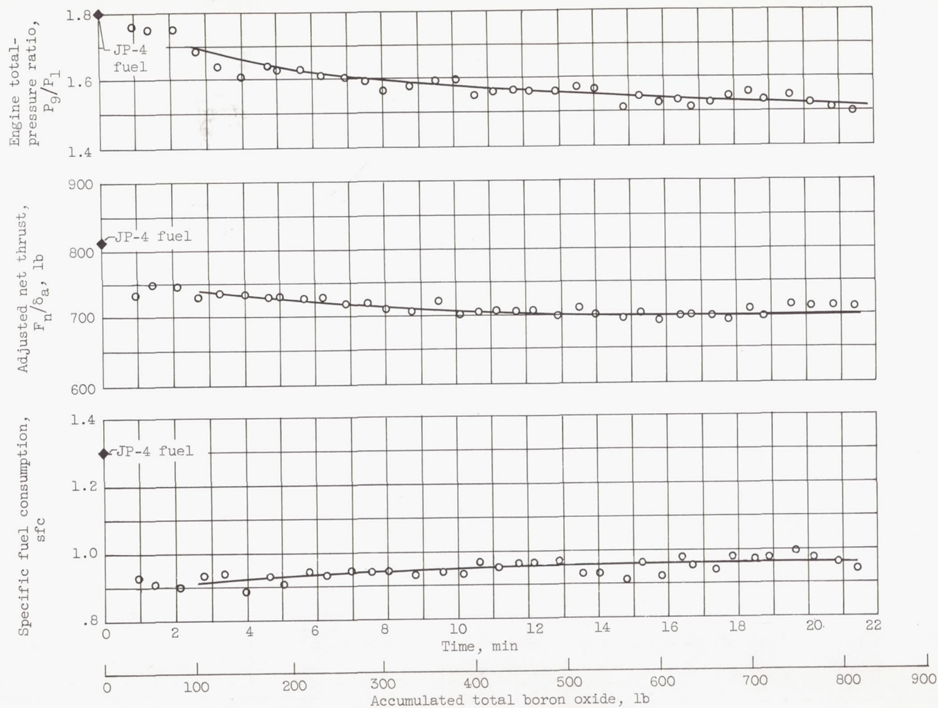
(a) Test 1; engine total-temperature ratio, 3.3.
