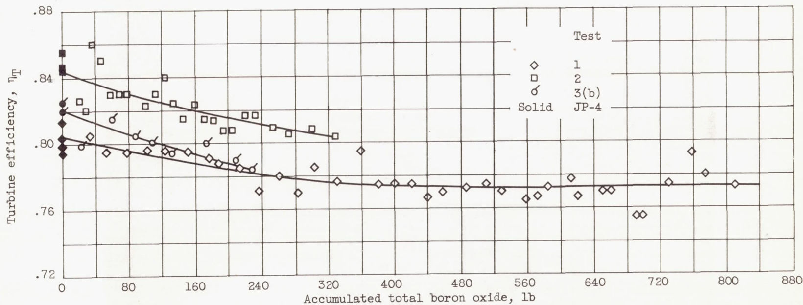
Figure 18. - Effect of boron oxide on turbine efficiency. Altitude, 50,000 feet; flight Mach number, 0.8; corrected engine speed, 90 to 98 percent of rated speed.
