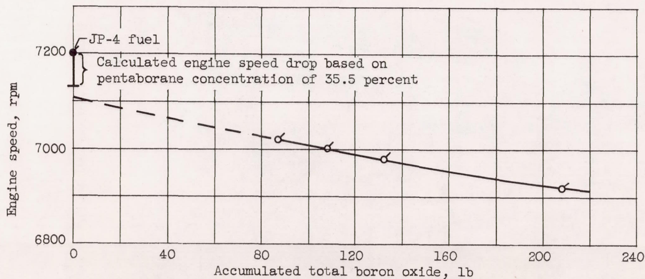
Figure 20. - Engine speed variation resulting from operation with pentaborane - JP-4 mixture in a turbojet engine having a fixed-area exhaust nozzle, test 3(b). Altitude, 50,000 feet; flight Mach number, 0.8; engine total-temperature ratio, 3.48; pentaborane concentration, 35.5 percent.
