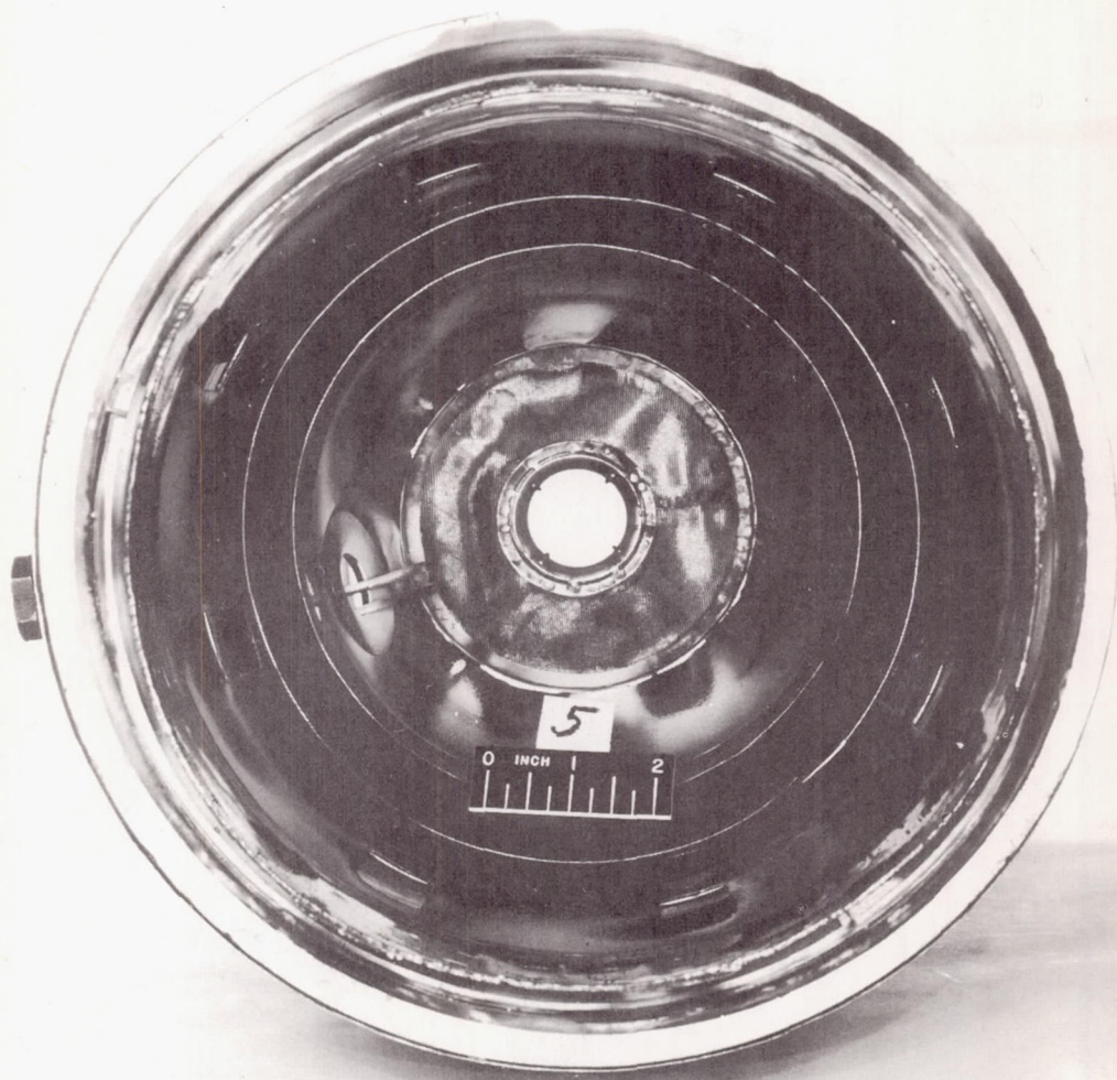
Figure 15. - Photograph of wire-cloth combustor after test 4. Total test time, 5 minutes.
