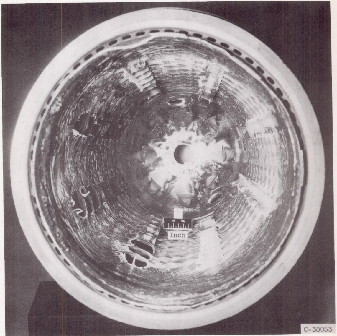
(b) Test 1, relatively clean combustion chamber. Total test time, 22 minutes.
