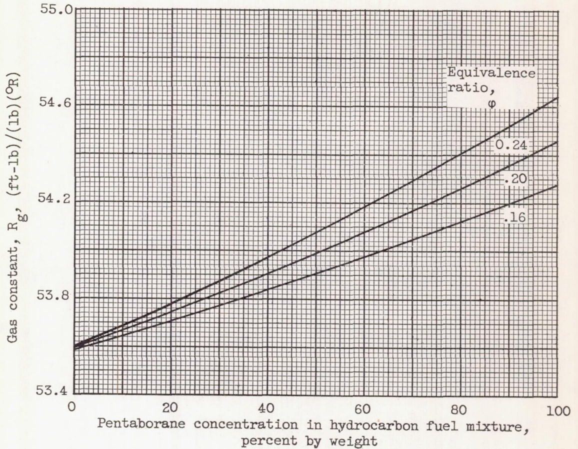
(c) Gas constant.
