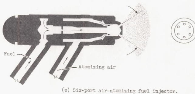
Figure 3. - Fuel injectors used in full-scale engine tests.
