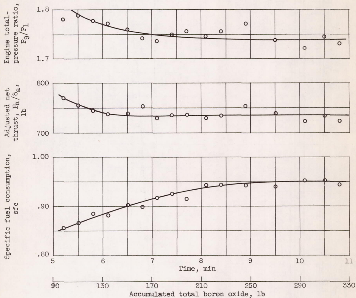
Figure 9. - Concluded. Effect of operation with 100 percent pentaborane fuel on turbojet-engine performance. Altitude, 50,000 feet; flight Mach number, 0.8; corrected engine speed, 98 percent of rated speed.
