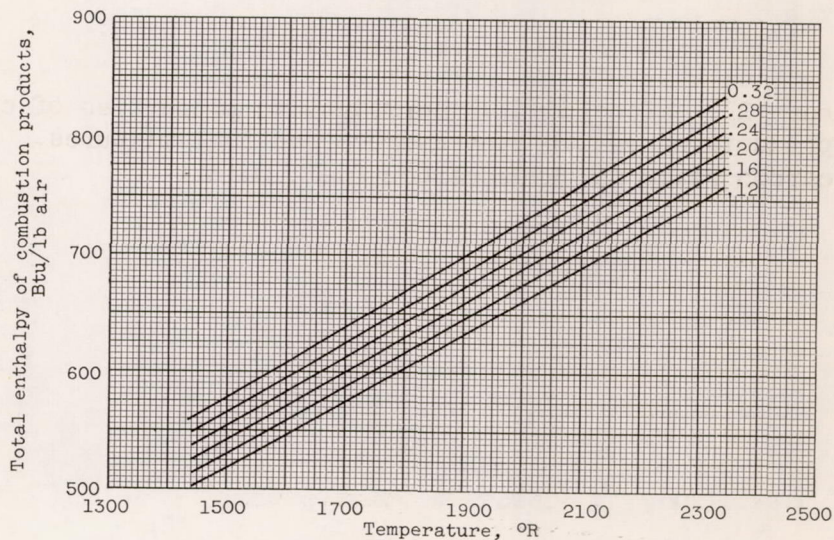
(c) Total enthalpy of combustion products.
