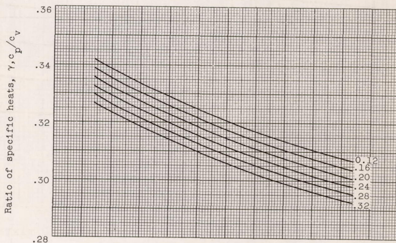
(b) Ratio of specific heats.
