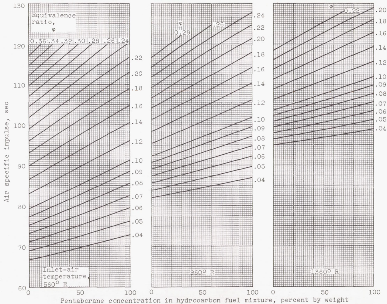
(a) Air specific impulse.
