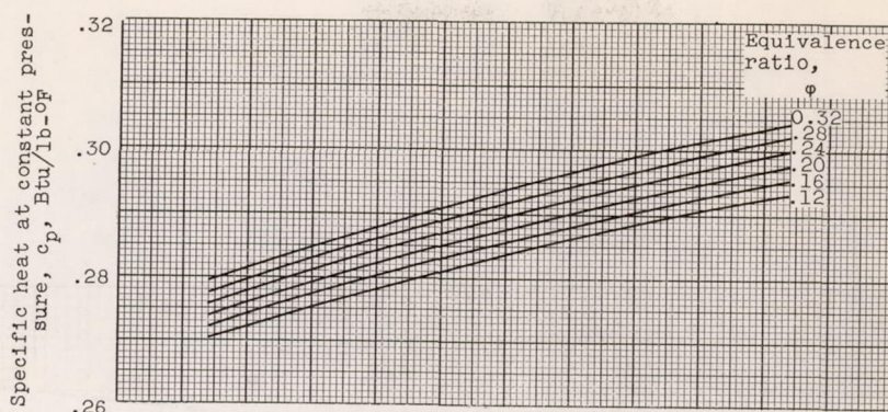
(a) Specific heat at constant pressure.
