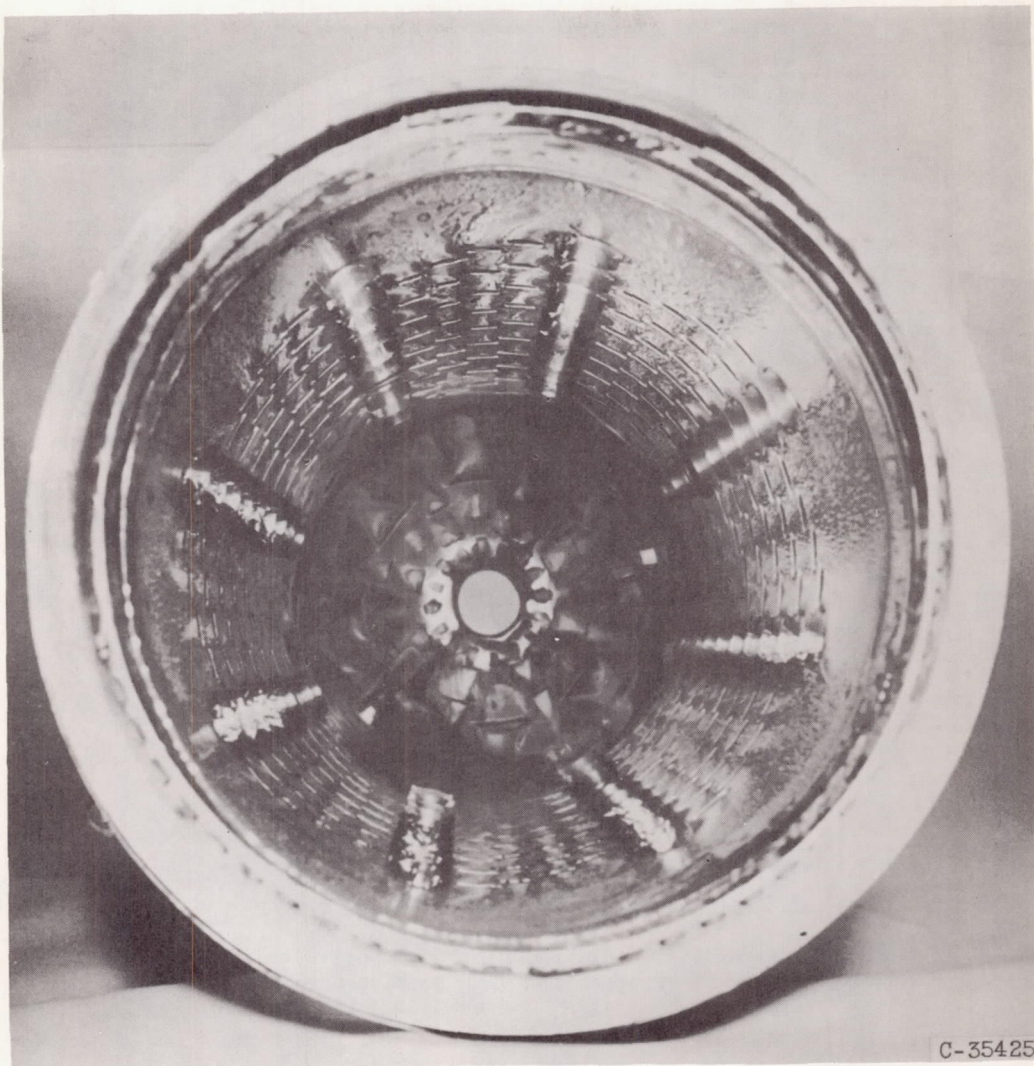
(a) Test 3. Total test time, 12 minutes.
