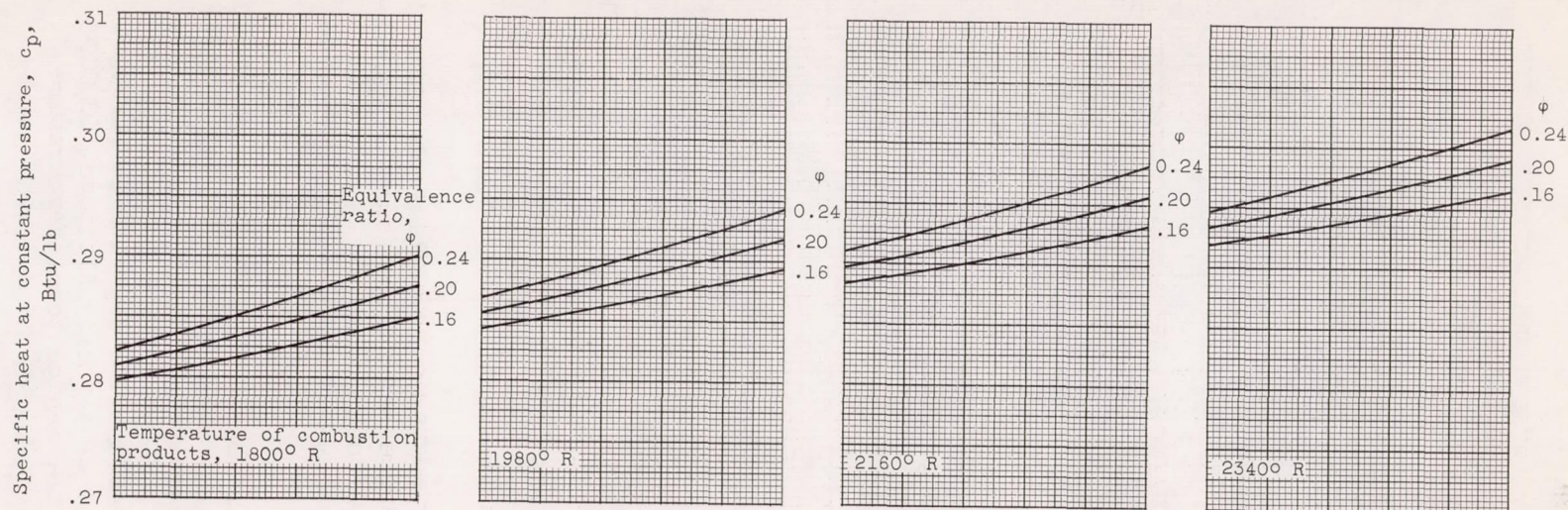
(a) Specific heat at constant pressure.
