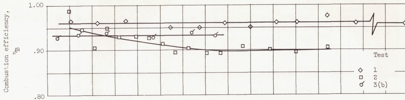
(a) Combustion efficiency.
