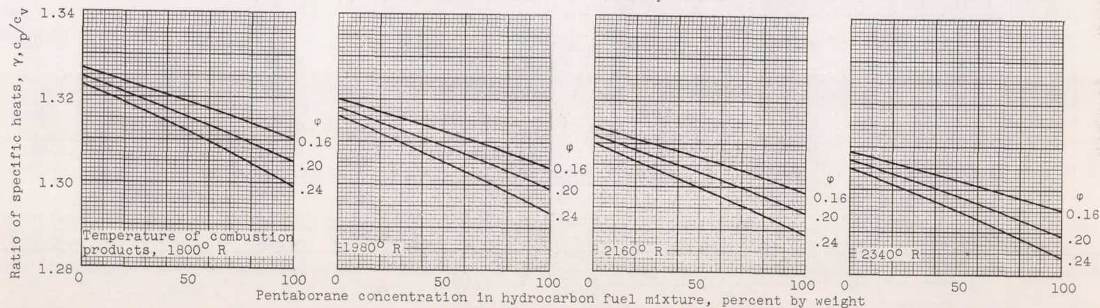
(b) Ratio of specific heats.
