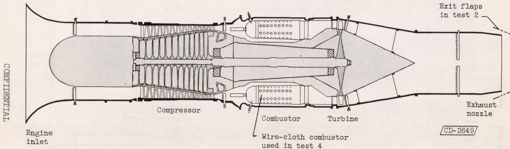
(b) Tests 2, 3, and 4.
