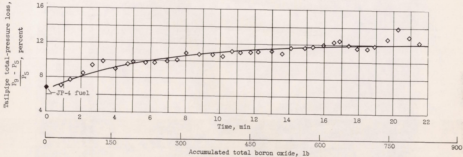
Figure 22. - Variation of tailpipe total-pressure loss during operation with pentaborane fuel in test 1.
