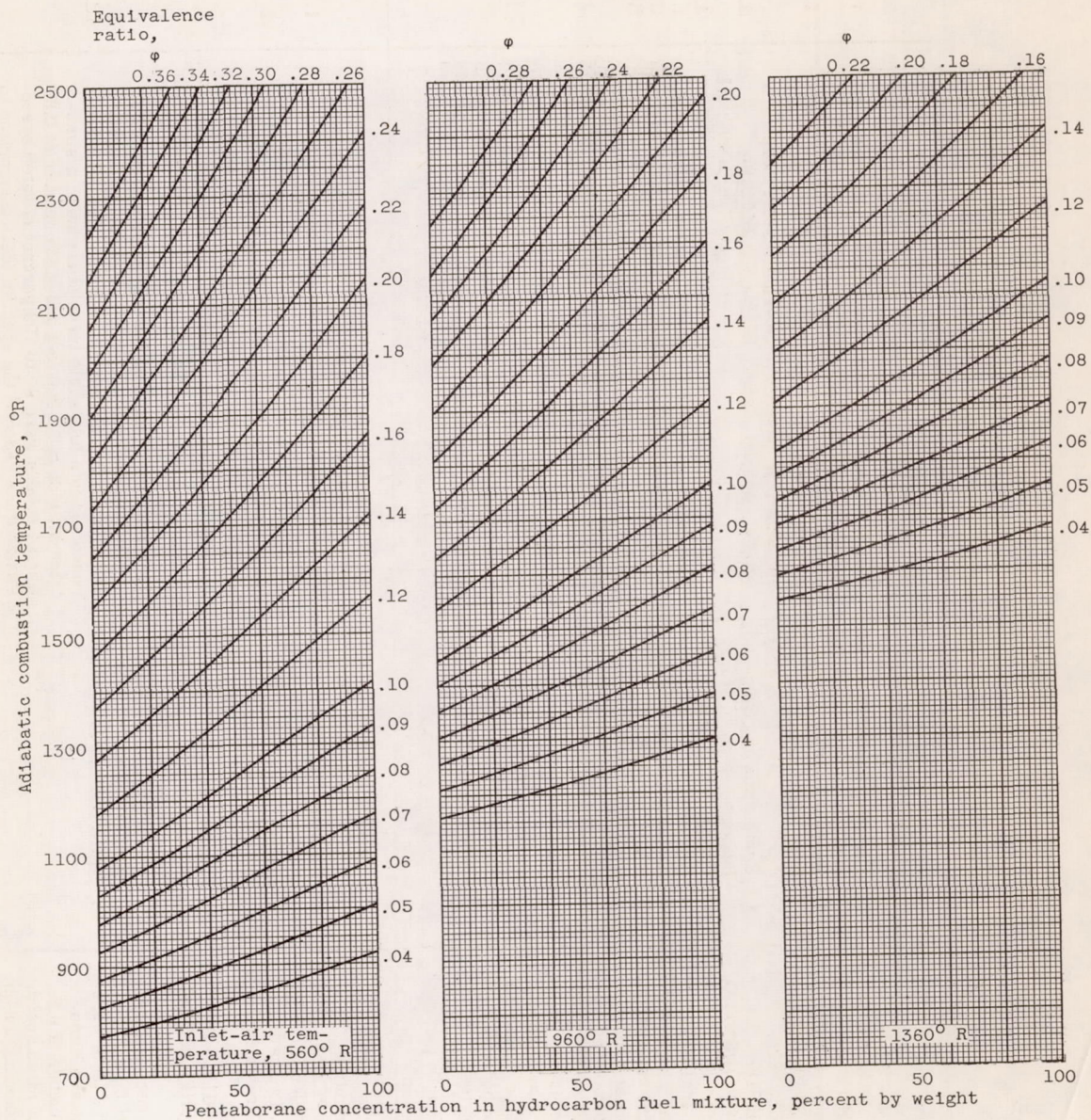
Figure 29. - Concluded. Air specific impulse and combustion temperature values for pentaborane-hydrocarbon fuel mixtures at several inlet-air temperatures. Hydrogen-carbon ratio for hydrocarbon fuel, 0.168.
