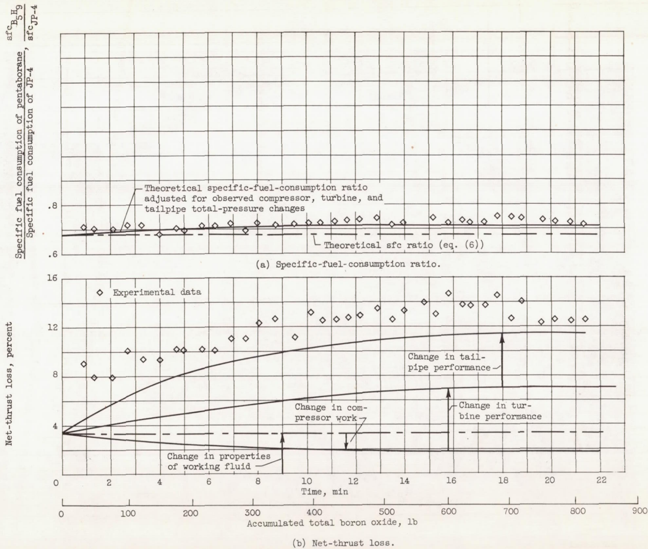
Figure 24. - Engine performance loss encountered with use of pentaborane fuel for test 1. Altitude, 50,000 feet; flight Mach number, 0.8.
