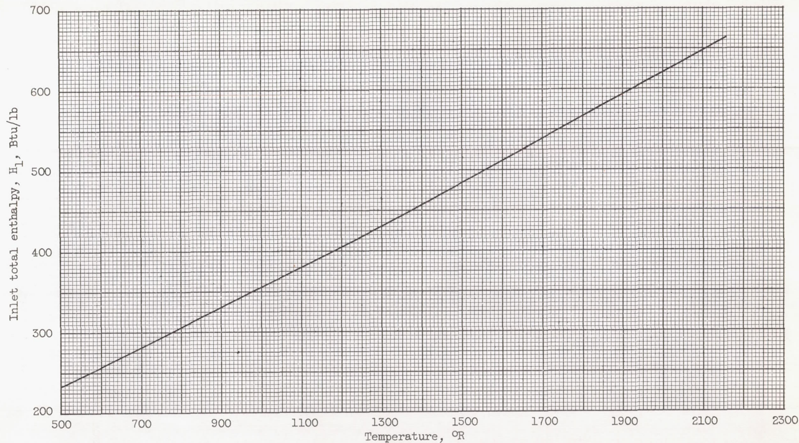
Figure 27. - Continued. Thermodynamic properties of combustion products of pentaborane-hydrocarbon fuel mixtures. Hydrogen-carbon ratio for hydrocarbon fuel, 0.168.
