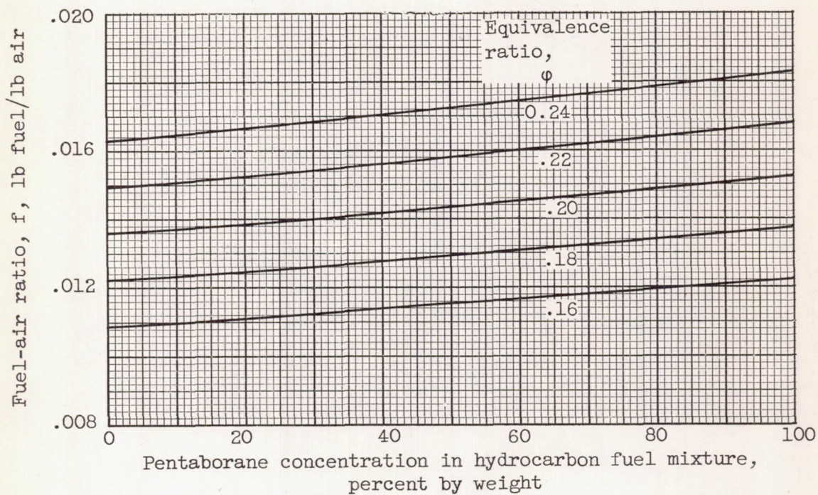
Figure 27. - Concluded. Thermodynamic properties of combustion products of pentaborane-hydrocarbon fuel mixtures. Hydrogen-carbon ratio for hydrocarbon fuel, 0.168.
