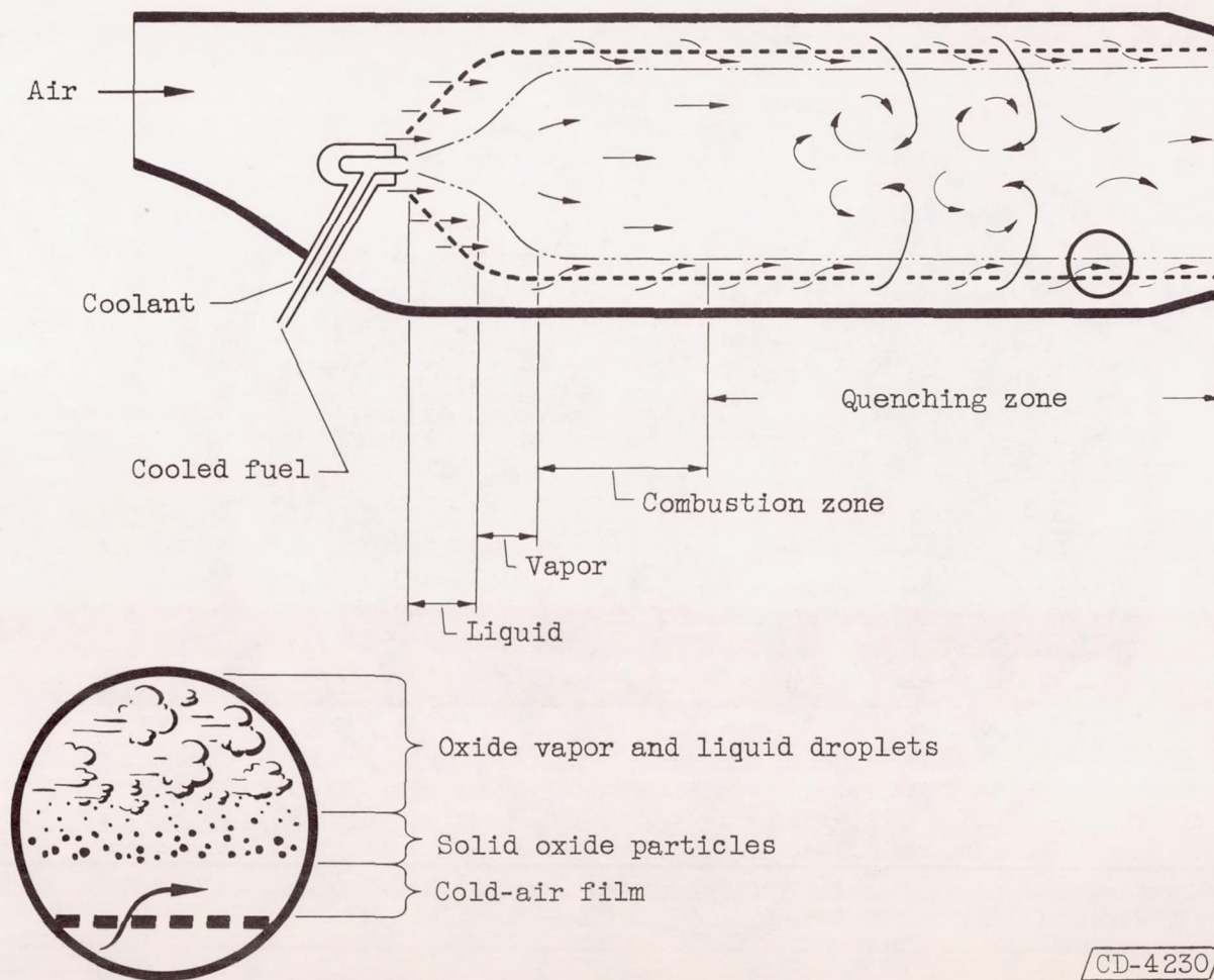
Figure 14. - Wire-cloth combustor design.
