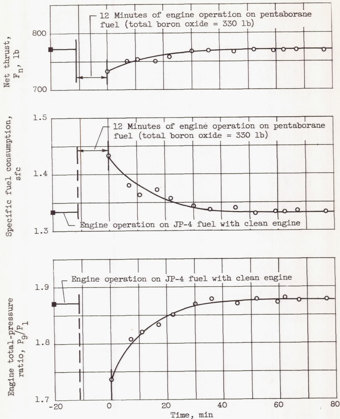
Figure 26. - Dissipation of boron oxide deposits in turbojet engine during operation with JP-4 fuel. Altitude, 50,000 feet; flight Mach number, 0.8; engine total-temperature ratio, 3.3.
