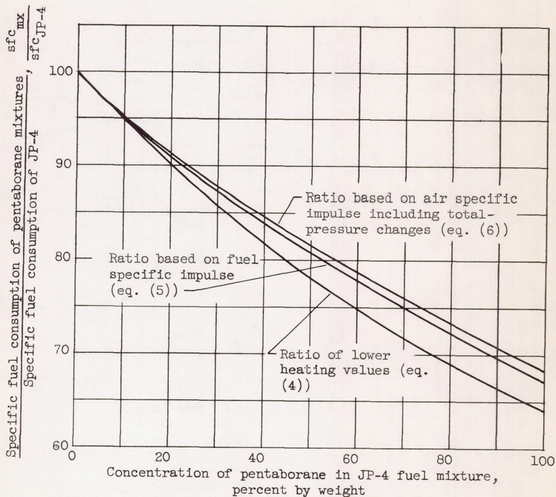
Figure 6. - Comparison of methods for calculating specific fuel consumption for pentaborane - JP-4 fuel mixtures. Flight Mach number, 0.8; altitude, 50,000 feet; 100 per cent of rated engine speed.
