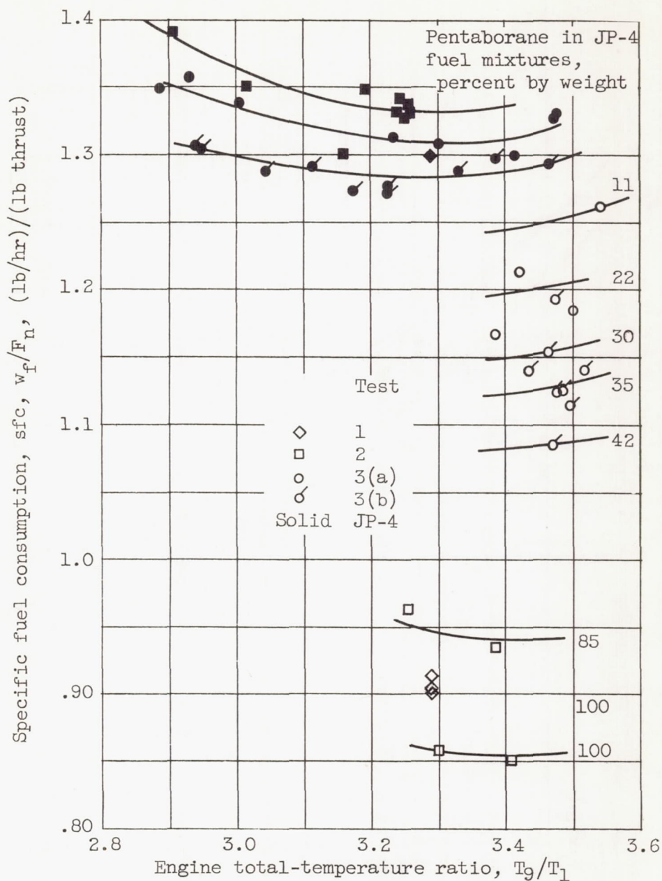
Figure 7. - Variation of specific fuel consumption based on net thrust with engine total-temperature ratio for a range of mixtures of pentaborane and JP-4 fuel. Altitude, 50,000 feet; flight Mach number, 0.8; corrected engine speed, 90 to 98 per cent of rated speed.
