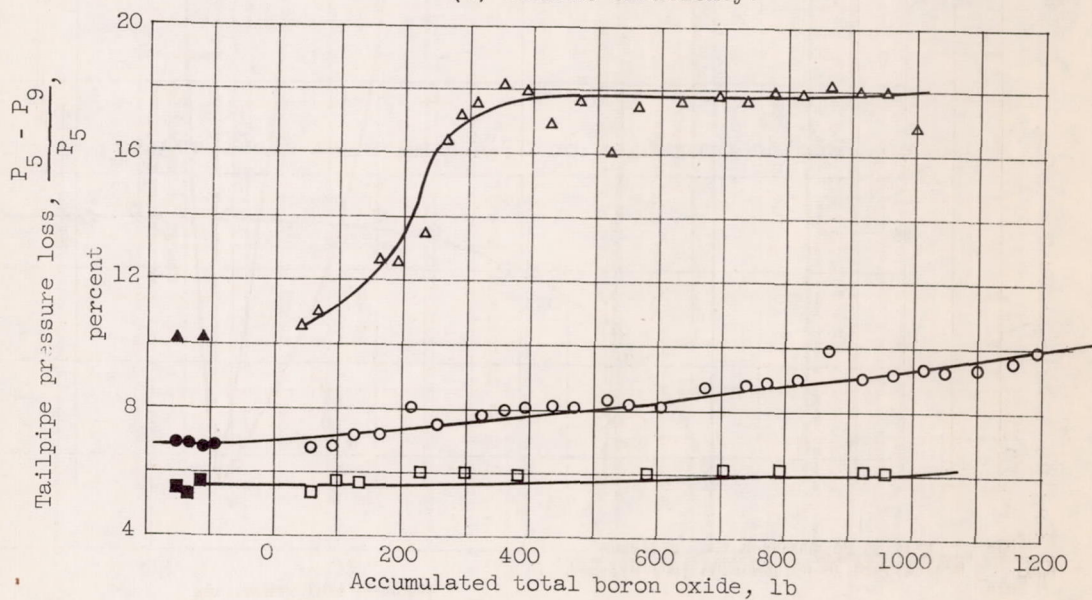
(c) Tailpipe pressure loss.
