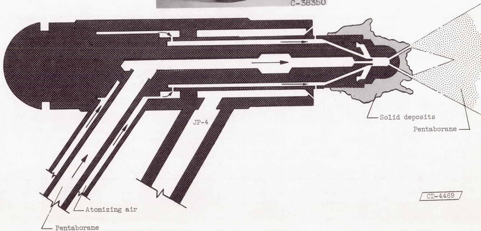
Figure 13. - Boron oxide deposits on turbojet-engine fuel nozzle after 22 minutes of operation with pentaborane.
