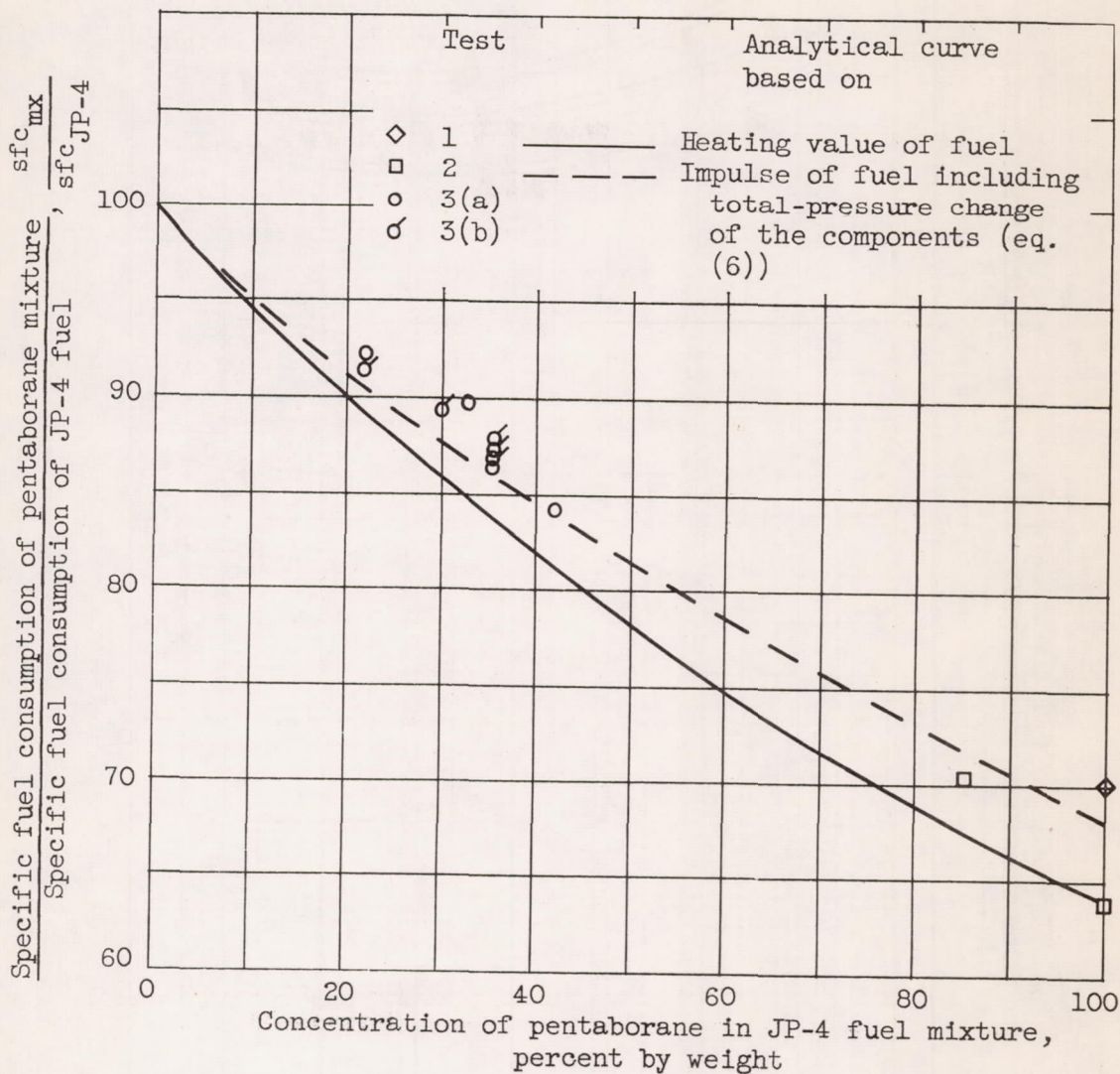
Figure 8. - Effect of pentaborane mixture concentration in JP-4 fuel on specific fuel consumption based on net thrust. Engine total-temperature ratio, 3.48; altitude, 50,000 feet; flight Mach number, 0.8; corrected engine speed, 90 to 98 percent of rated speed.
