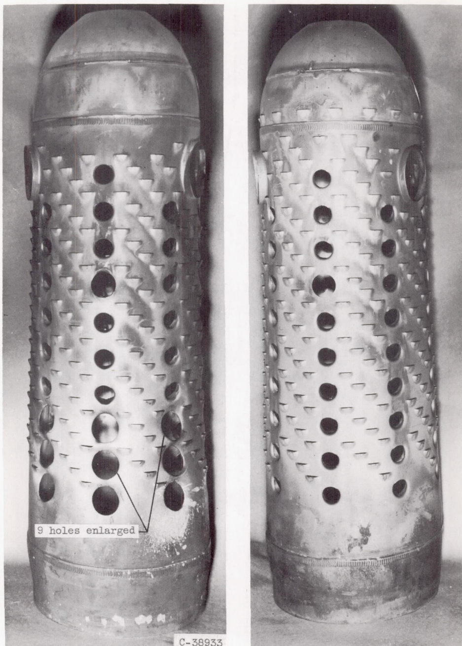
(b) Tests 2 and 3.
