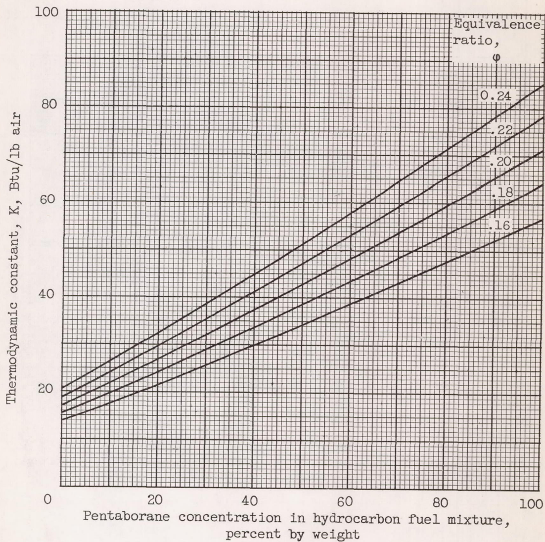
Figure 27. - Continued. Thermodynamic properties of combustion products of pentaborane-hydrocarbon fuel mixtures. Hydrogen-carbon ratio for hydrocarbon fuel, 0.168.
