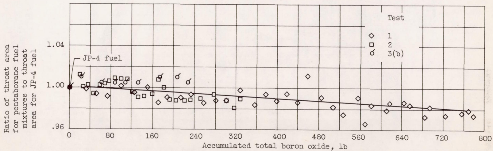
Figure 16. - Influence of engine operation with pentaborane fuel mixtures on calculated turbine-nozzle-diaphragm throat area.
