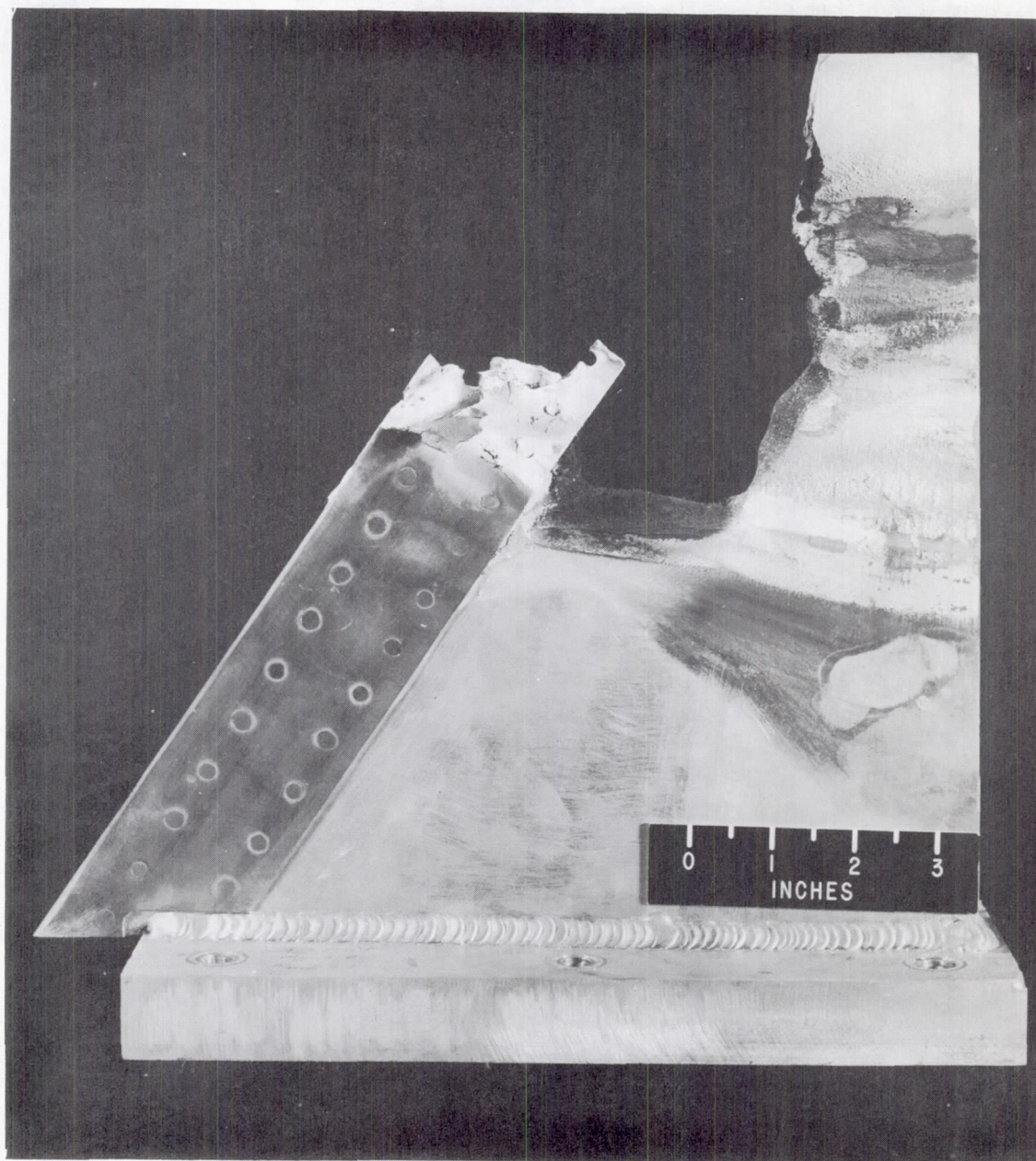
Figure 6.- Damage to model 3 after exposure for 3.2 seconds at 3,500^{\circ} R.
