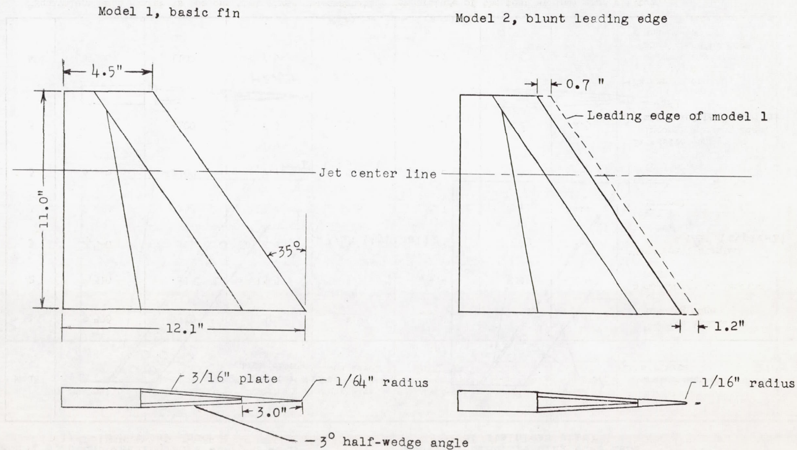
Figure 1.- General features of the models.
