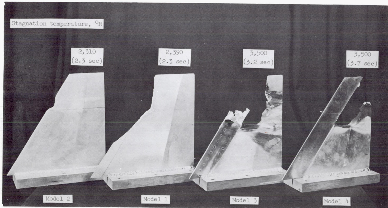
Figure 8.- Damage to all models under indicated conditions. L-93484.1
