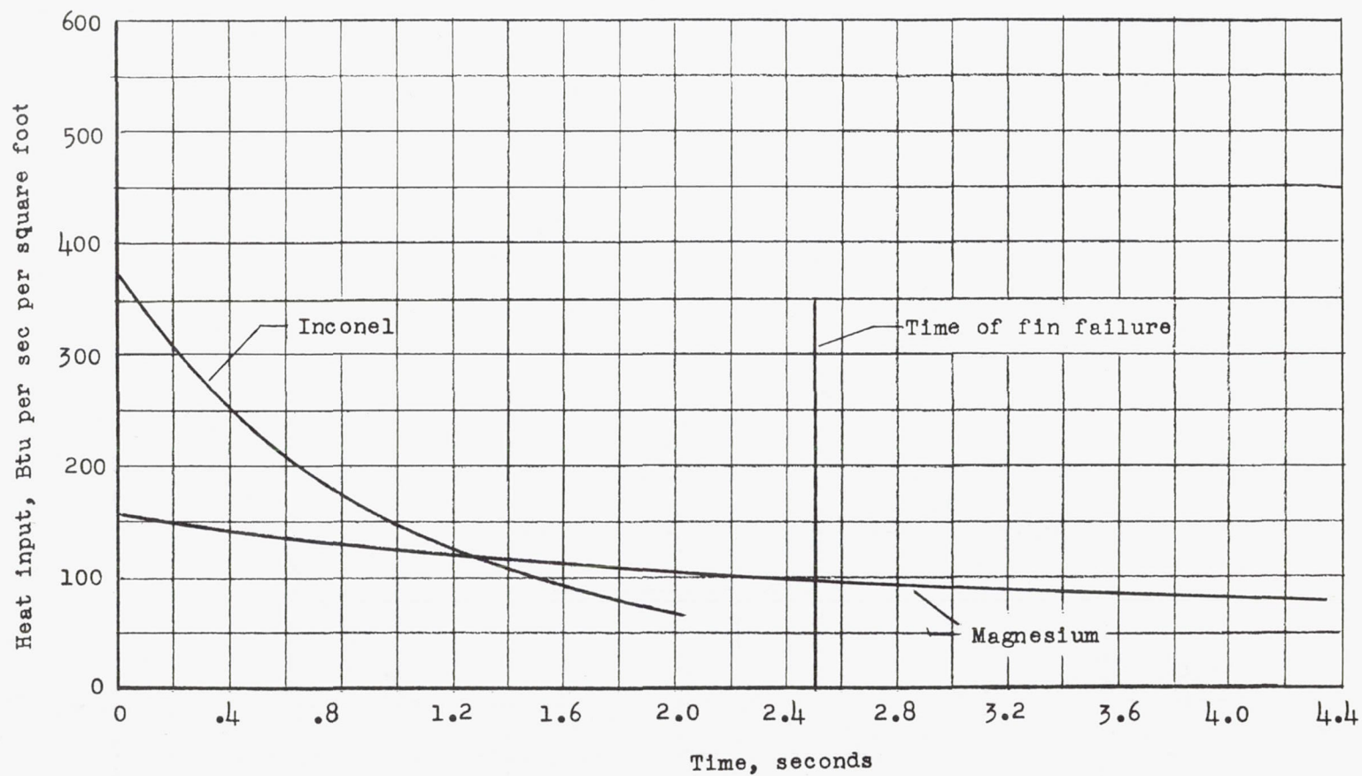
Figure 10.- Calculated heat input to the leading edge and to the surface 2.5 inches behind the leading edge of model 3 for a stagnation temperature of 3,500° R.
