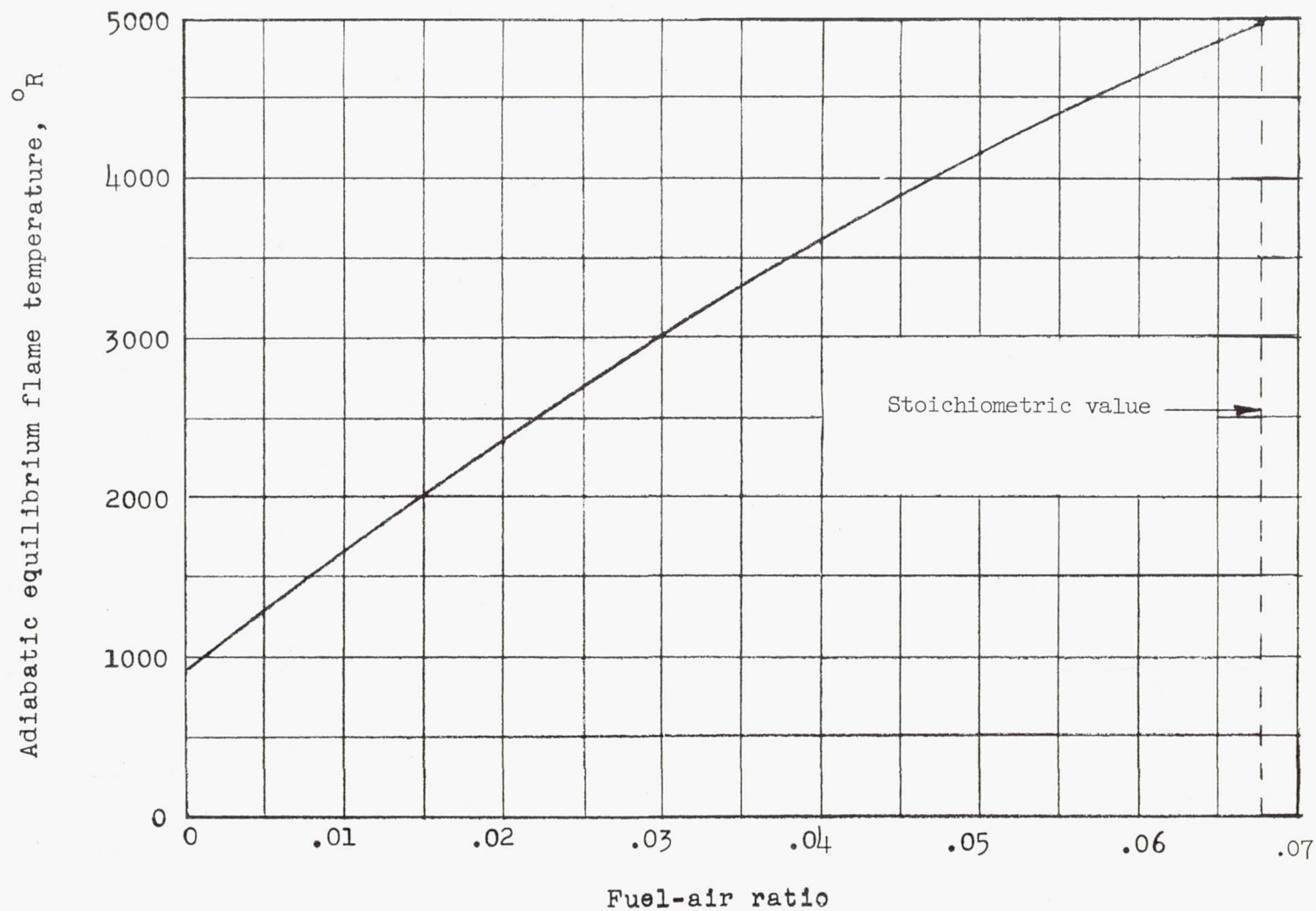
Figure 12.- Computed adiabatic equilibrium flame temperature from combustion of ethylene ( C_2H_4 ) fuel in air. Air preheat temperature, 900^{\circ}R .
