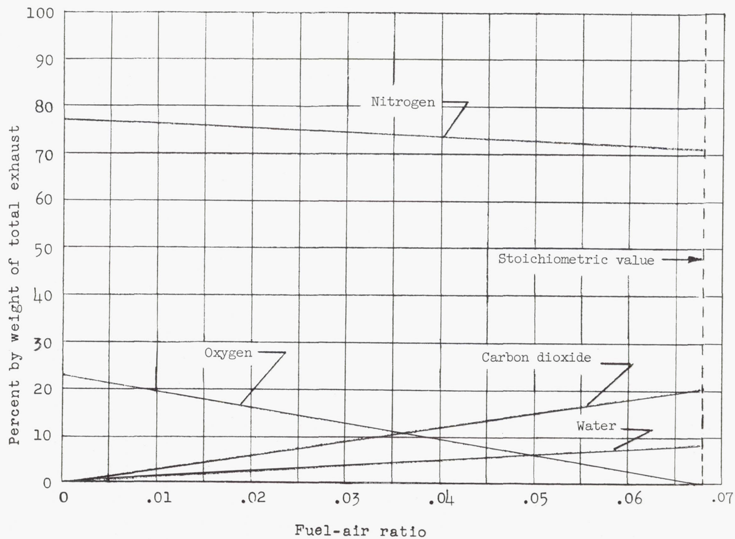
Figure 14.- Composition of exhaust from combustion of ethylene ( C_2H_4 ) in air.
