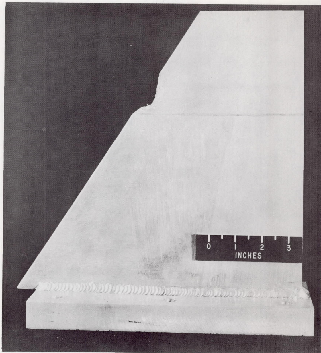
L-93485.1 Figure 5.- Damage to the leading edge of model 2 after exposure for 2.3 seconds at 2,310^{\circ} R.
