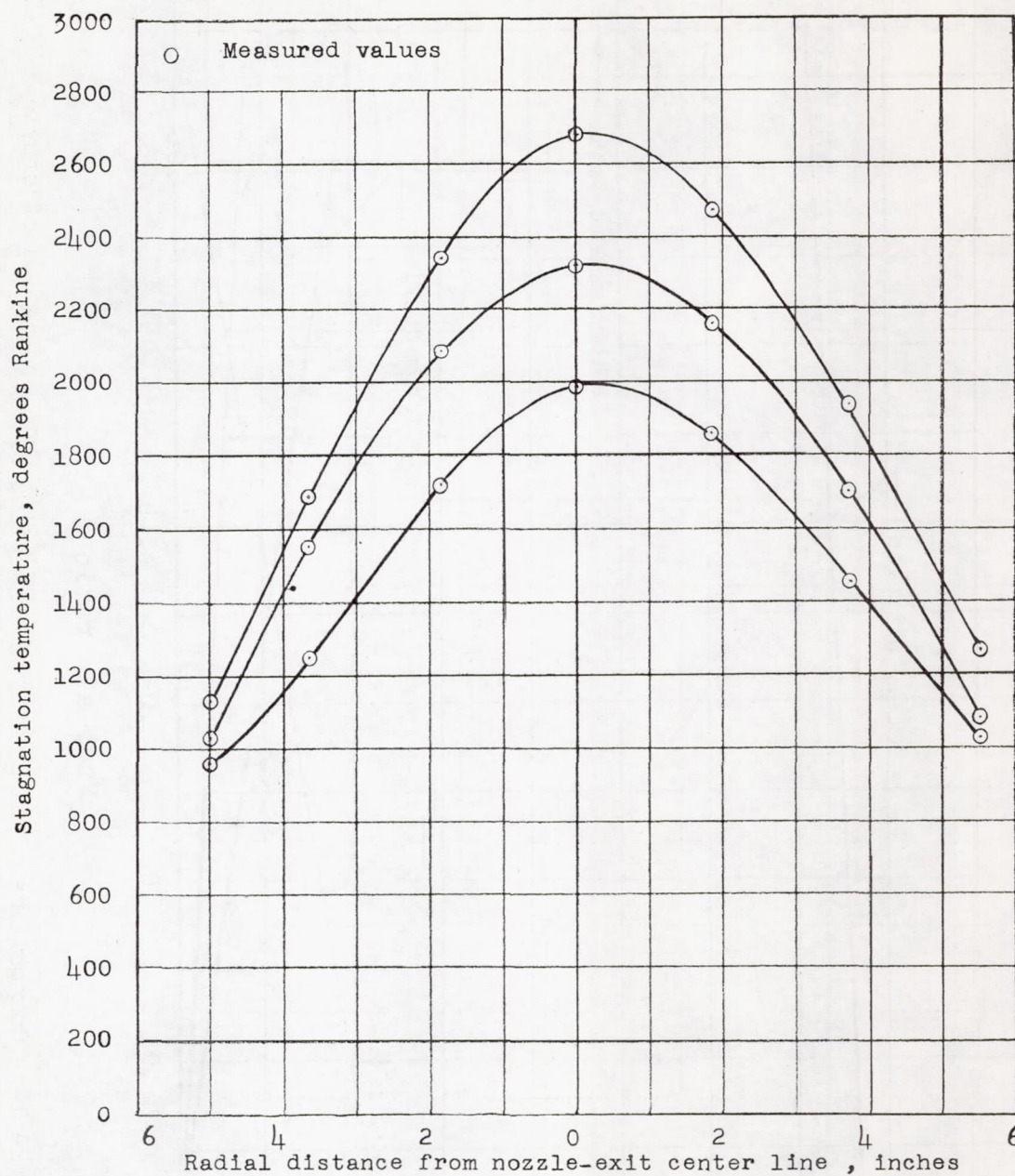
Figure 13.- Typical stagnation-temperature profiles across nozzle exit.
