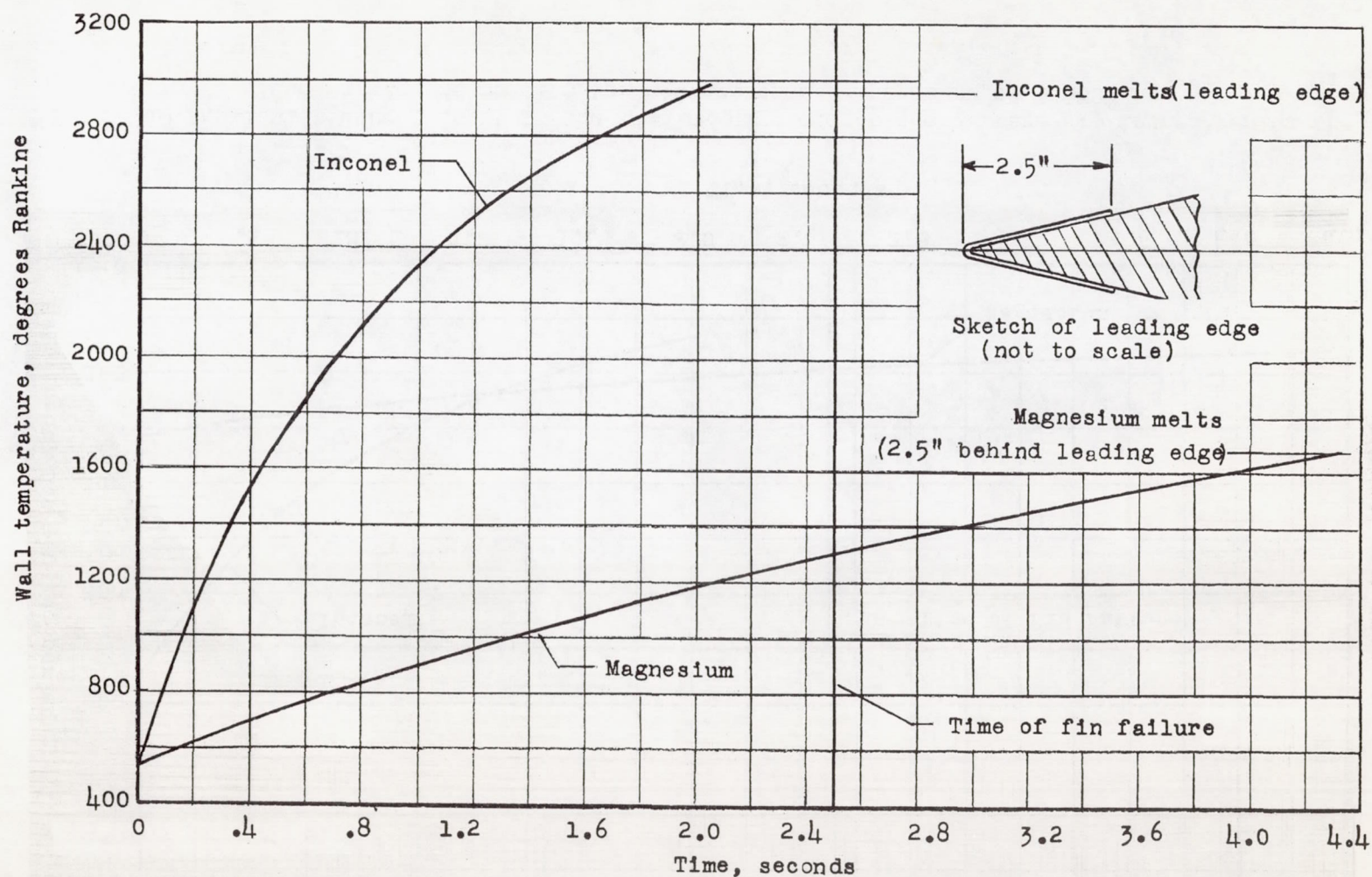
Figure 9.- Calculated wall temperature at the leading edge and on the surface 2.5 inches behind the leading edge of model 3 for a stagnation temperature of 3,500^{\circ}\text{R} .
