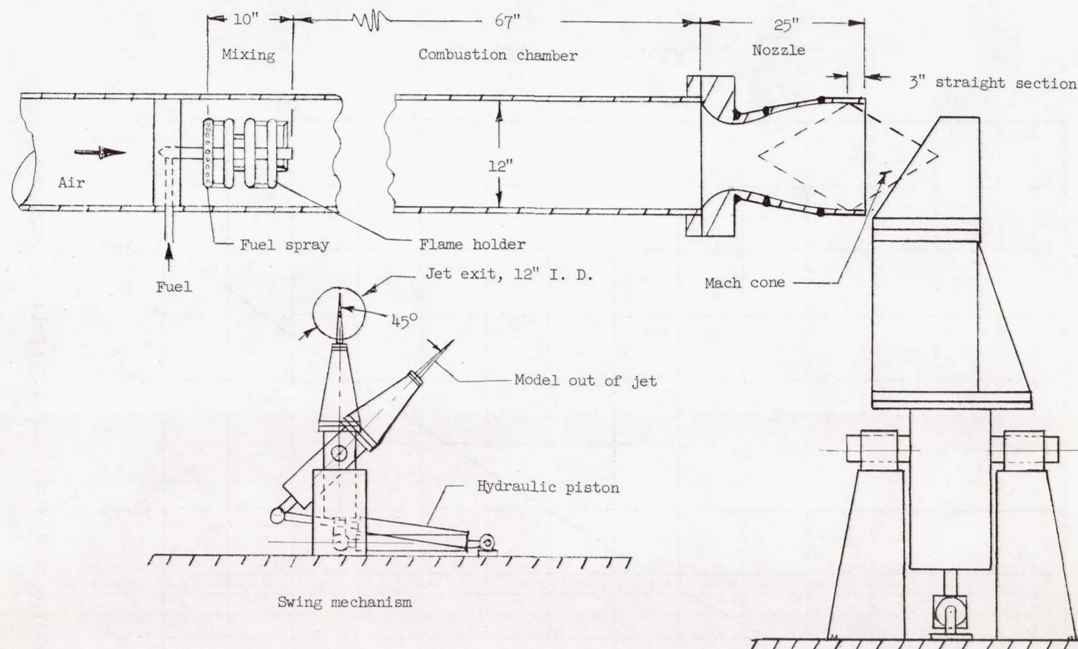
Figure 11.- Schematic drawing of preflight high-temperature jet.
