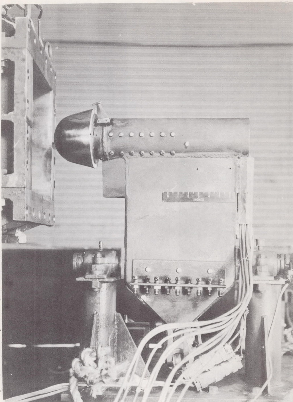
Figure 2.- Photograph of model A mounted at the exit of the 12- by 12-inch nozzle in the preflight-jet facility.
