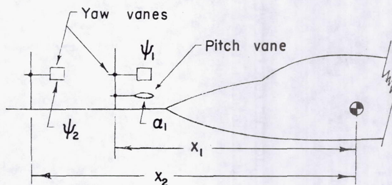
(b) Two yaw vanes and a pitch vane.
