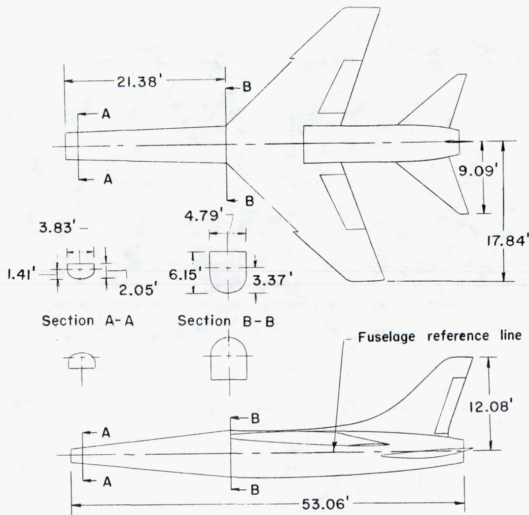
Figure 18.- Cross-sectional shapes of noses investigated on free-spinning model. Model 1. (Test data presented on charts 1 and 2.) Full-scale values given.
