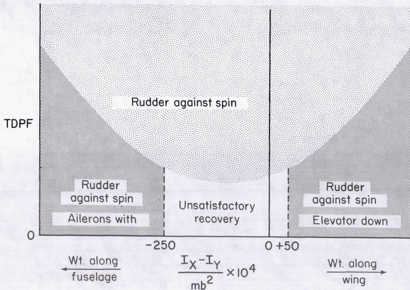
Figure 13.- Influence of mass distribution on optimum control movement for recovery from the spin.
