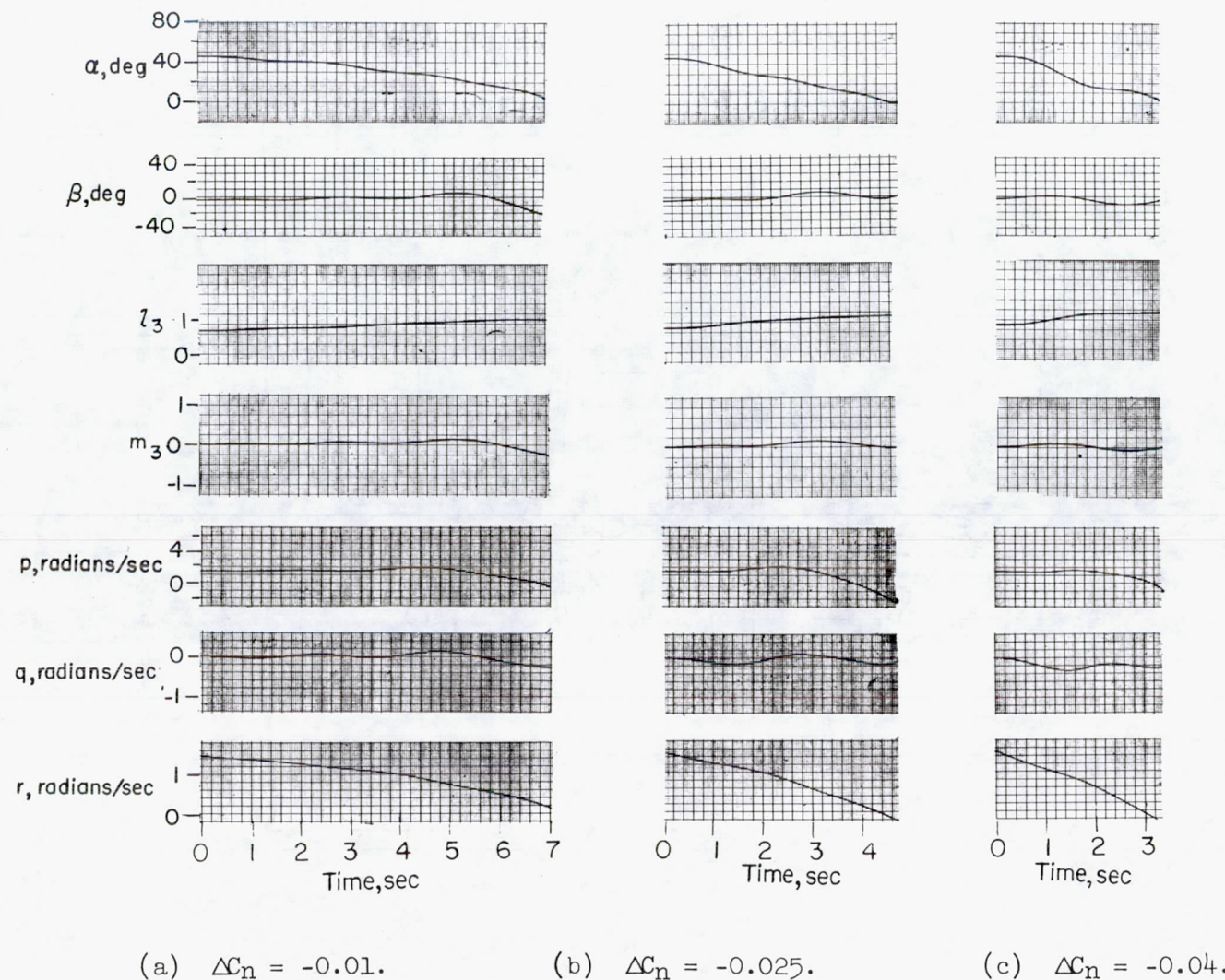
Figure 6.- Time histories following application of negative yawing moment (moment applied to steady spin at time zero).
