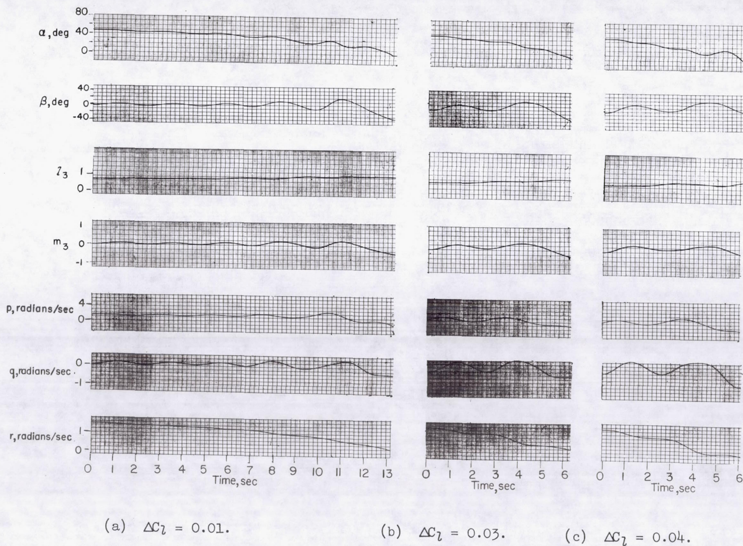
Figure 7.- Time histories following application of positive rolling moment (moment applied to steady spin at time zero).
