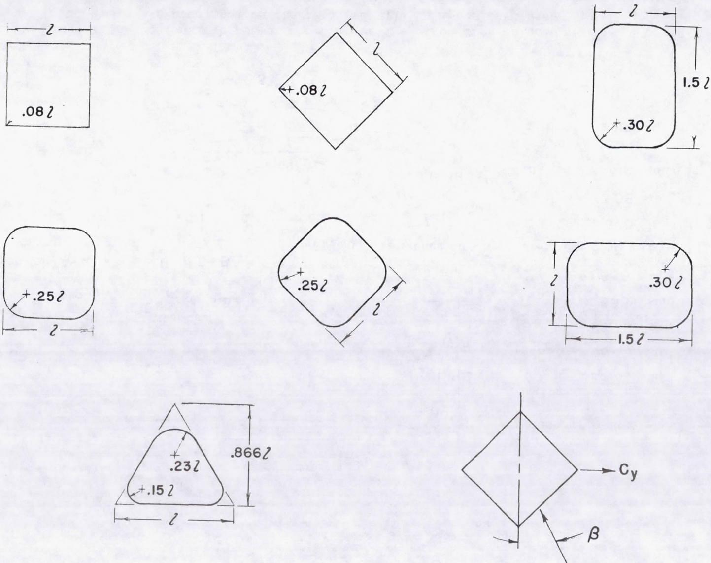
Figure 17.- Detailed dimensions of various shapes presented in figure 16.
