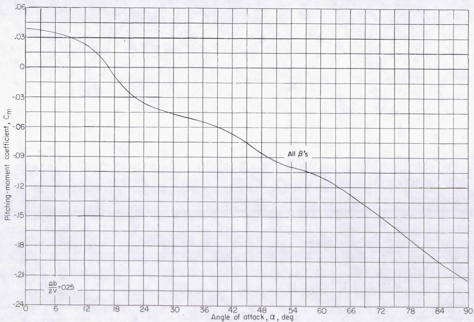
(e) Variation of C_m with \alpha .
