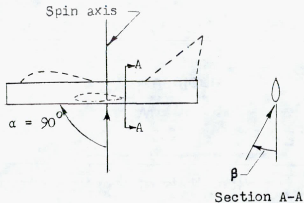
(a) Rectangular fuselage at 90^\circ angle of attack.
