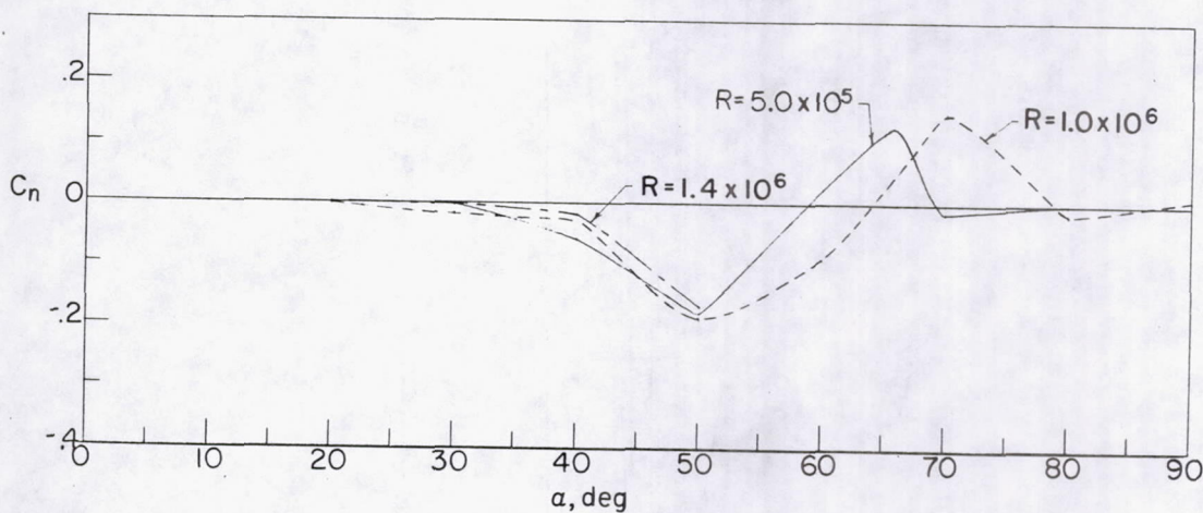
Figure 21.- Variation of yawing moment and side force with angle of attack for model 2. \beta = 0^\circ . Horizontal tail on. Dimensions given are full scale.
