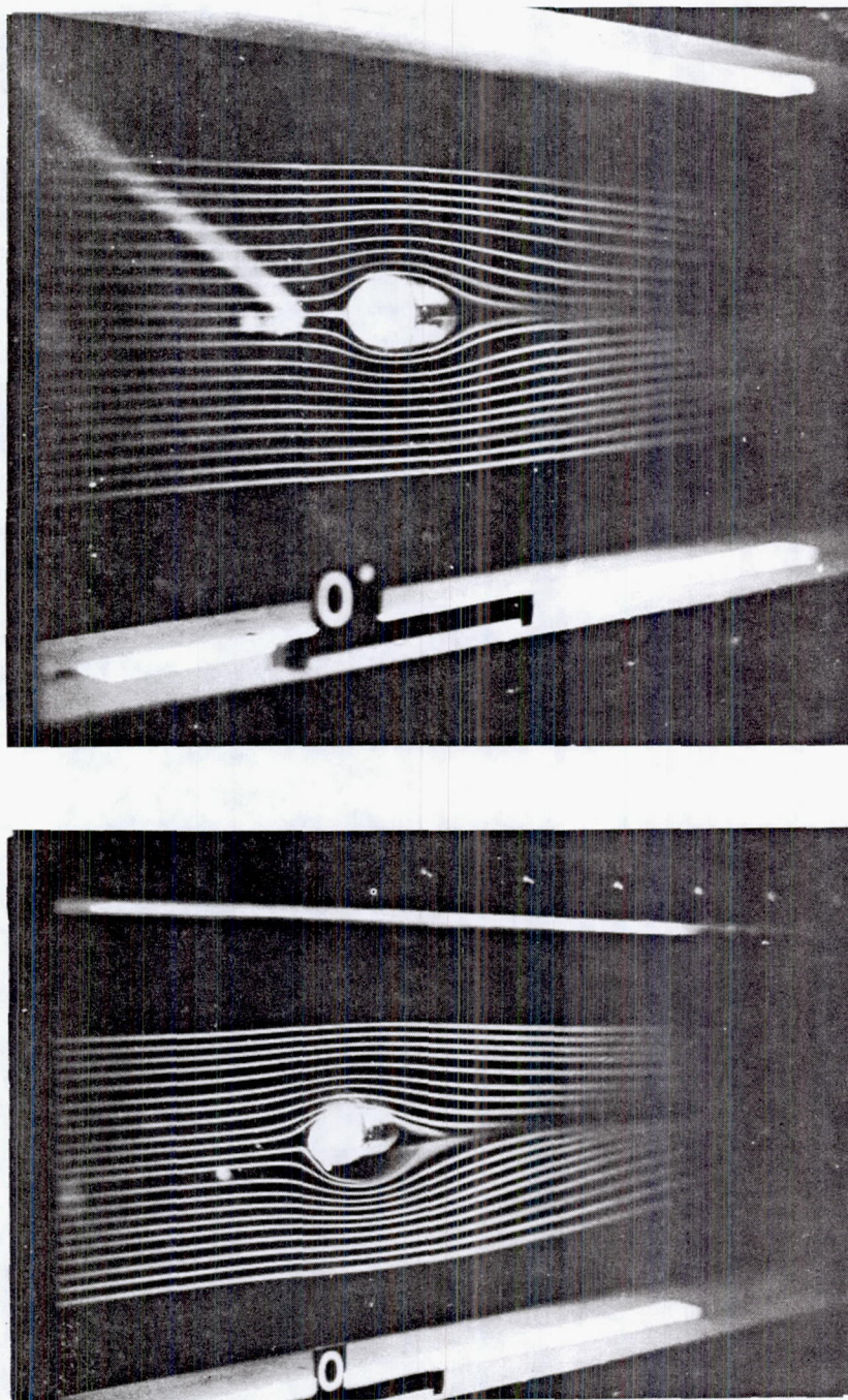
Figure 20.- Flow lines about a sharp-nosed model with and without a strake installed. \alpha = 50^\circ ; \beta = 0^\circ .
