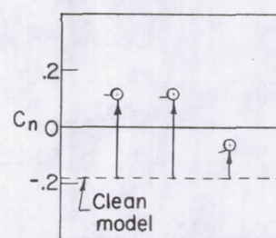
(d) Left strake positioned at various vertical locations; horizontal tail off; \alpha = 50^\circ .
