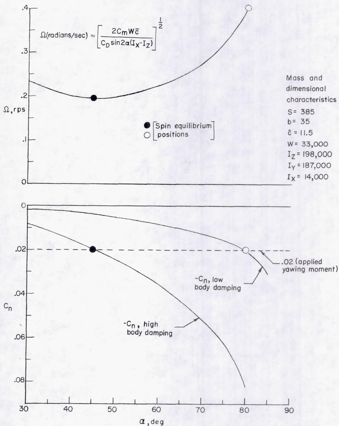
Figure 15.- Illustration of the manner in which the damping in yaw of a fuselage (assumed analogous to the damping in roll of a skewed wing) might affect the spin attitude of a contemporary fighter. An applied yawing-moment coefficient of 0.02 in the spin is assumed.
