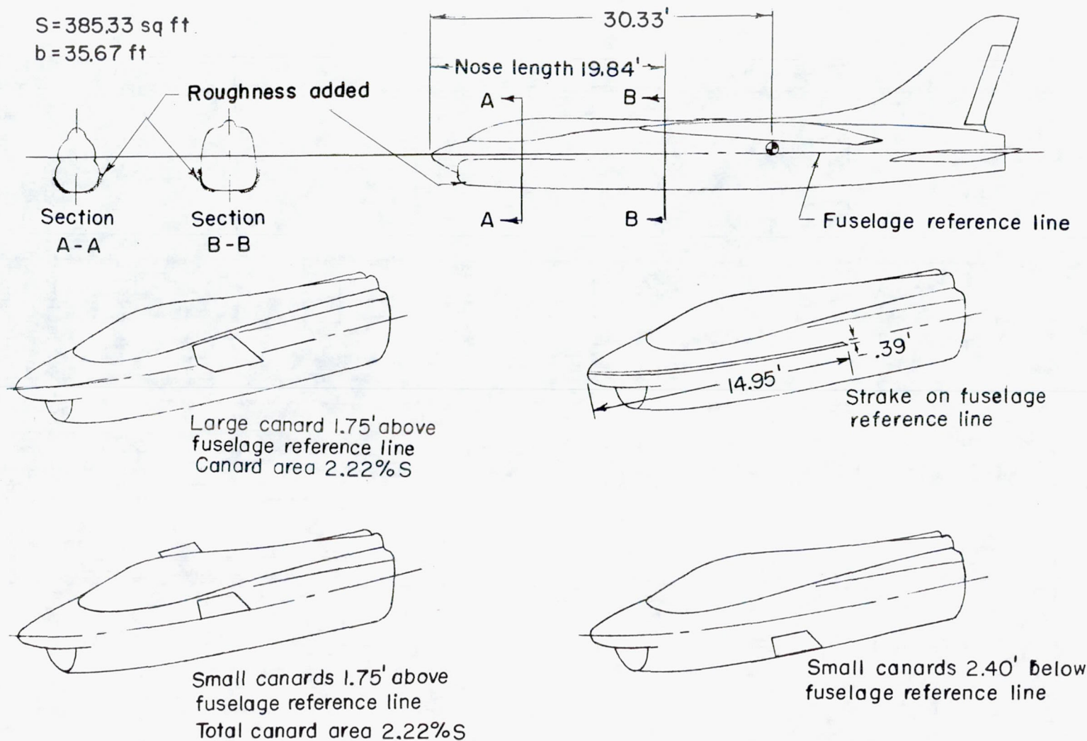
Figure 26.- Canards and strake investigated on model 4. Region in which roughness added is indicated by shaded areas. Full-scale dimensional values given.
