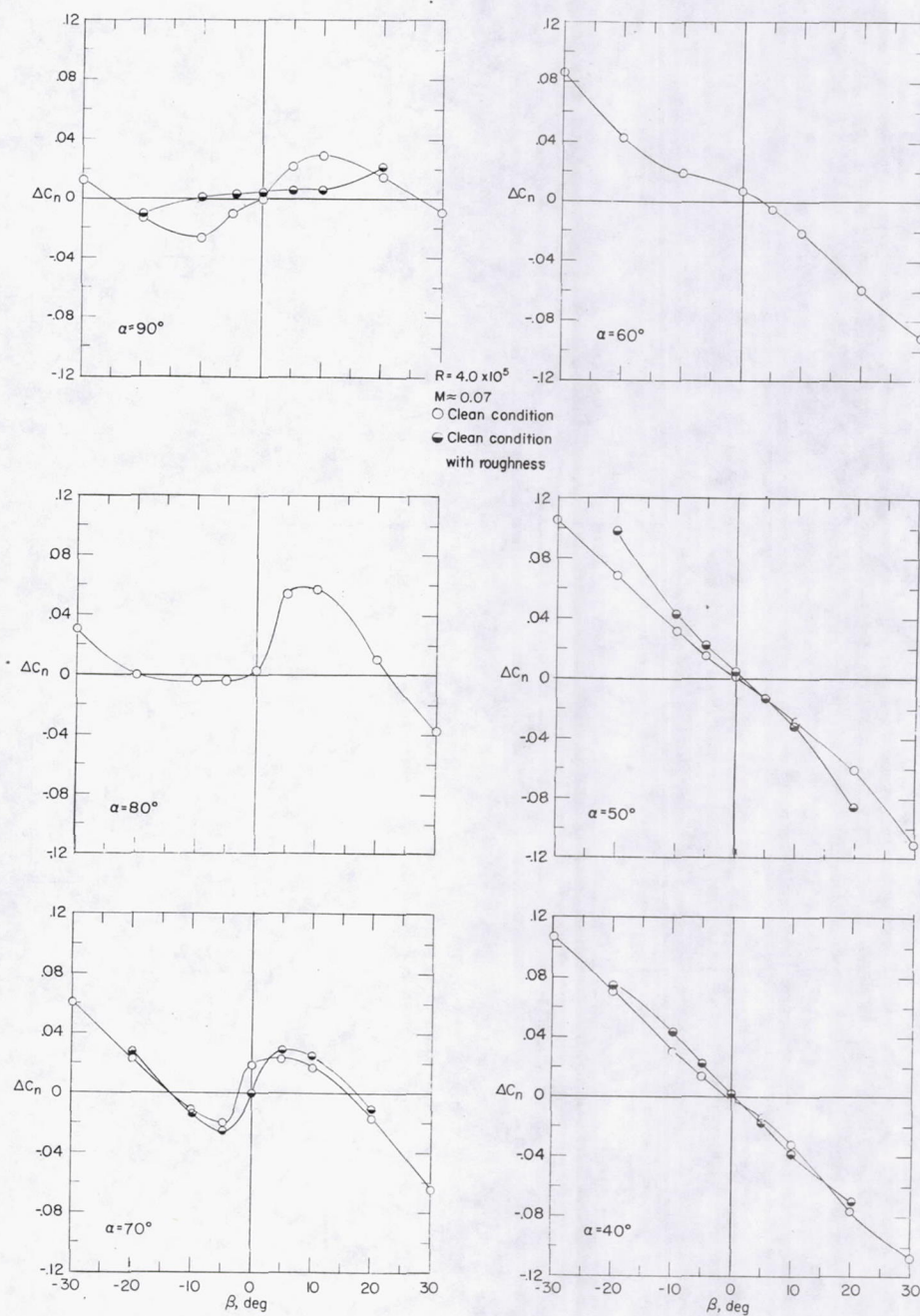
Figure 27.- Contribution of the nose on model 4 to the yawing moment about the center of gravity of the model.
