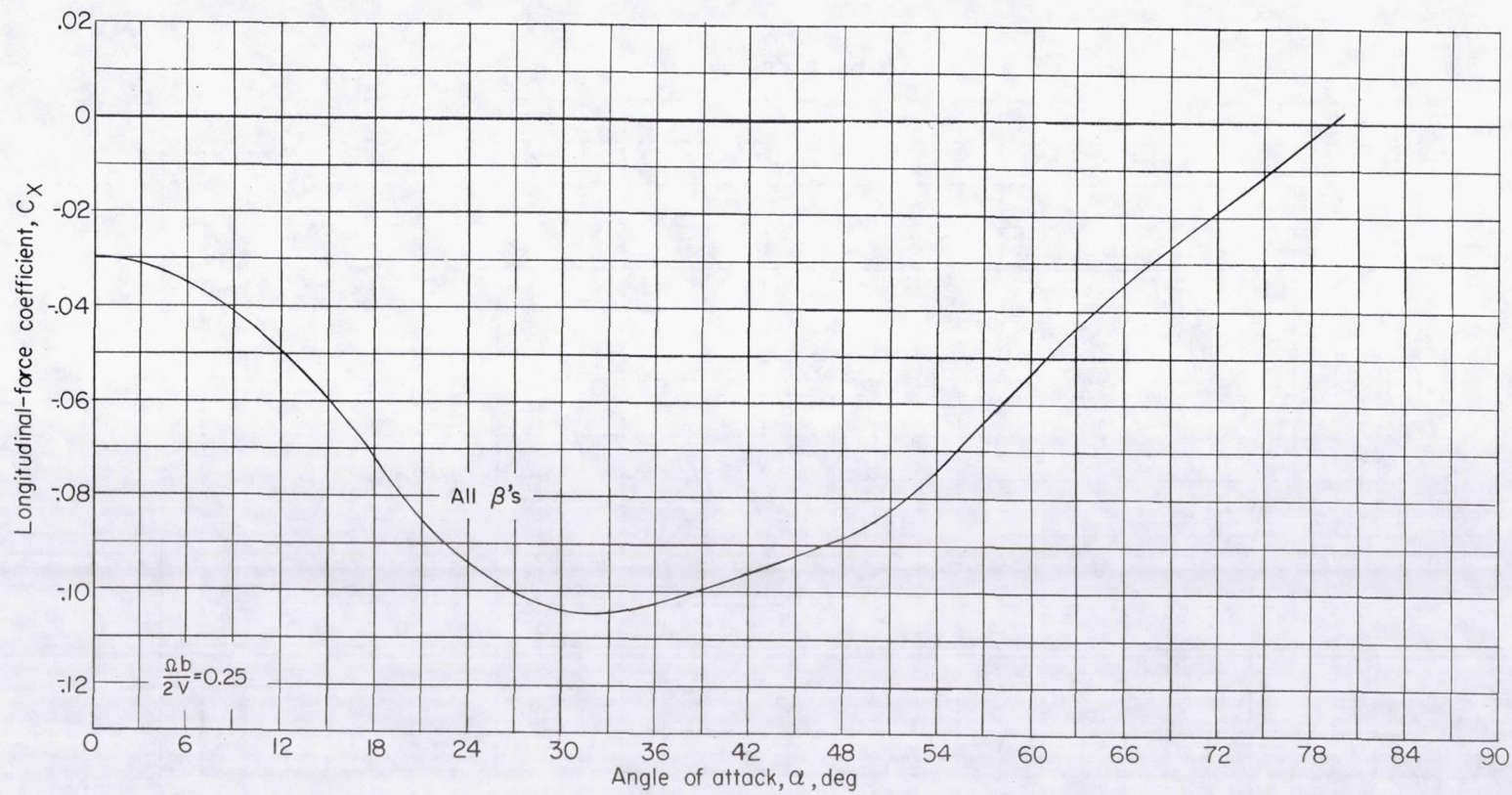
(a) Variation of C_x with \alpha .
