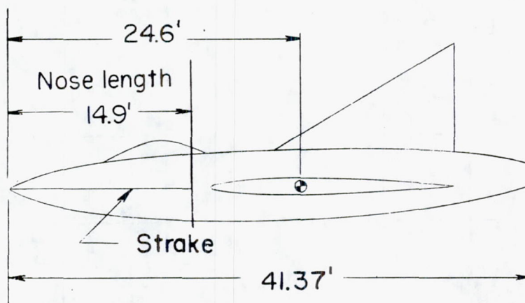
Figure 24.- Strakes investigated on model 3. Full-scale dimensional values given.
