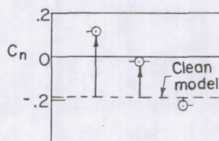
(b) Horizontal tail off; \alpha = 50^\circ .
