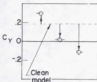
(c) Horizontal tail off; \alpha = 66^\circ .
