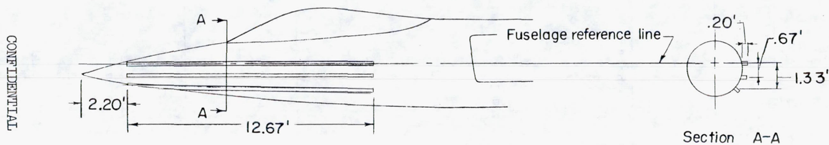
Figure 22.- Strake positions investigated on model 2. Dimensions given are full scale.
