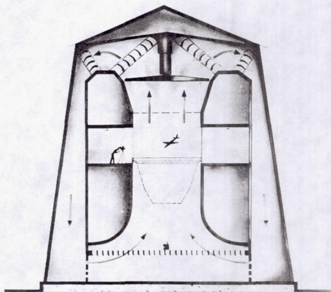
Figure 2.- Exterior and cross-sectional views of Langley 20-foot free-spinning tunnel.
