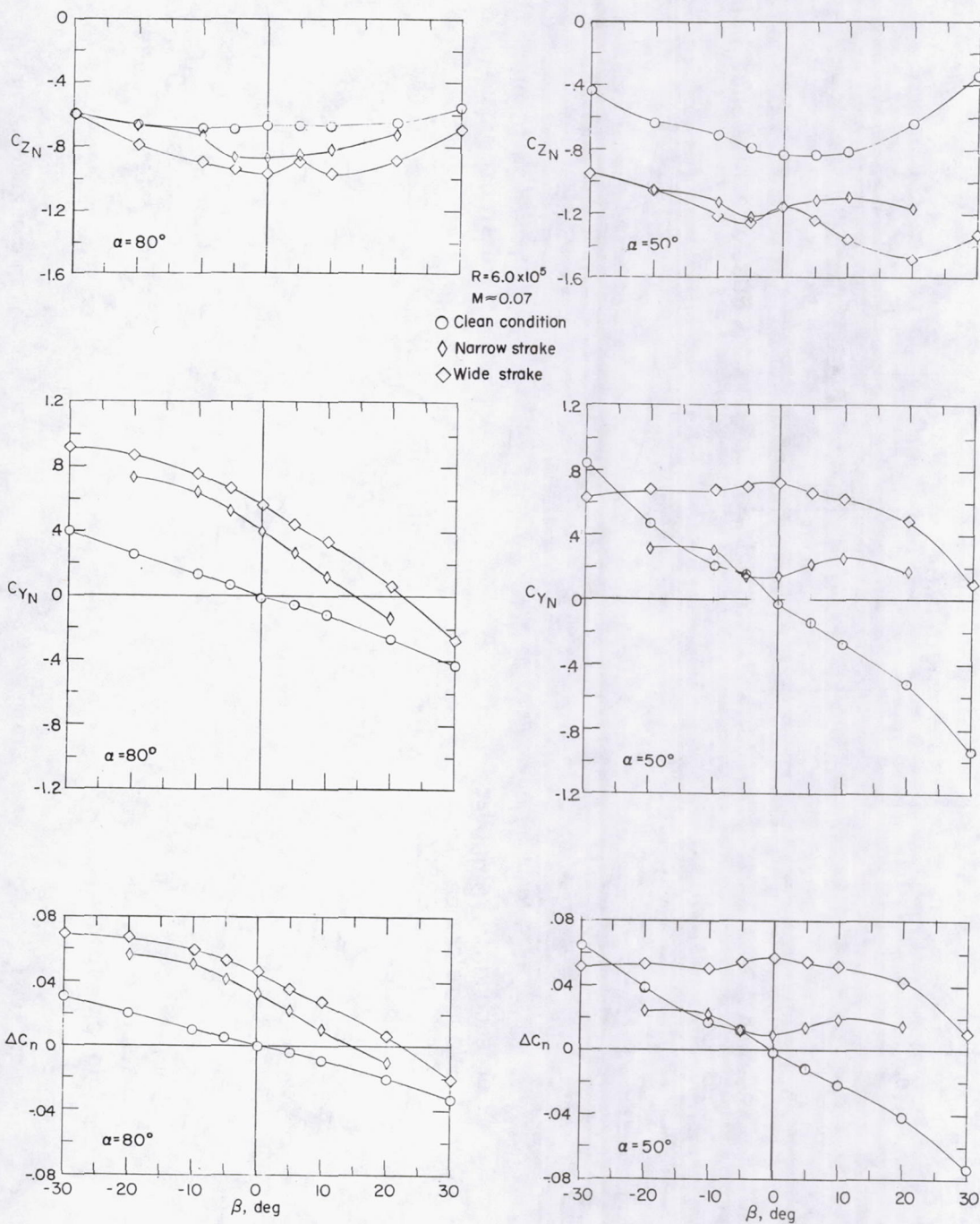
Figure 25.- Normal-force and side-force variation with angle of attack and sideslip on the nose of model 3, and the contribution of the nose of model 3 to the yawing moment about the center of gravity of the model.
