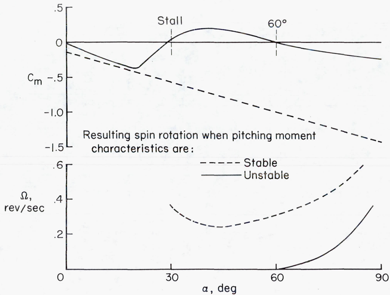
Figure 12.- Effective pitching-moment characteristics on rate of rotation at angle of attack in the spin.
