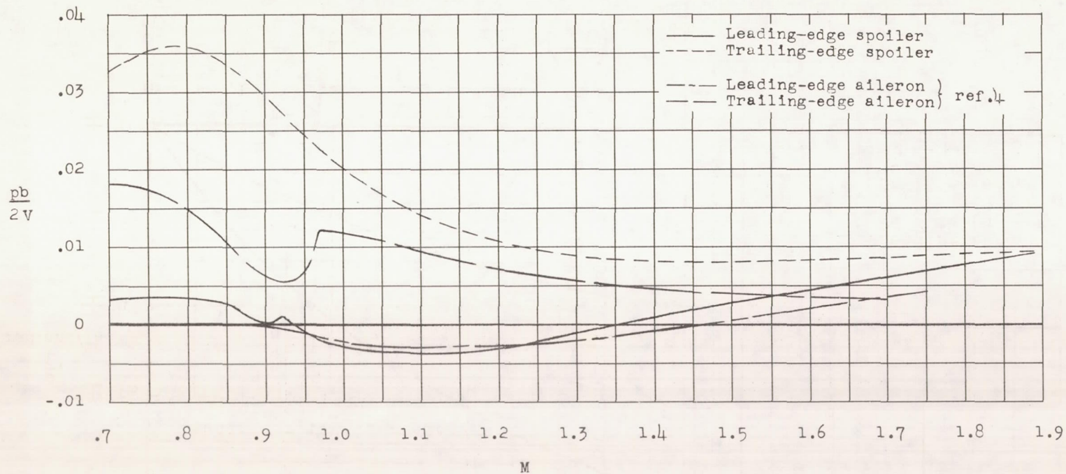
Figure 5.- Variation of rolling effectiveness of leading-edge and trailing-edge air-jet spoilers and ailerons (deflected 1^\circ ).
