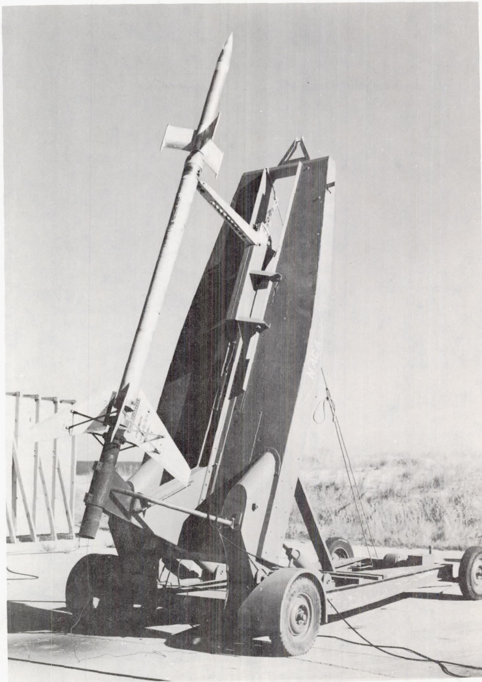
(e) Trailing-edge-spoiler model on launcher.
