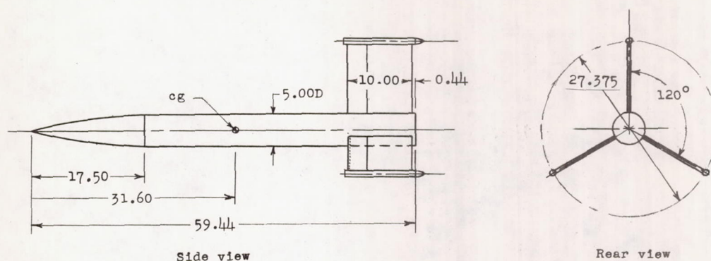
(a) Leading-edge jet-spoiler model.
