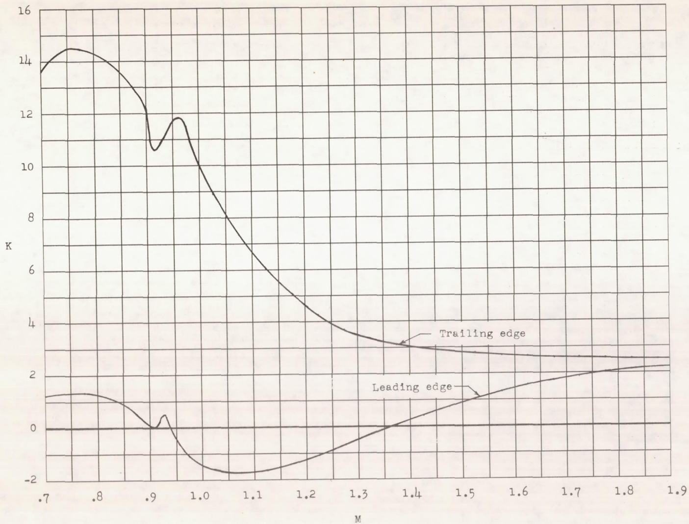
Figure 8.- Variation with Mach number of the magnification factor K for each model.
