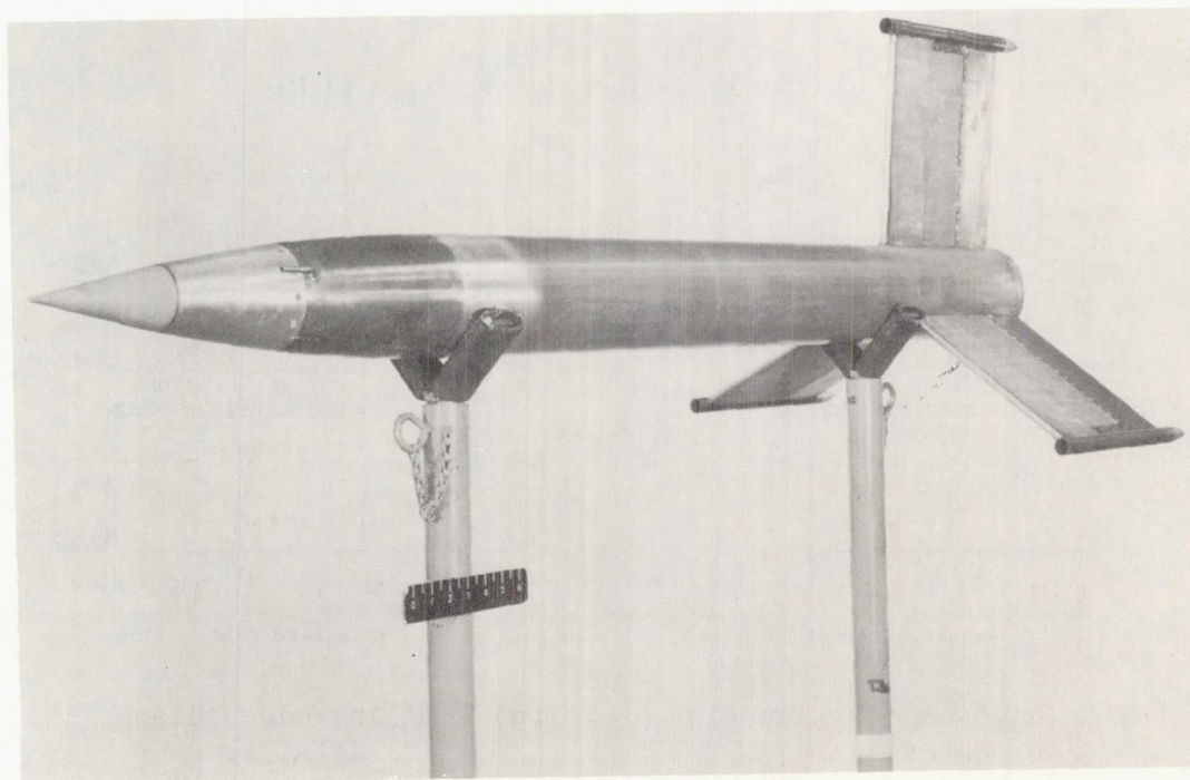
(b) Three-quarter front view of trailing-edge-spoiler model. L-57-1596
