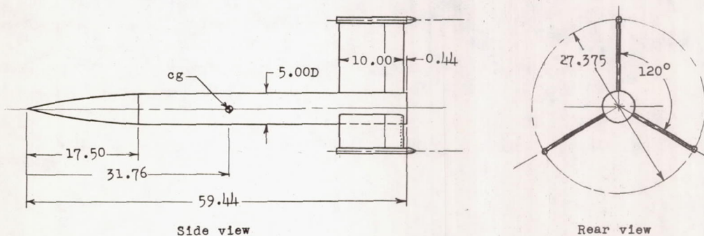
(b) Trailing-edge jet-spoiler model.
