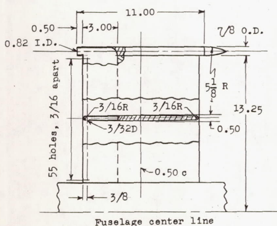
(c) Leading-edge jet-spoiler details.
