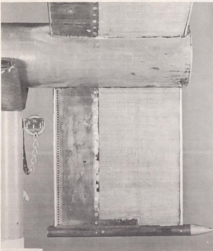
(c) Leading-edge-spoiler panel.
