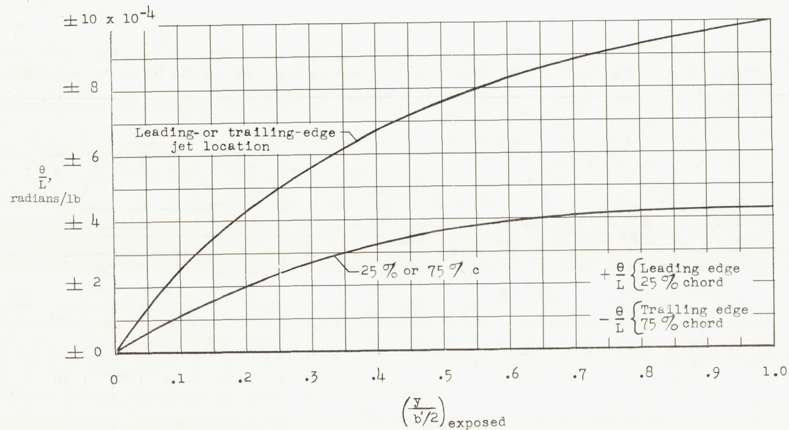
Figure 4.- Variation of wing twist with spanwise location for a uniform load distributed along the leading-edge and trailing-edge jet positions and the 25 percent and 75 percent chord lines.
