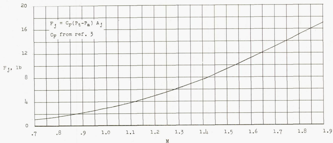
Figure 6.- Variation with Mach number of leading-edge and trailing-edge jet force per wing panel.
