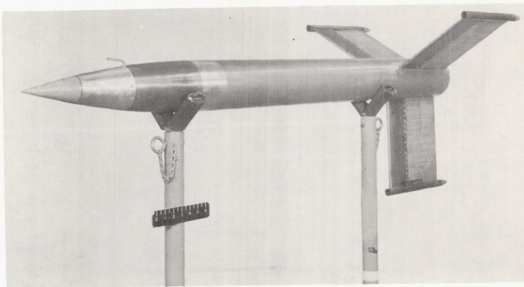
(a) Three-quarter front view of leading-edge-spoiler model.
