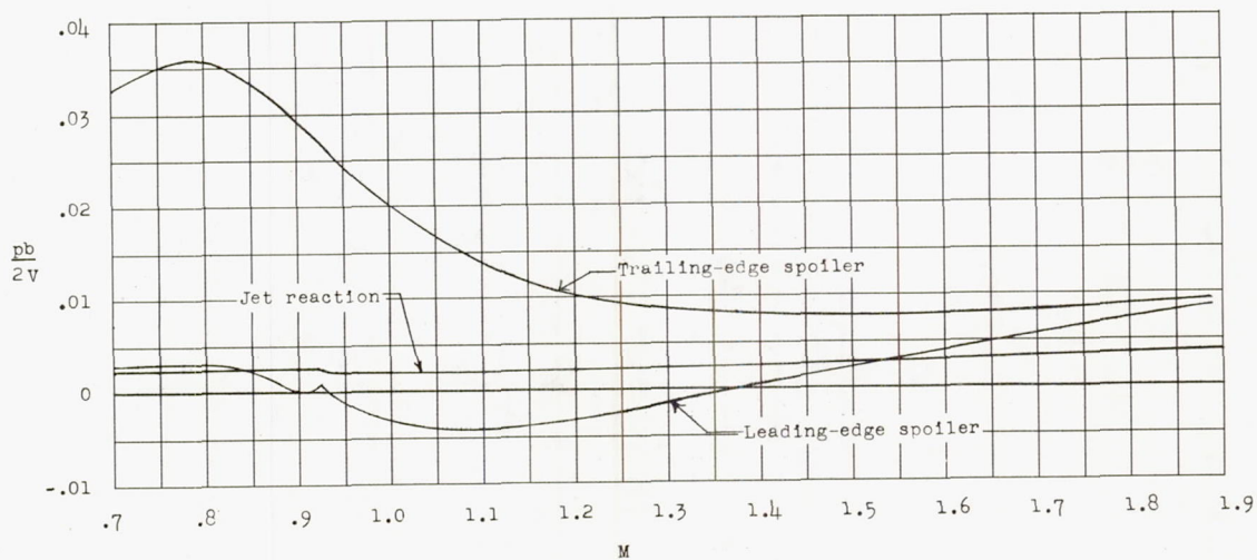
Figure 7.- Variation with Mach number of \frac{pb}{2V} of each model and \frac{pb}{2V} caused by jet reaction.
