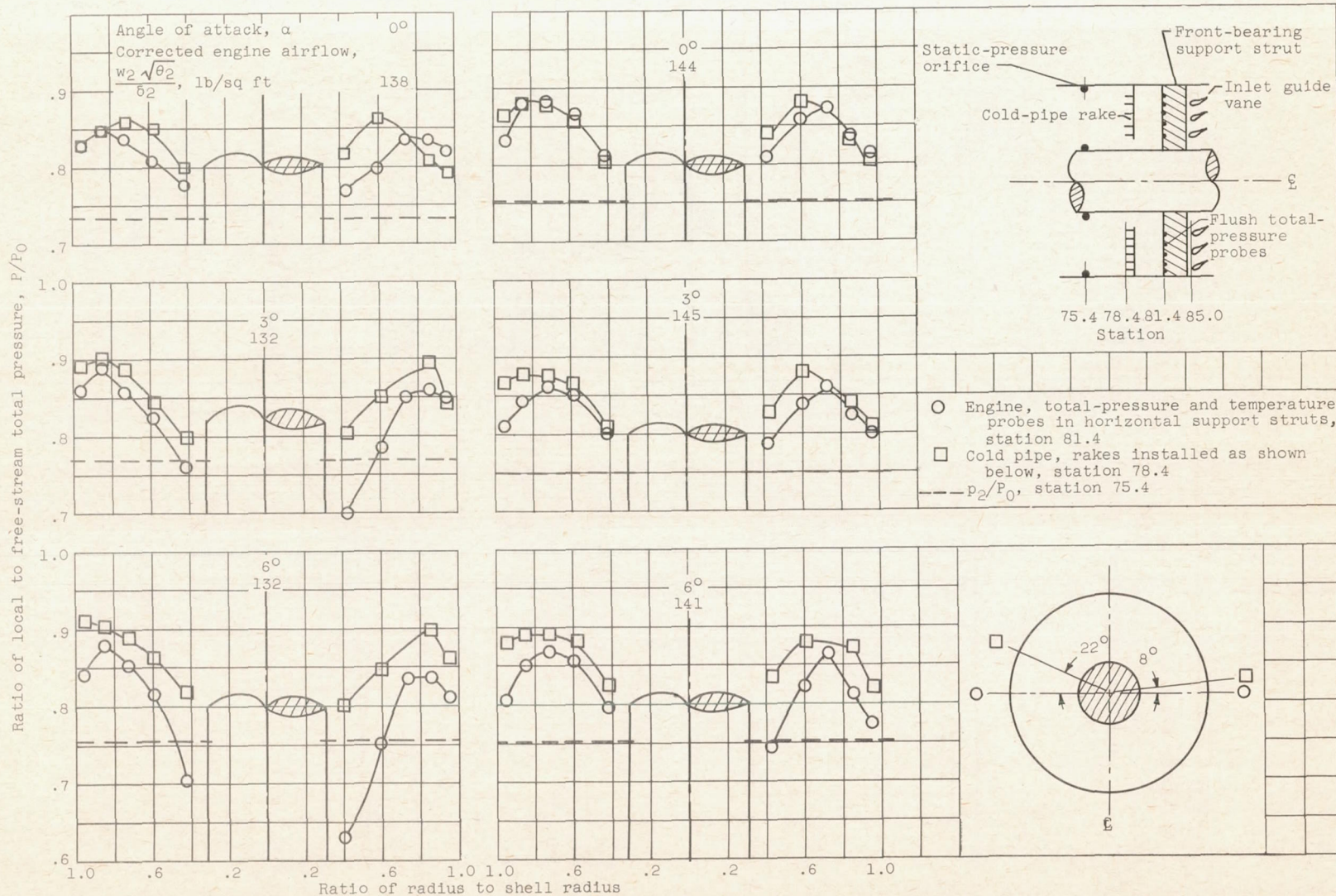
Figure 5. - Effect of engine installation on horizontal total-pressure profile. Slightly supercritical operation.
