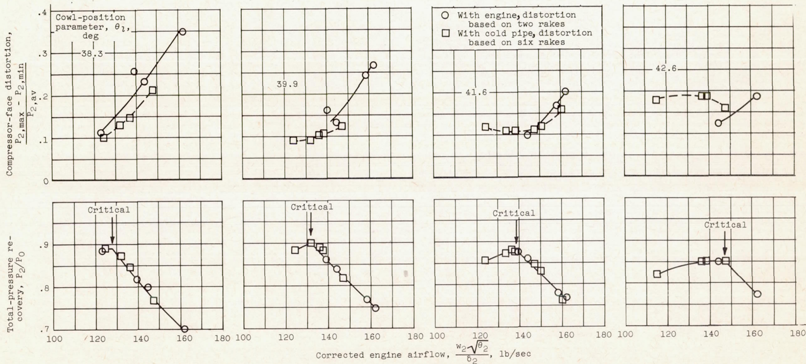
Figure 4. - Continued. Inlet performance.
