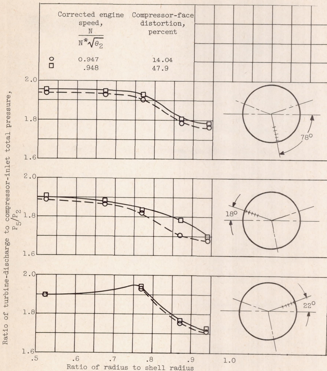
Figure 6. - Total-pressure profiles at turbine discharge.
