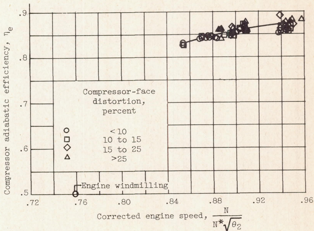
Figure 8. - Concluded. Engine performance.
