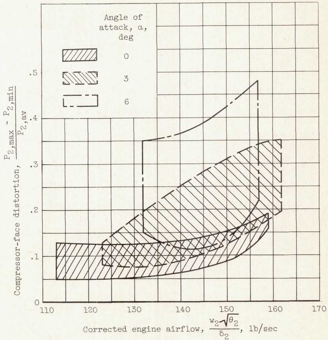
Figure 7. - Range of engine operating conditions.
