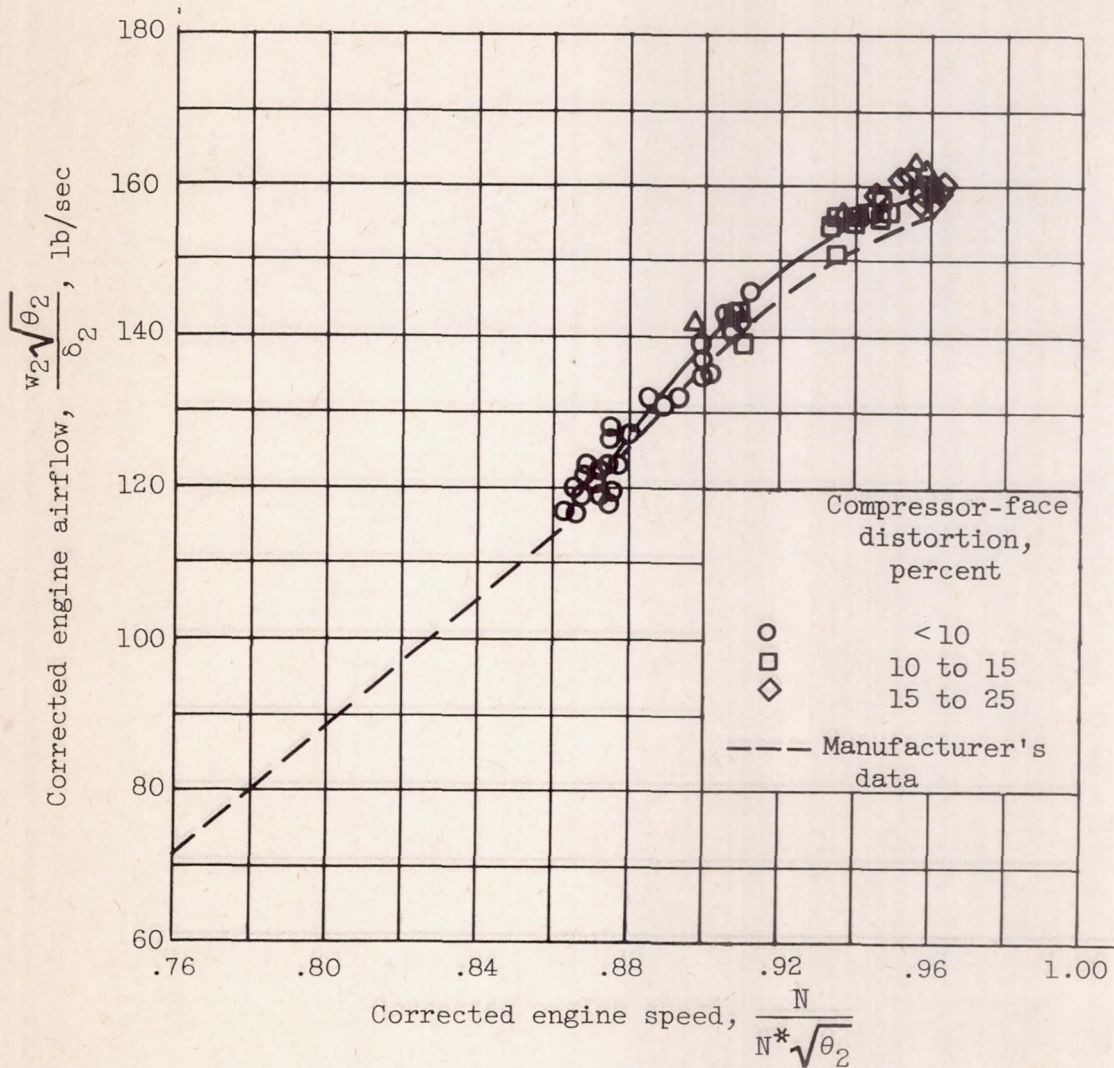
(a) Airflow.
