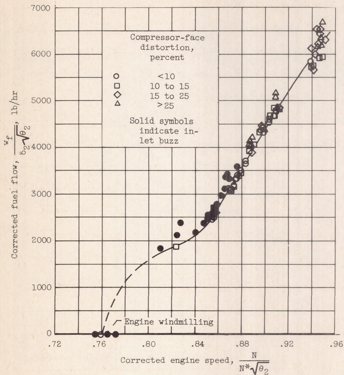
(c) Fuel flow.
