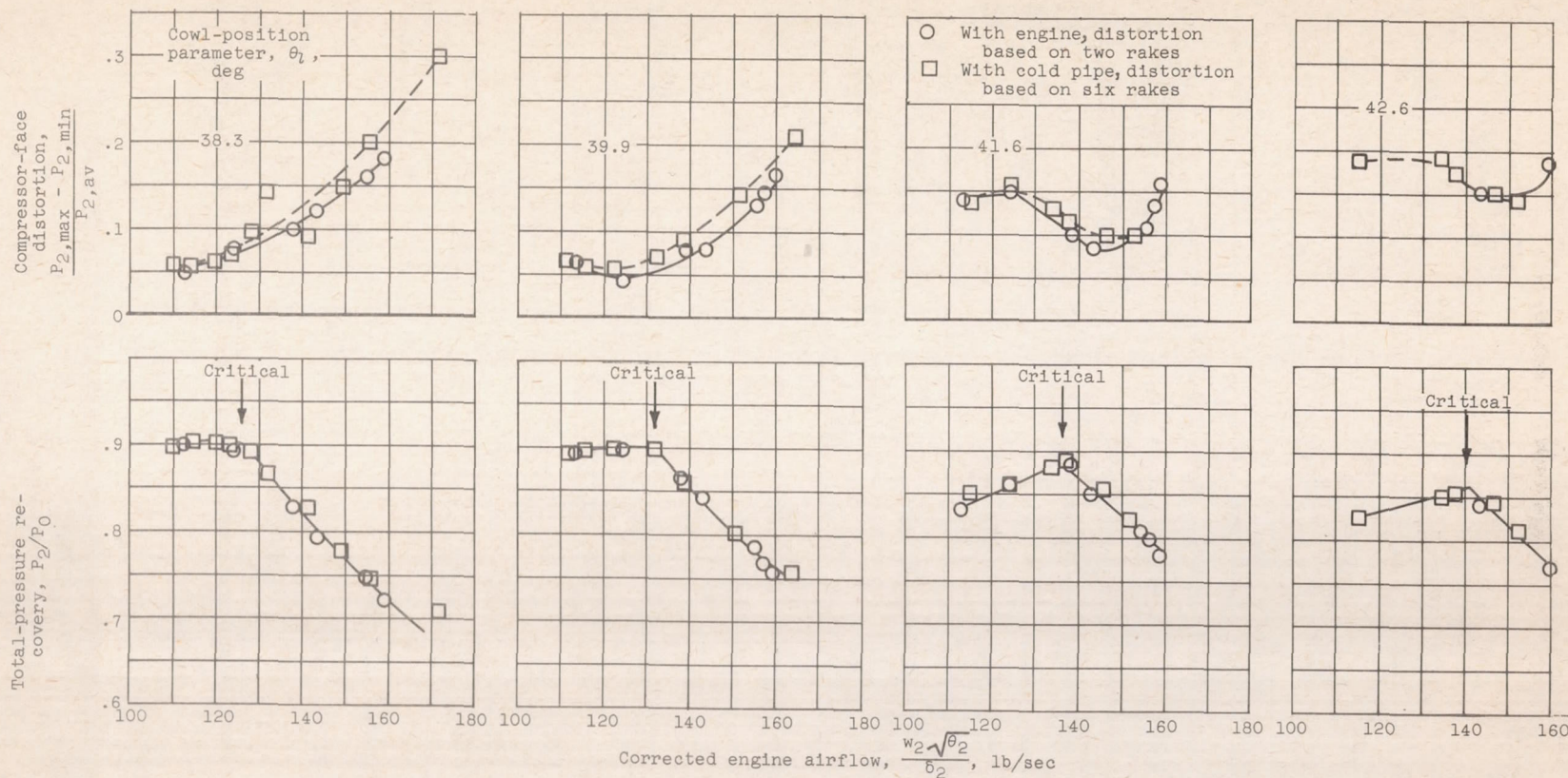
Figure 4. - Inlet performance.
