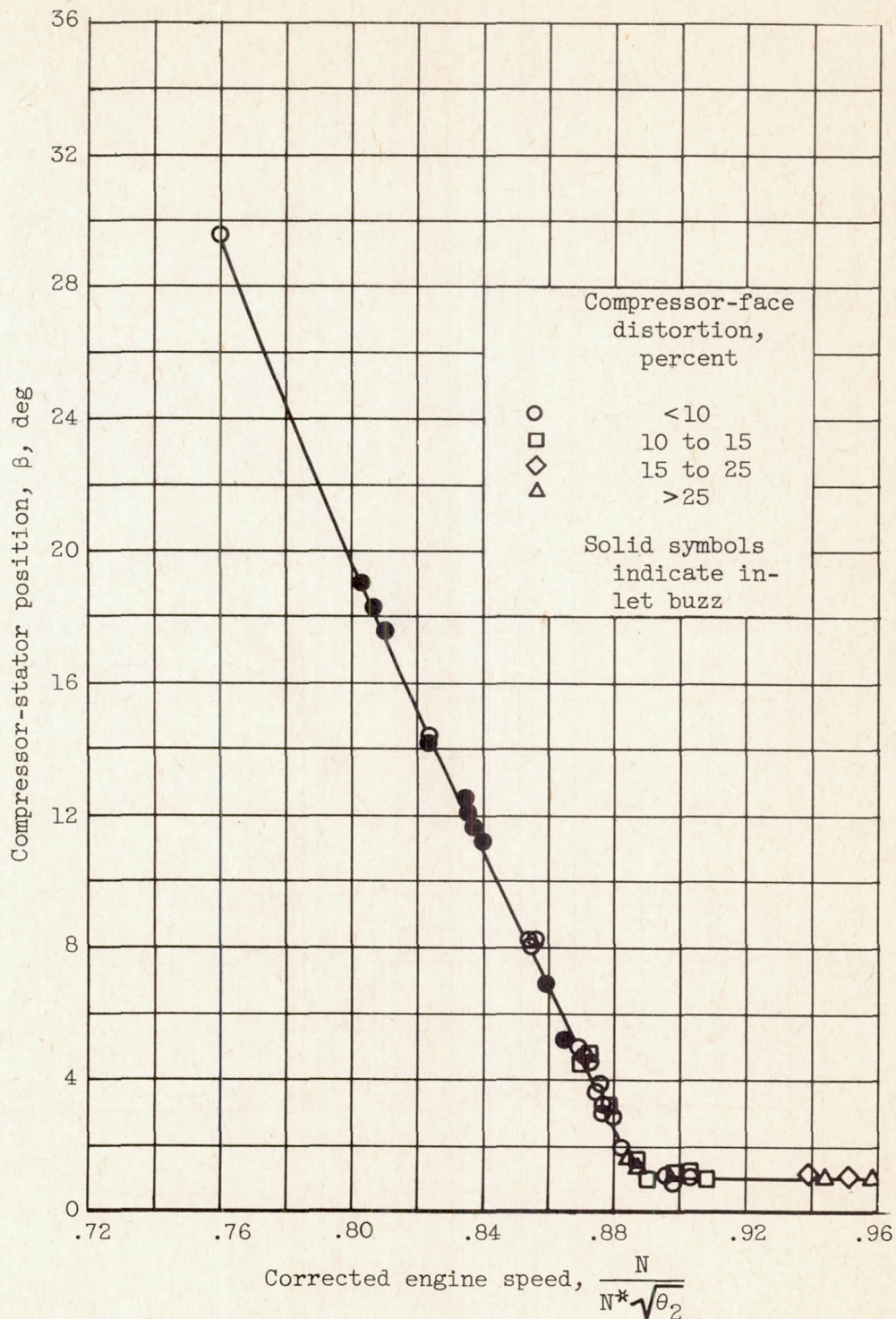
(b) Variation of compressor stators. Compressor-face temperature, 540° R.
