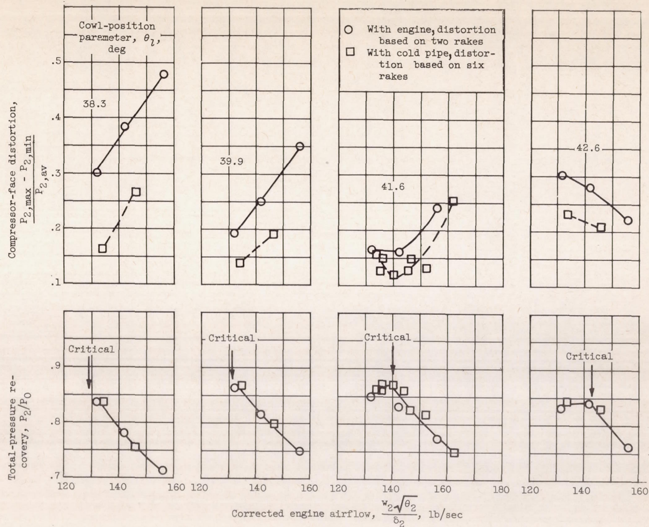
Figure 4. - Concluded. Inlet performance.
