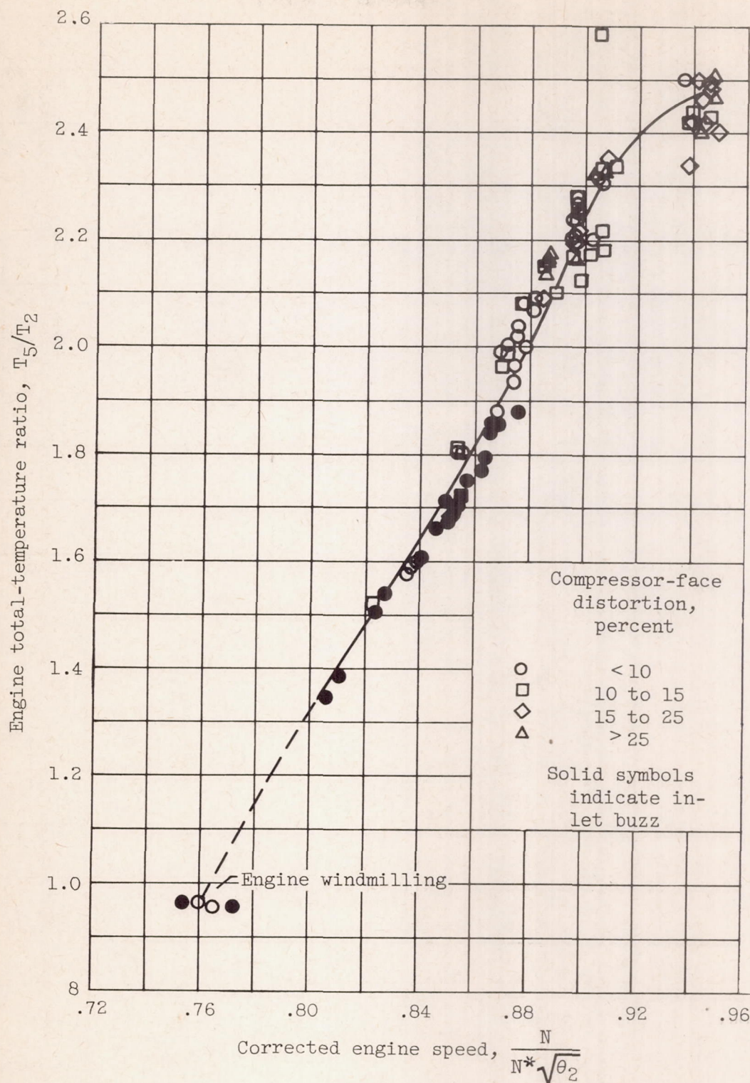
Figure 8. - Continued. Engine performance.
