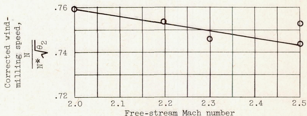
Figure 10. - Engine windmilling speed characteristics. Compressor-face temperature, 538° to 542° R.
