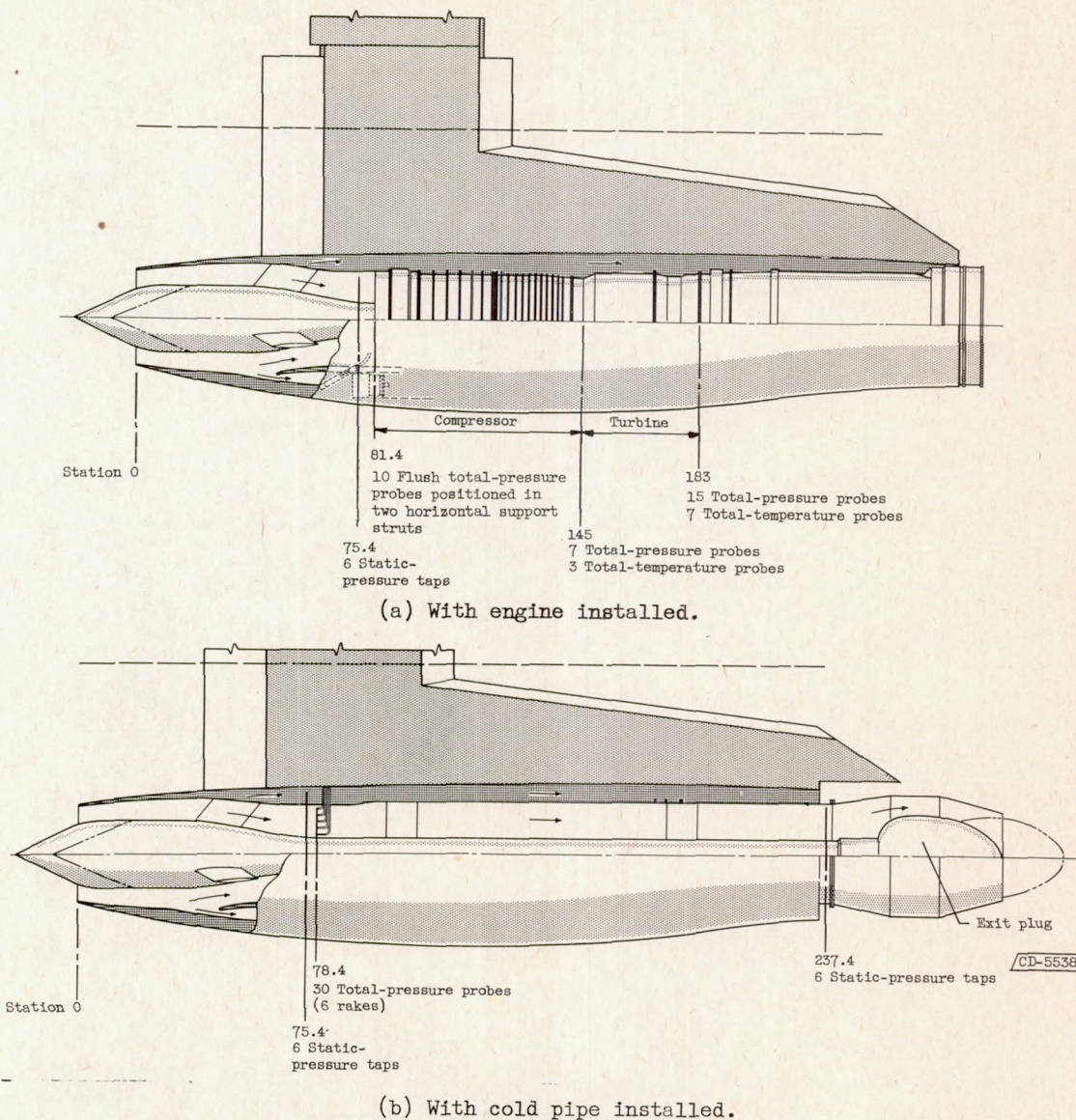
Figure 3. - Nacelle and instrumentation for engine and cold-pipe installations.
