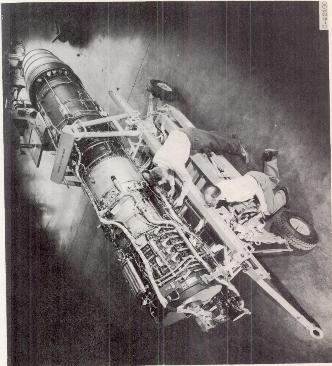
Figure 1. - Turbojet engine.
