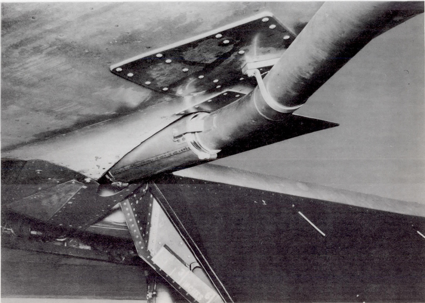
Figure 6.- View showing ducting at root of flap.
