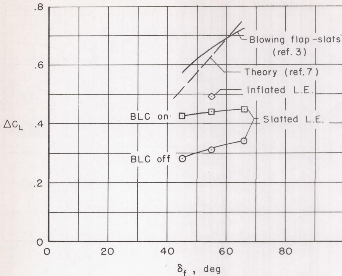
Figure 13.- Variation of flap lift increment with flap deflection; 80 percent engine rpm, \alpha = 8^\circ .
