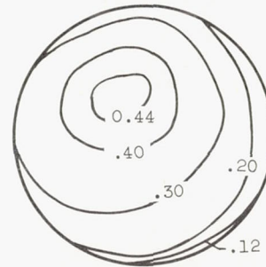
Diffuser total-pressure recovery, P_z/P_0 , 0.459; average Mach number, M_{av} , 0.317; profile factor, \Delta M/M_{av} , 0.211; continuity Mach number, M_{con} , 0.294.
