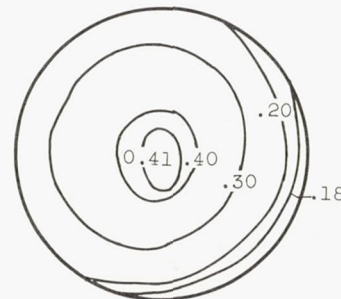
Diffuser total-pressure recovery, P_z/P_0 , 0.484; average Mach number, M_{av} , 0.297; profile factor, \Delta M/M_{av} , 0.201; continuity Mach number, M_{con} , 0.276.
