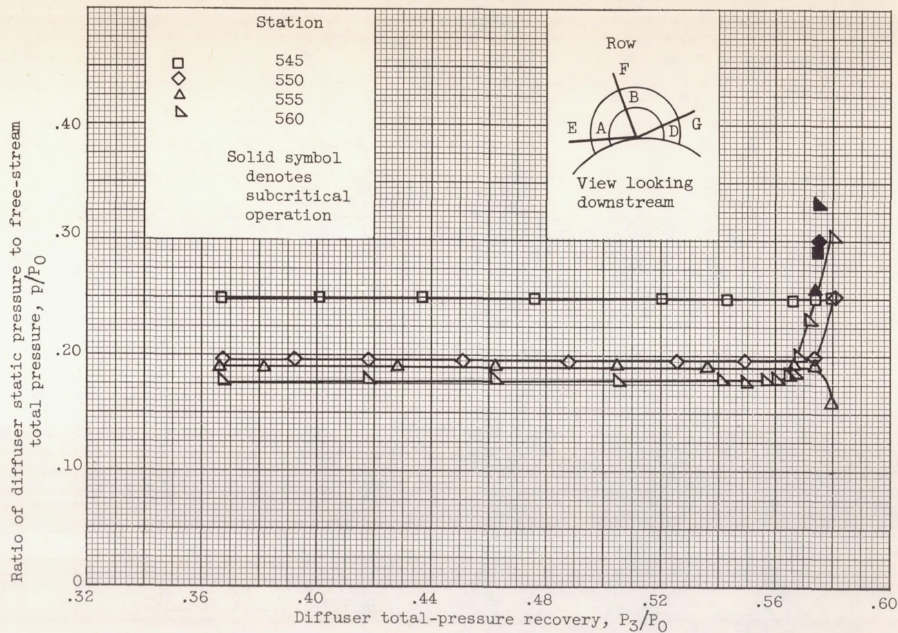
(f) Instrumentation row G (cowl).
