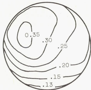
Diffuser total-pressure recovery, P_z/P_0 , 0.540; average Mach number, M_{av} , 0.255; profile factor, \Delta M/M_{av} , 0.213; continuity Mach number, M_{con} , 0.246.
