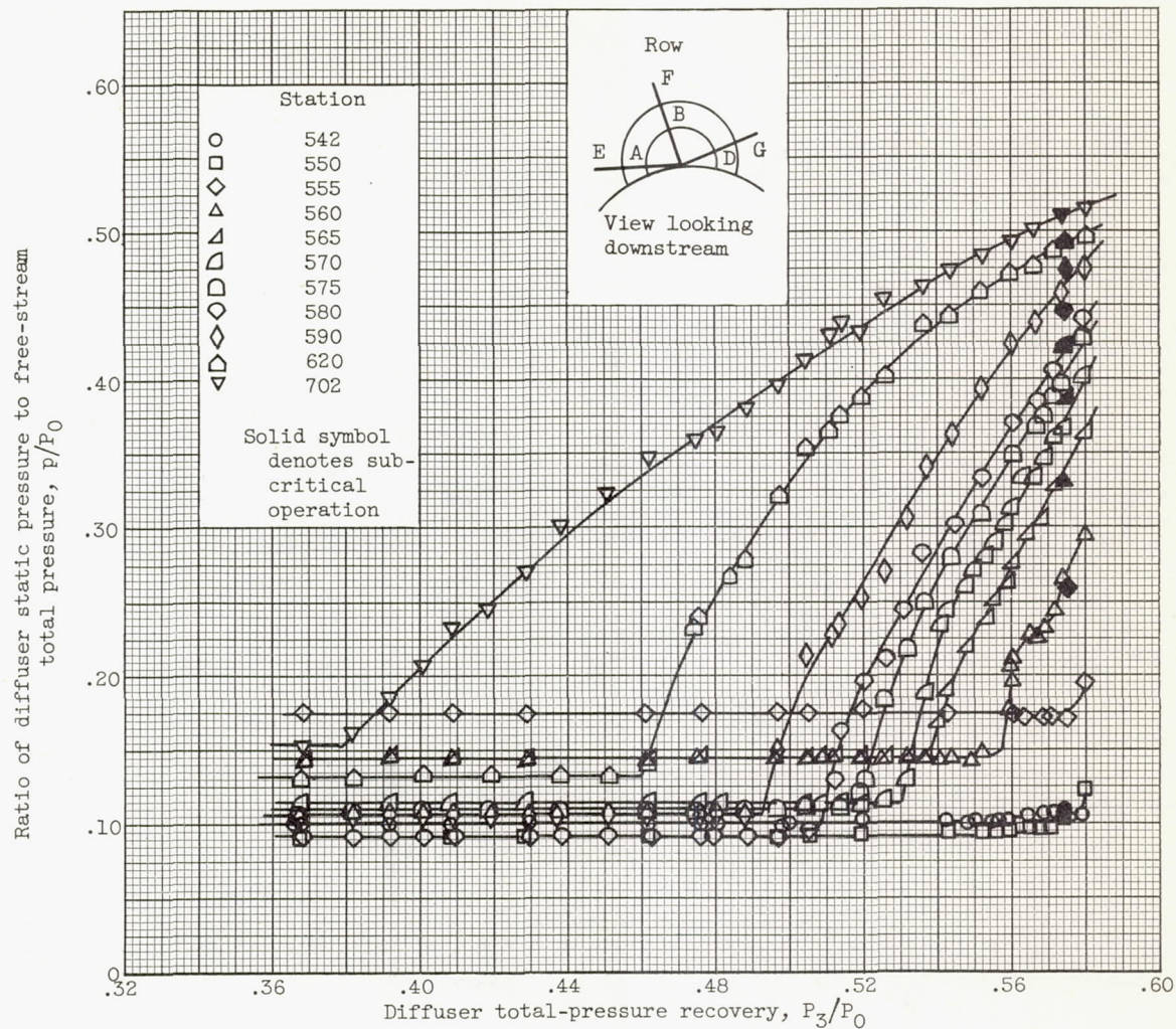
(a) Instrumentation row B (inner body).
