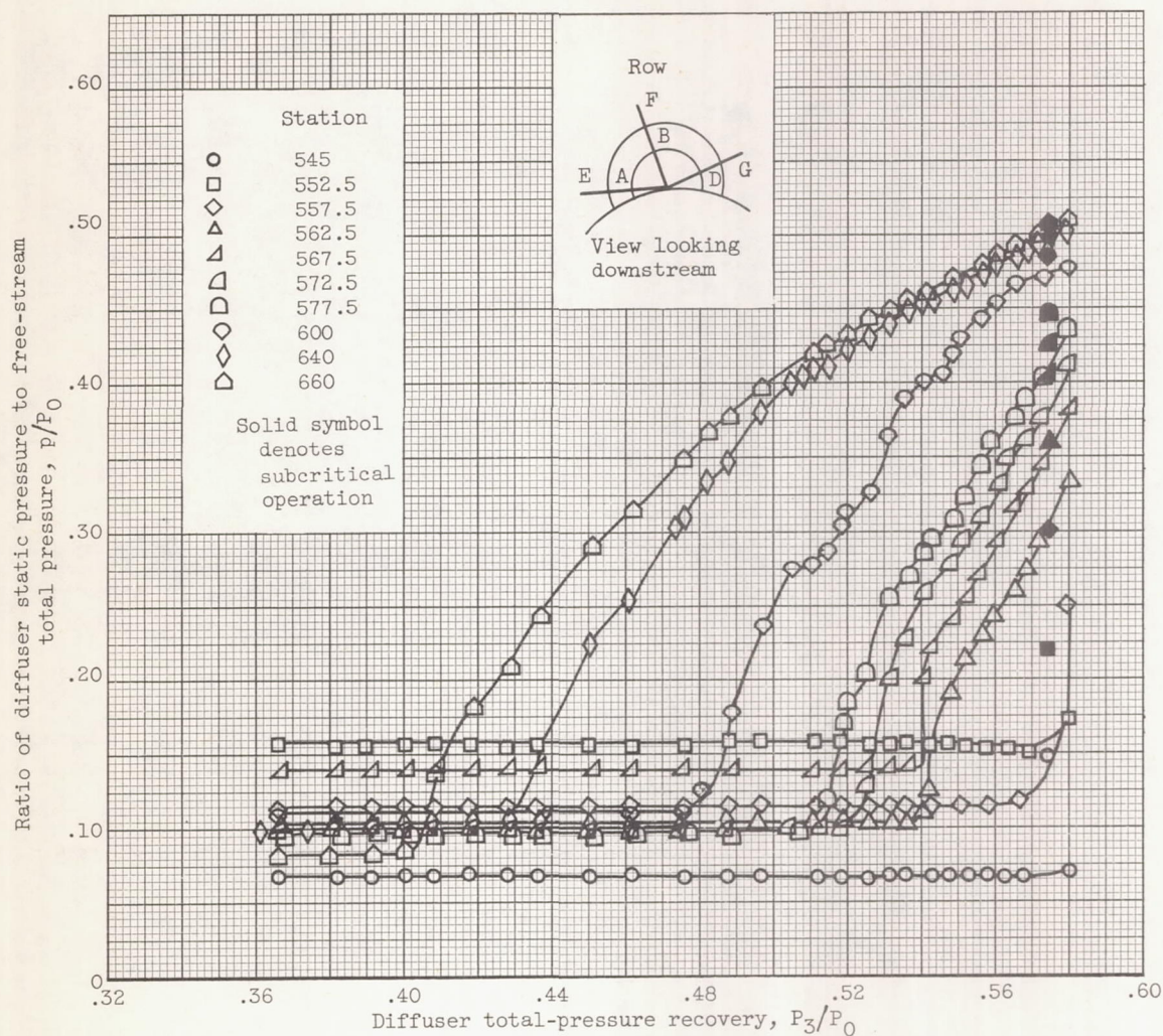
(a) Concluded. Instrumentation row B (inner body).
