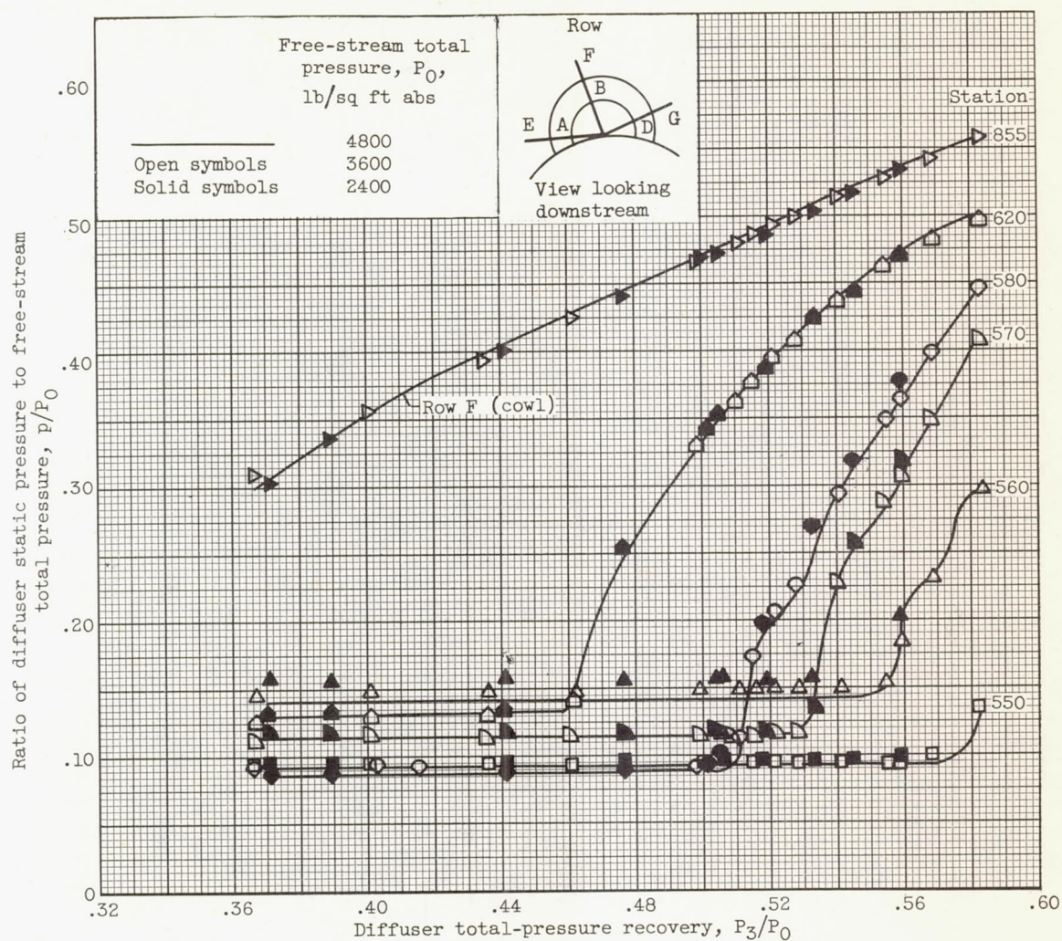
Figure 8. - The effect of free-stream total pressure on the variation of internal-diffuser wall static pressures presented as ratios to free-stream total pressure with diffuser total-pressure recovery under cold-flow conditions (combustor not operating). Row B (inner body). Free-stream total temperature, 760° F.
