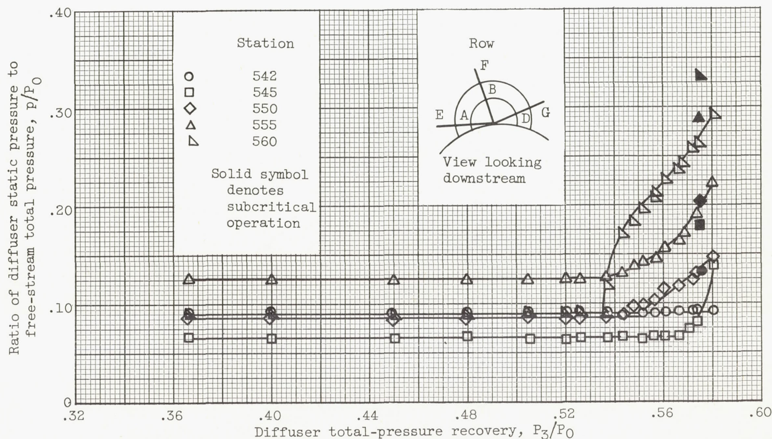
(c) Instrumentation row A (inner body).
