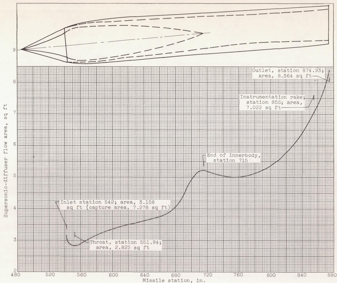
Figure 3. - Diffuser area variation.
