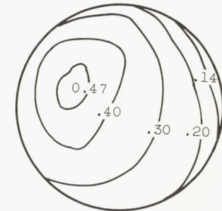
Diffuser total-pressure recovery, P_z/P_0 , 0.448; average Mach number, M_{av} , 0.328; profile factor, \Delta M/M_{av} , 0.230; continuity Mach number, M_{con} , 0.302.
