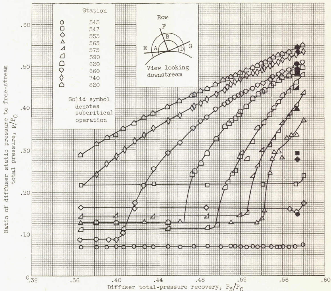
(b) Instrumentation row F (cowl).
