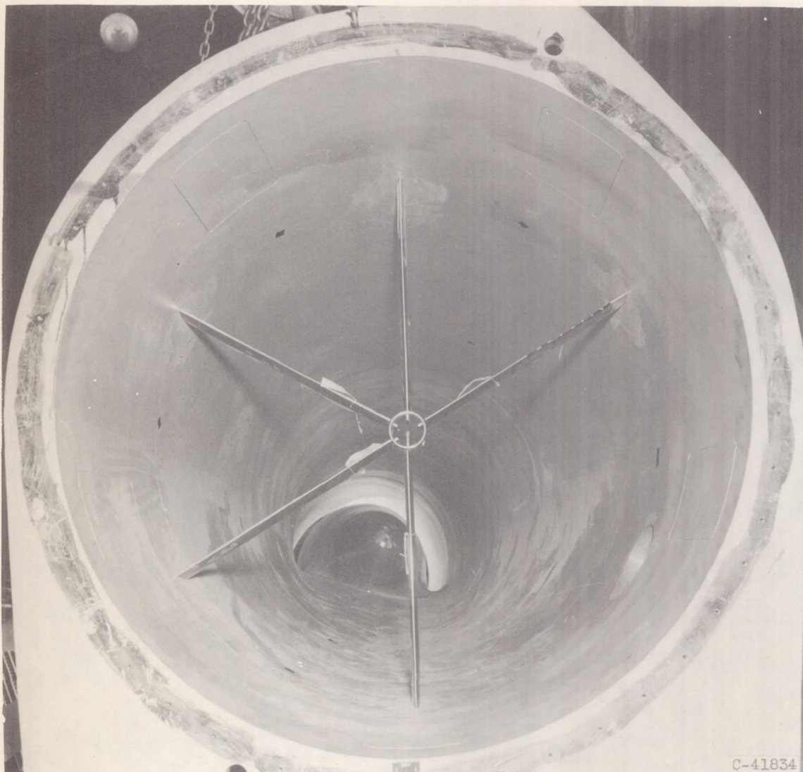
(b) View looking upstream through diffuser duct.
