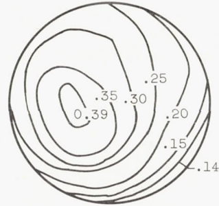
Diffuser total-pressure recovery, P_z/P_0 , 0.506; average Mach number, M_{av} , 0.273; profile factor, \Delta M/M_{av} , 0.213; continuity Mach number, M_{con} , 0.264.
