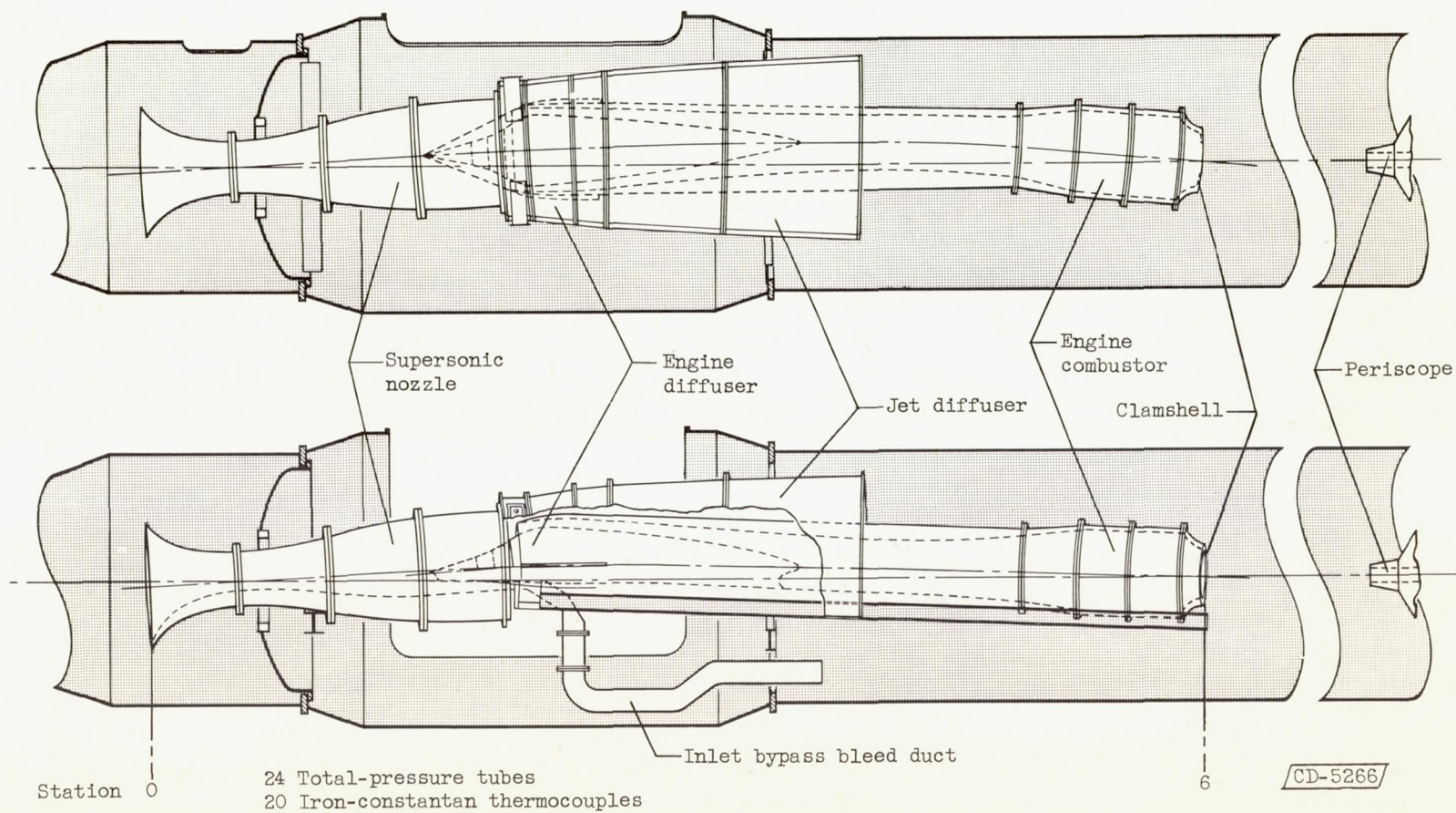
Figure 4. - Free-jet test facility and engine installation.
