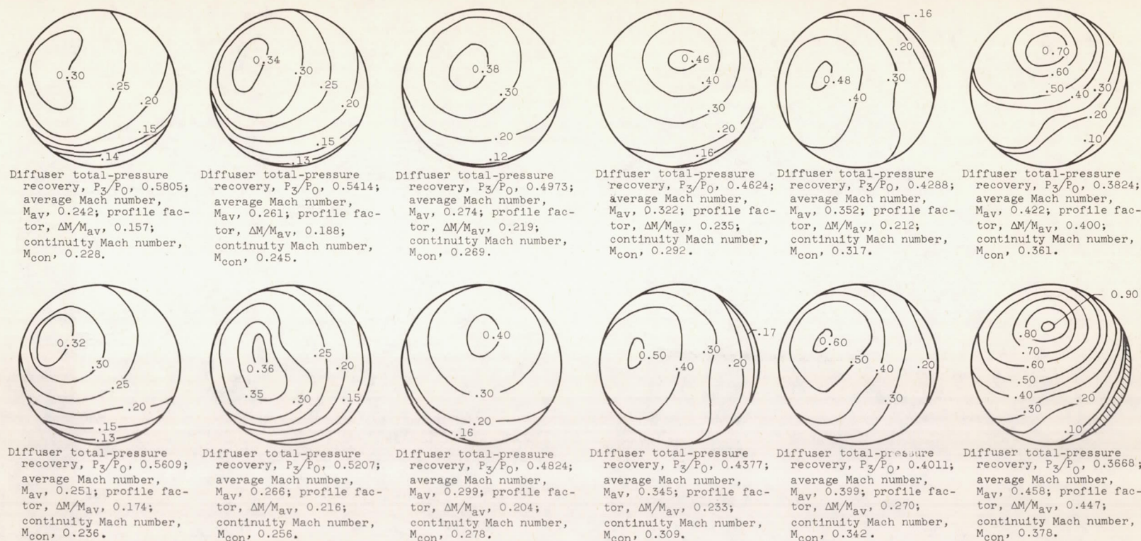
Figure 11. - Diffuser Mach-number contours for various diffuser total-pressure recoveries with average Mach number, continuity Mach number, and flow profile factor at missile station 855 (station 3). View looking downstream. Free-stream total pressure, 4800 pounds per square foot absolute; free-stream total temperature, 760° F.
