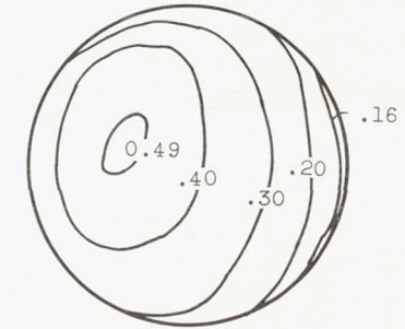
Diffuser total-pressure recovery, P_z/P_0 , 0.437; average Mach number, M_{av} , 0.343; profile factor, \Delta M/M_{av} , 0.215; continuity Mach number, M_{con} , 0.310.
