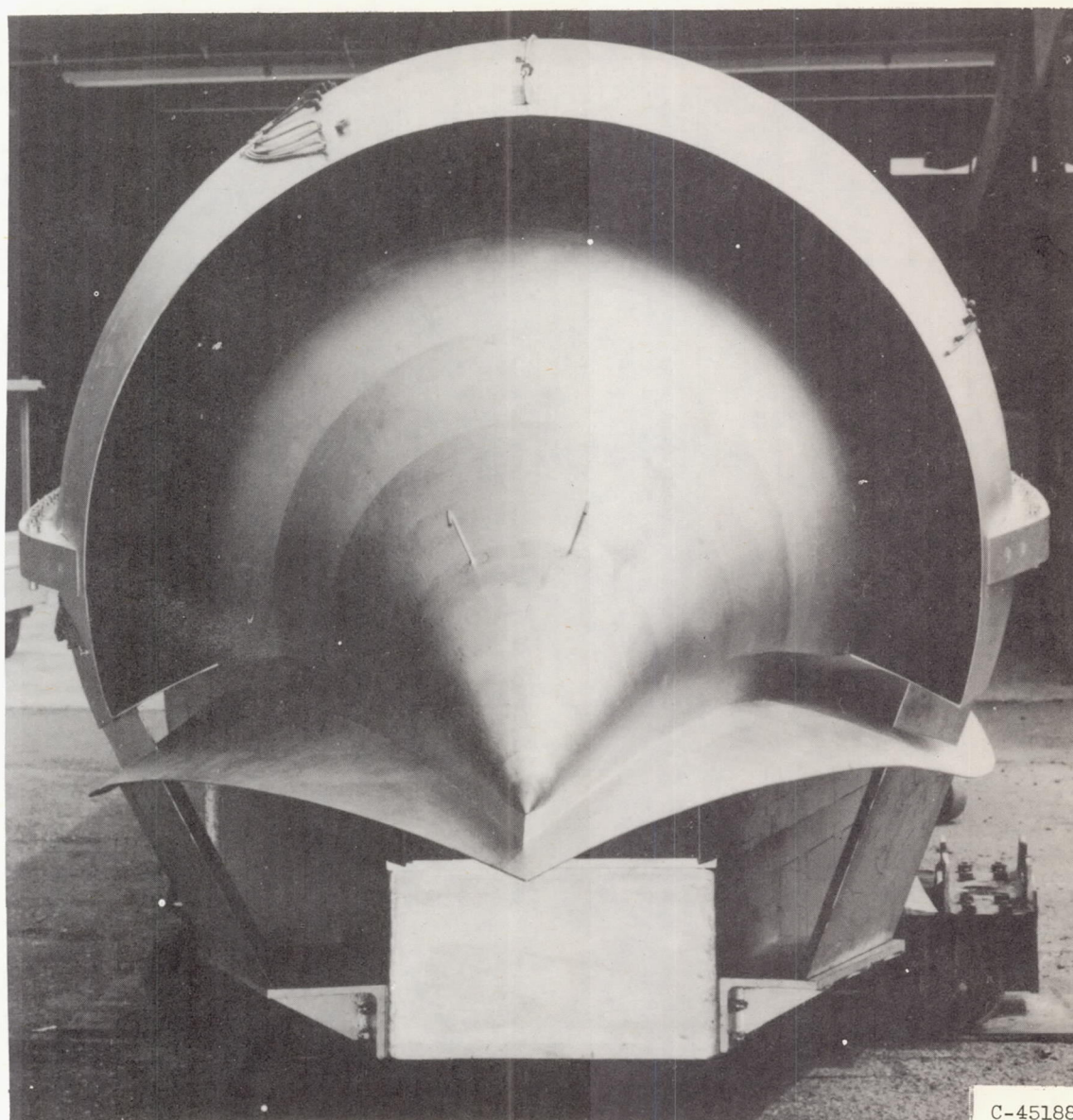
(a) Diffuser inlet.
