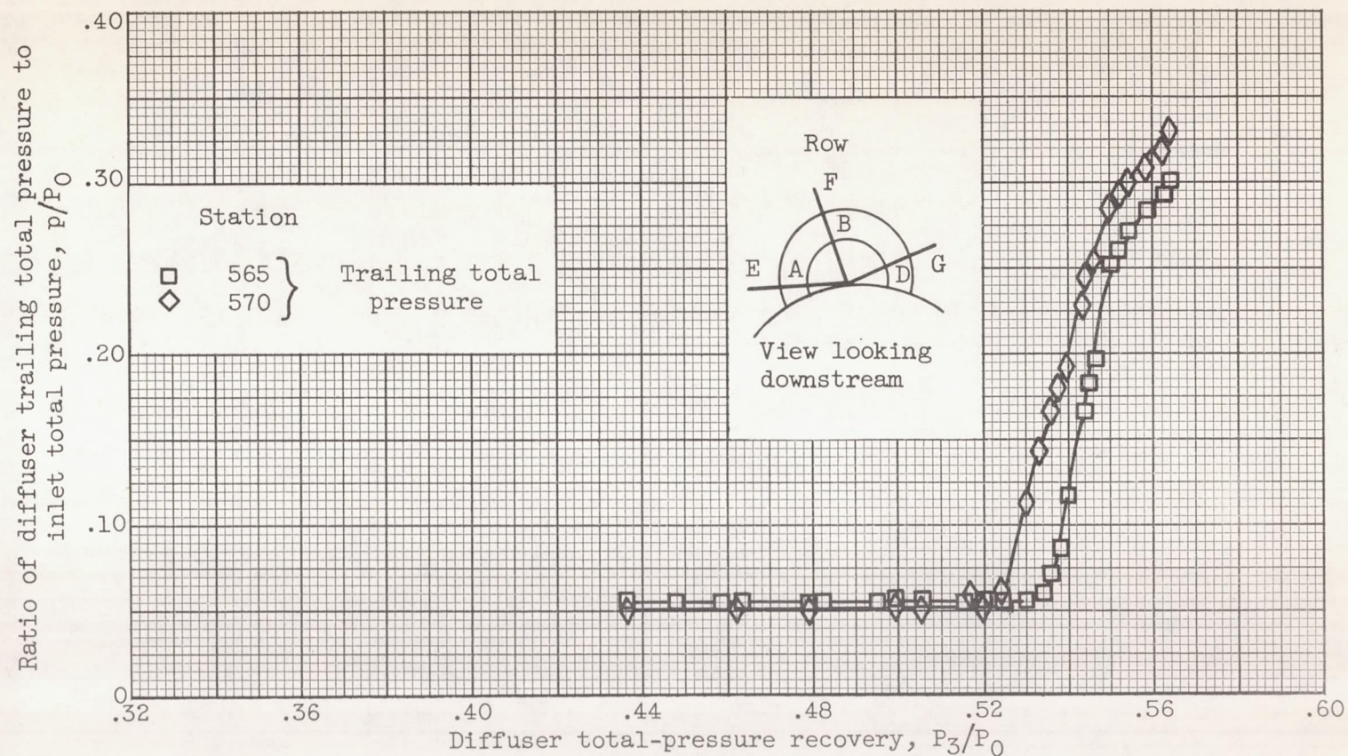
(b) Hot-flow conditions (combustor operating).
