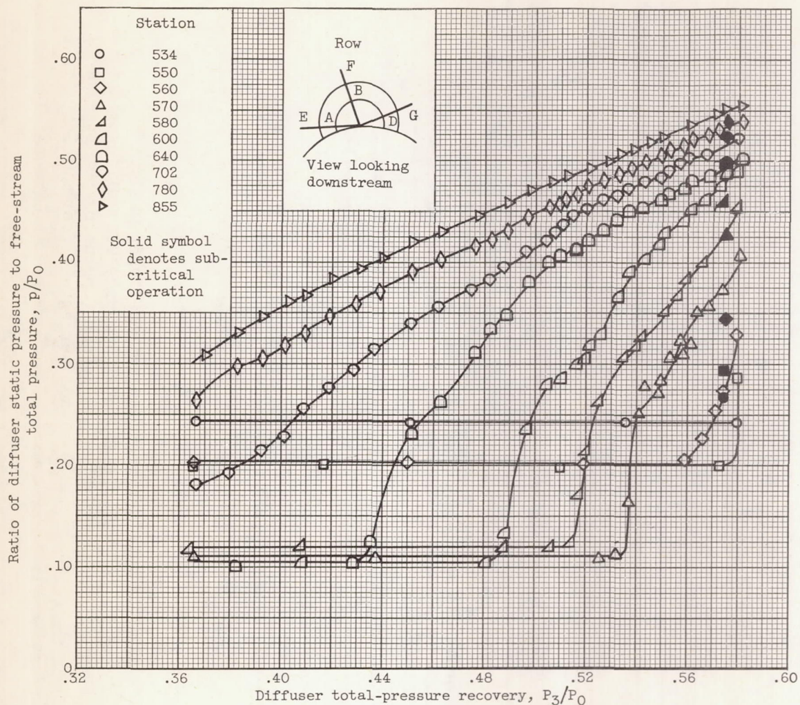
(b) Concluded. Instrumentation row F (cowl).
