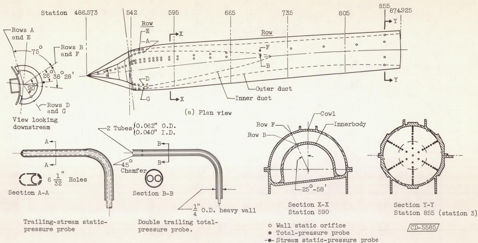
(b) Diffuser instrumentation stations
