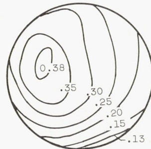
Diffuser total-pressure recovery, P_z/P_0 , 0.520; average Mach number, M_{av} , 0.276; profile factor, \Delta M/M_{av} , 0.204; continuity Mach number, M_{con} , 0.256.
