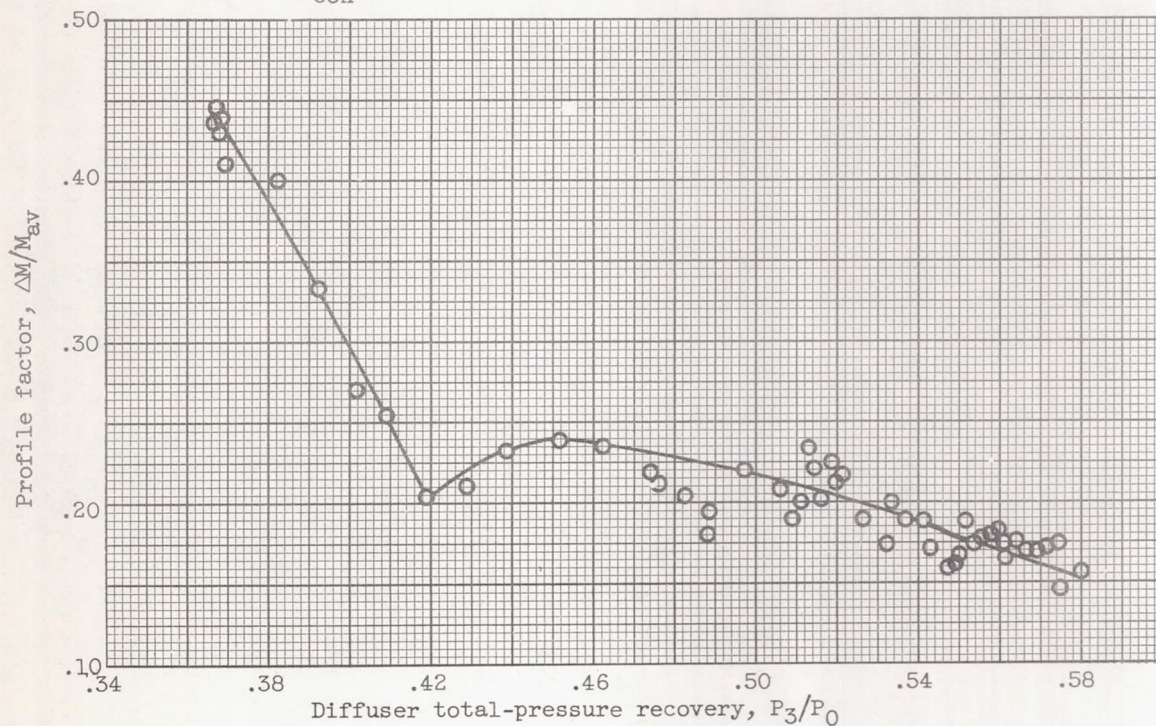
(b) Variation of flow profile factor \frac{\Delta M}{M_{av}} .
