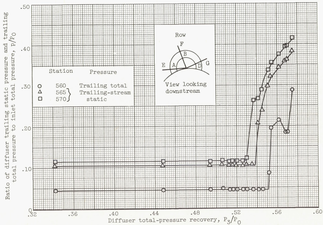
(a) Cold-flow conditions (combustor not operating).
