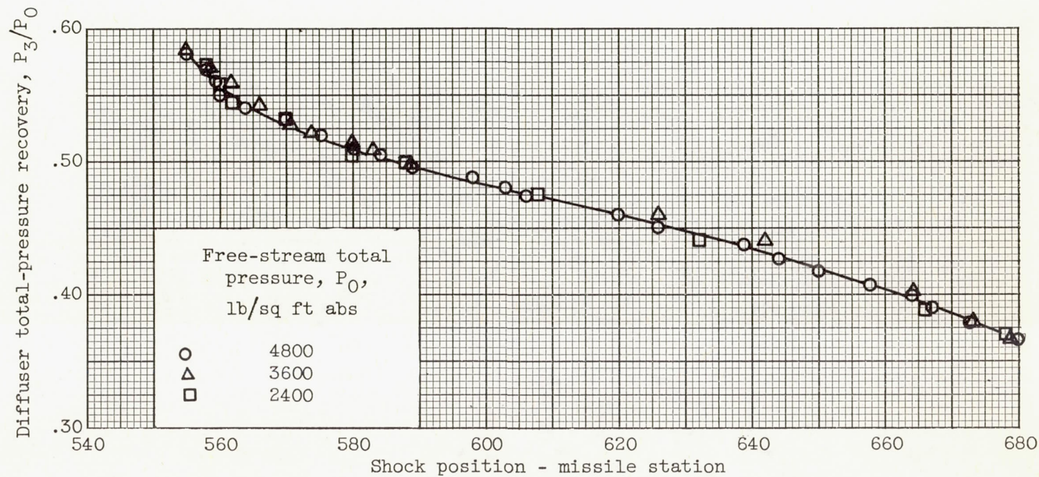
Figure 10. - Relationship between diffuser total-pressure recovery and internal-shock position based on wall static pressures of instrumentation row B (inner body). Free-stream total-pressure effect under cold-flow conditions (combustor not operating).
