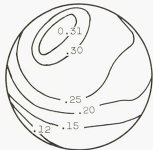
Diffuser total-pressure recovery, P_z/P_0 , 0.564; average Mach number, M_{av} , 0.238; profile factor, \Delta M/M_{av} , 0.200; continuity Mach number, M_{con} , 0.234.
