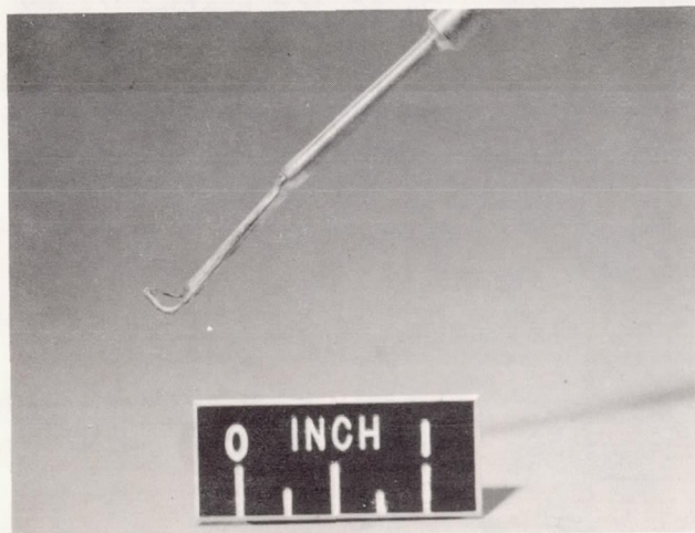
(a) Total-pressure, total-temperature, and angle probe.
