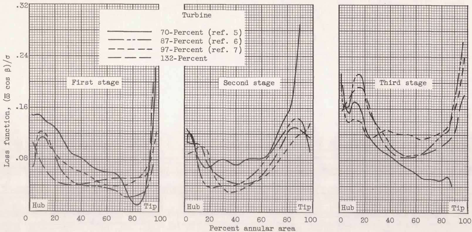
Figure 6. - Variation of loss function with annular flow area.
