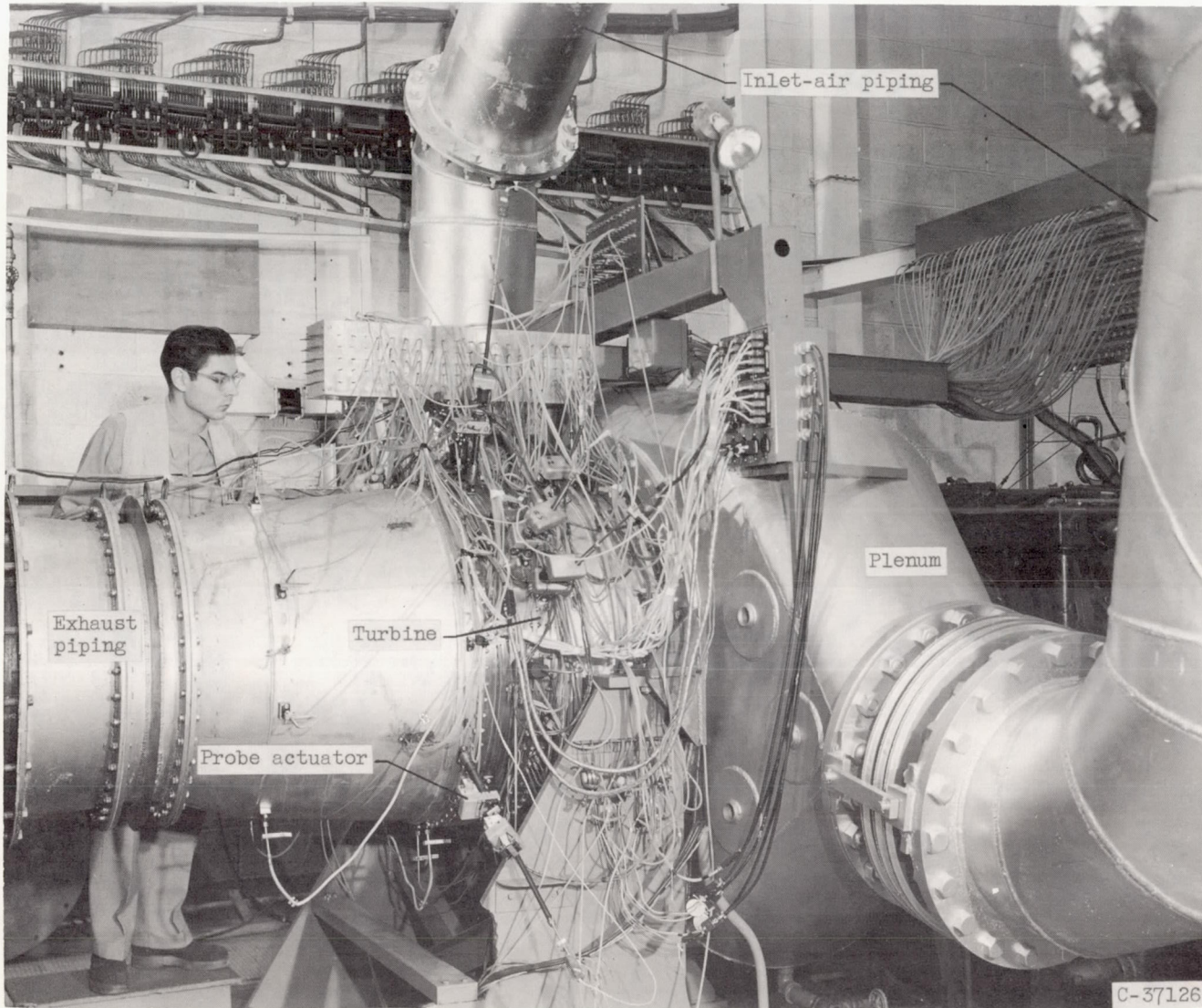
Figure 1. - Installation of J71-132 experimental three-stage turbine in full-scale turbine-component test facility.
