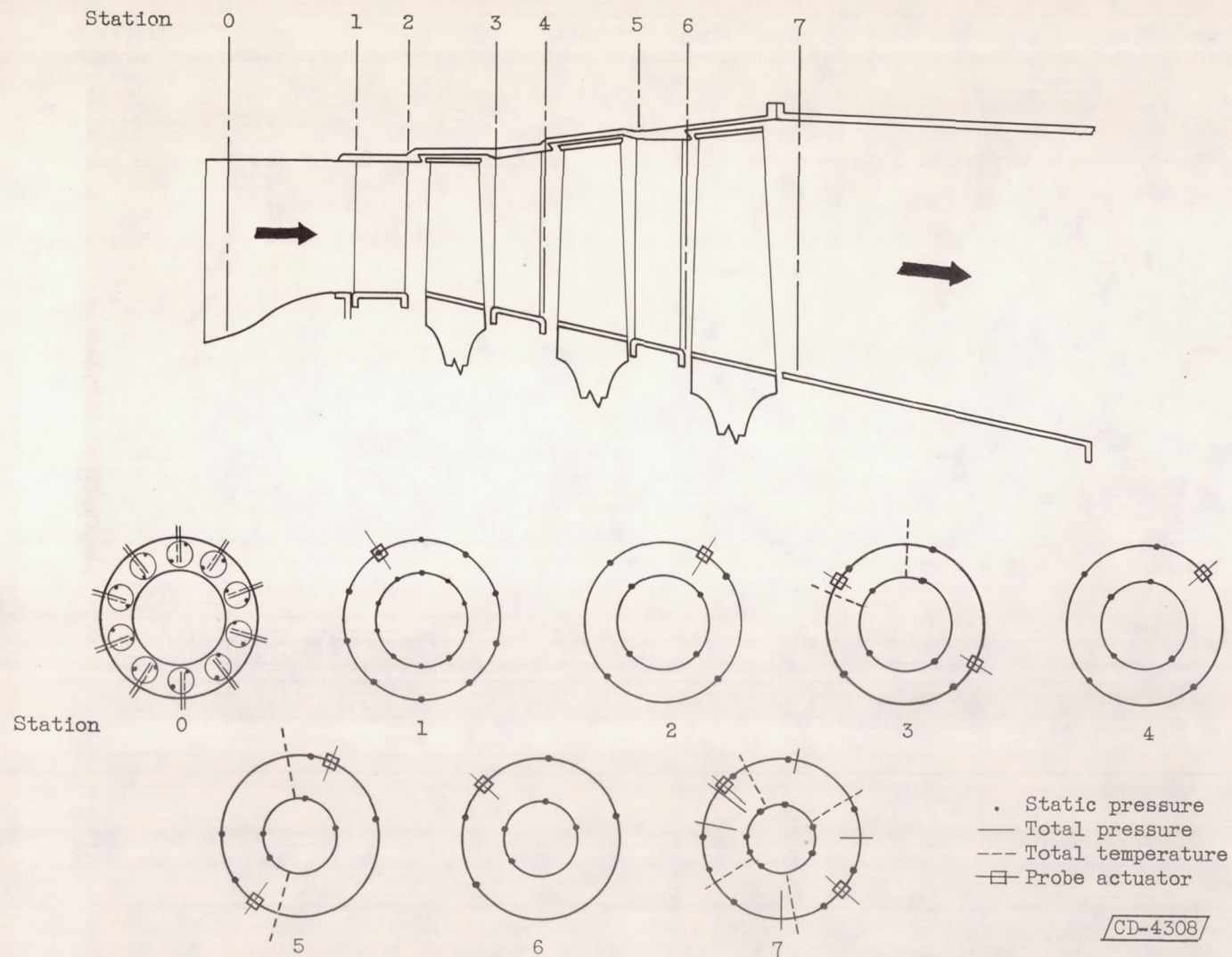
Figure 2. - Schematic diagram of J71-132 turbine showing instrumentation.
