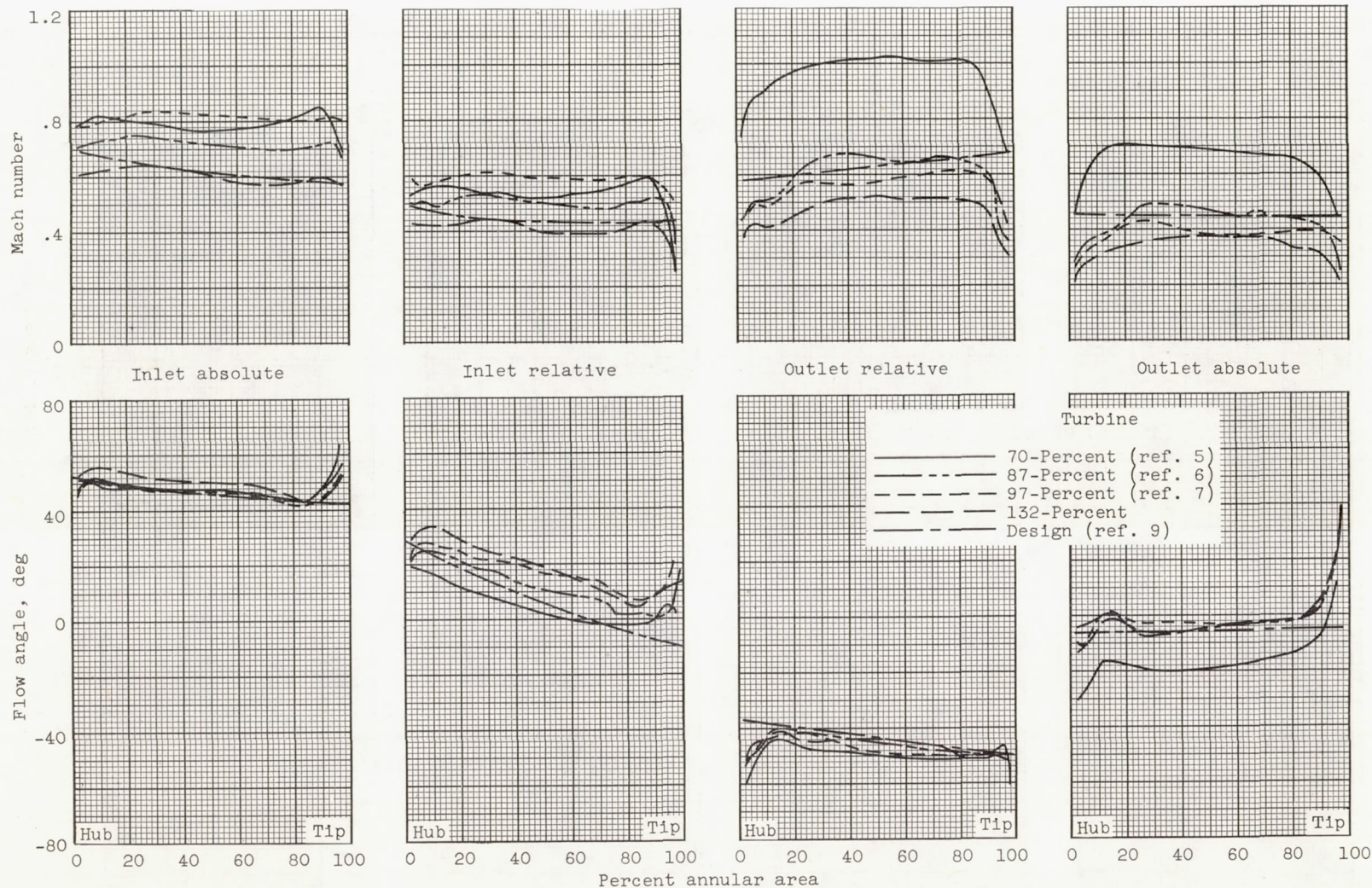
(c) Third rotor.
