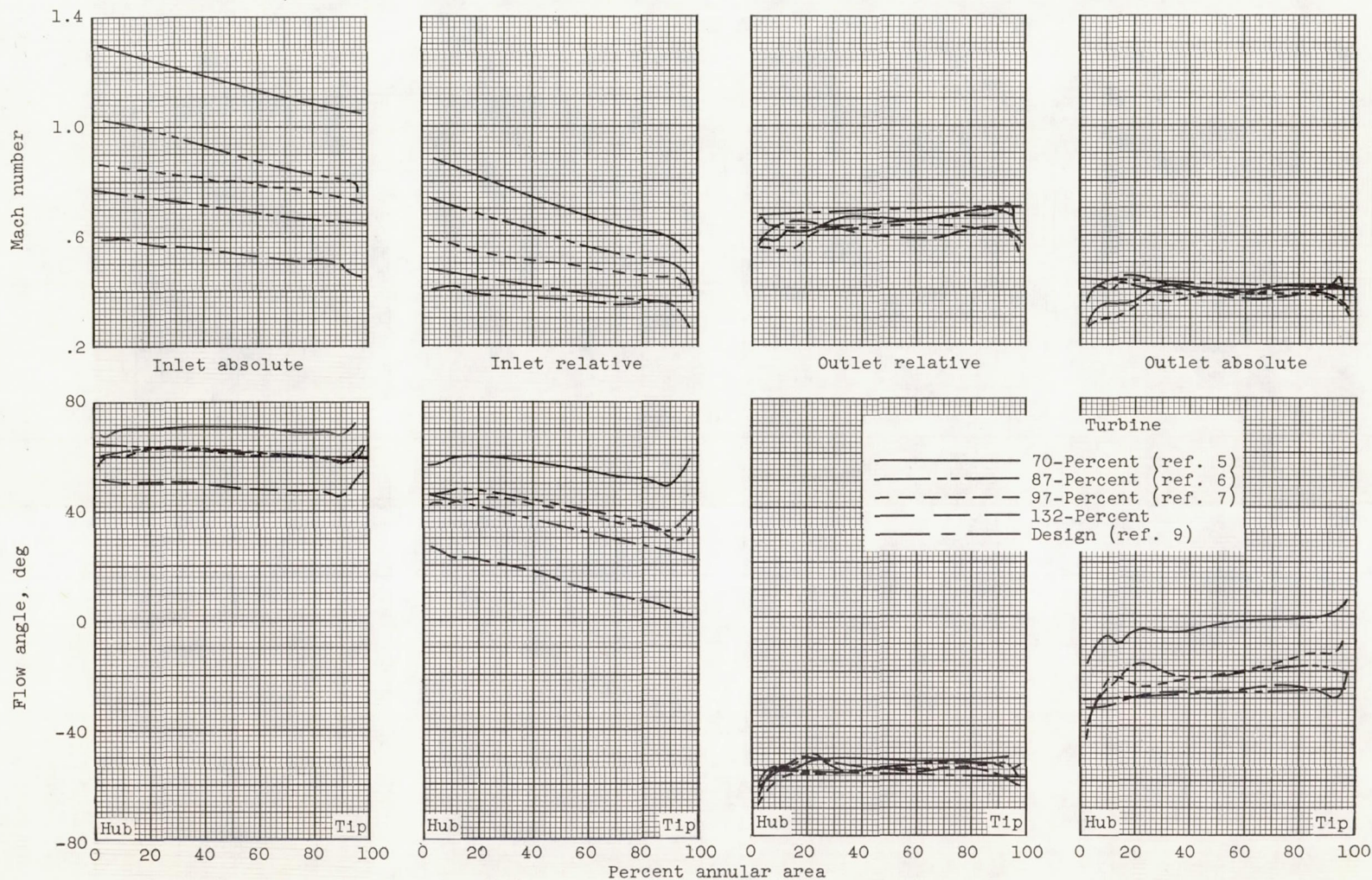
Figure 5. - Variation of absolute and relative Mach number and flow angle at rotor inlet and outlet with annular area.
