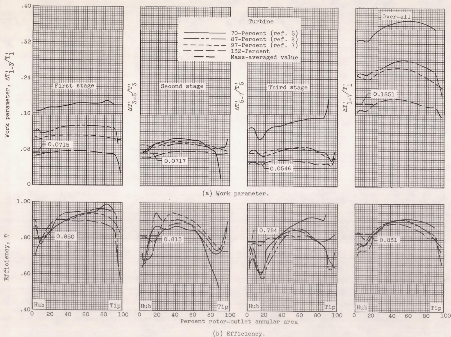
Figure 4. - Variation of stage and over-all work and efficiency with annular area at rotor outlets.
