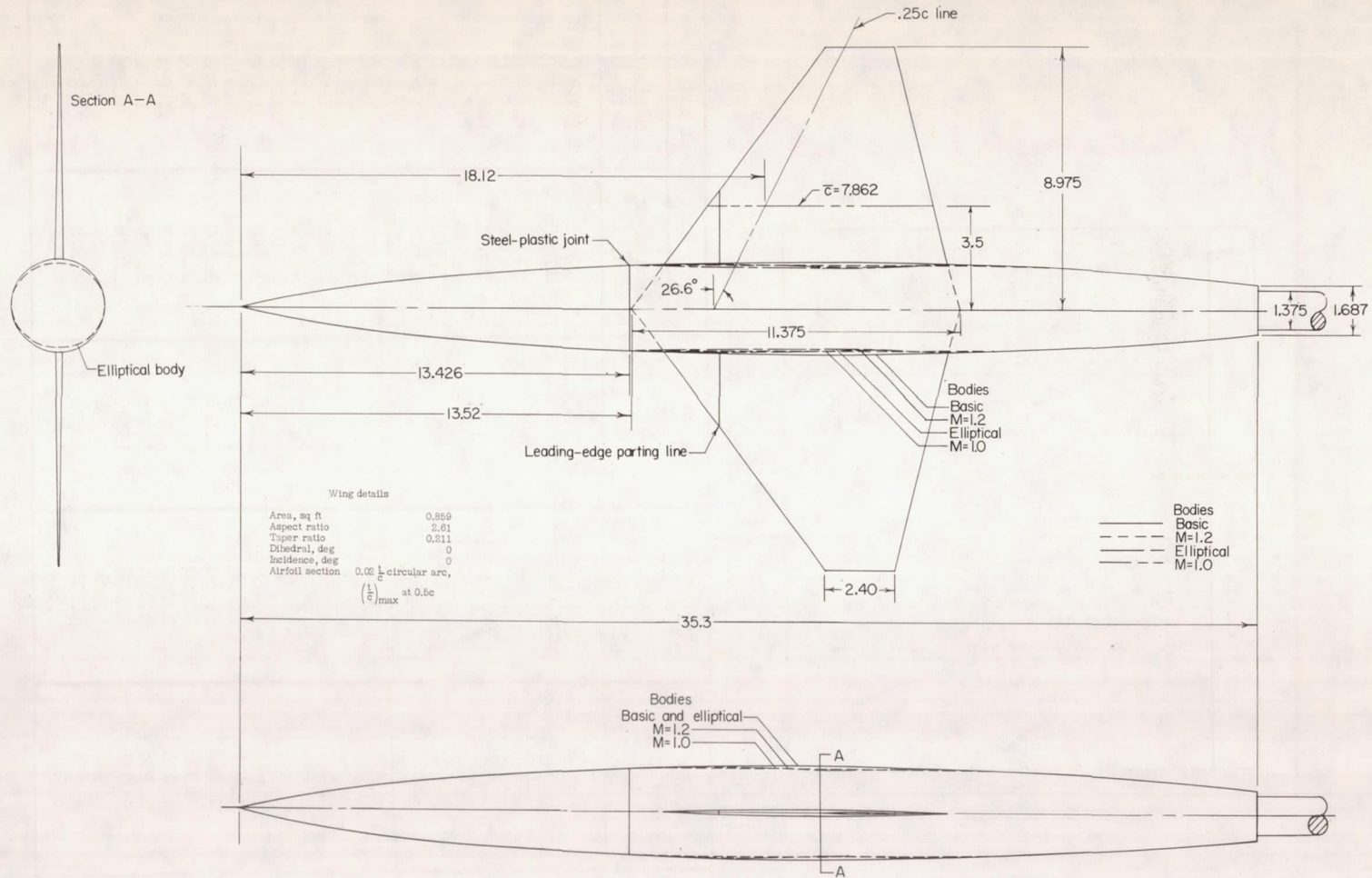
(a) Wing-body combinations.
