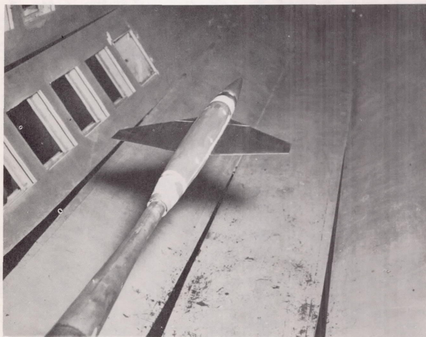
Figure 2.- The 0.02t/c wing—basic-body combination mounted in the slotted test section of the Langley 8-foot transonic tunnel.
