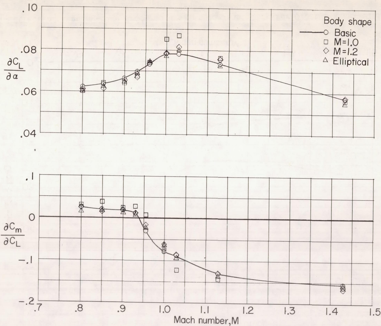
Figure 10.- Variation with Mach number of lift-curve and pitching-moment-curve slopes for the 0.02t/c plane-wing configurations. C_L = 0 .
